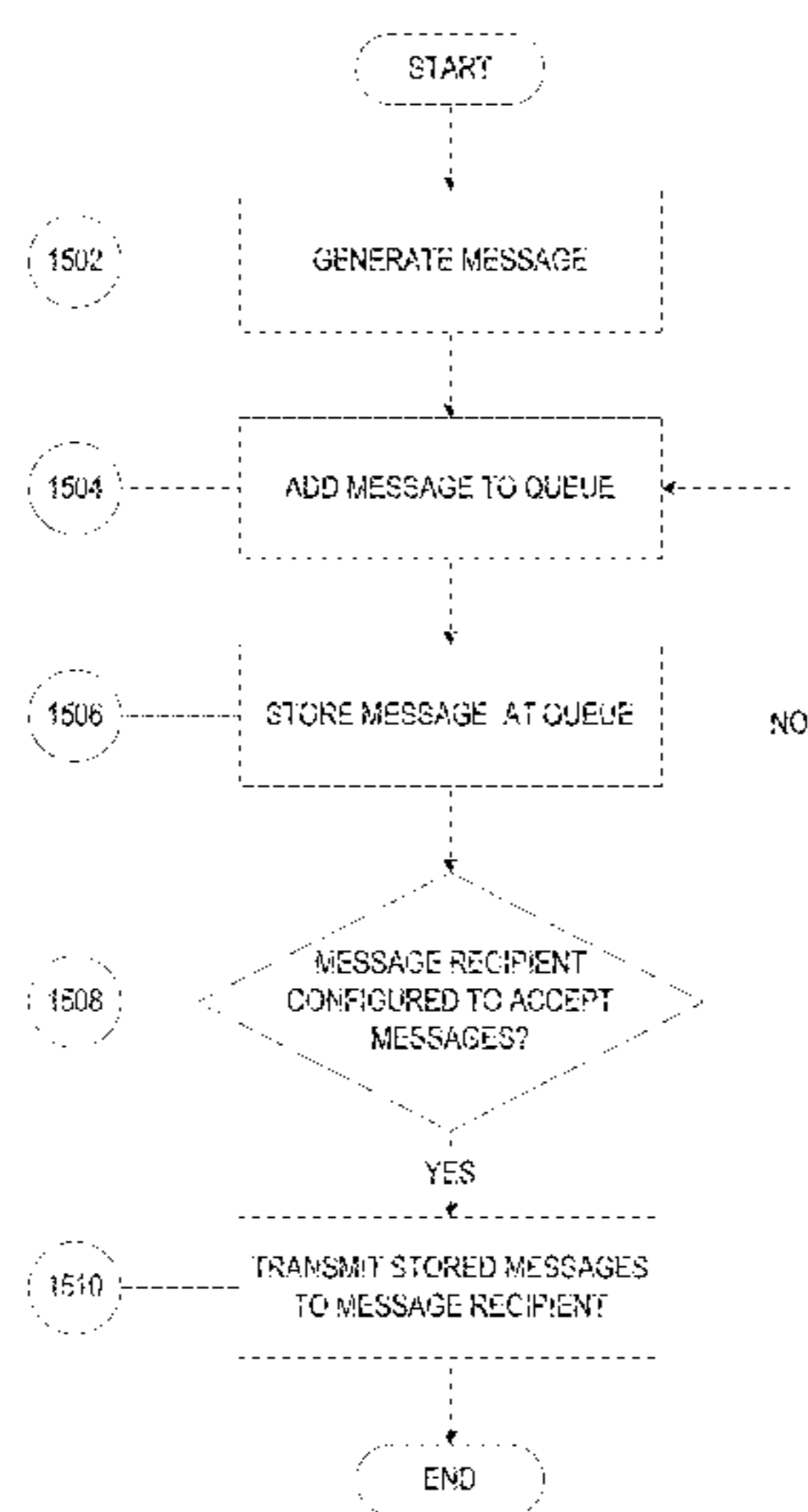
EXEMPLARY QUEUING PROCESS
