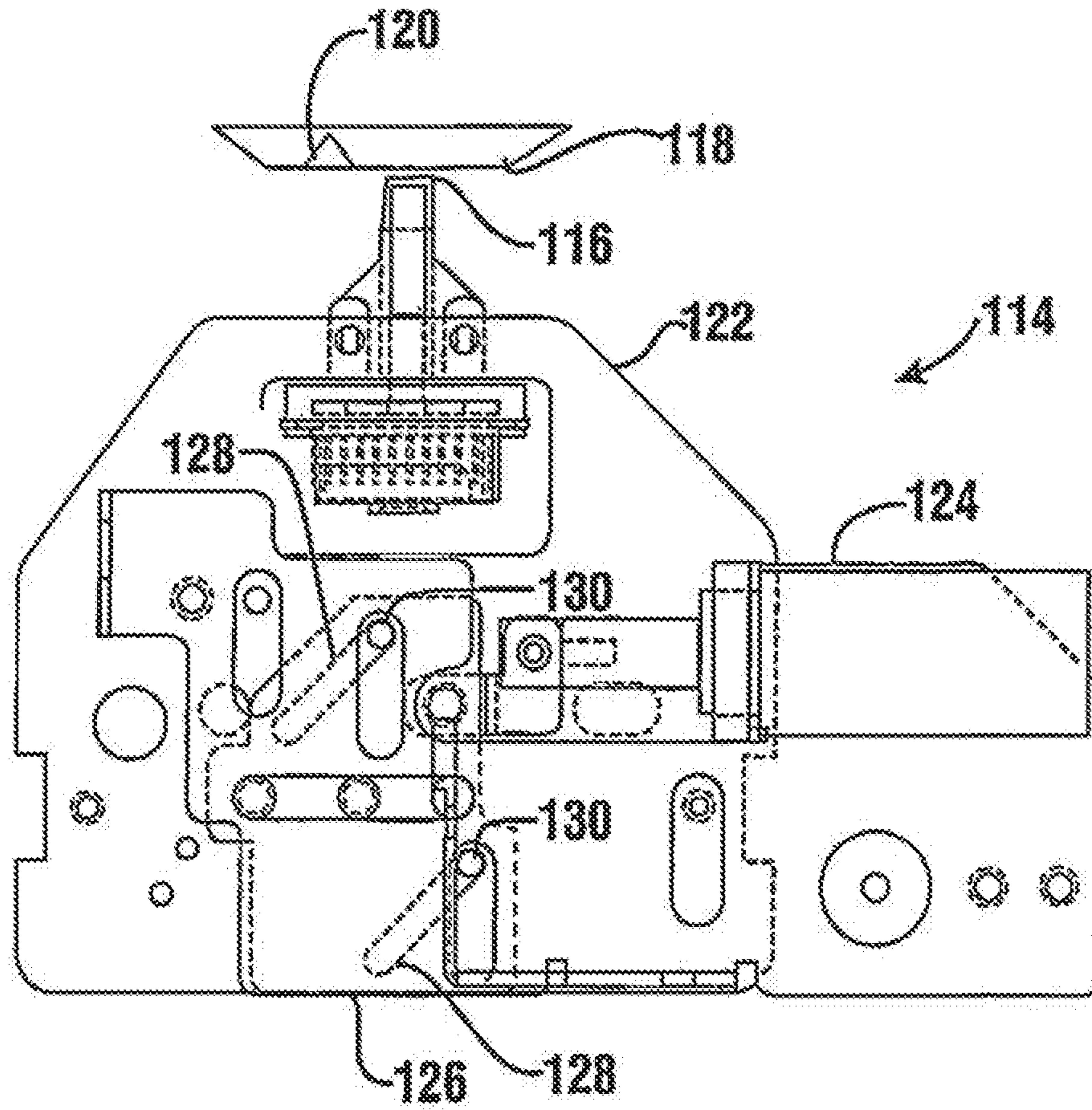
Printing Position
