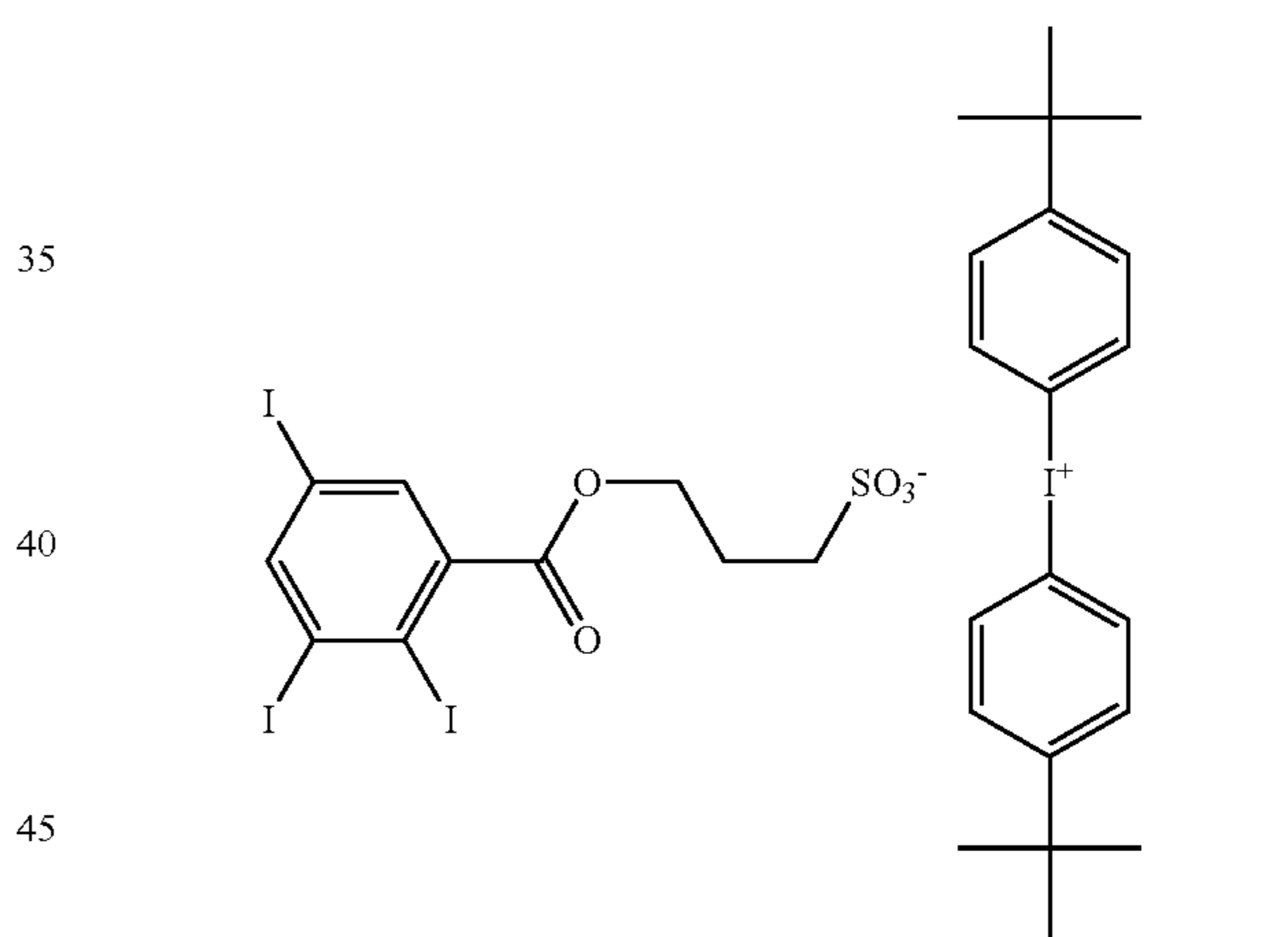
Iodonium salt 2
