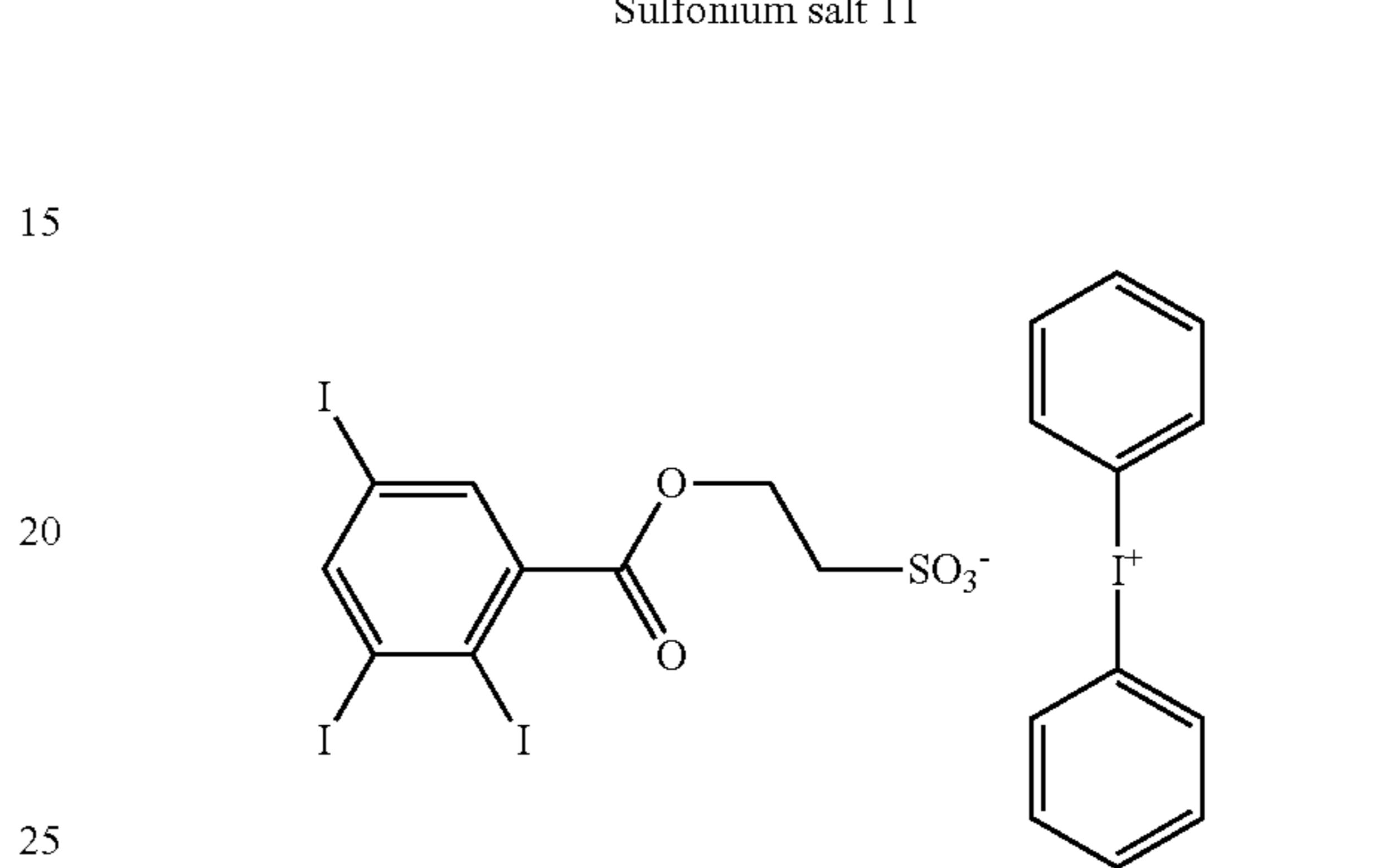
Iodonium salt 1
