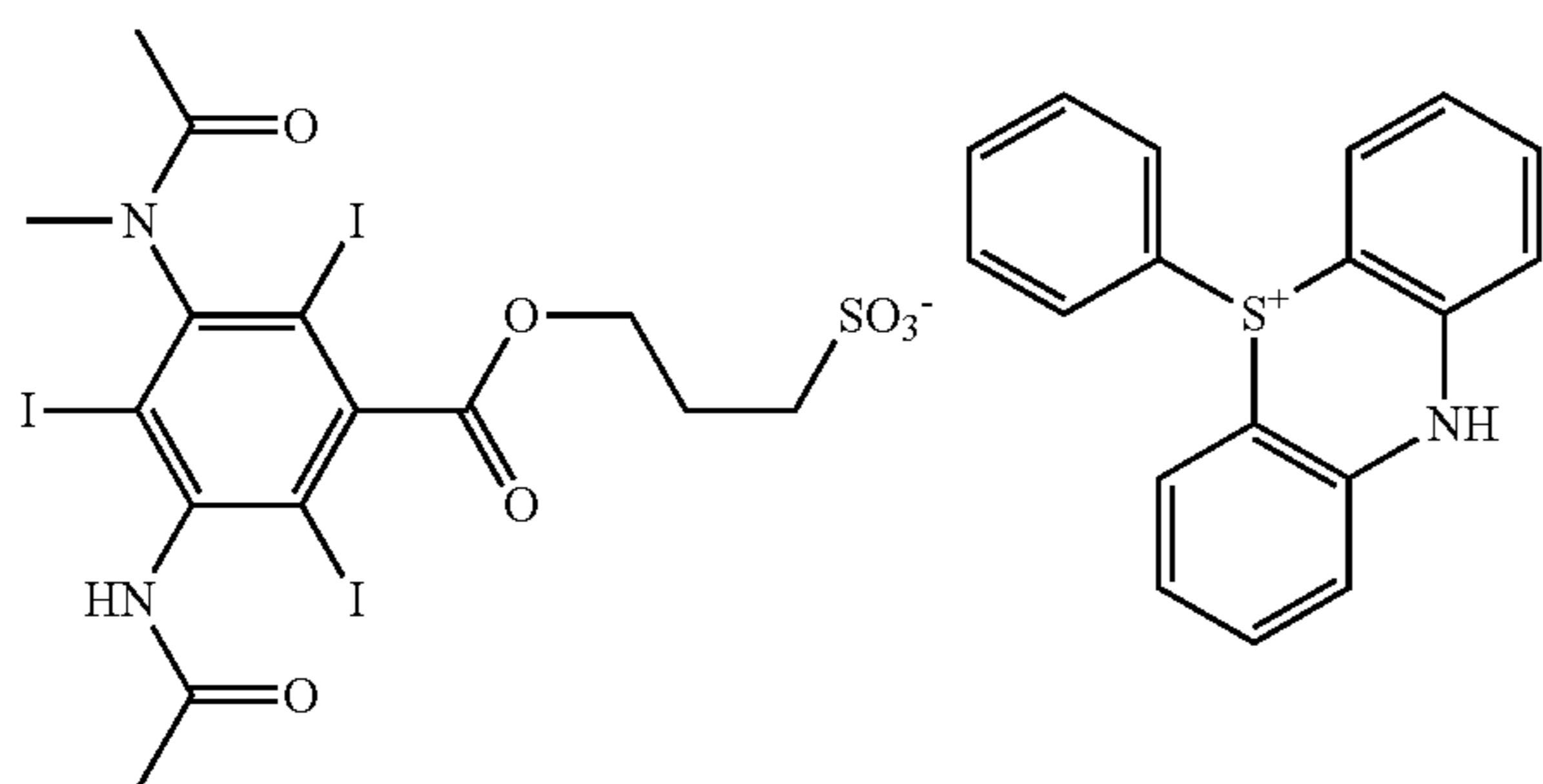
Sulfonium salt 8
