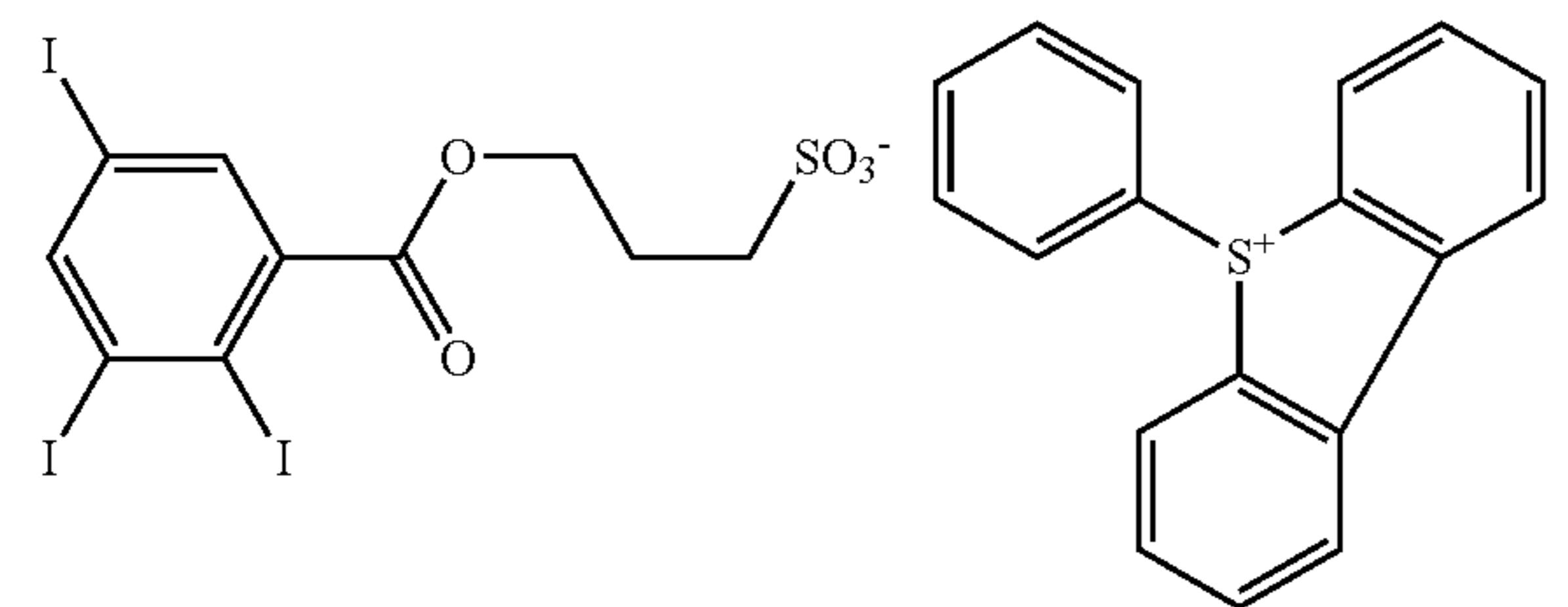
Sulfonium salt 6
