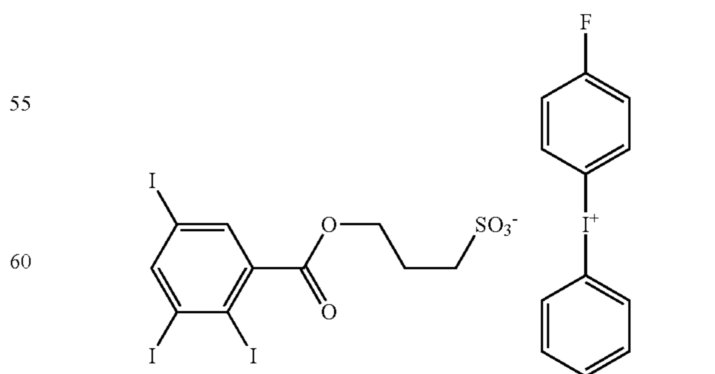
Iodonium salt 3
