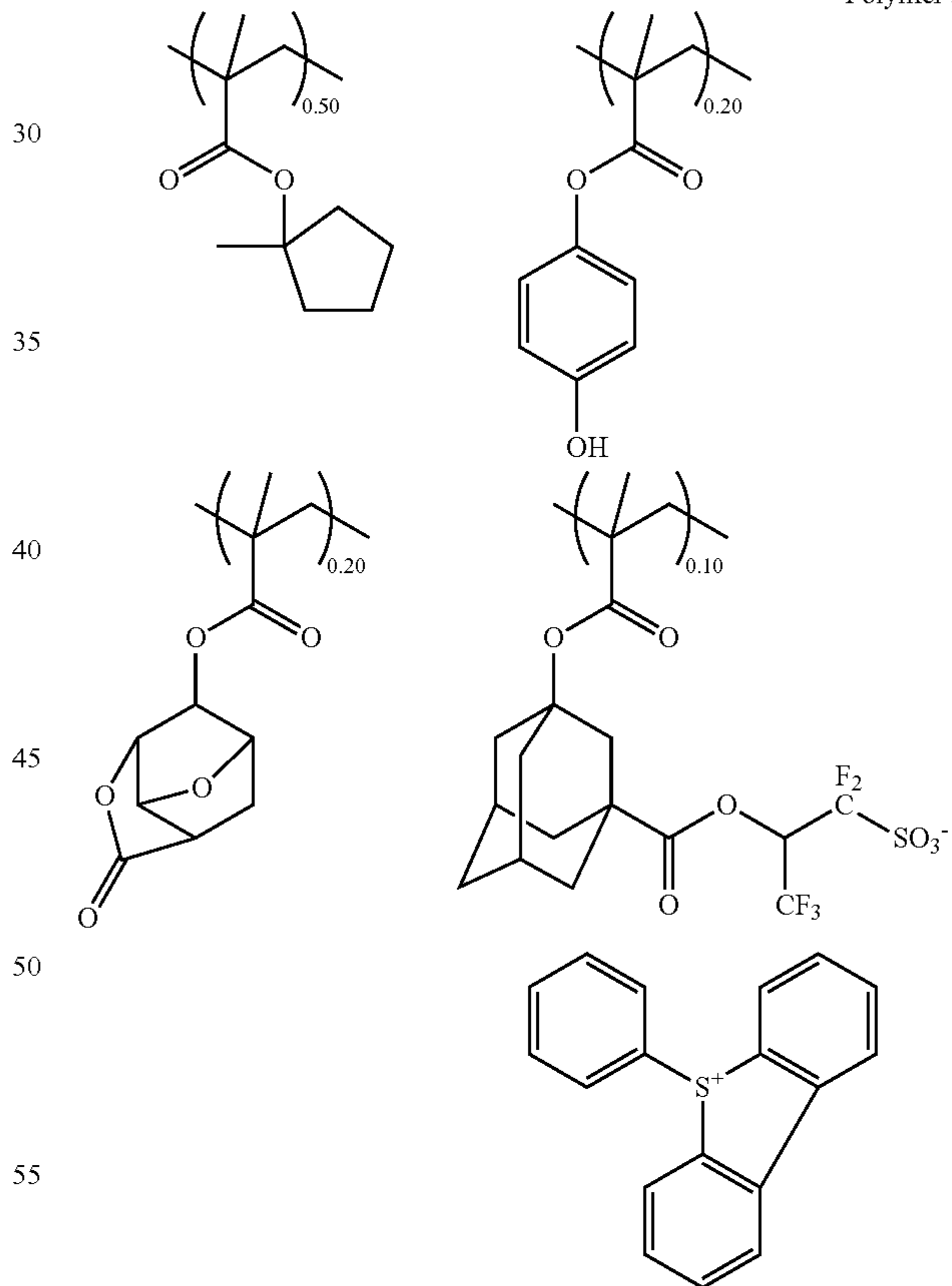
Polymer 3
