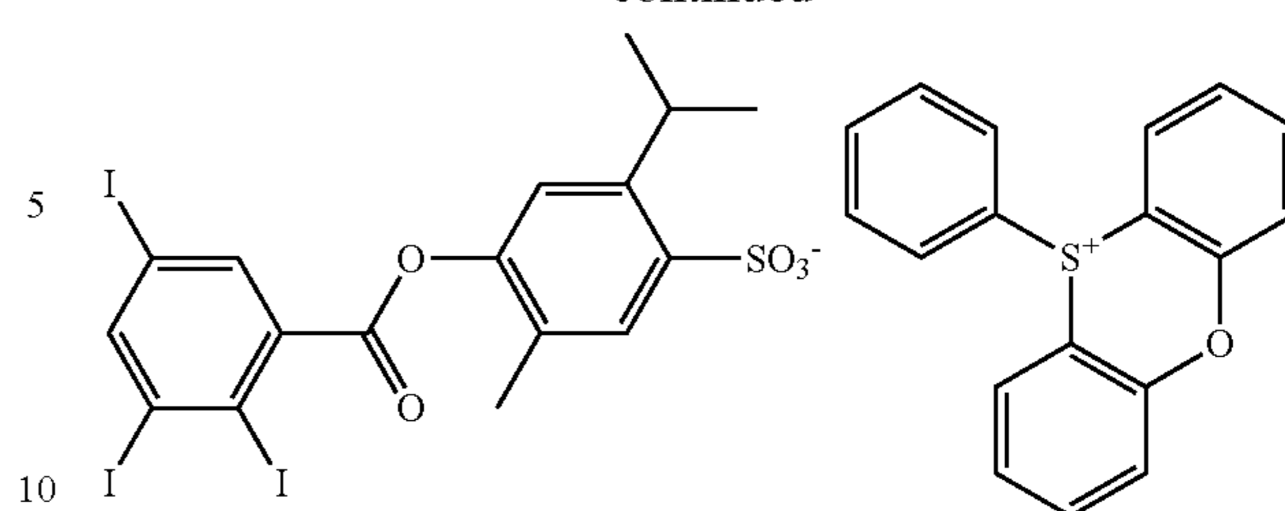
Sulfonium salt 11
