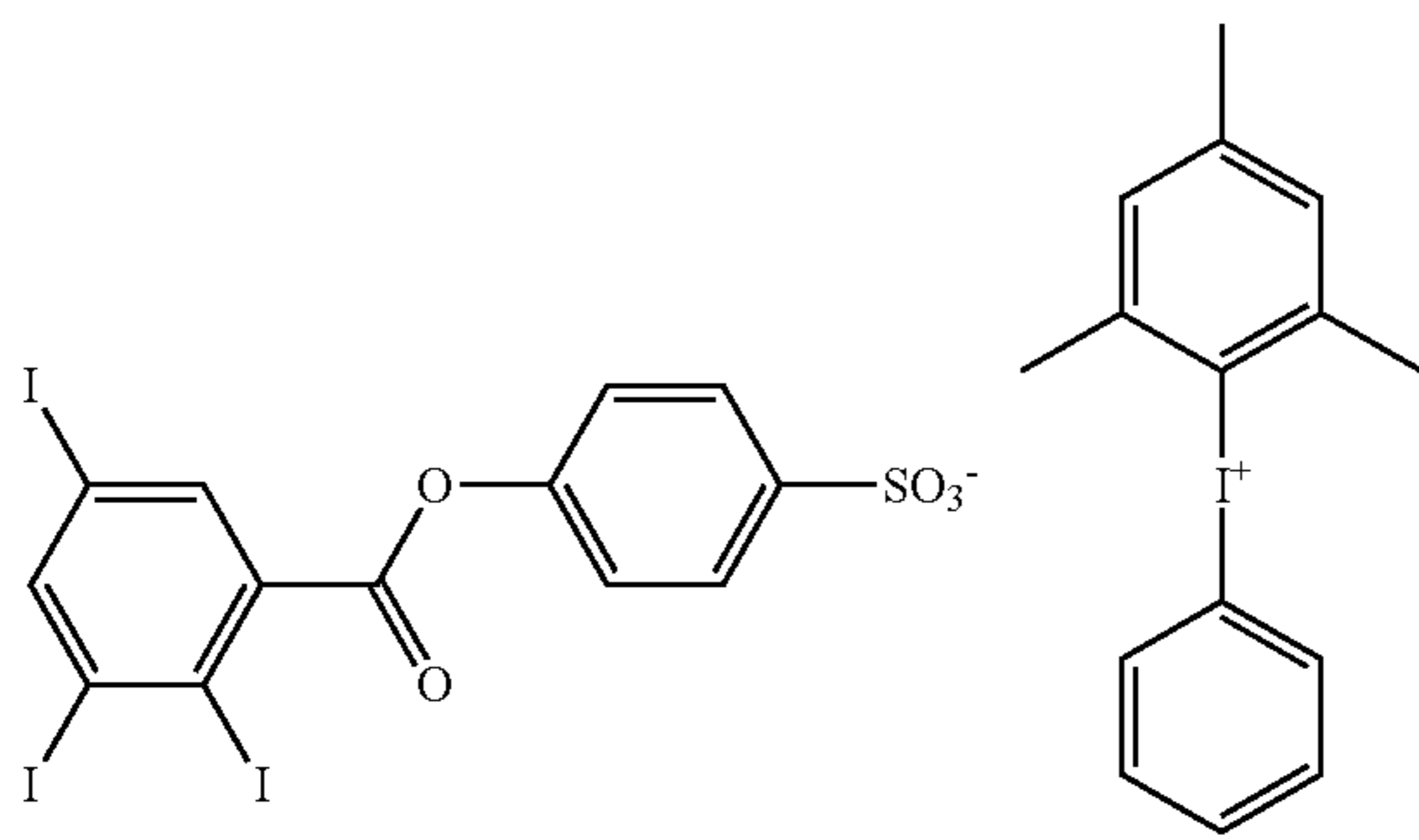
Iodonium salt 4
