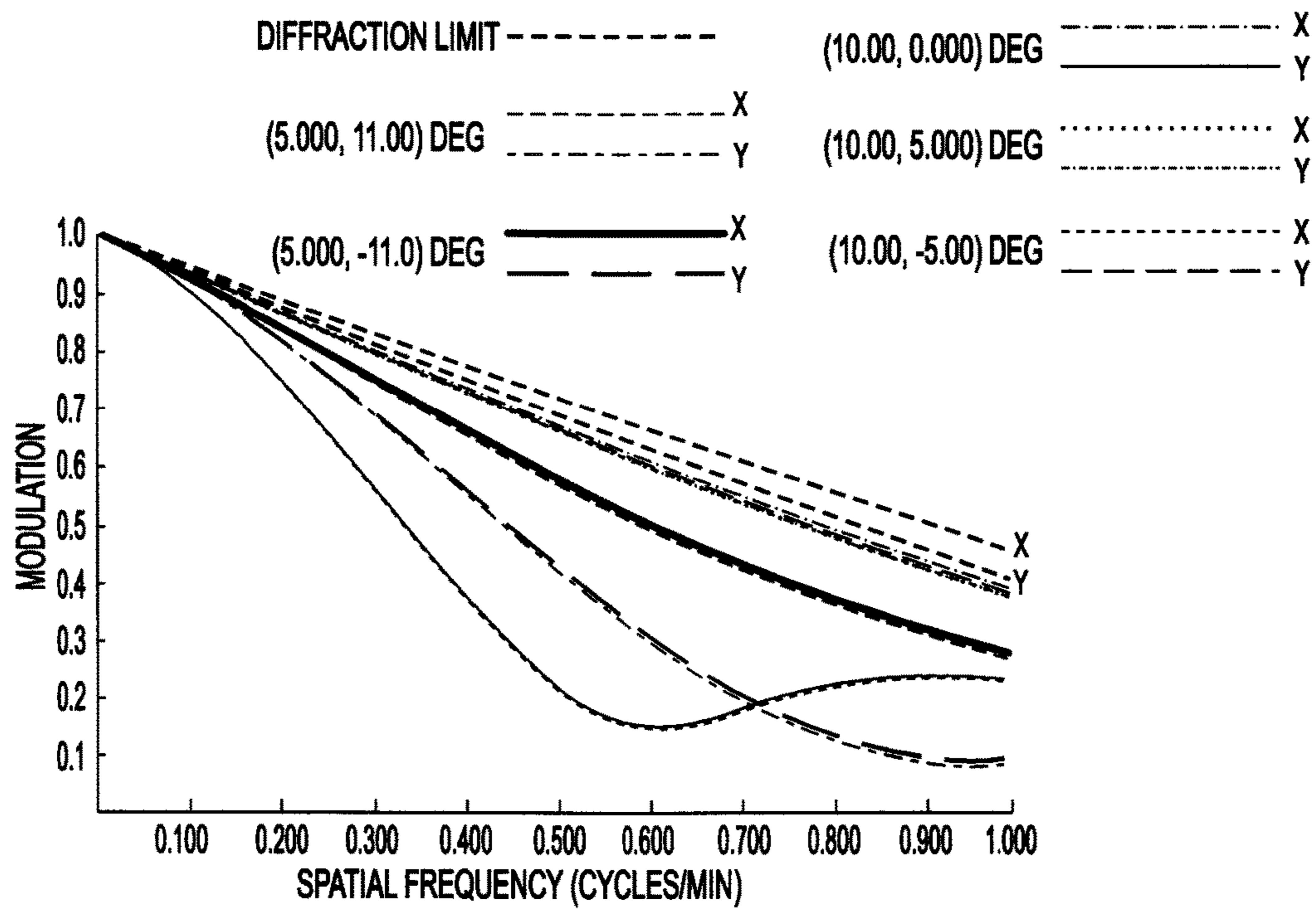
FIG. 13D
