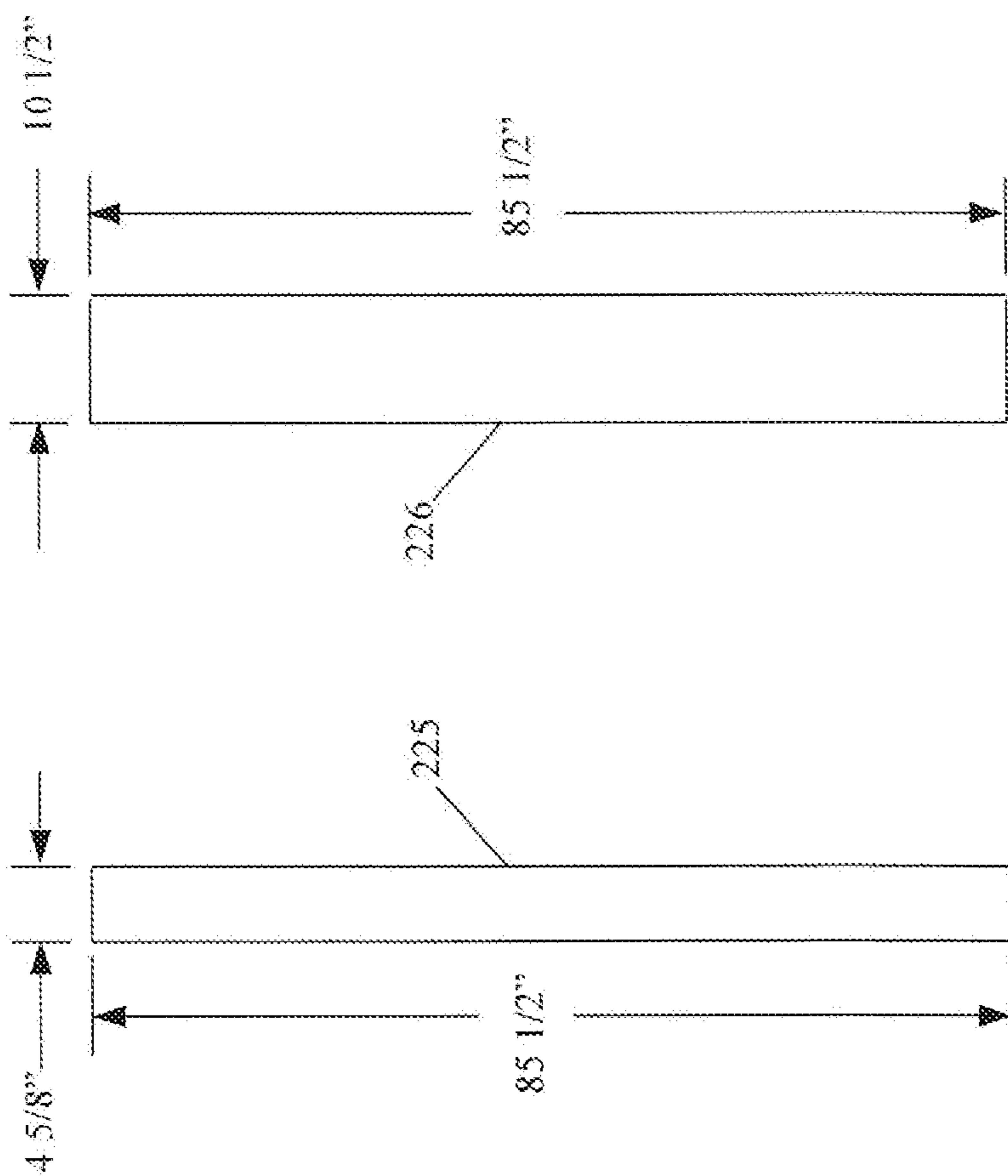
FIG. 16A (Precut Drywall Piece)
