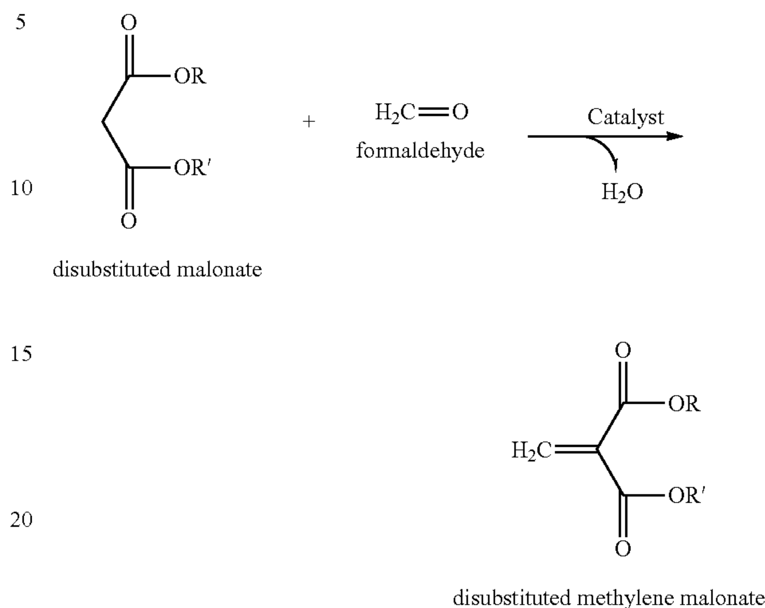
Schematic 1. Knoevenagel reaction with formaldehyde for the synthesis of a methylene malonate.
