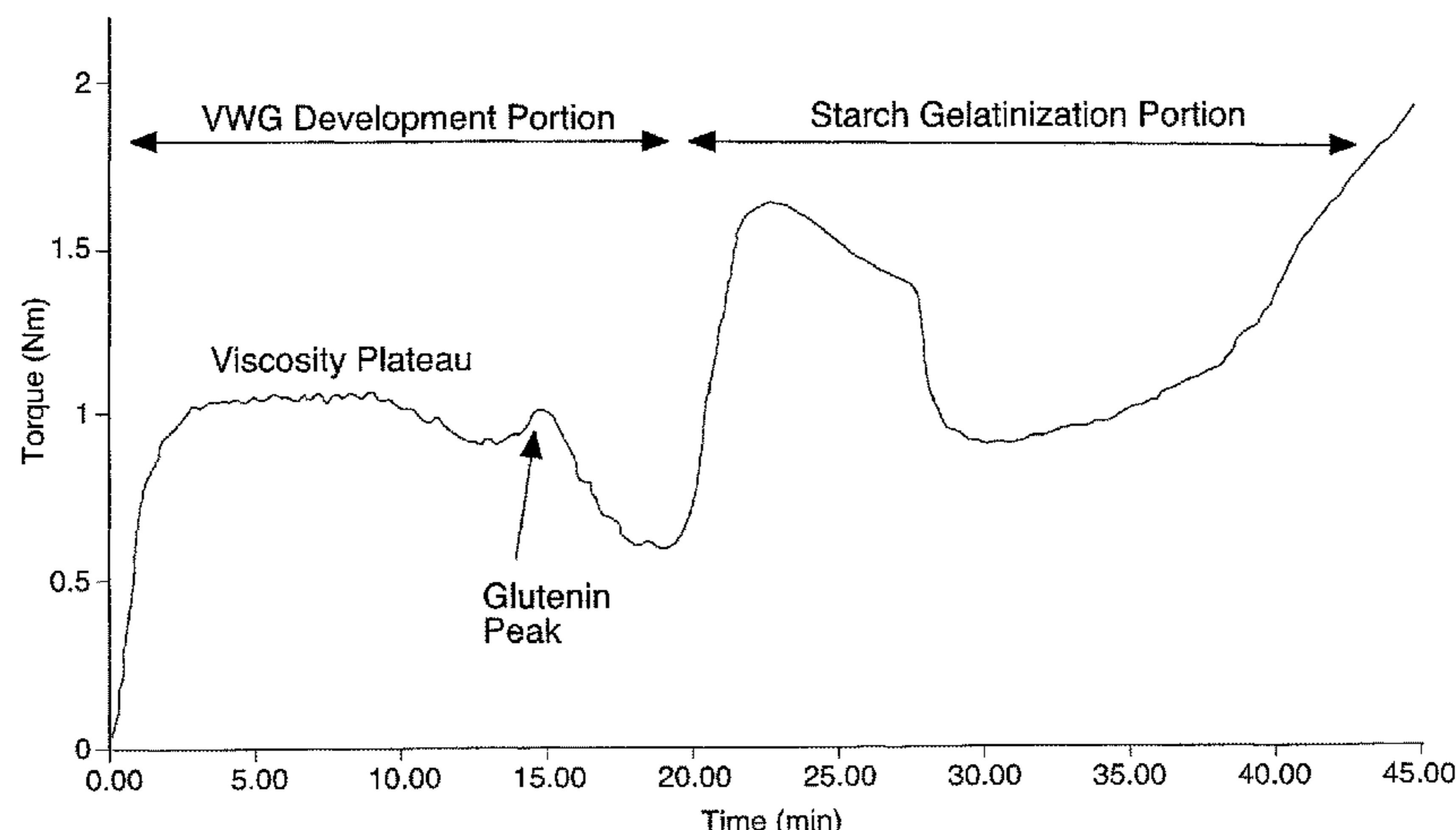
40% VWG / 60% Wheat Starch Rheology Curve Chopin Mixolab, Chopin+ Protocol
