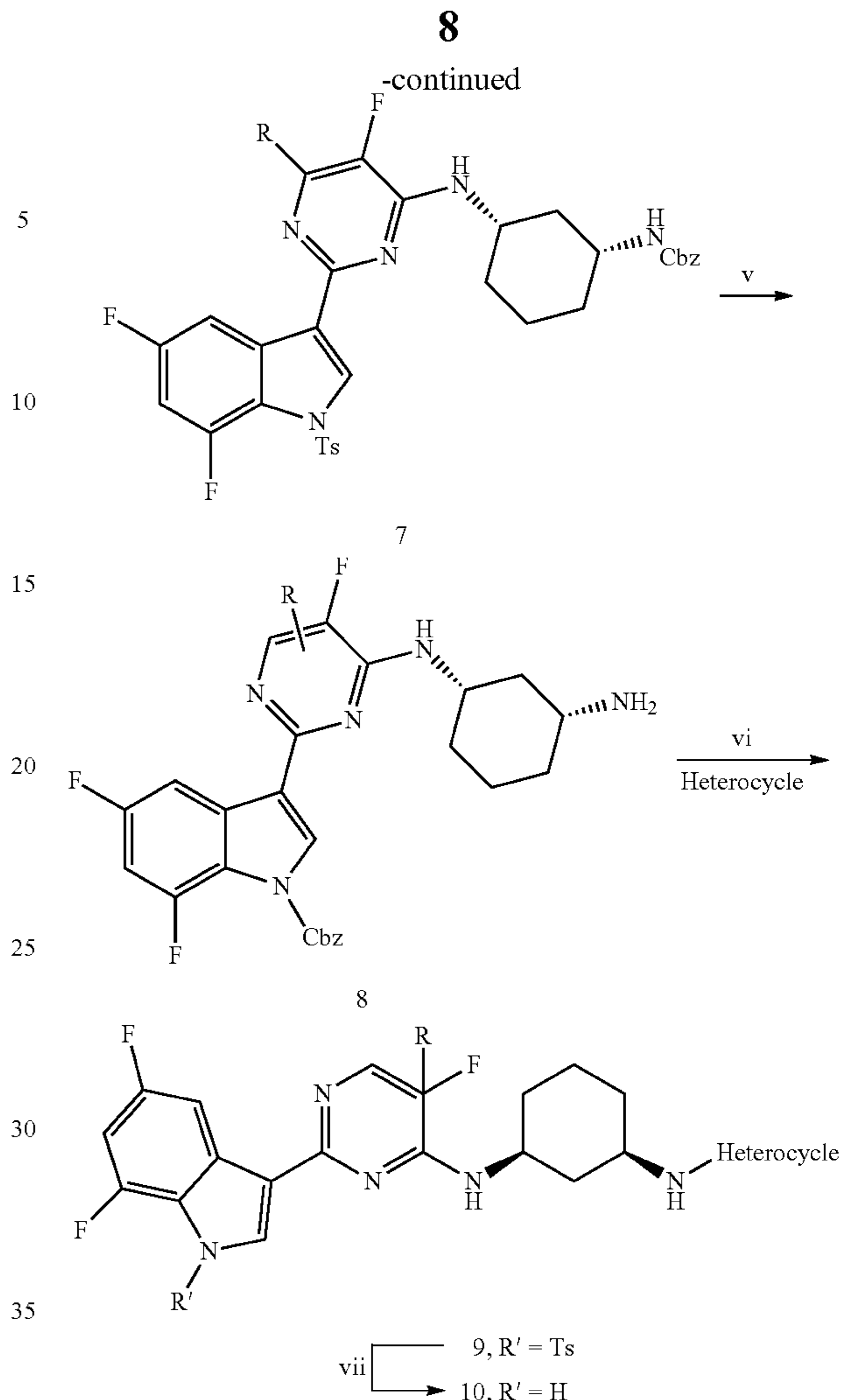
Scheme 2. General Scheme toward products of formula (I). Preparation of 10.
