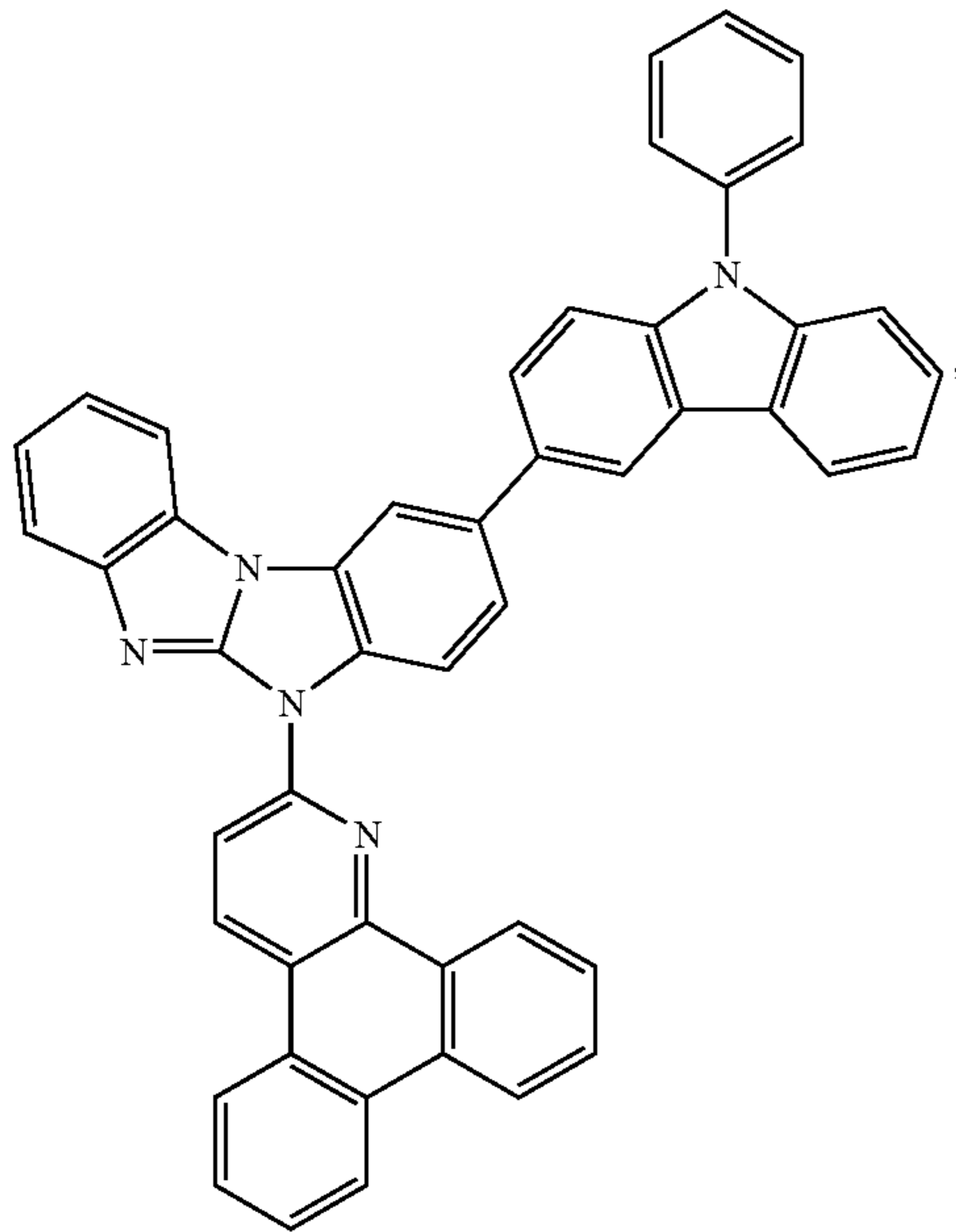
Compound 90
