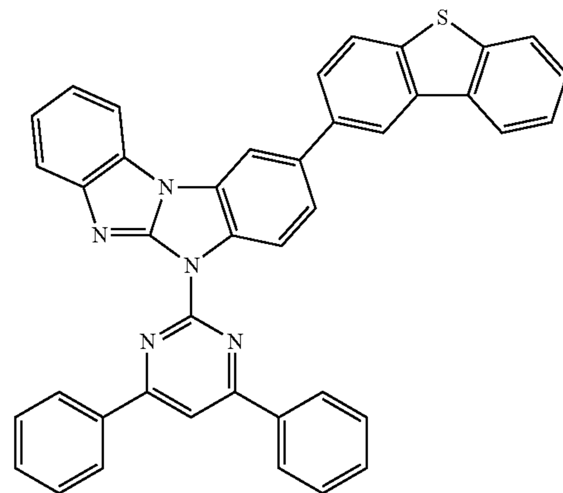
Compound 45
