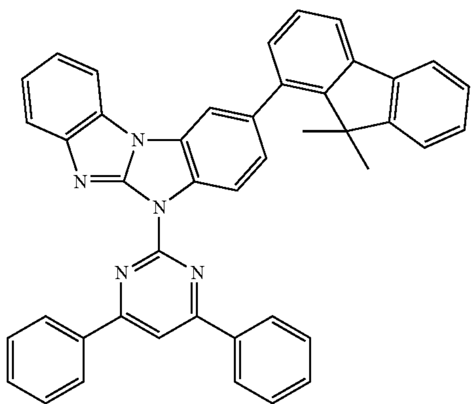
Compound 44
