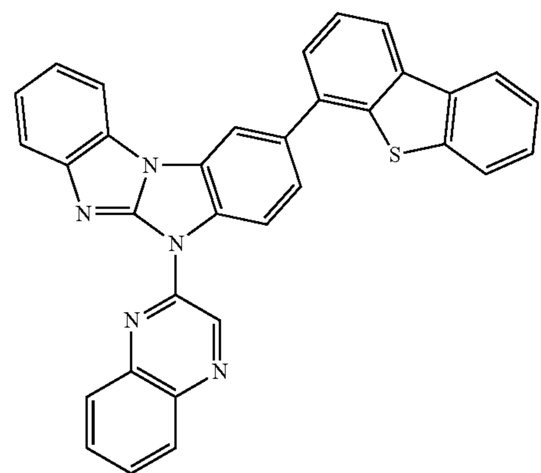
Compound 66
