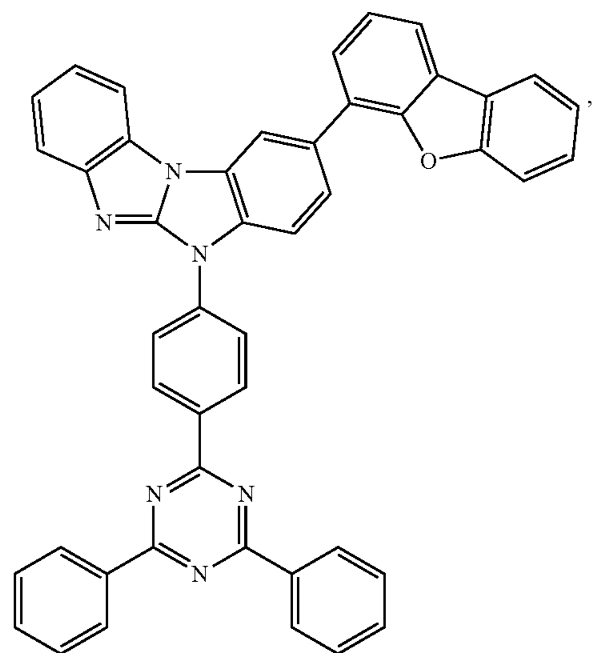
Compound 30
