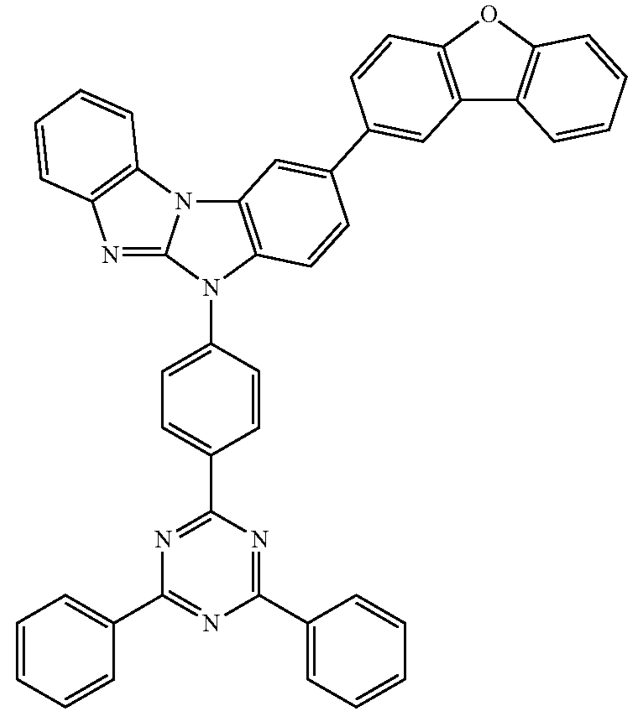
Compound 33
