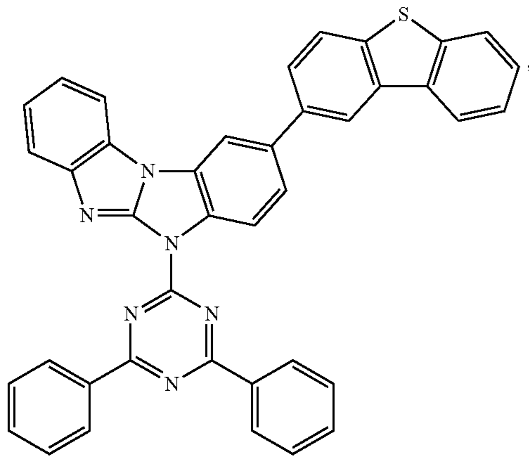
Compound 14
