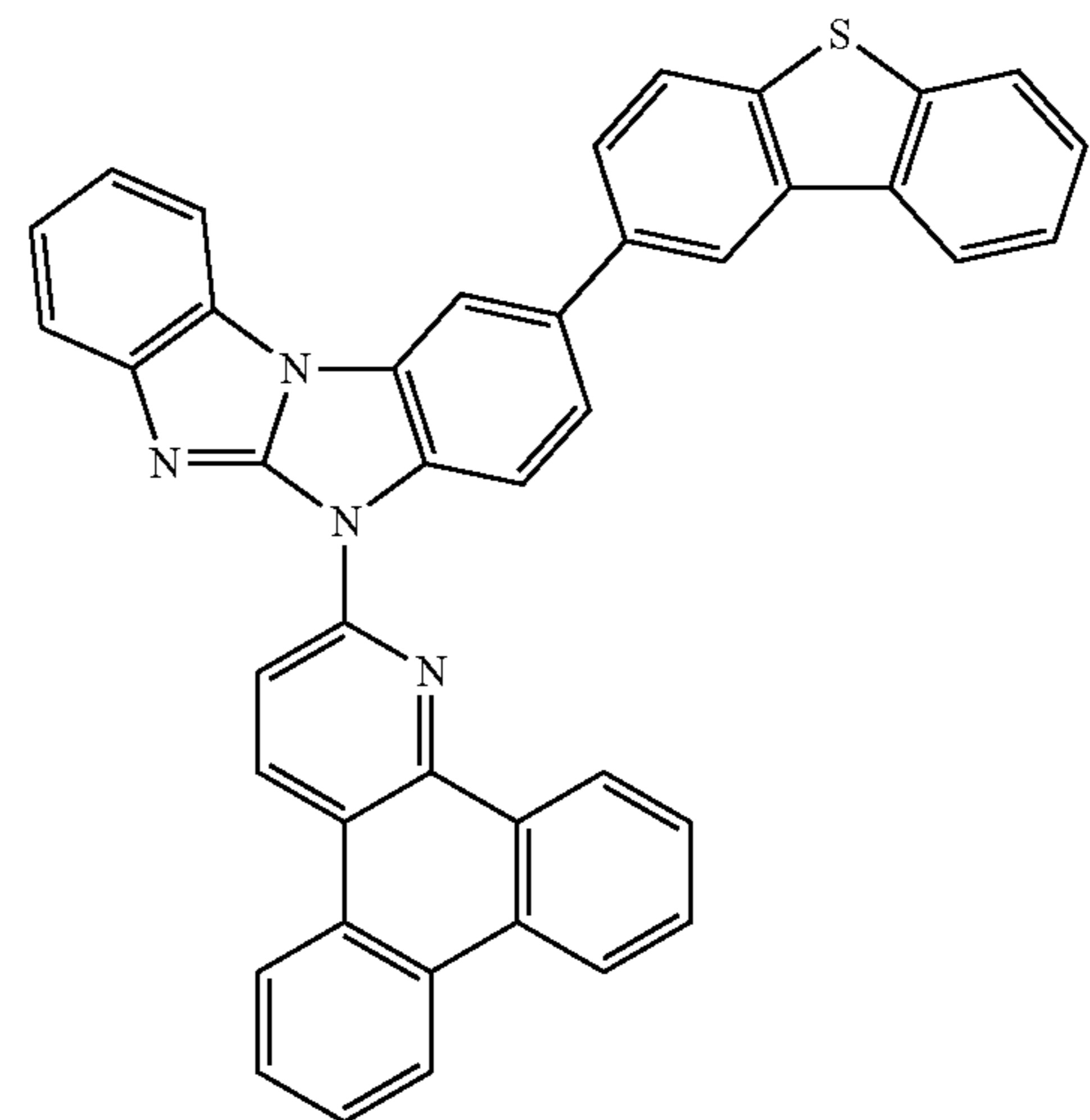
Compound 87
