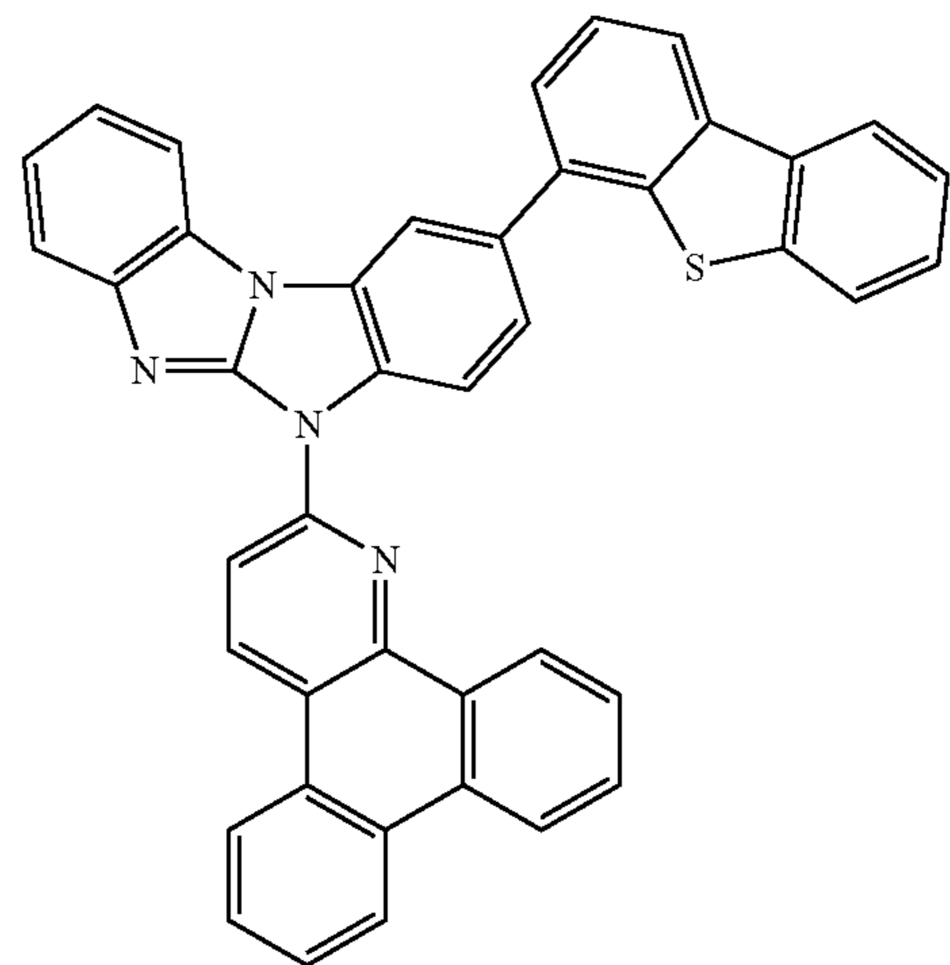
Compound 85
