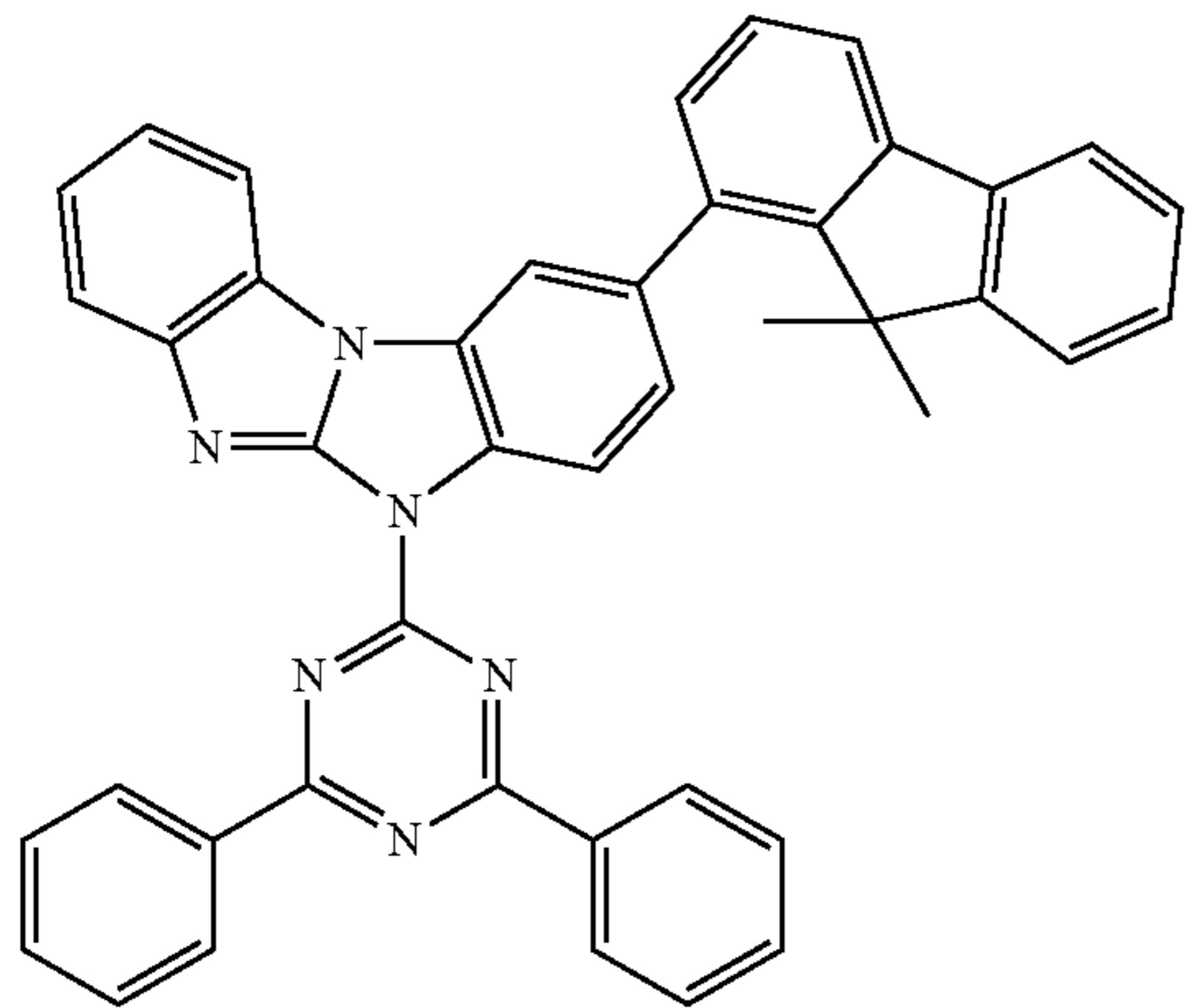
Compound 13
