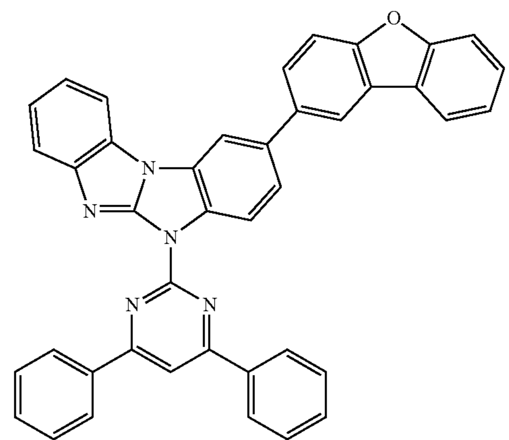
Compound 46
