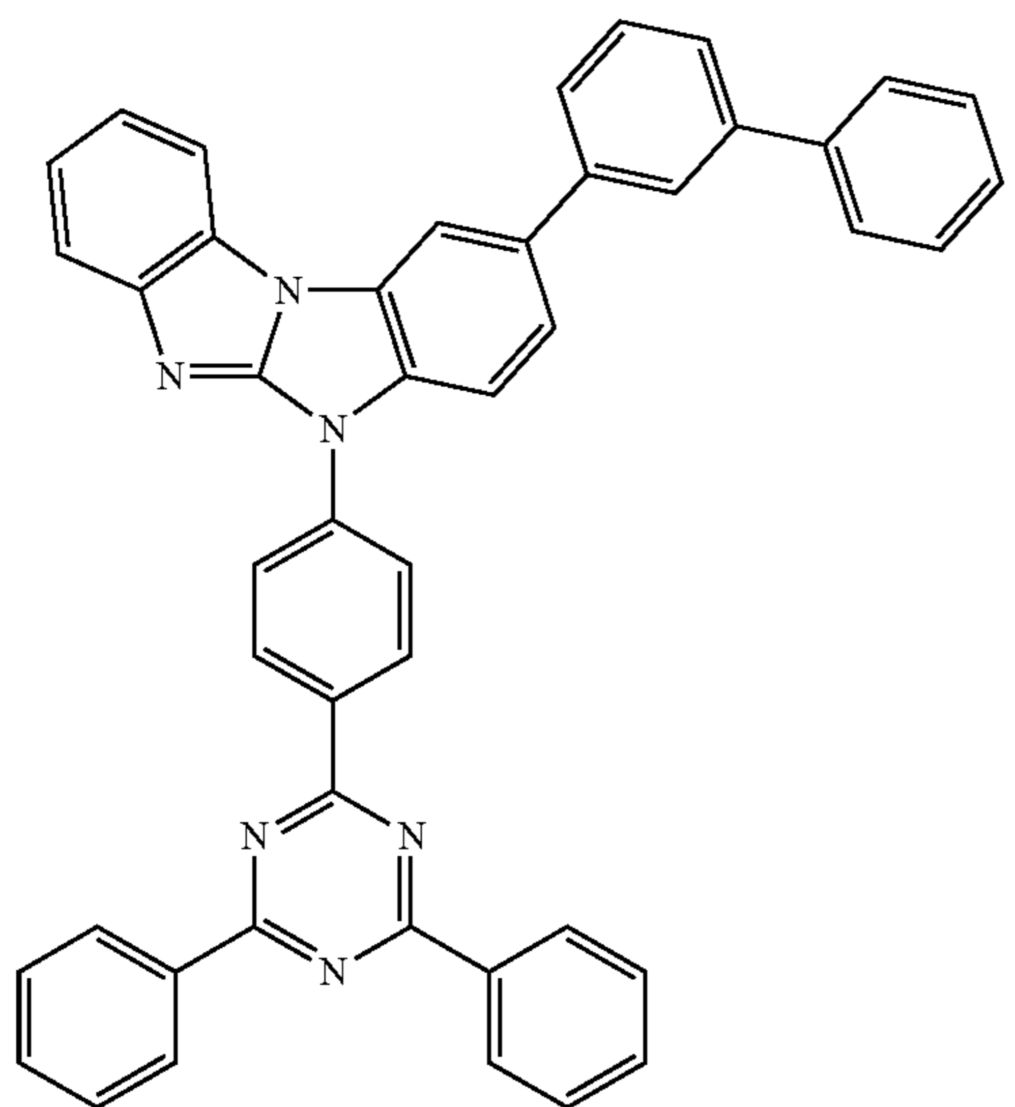
Compound 27
