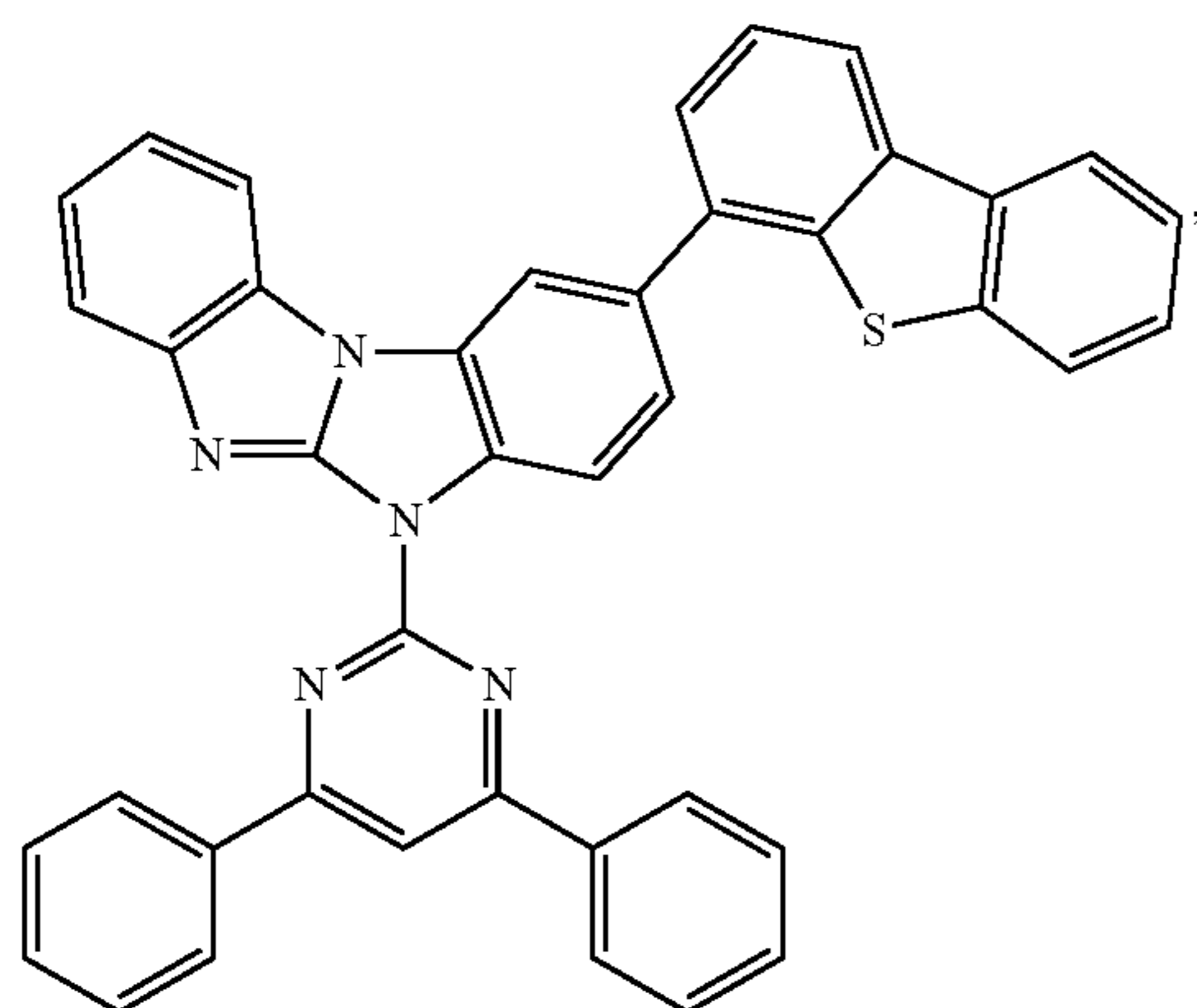
Compound 43
