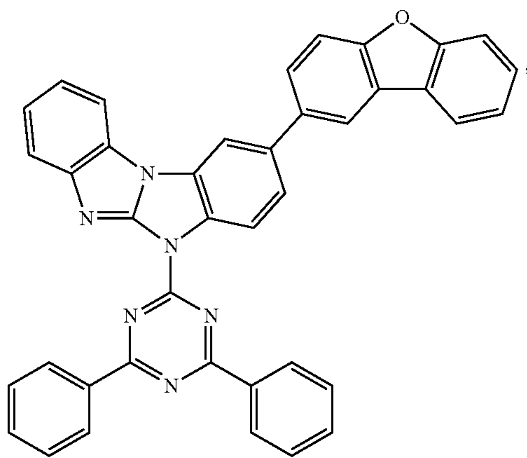
Compound 15
