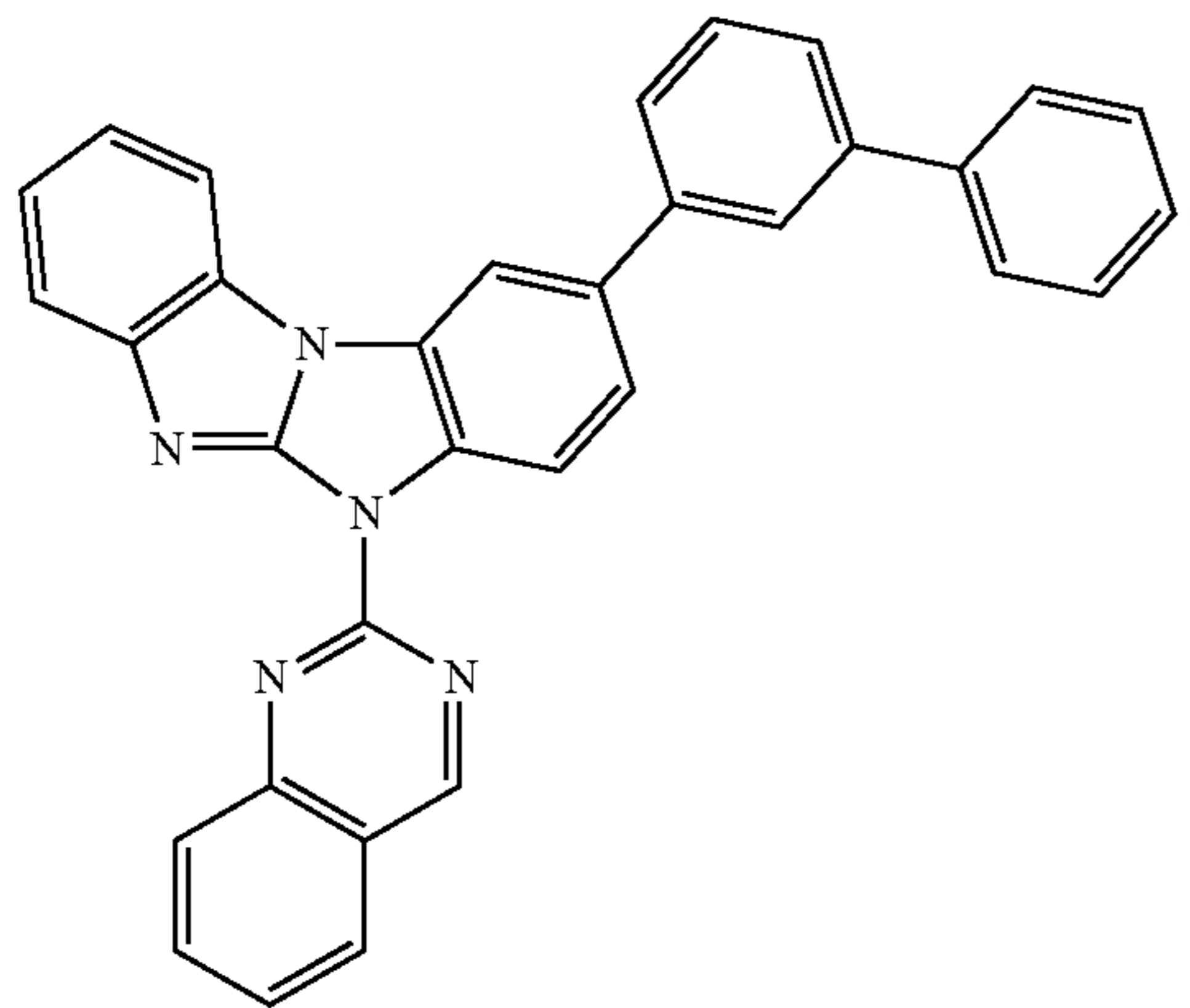
Compound 75
