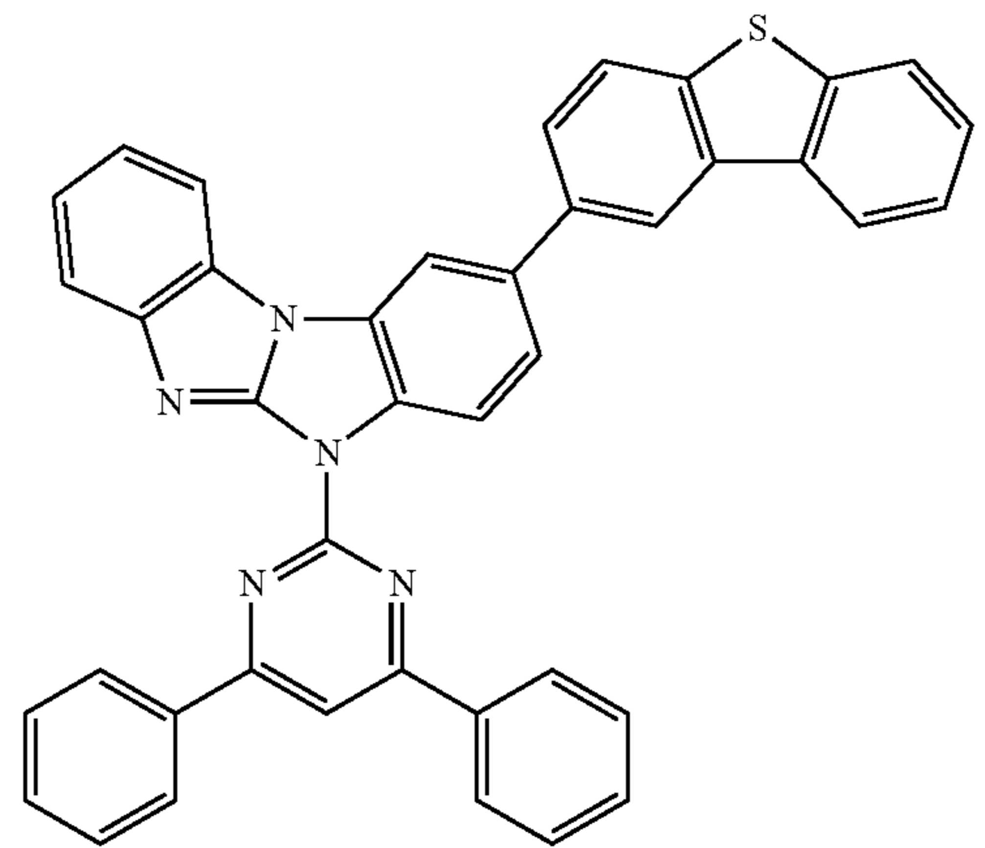
Compound 45
