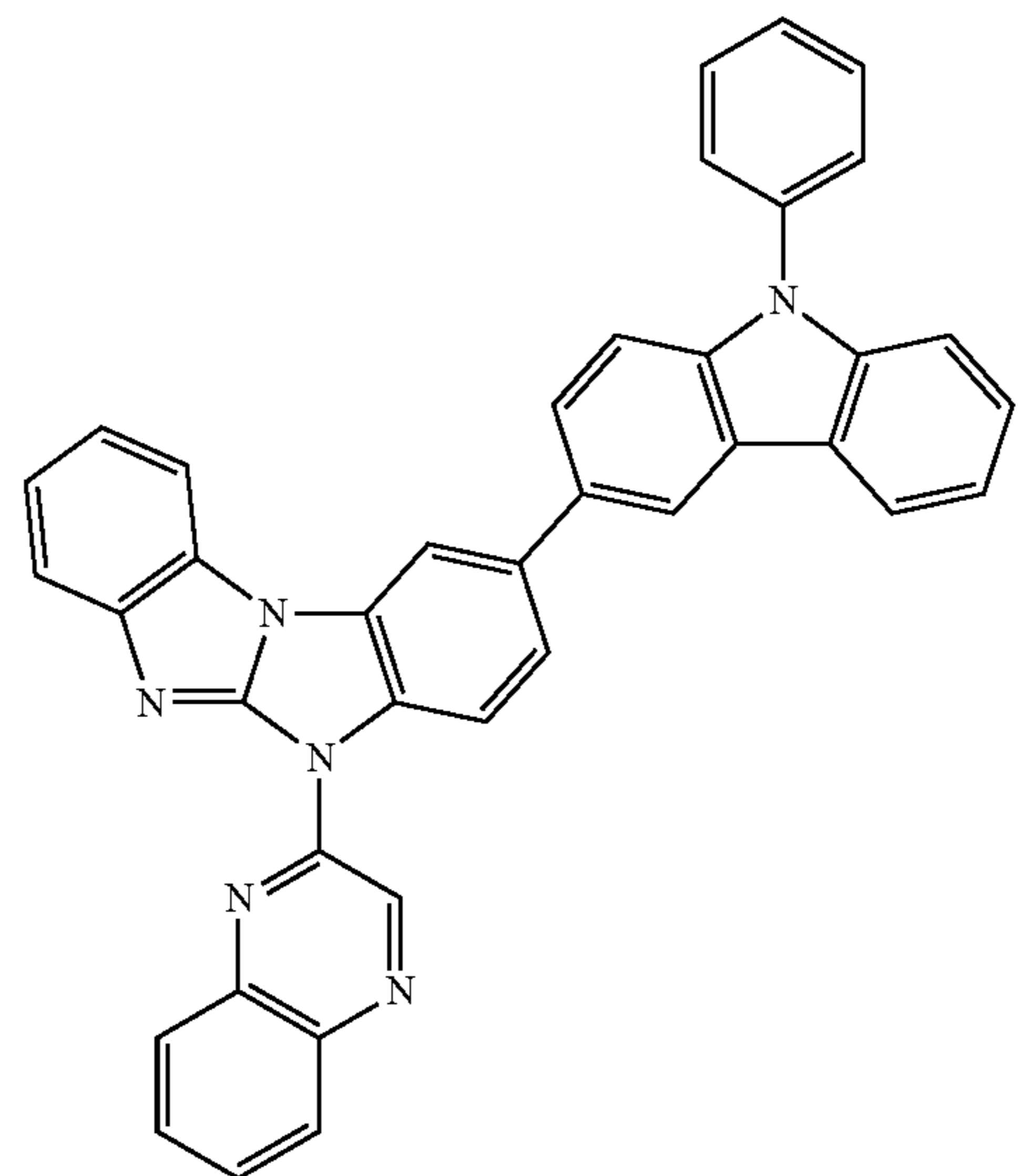
Compound 70
