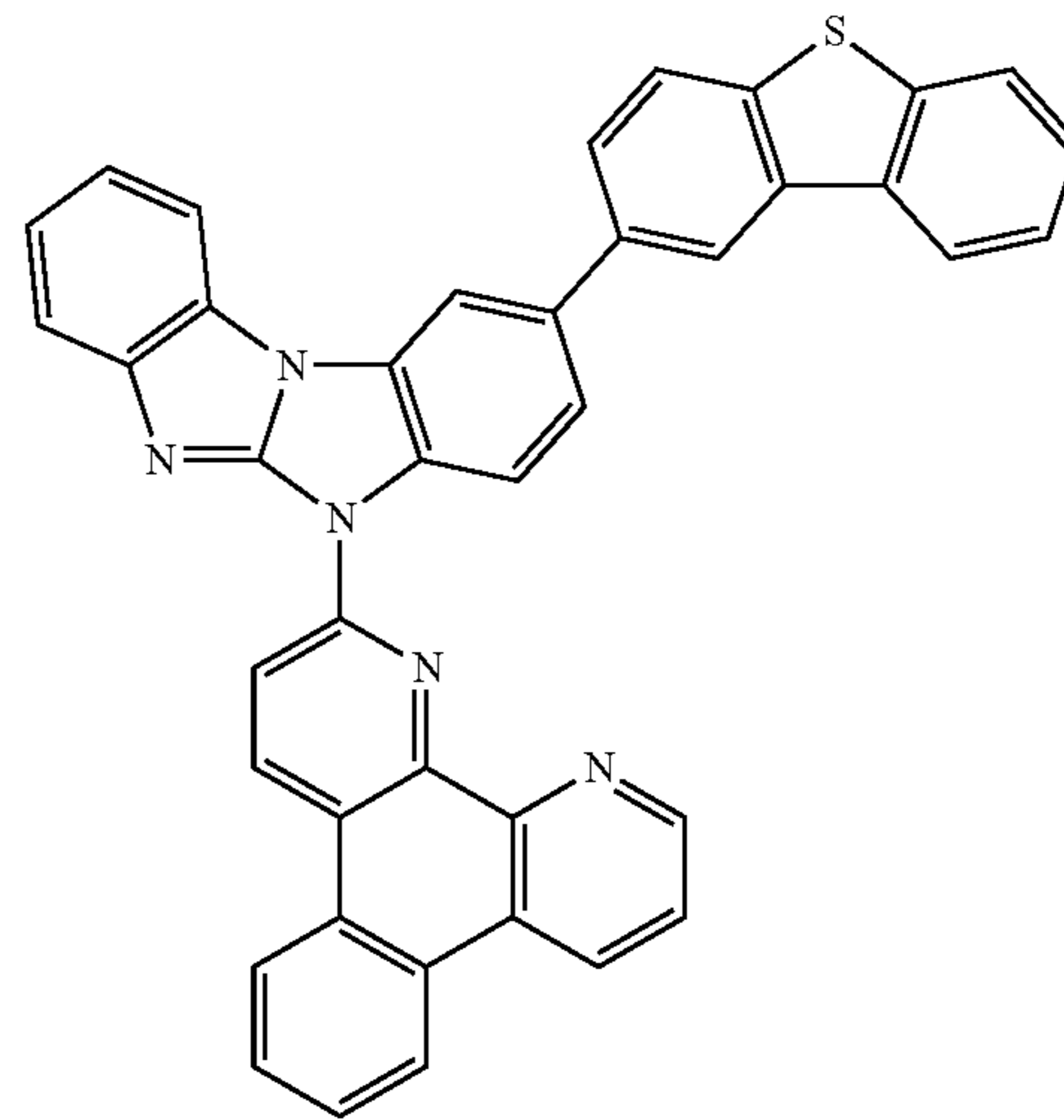
Compound 94
