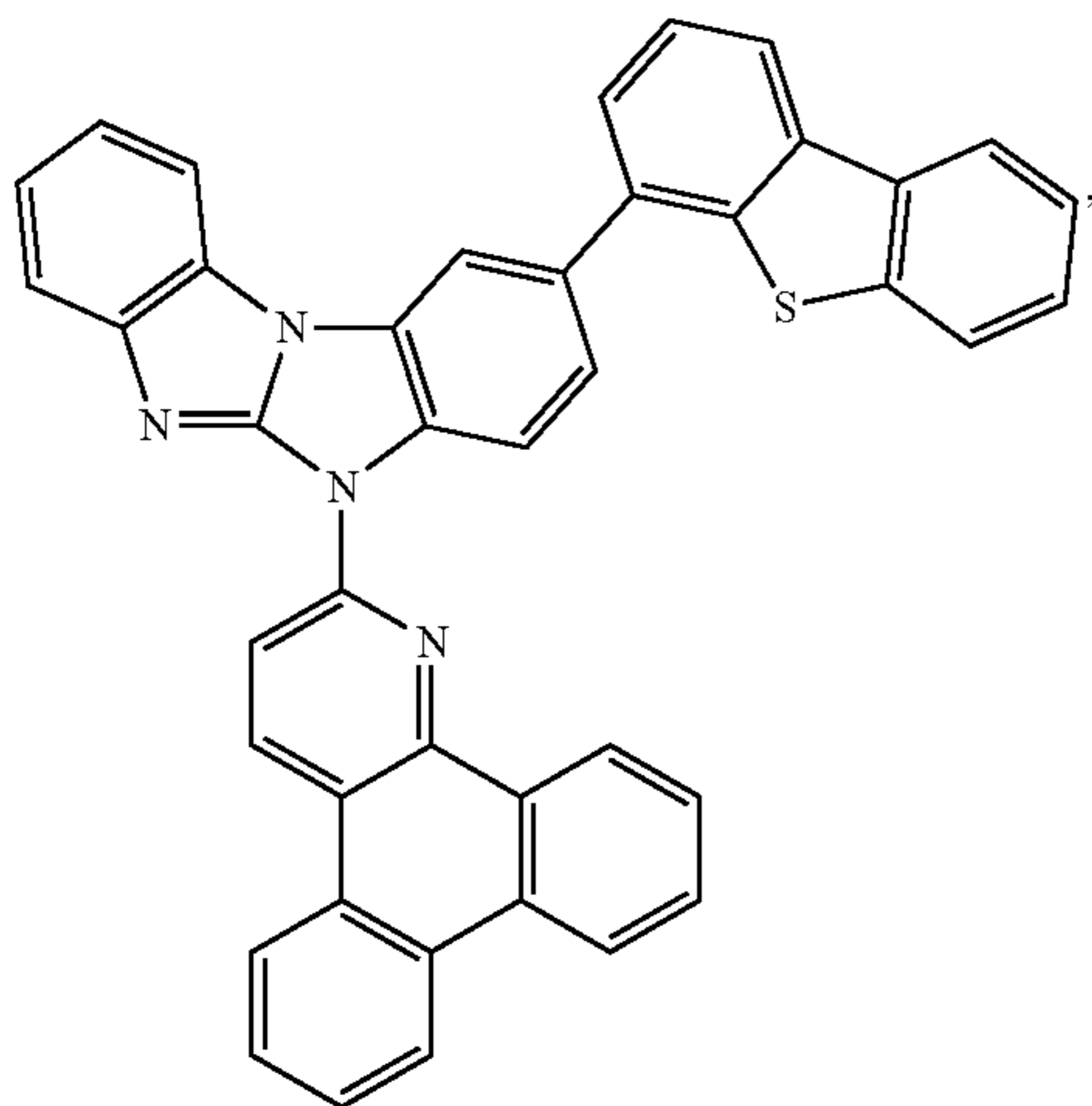
Compound 85
