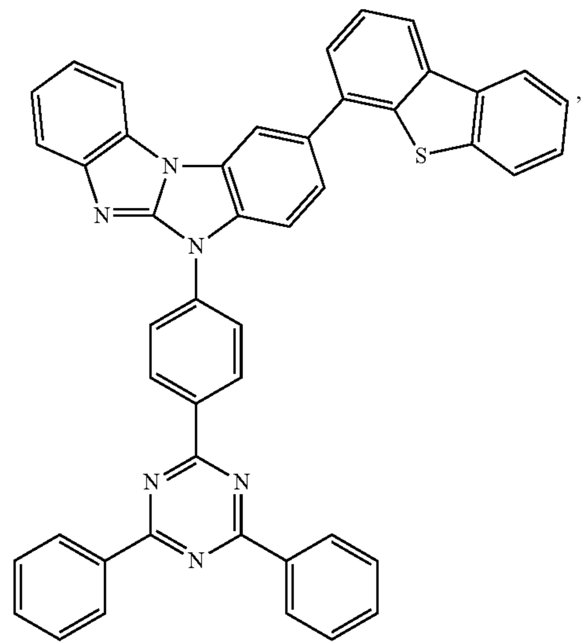
Compound 29
