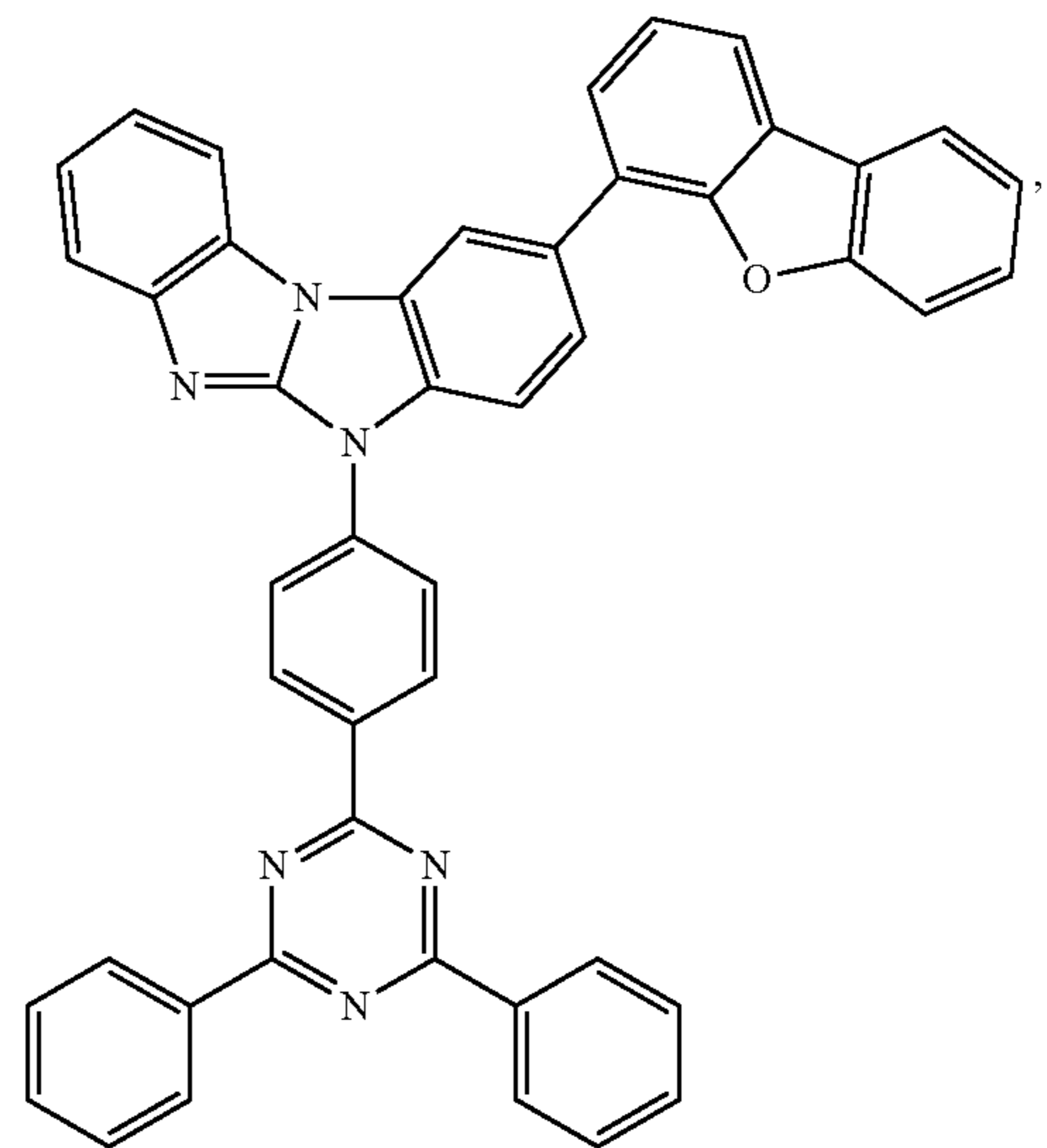
Compound 30
