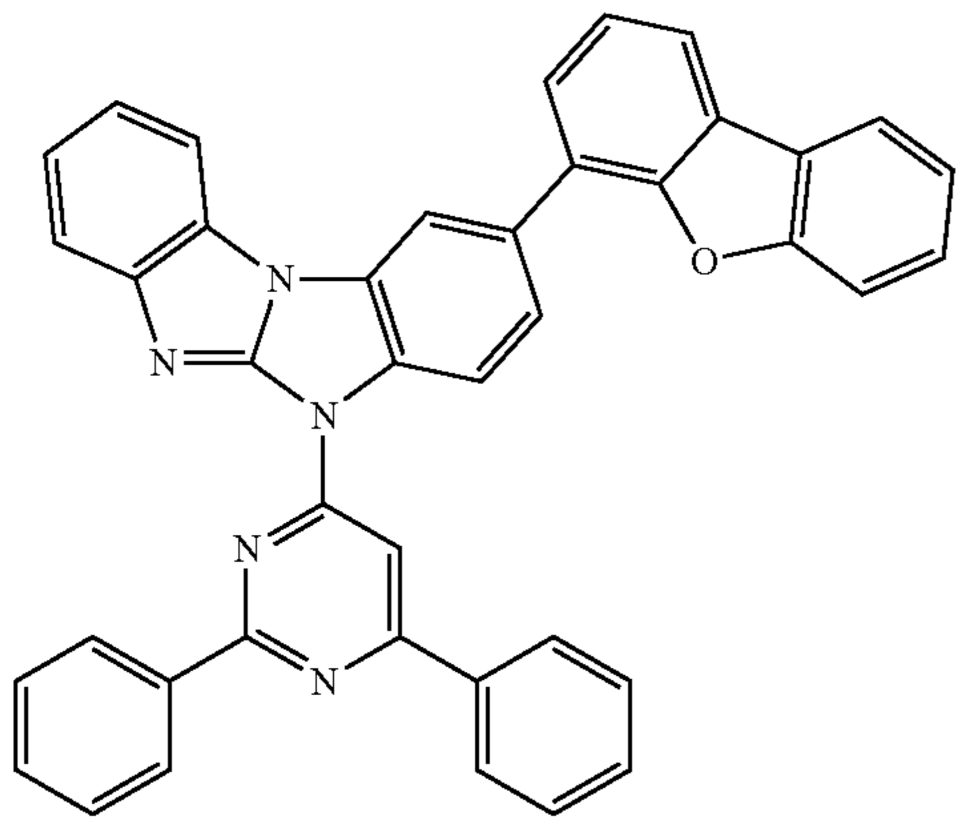
Compound 56
