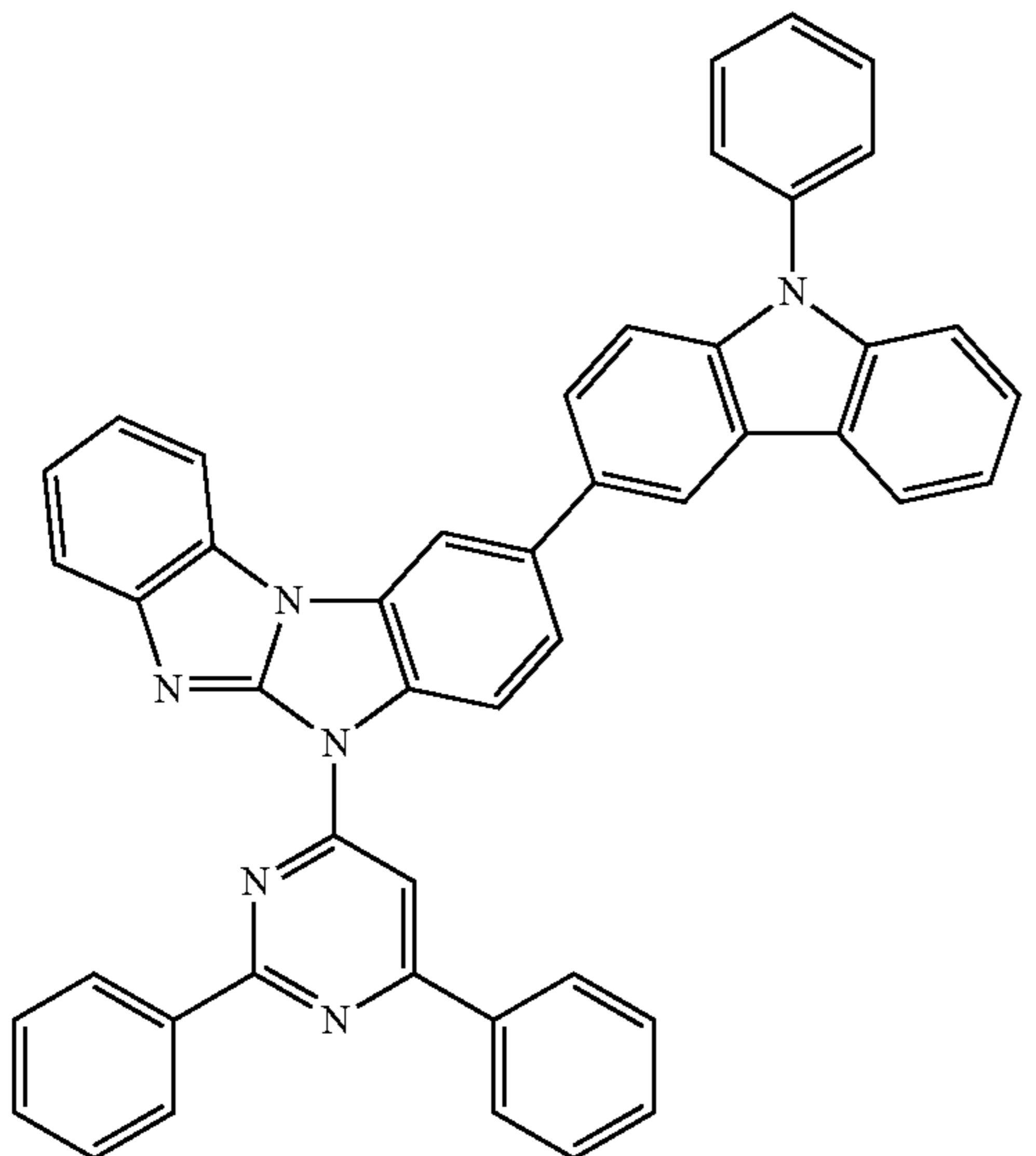
Compound 60
