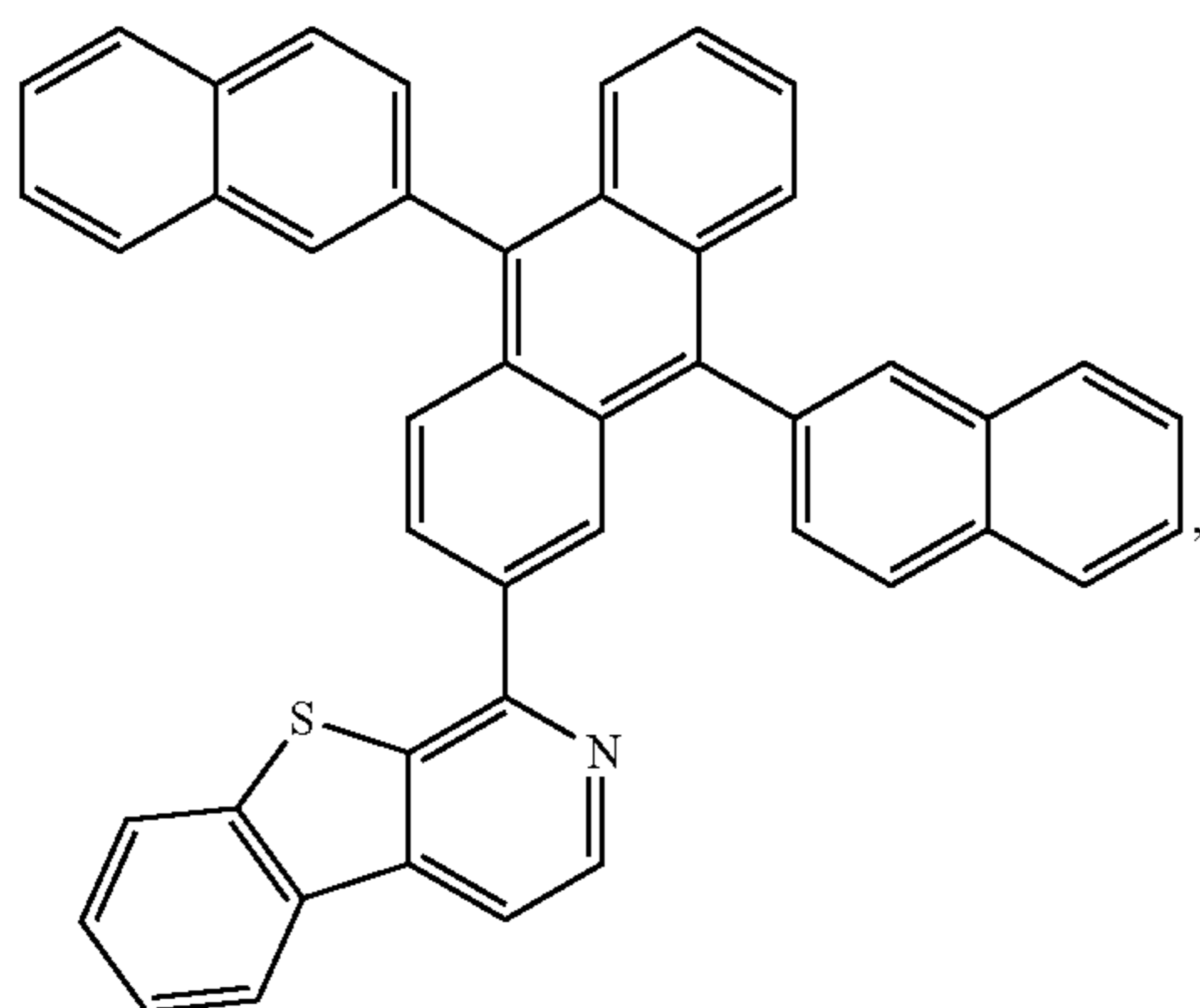
aDBT-ADN
