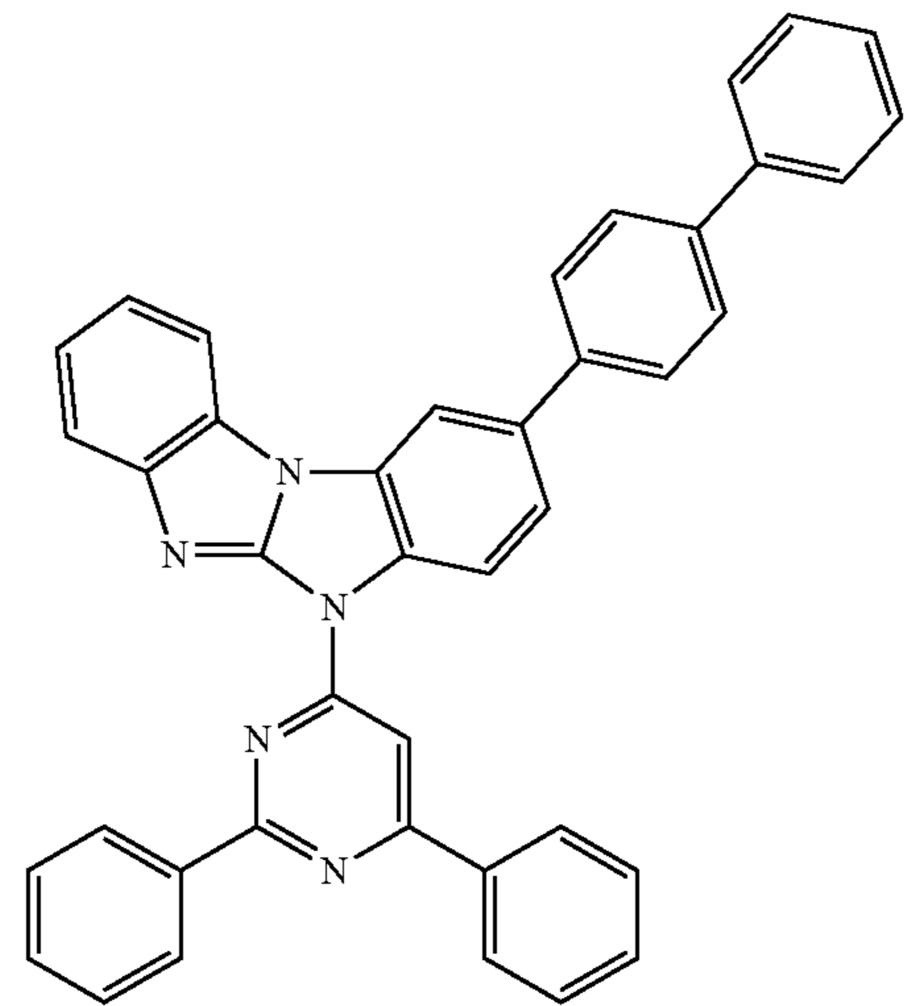
Compound 52
