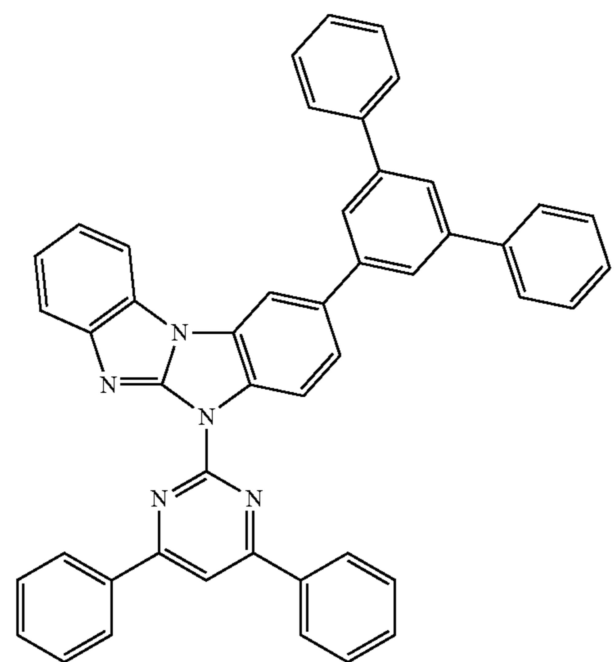
Compound 41
