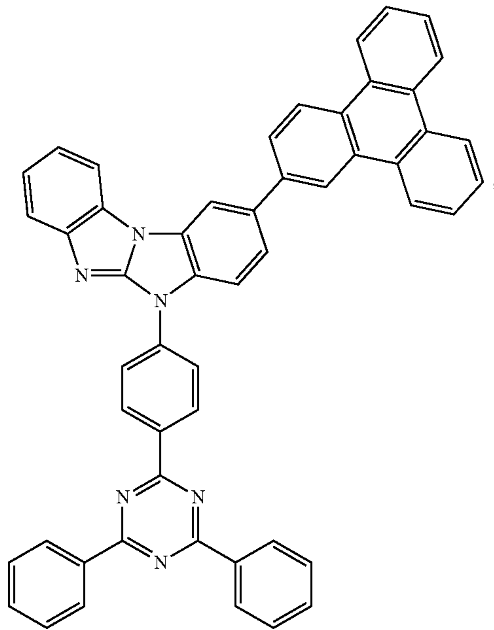
Compound 35
