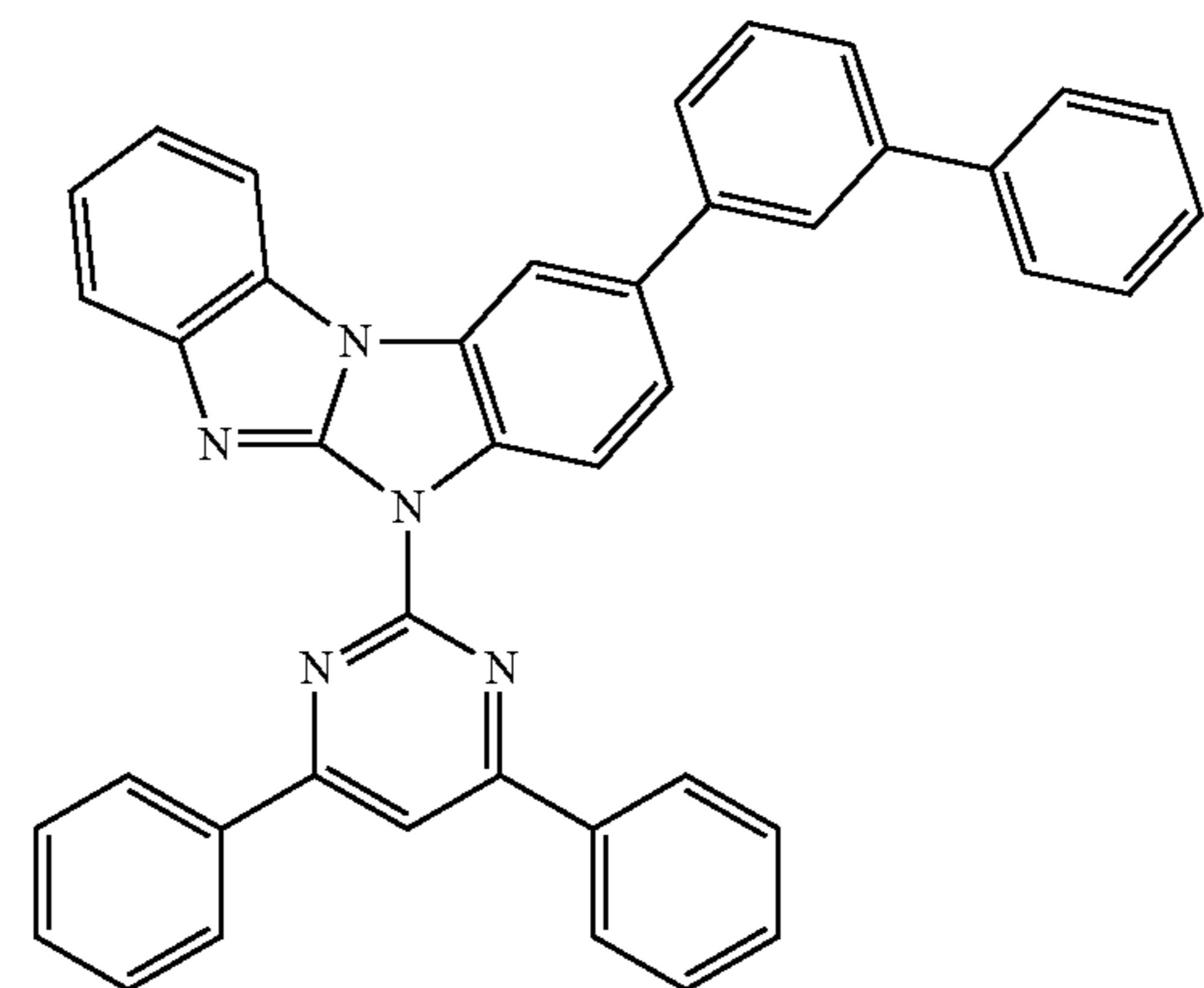
Compound 39
