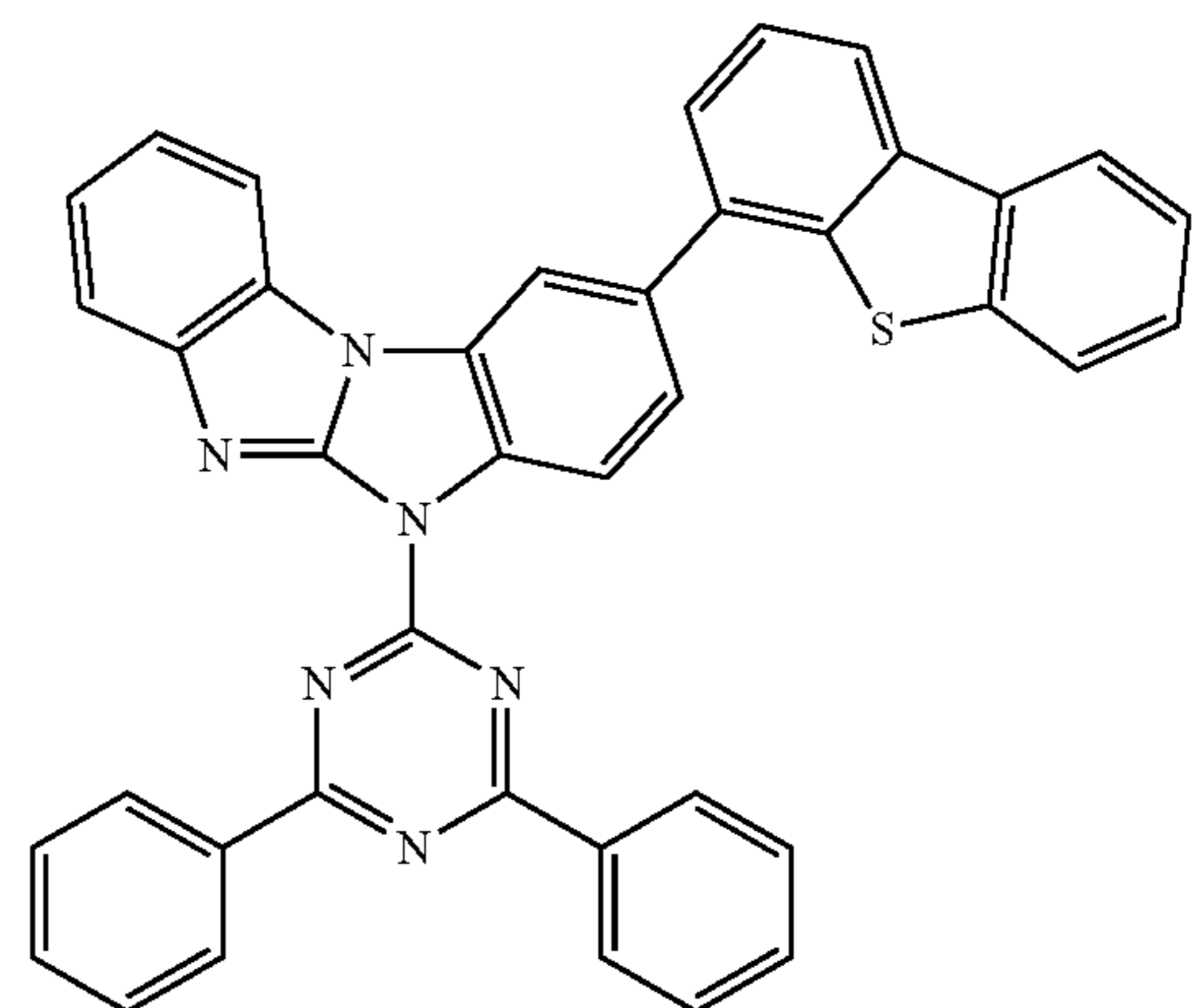
Compound 11
