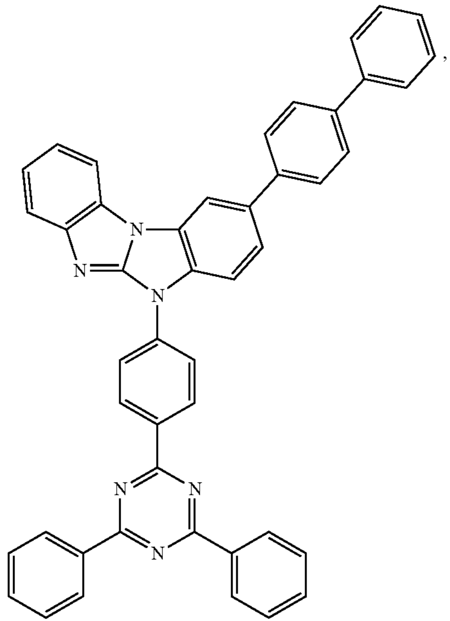
Compound 26
