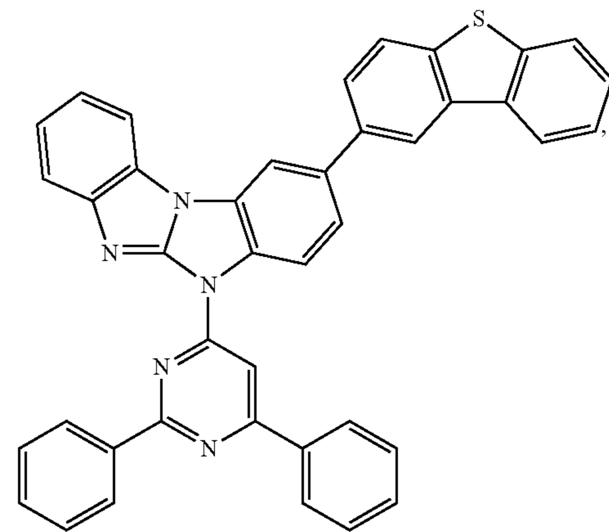
Compound 58
