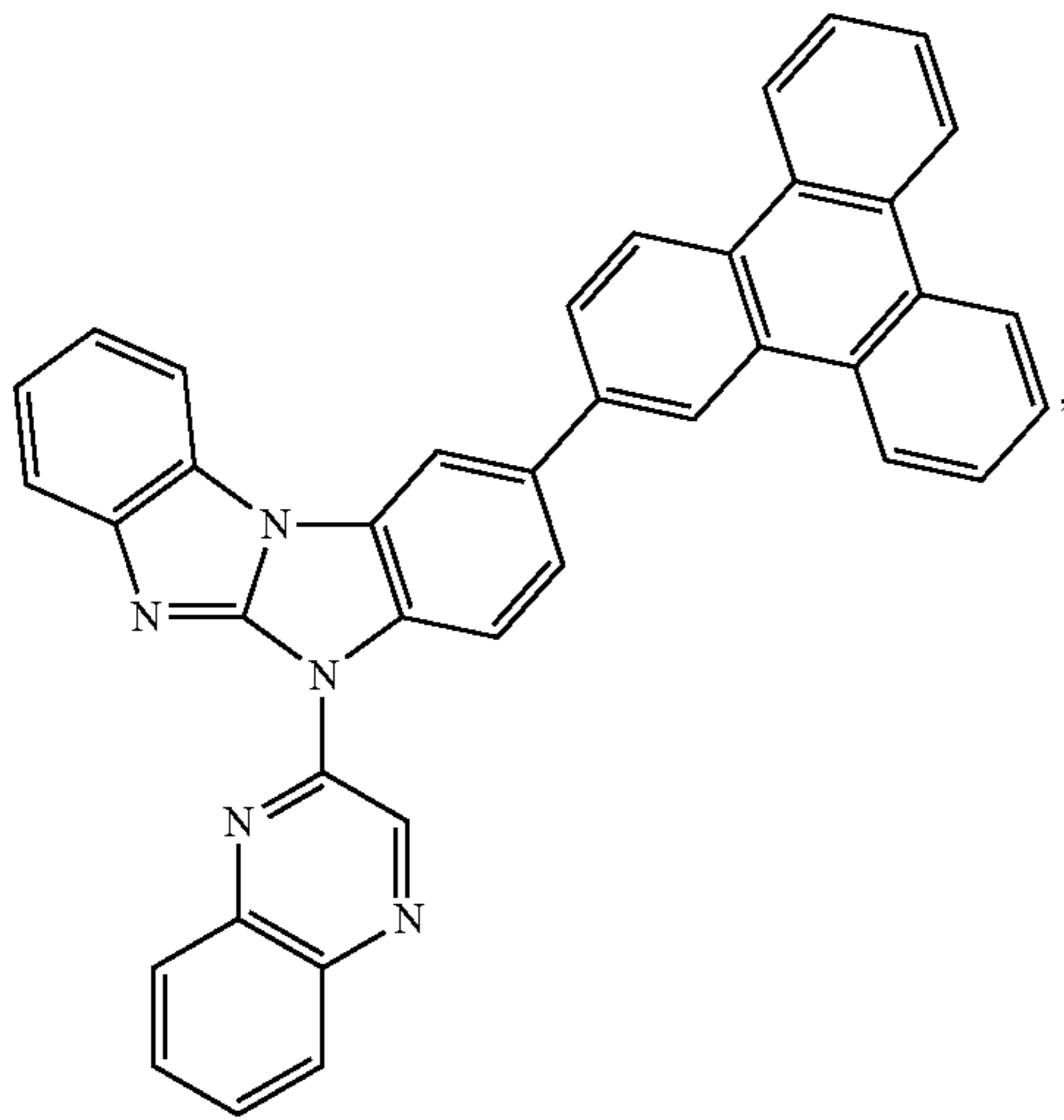
Compound 71
