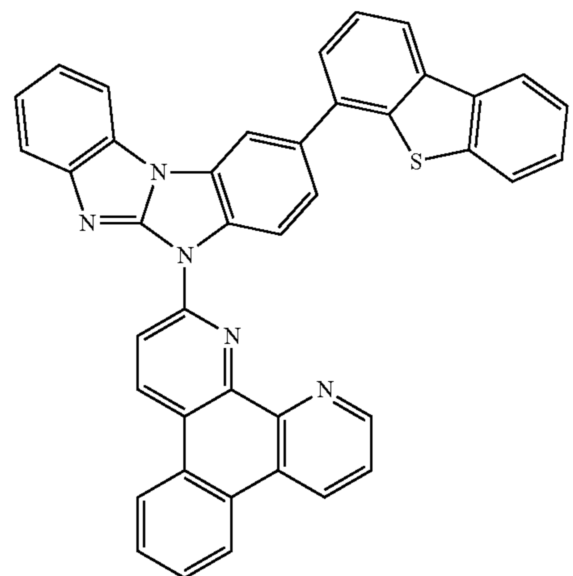
Compound 92
