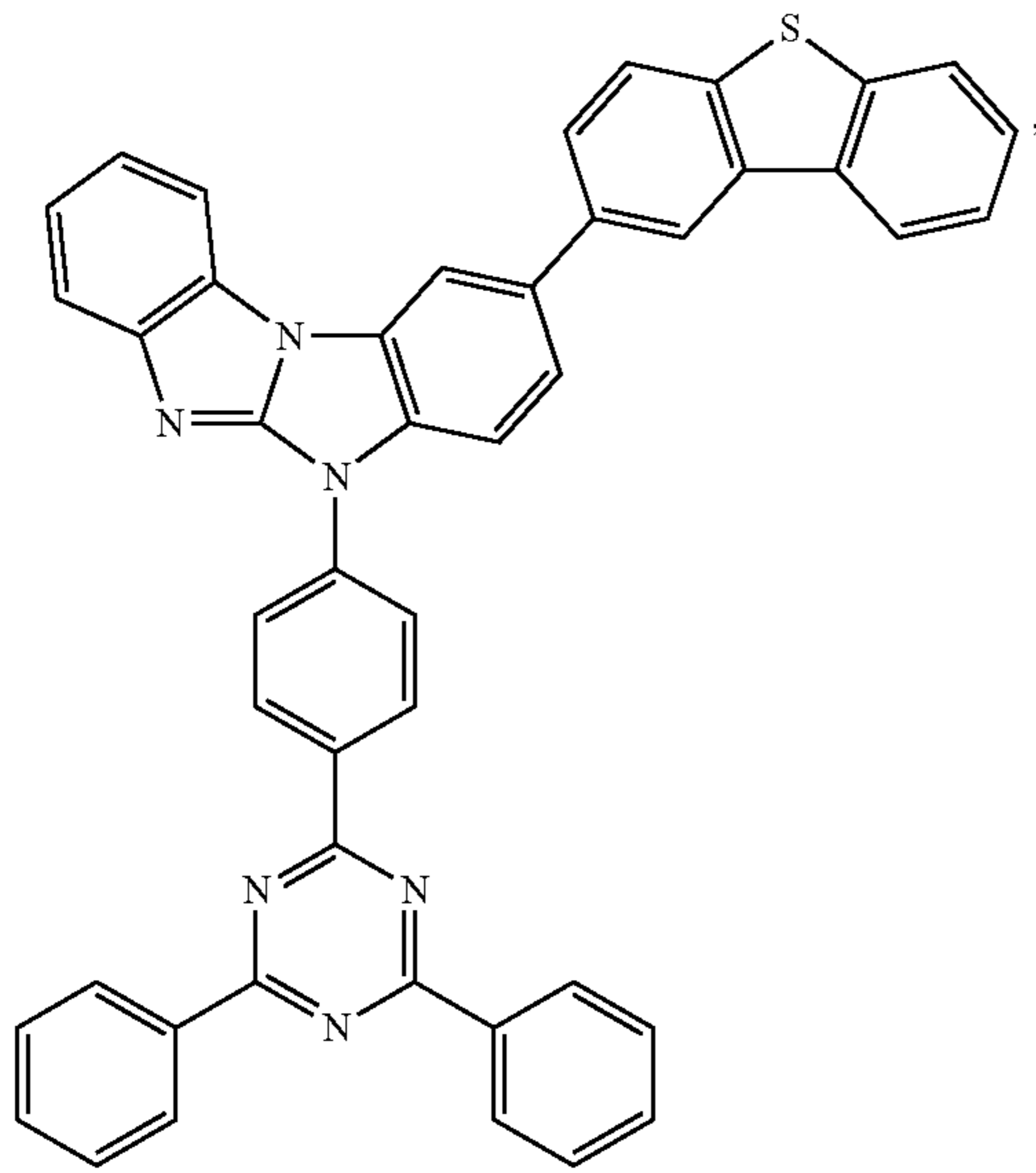
Compound 31
