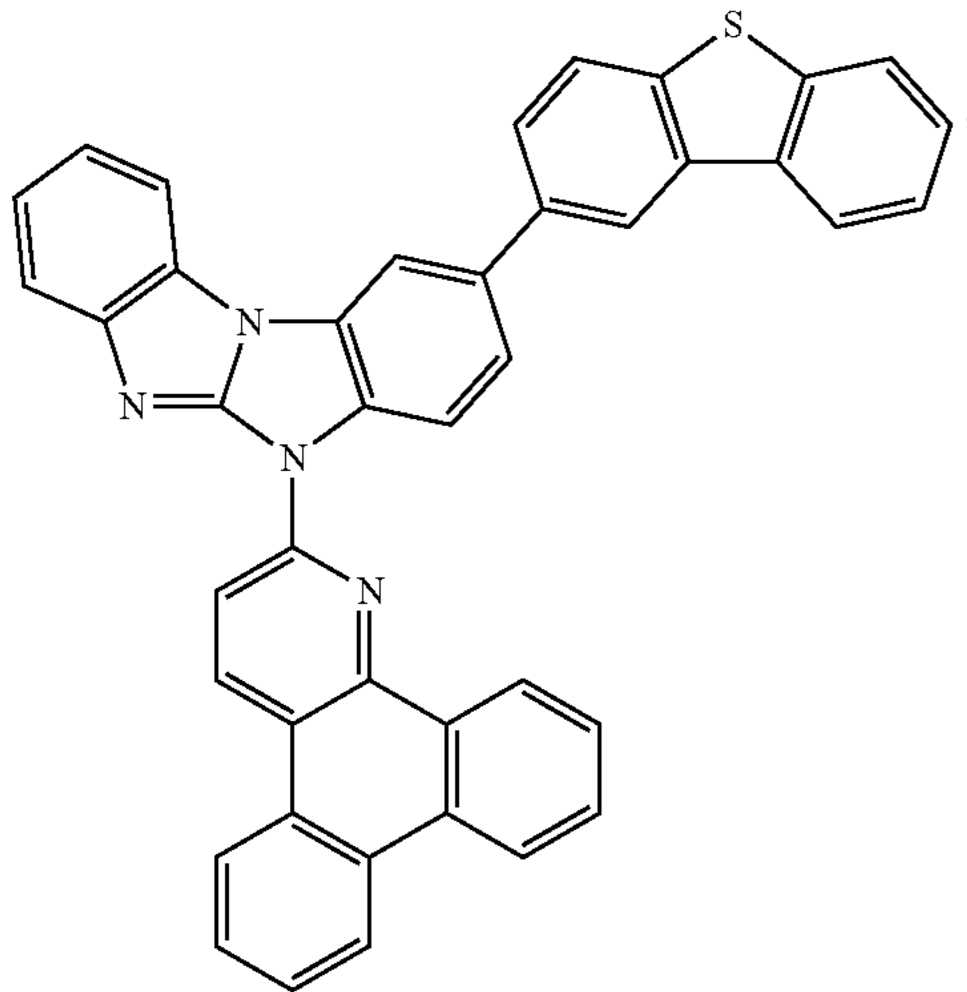
Compound 87
