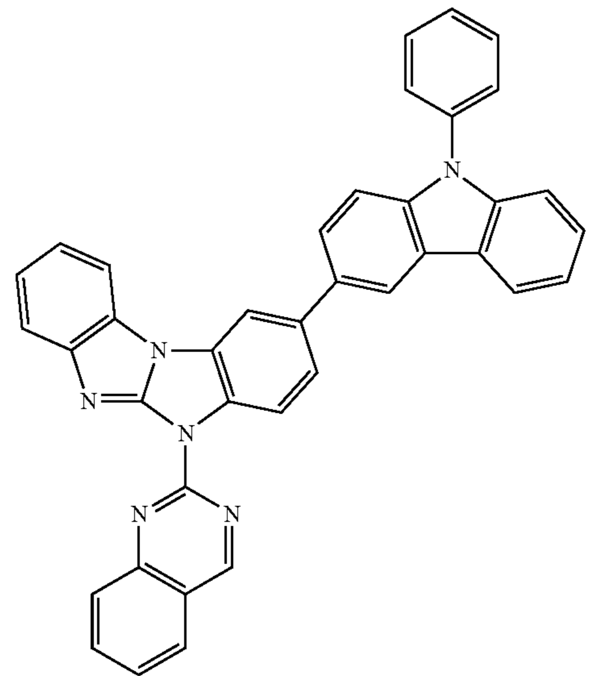
Compound 80
