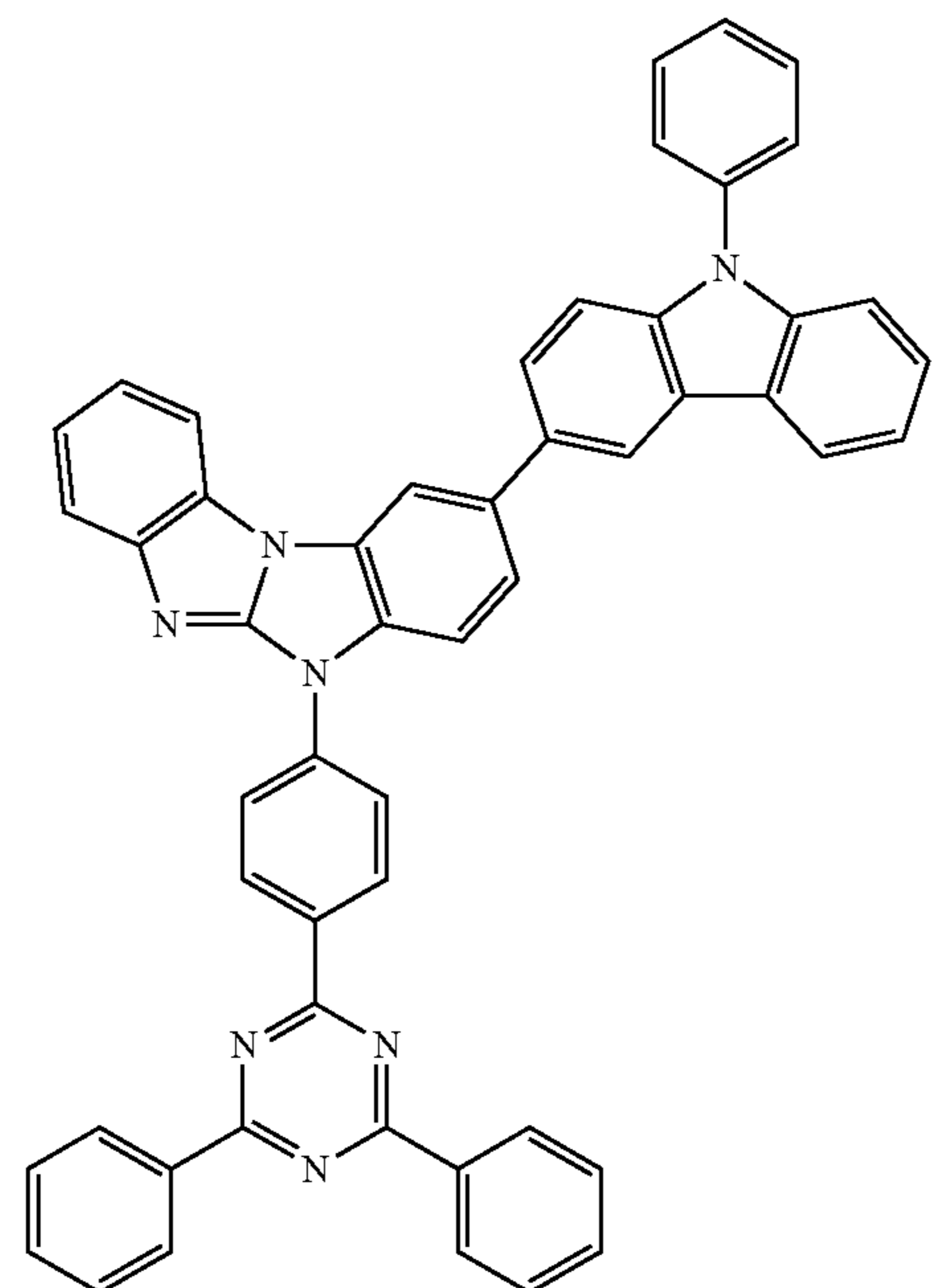
Compound 34
