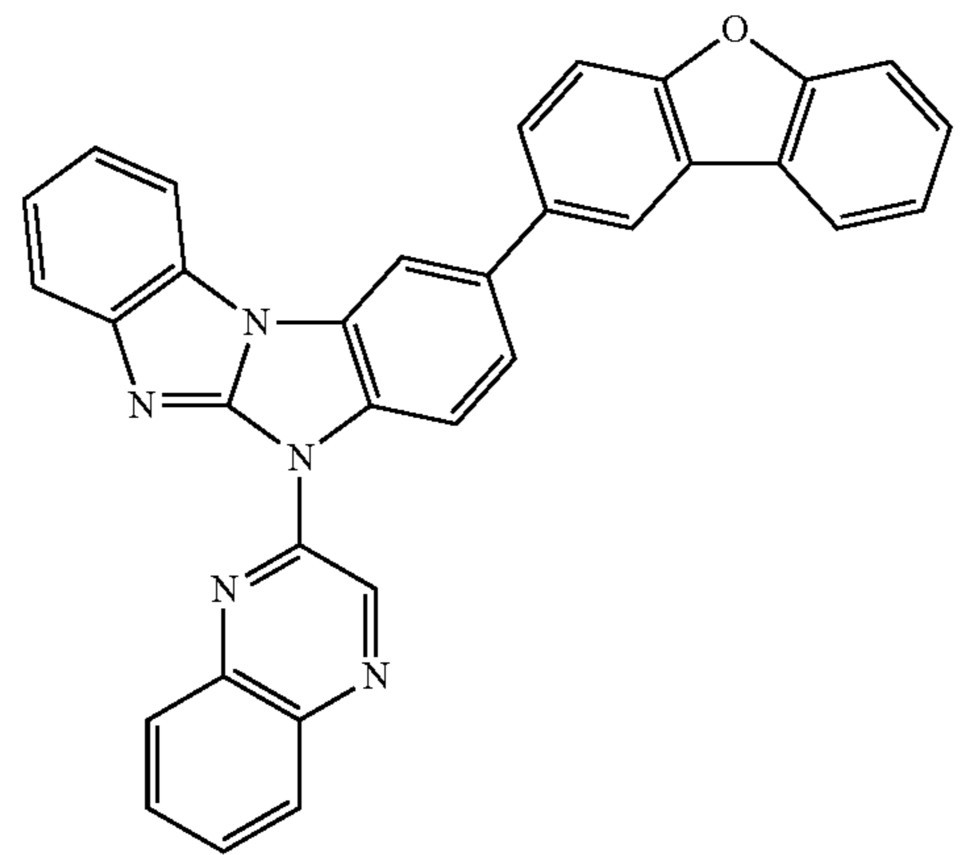
Compound 69
