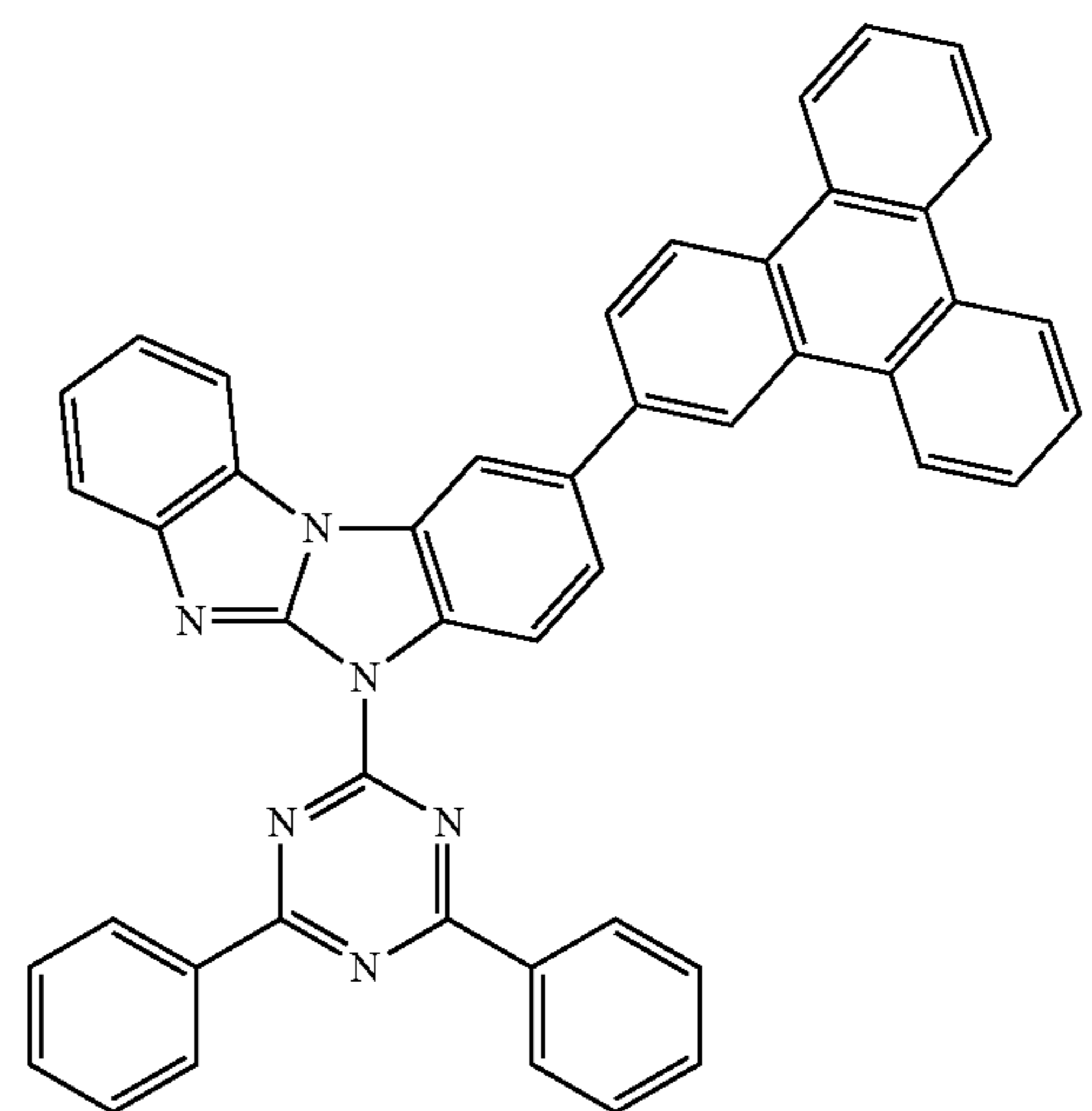
Compound 18
