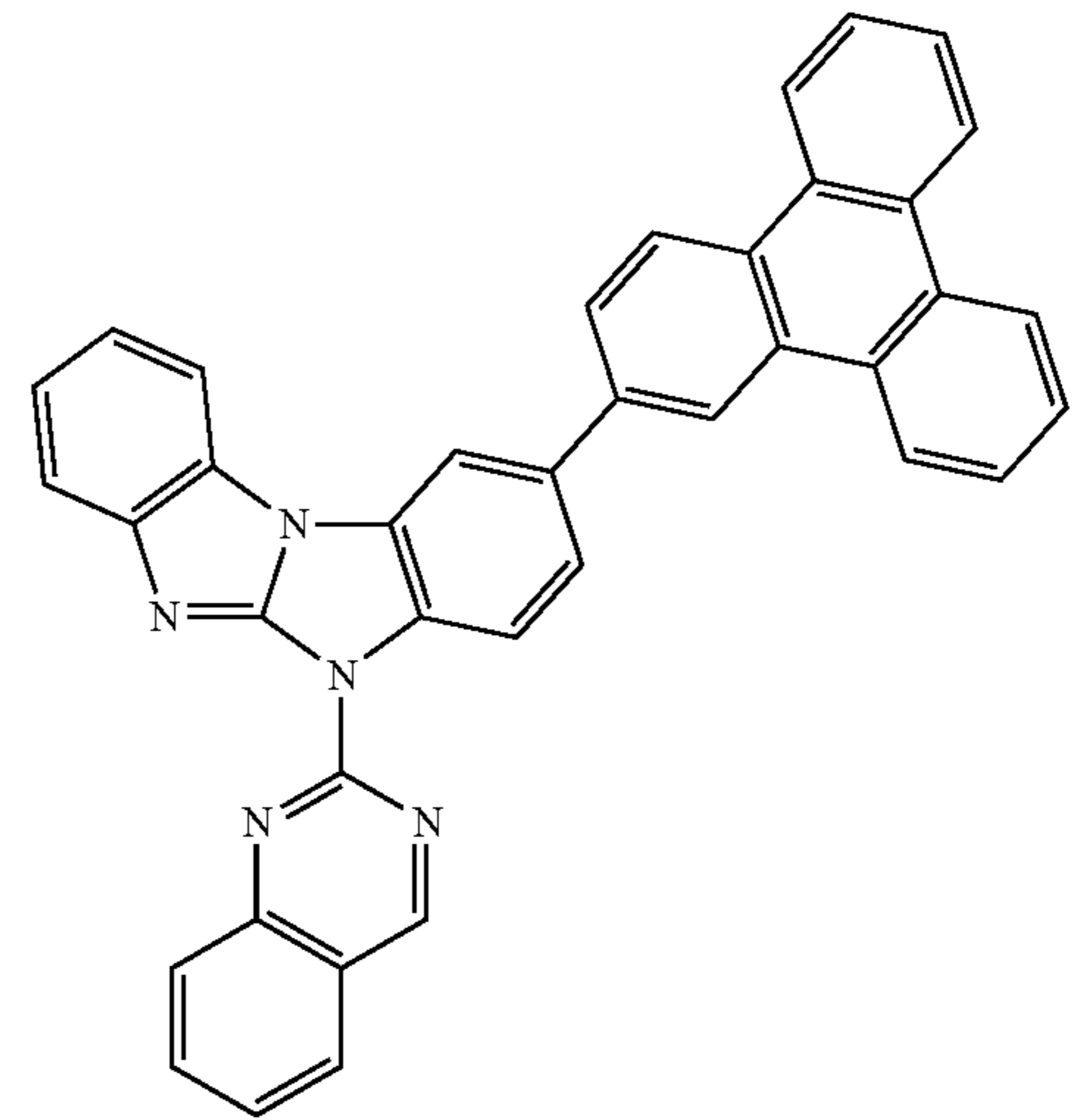
Compound 81
