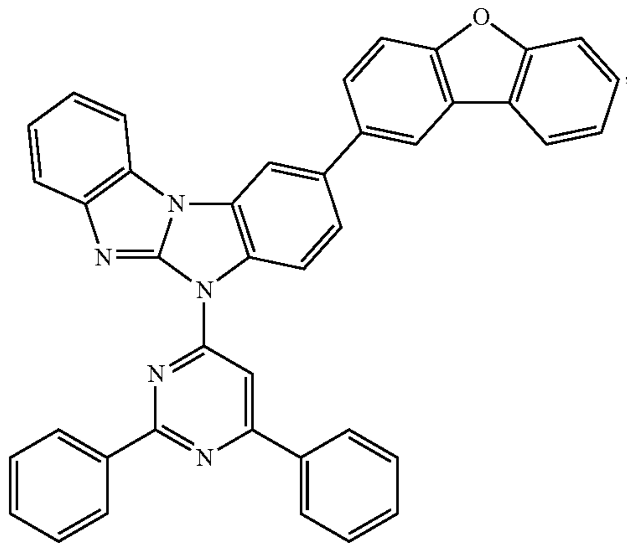
Compound 59
