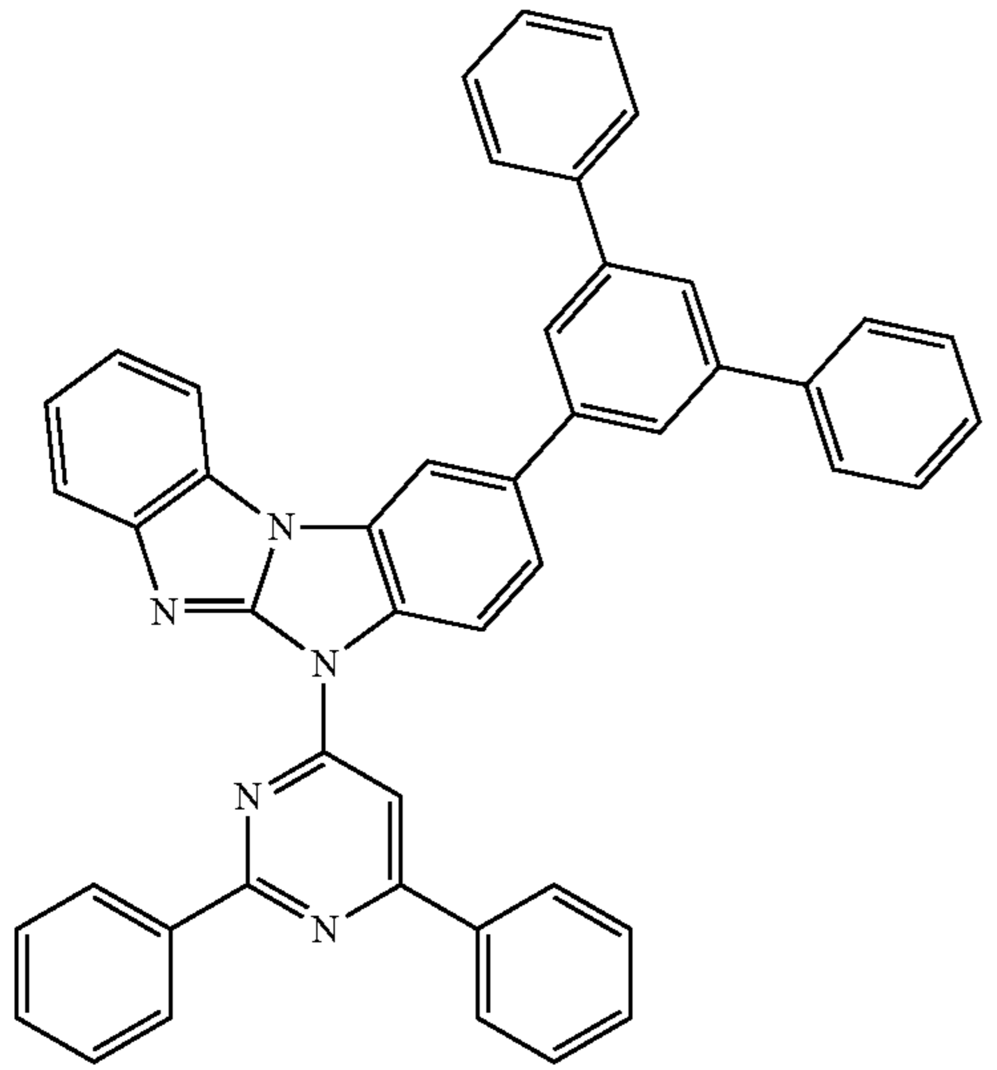
Compound 55
