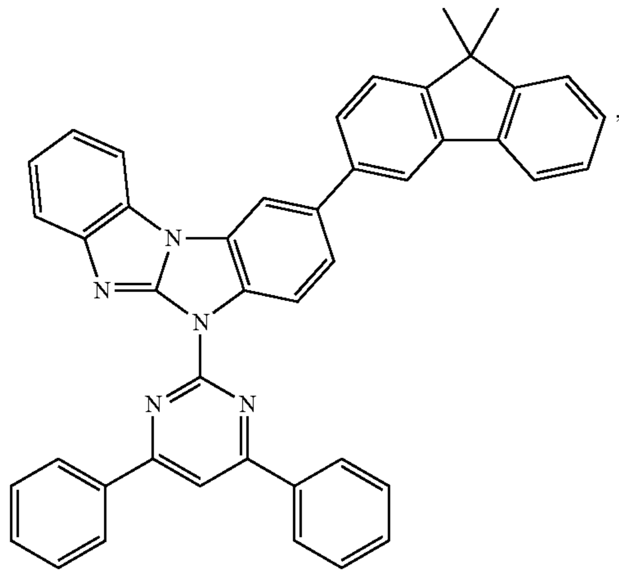
Compound 48
