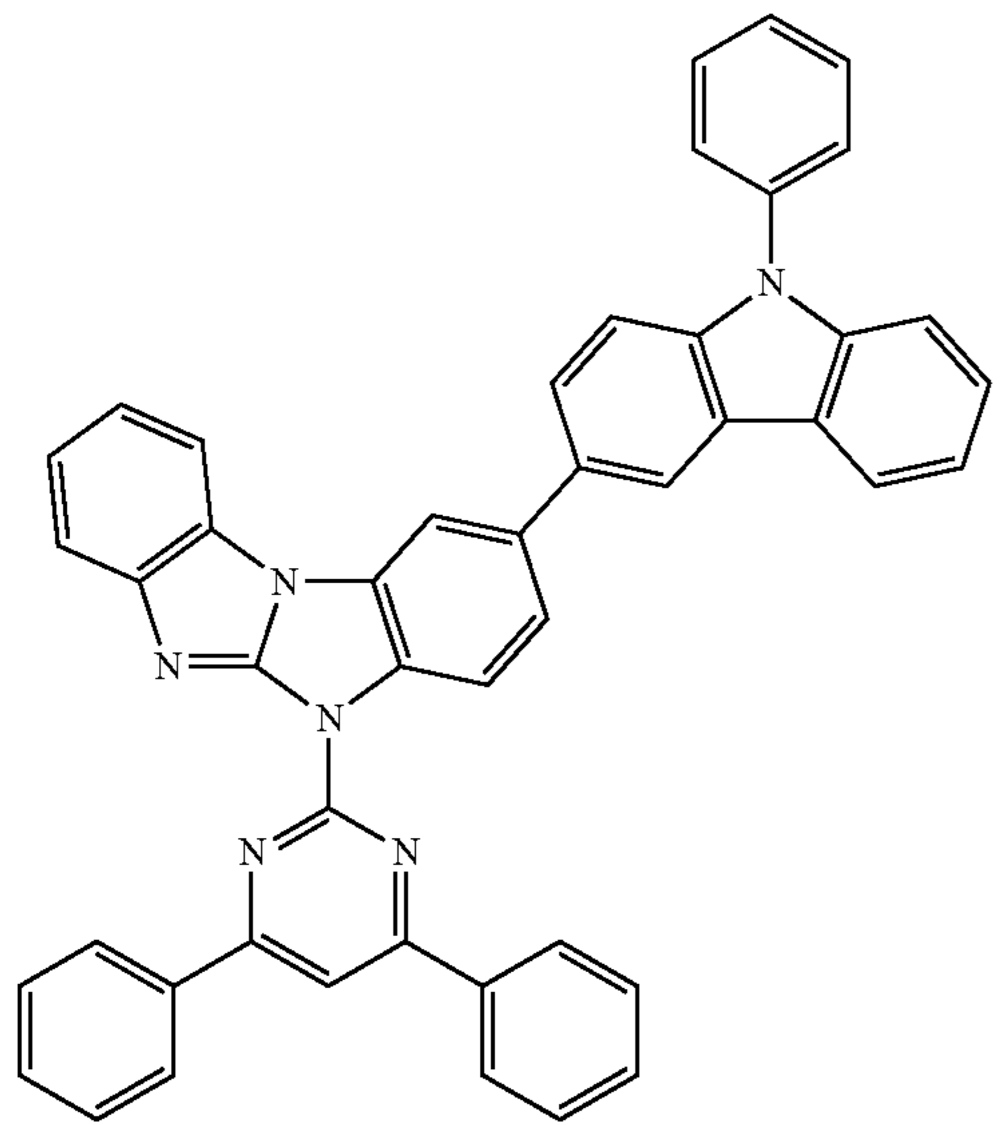
Compound 47
