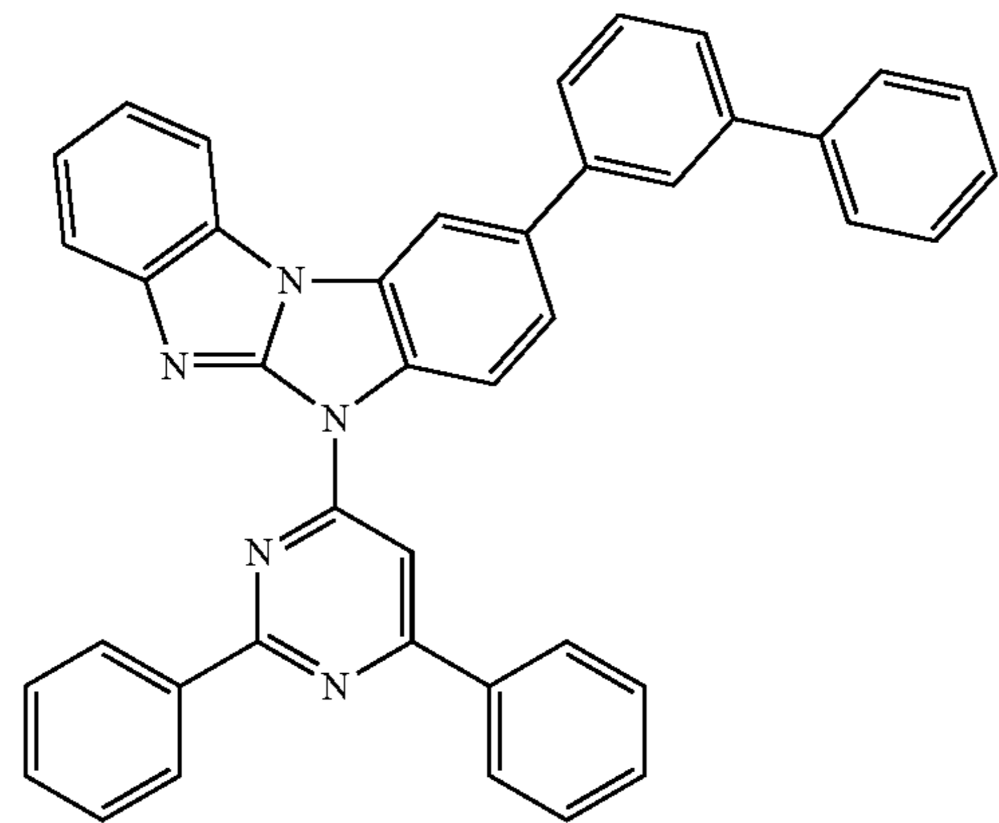
Compound 53
