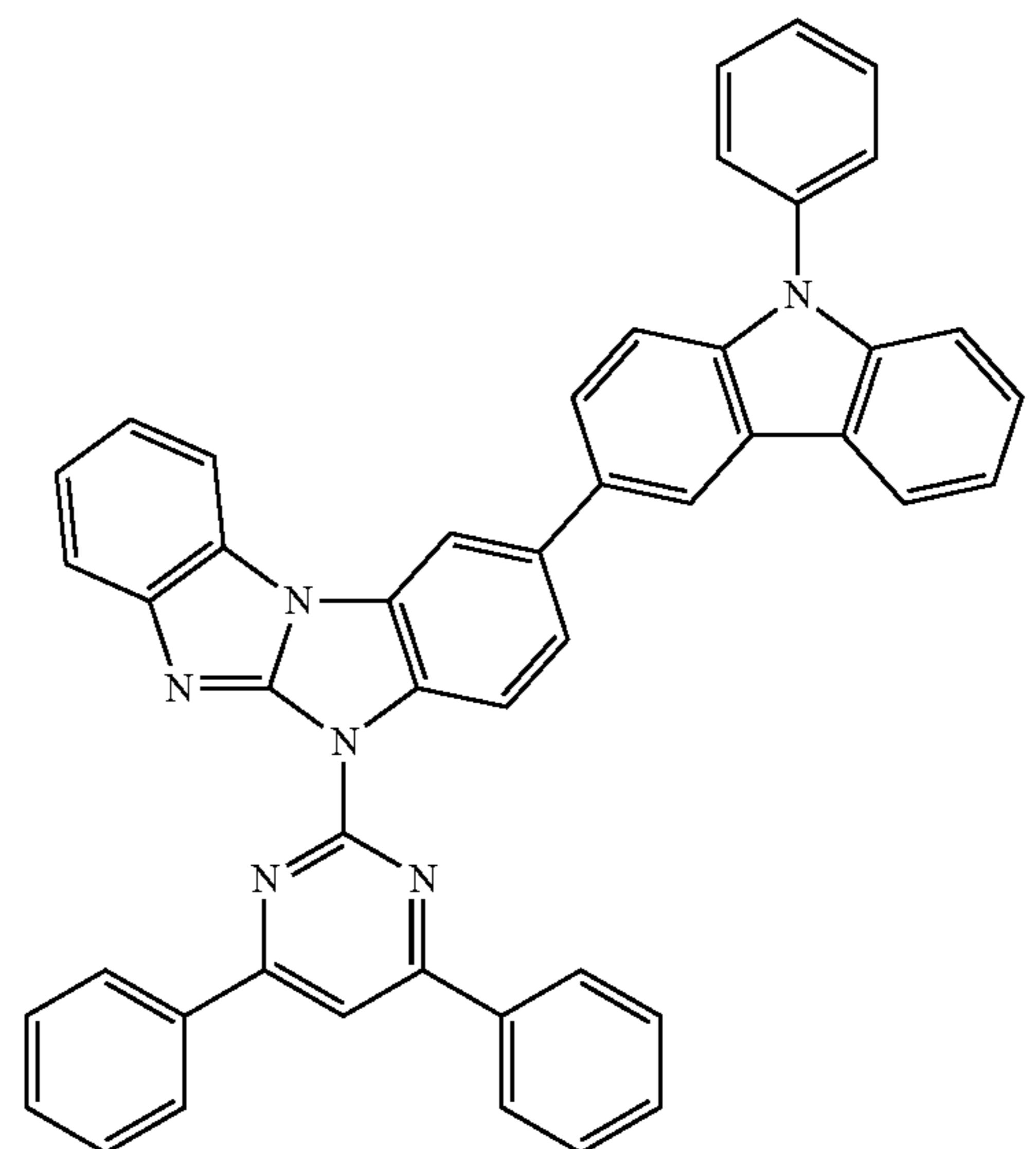
Compound 47
