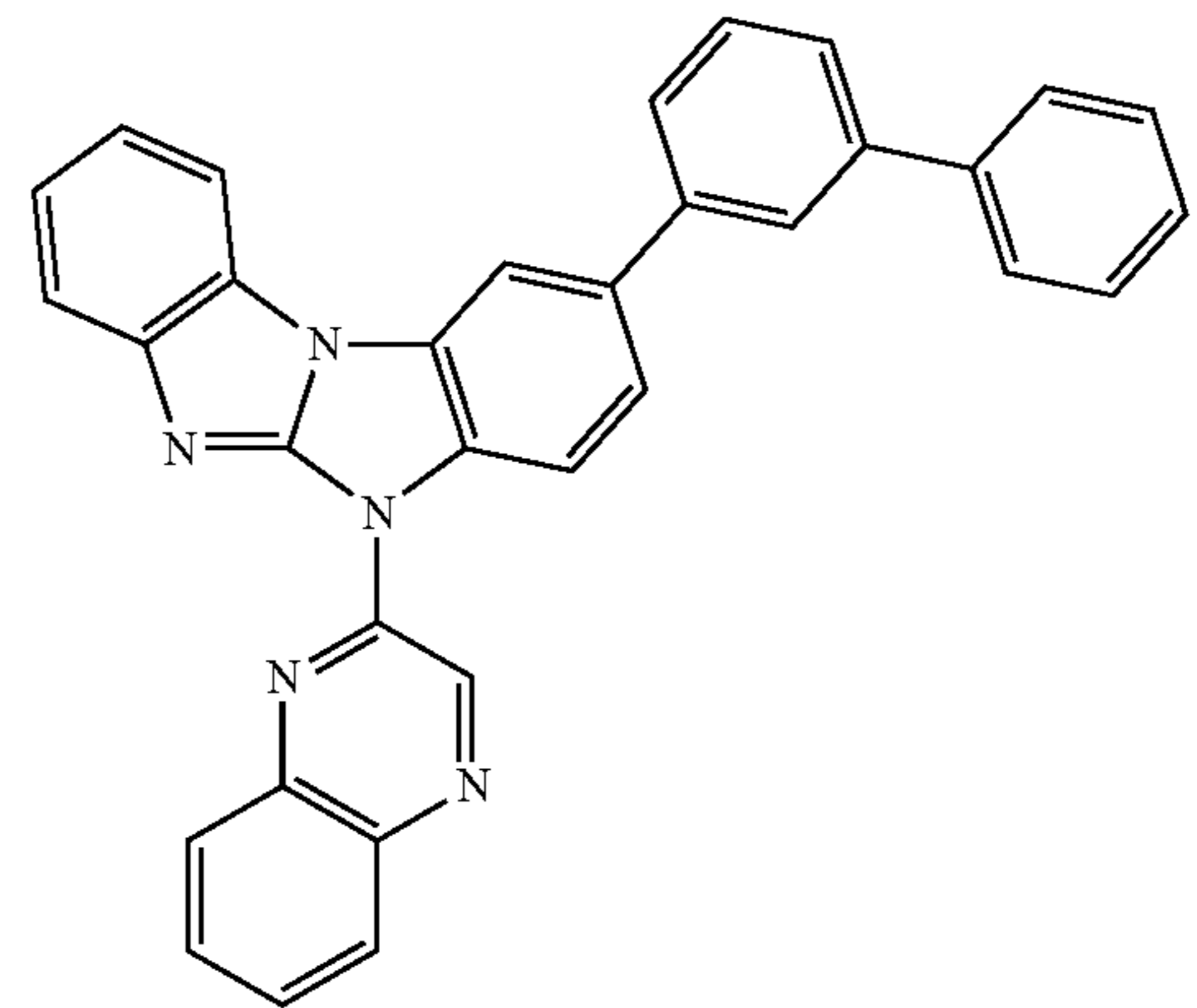
Compound 65
