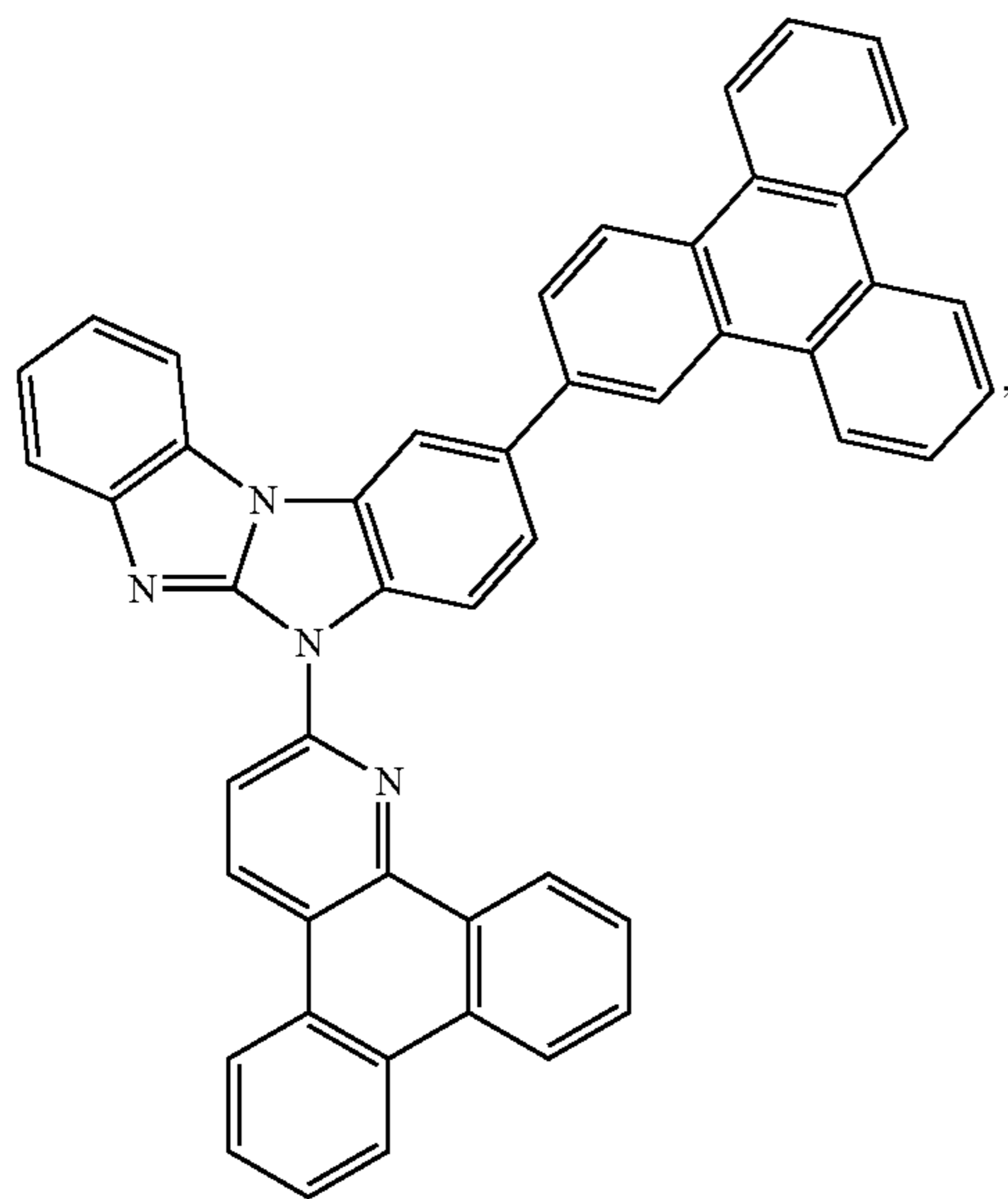
Compound 91
