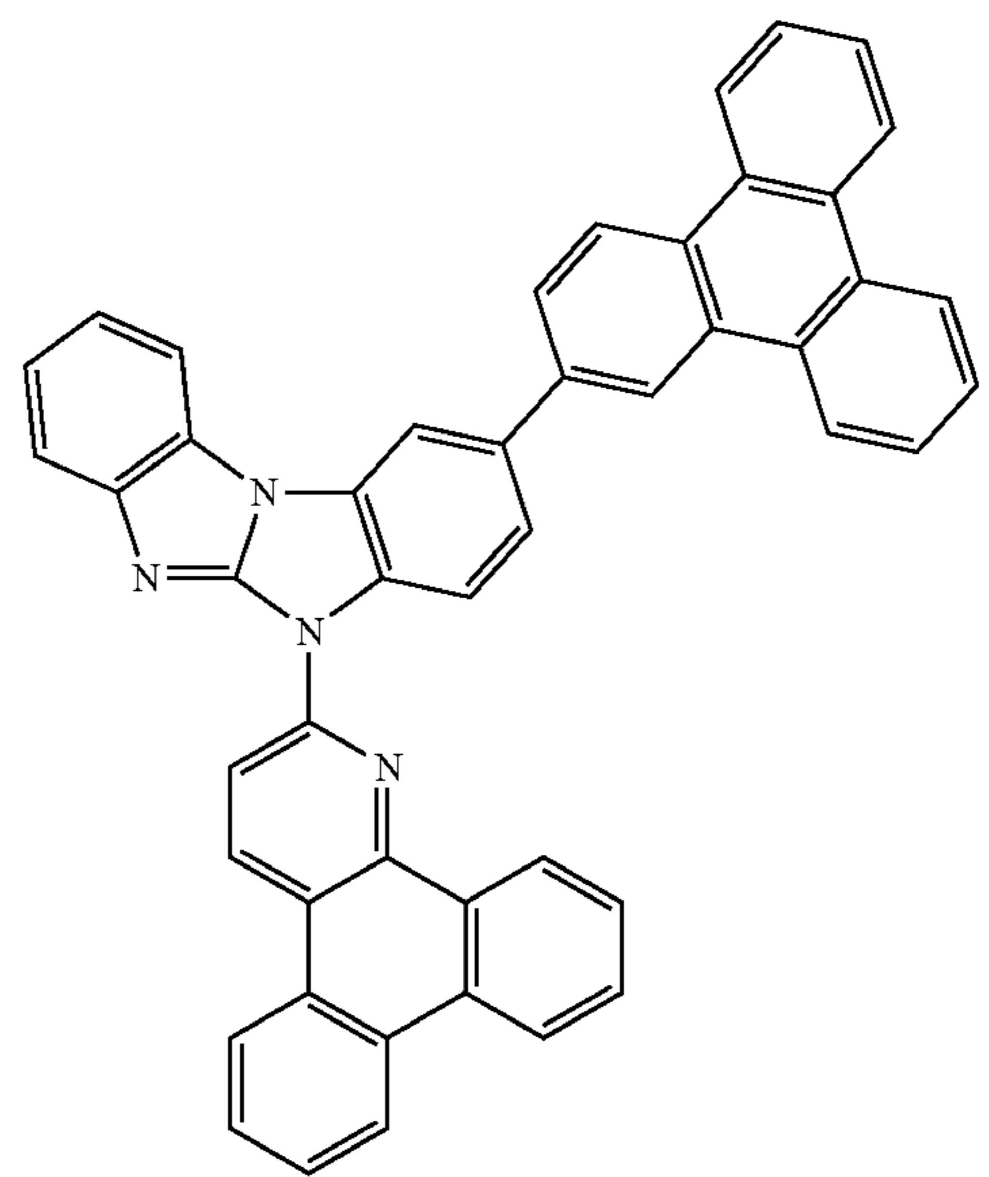
Compound 90
