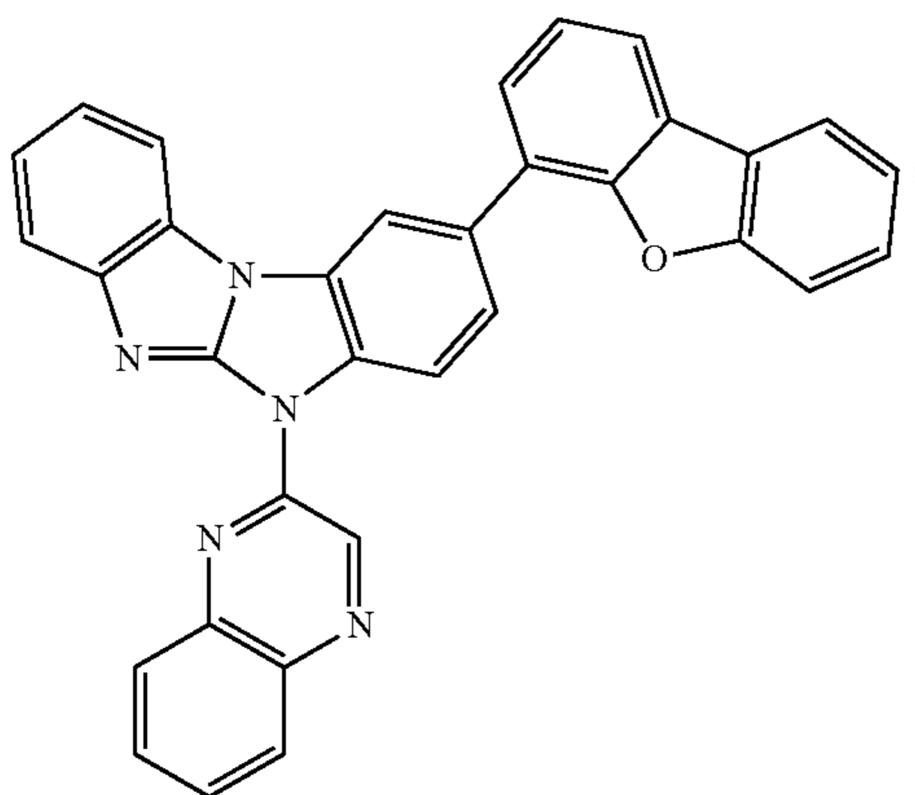
Compound 67
