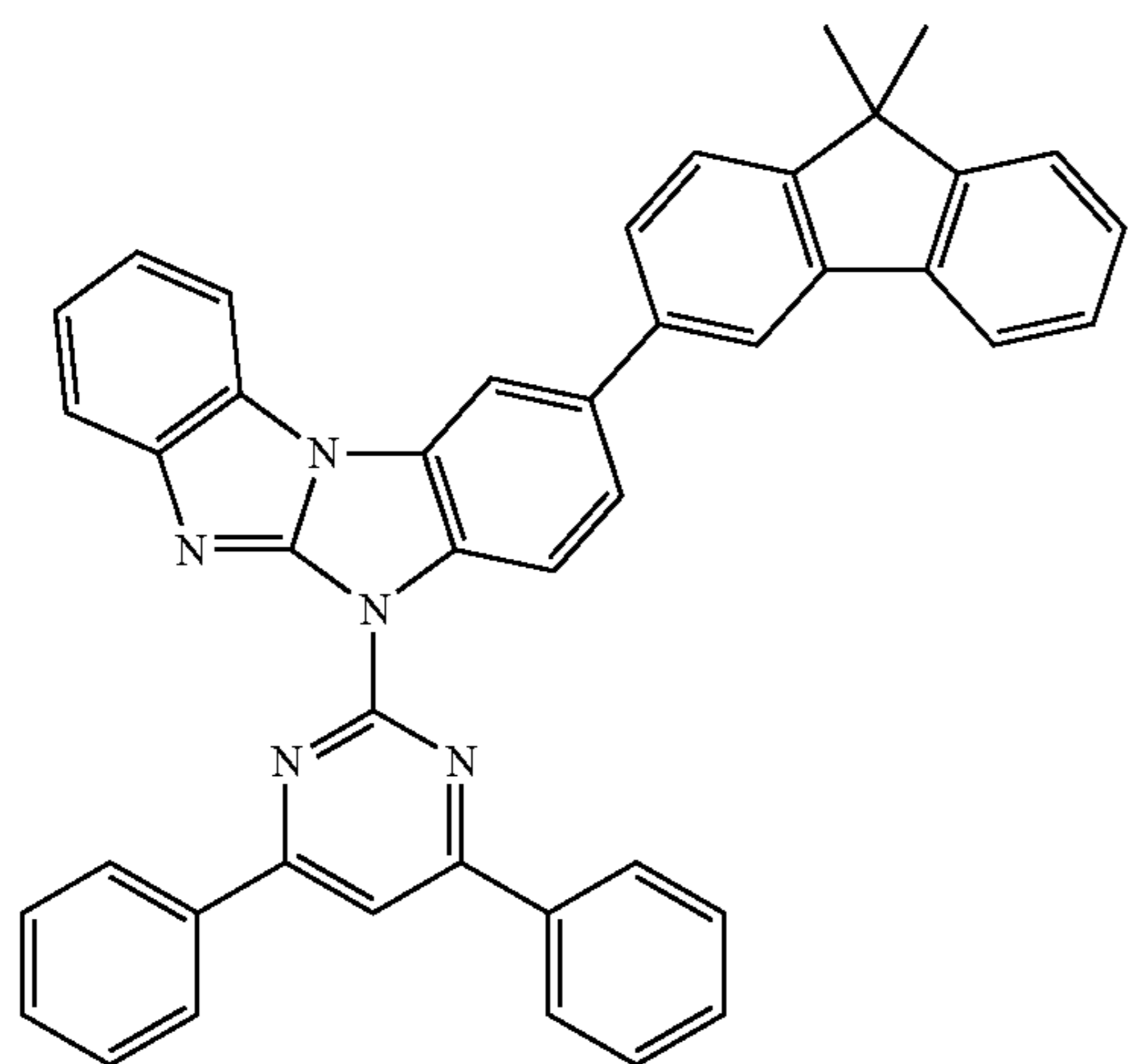
Compound 48
