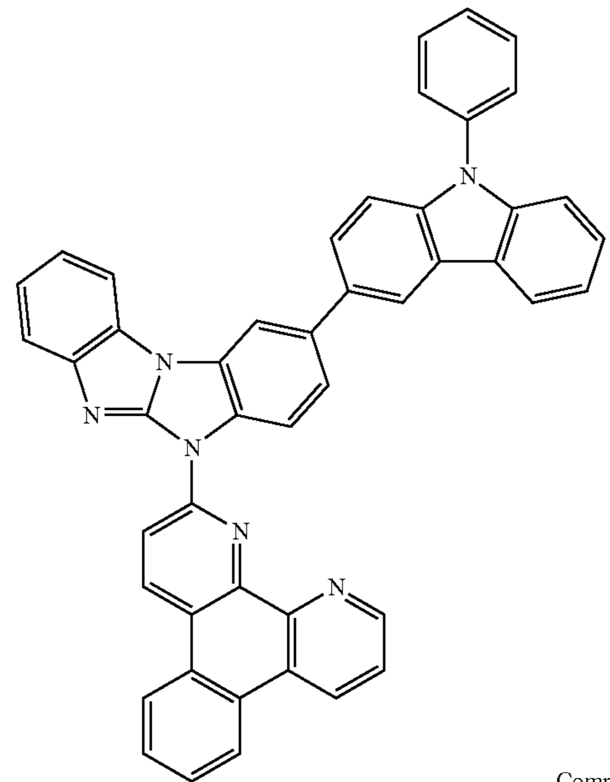
Compound 97
