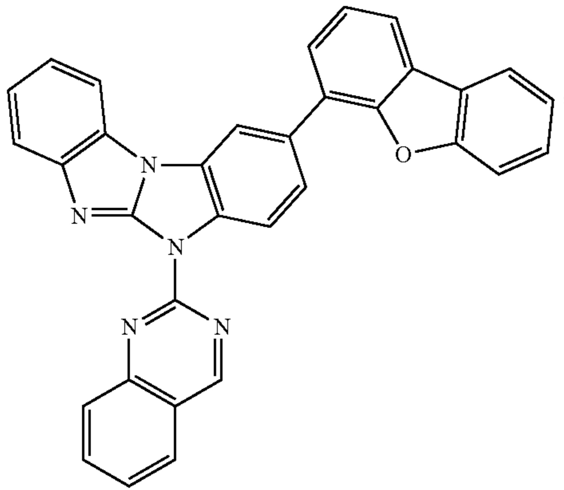
Compound 77
