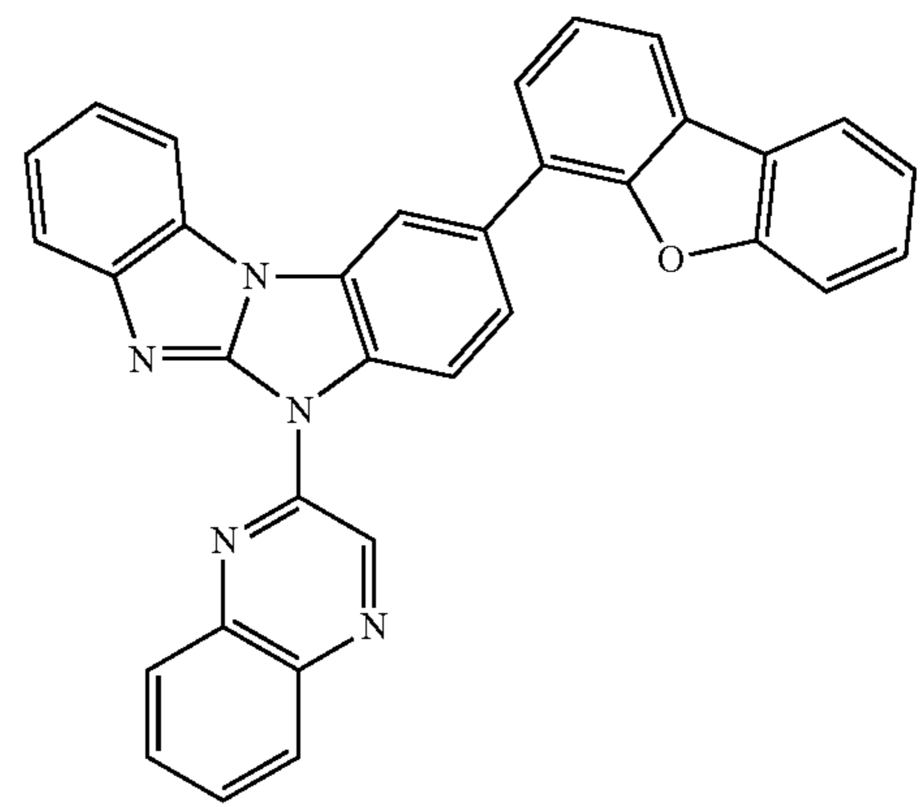
Compound 67
