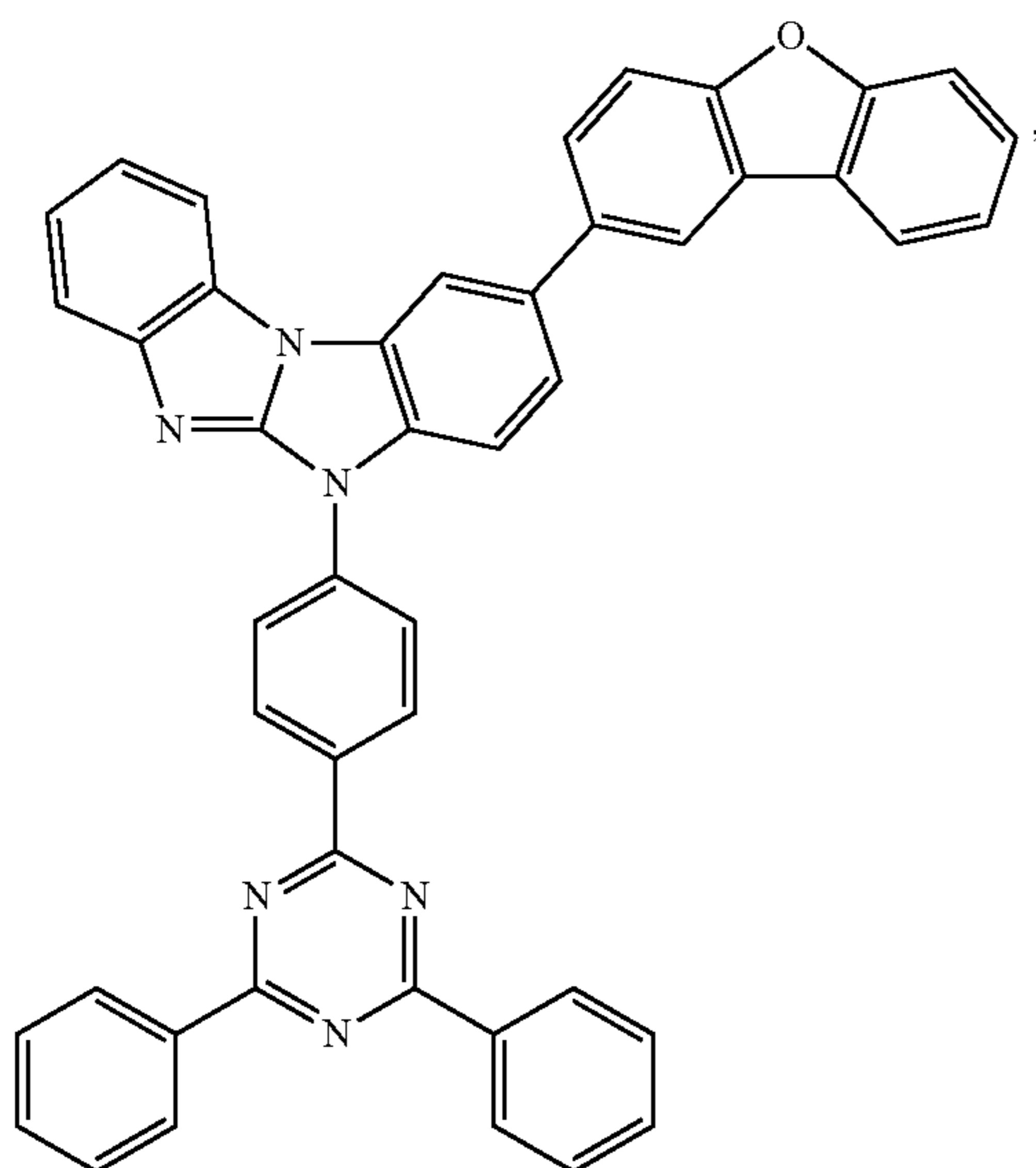
Compound 32
