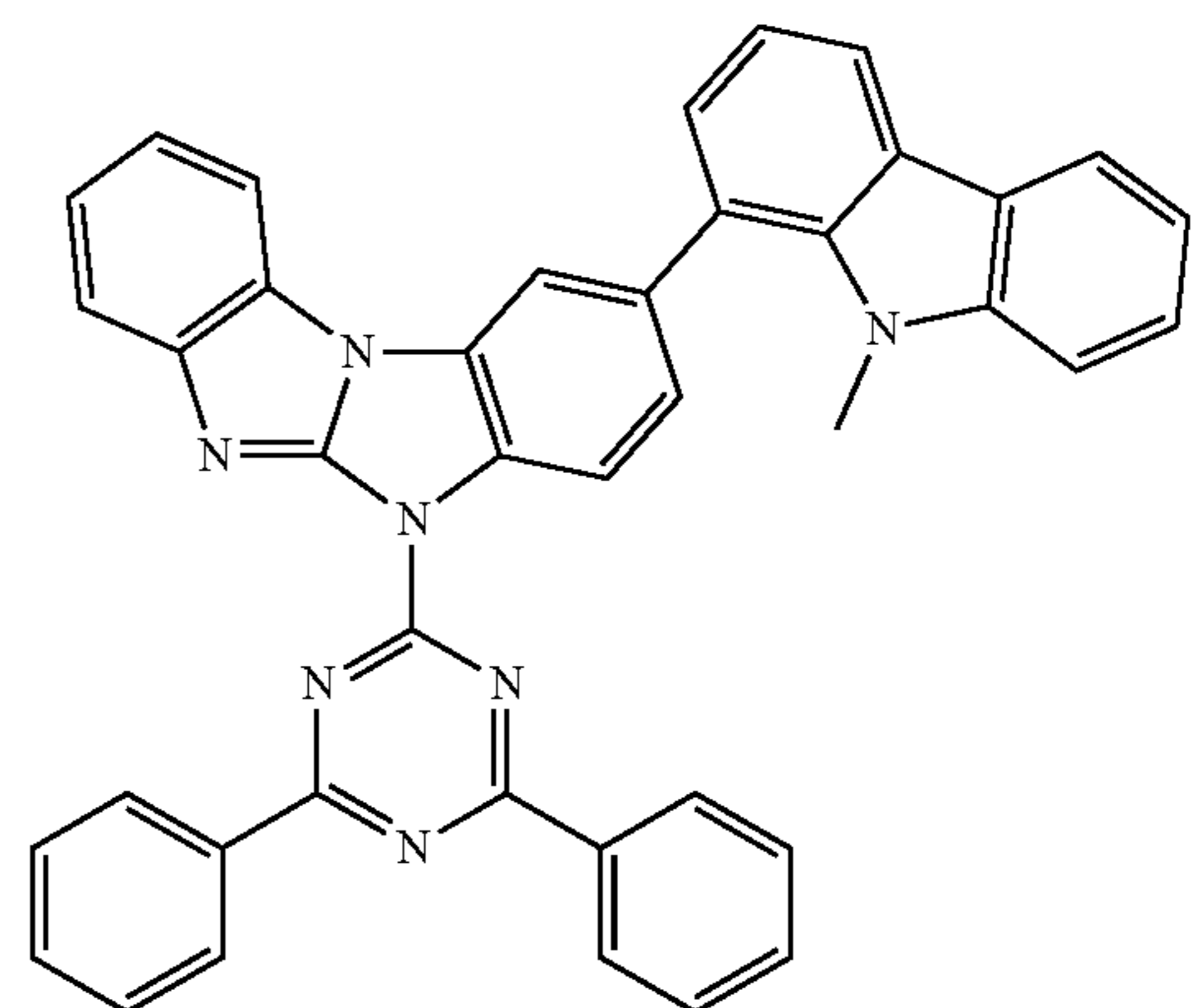
Compound 12
