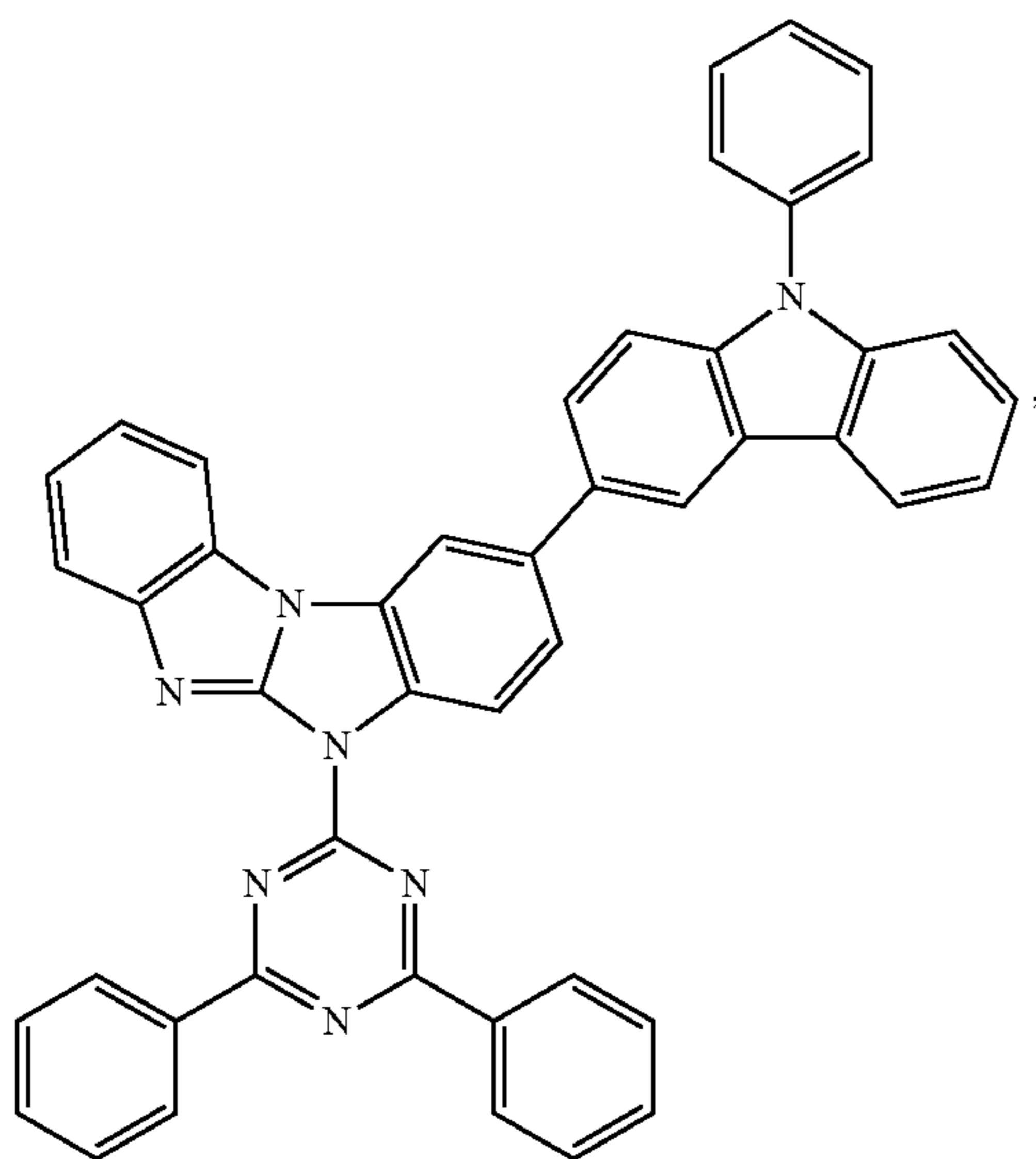
Compound 16
