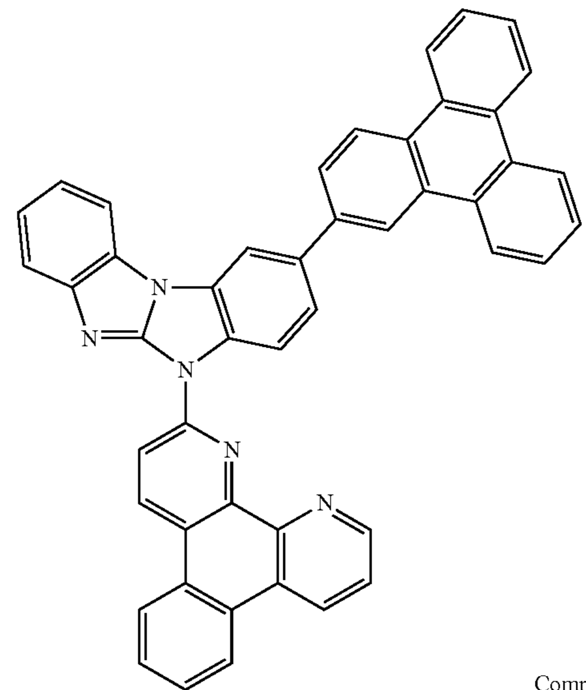
Compound 98
