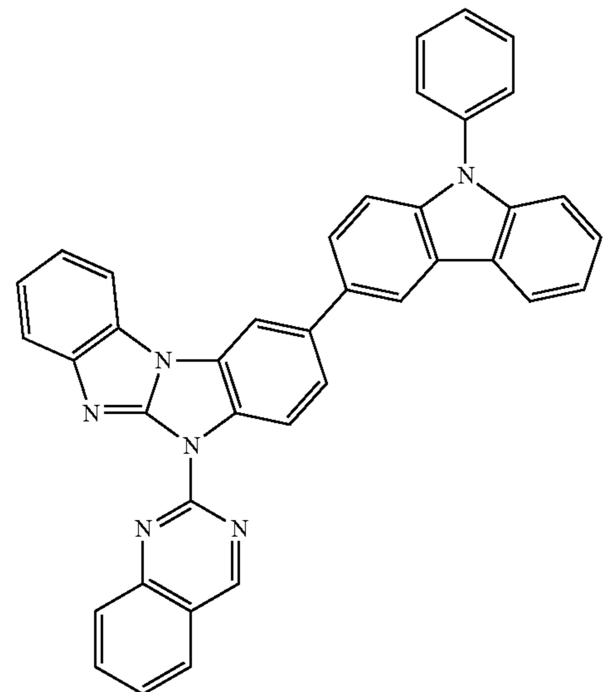
Compound 80
