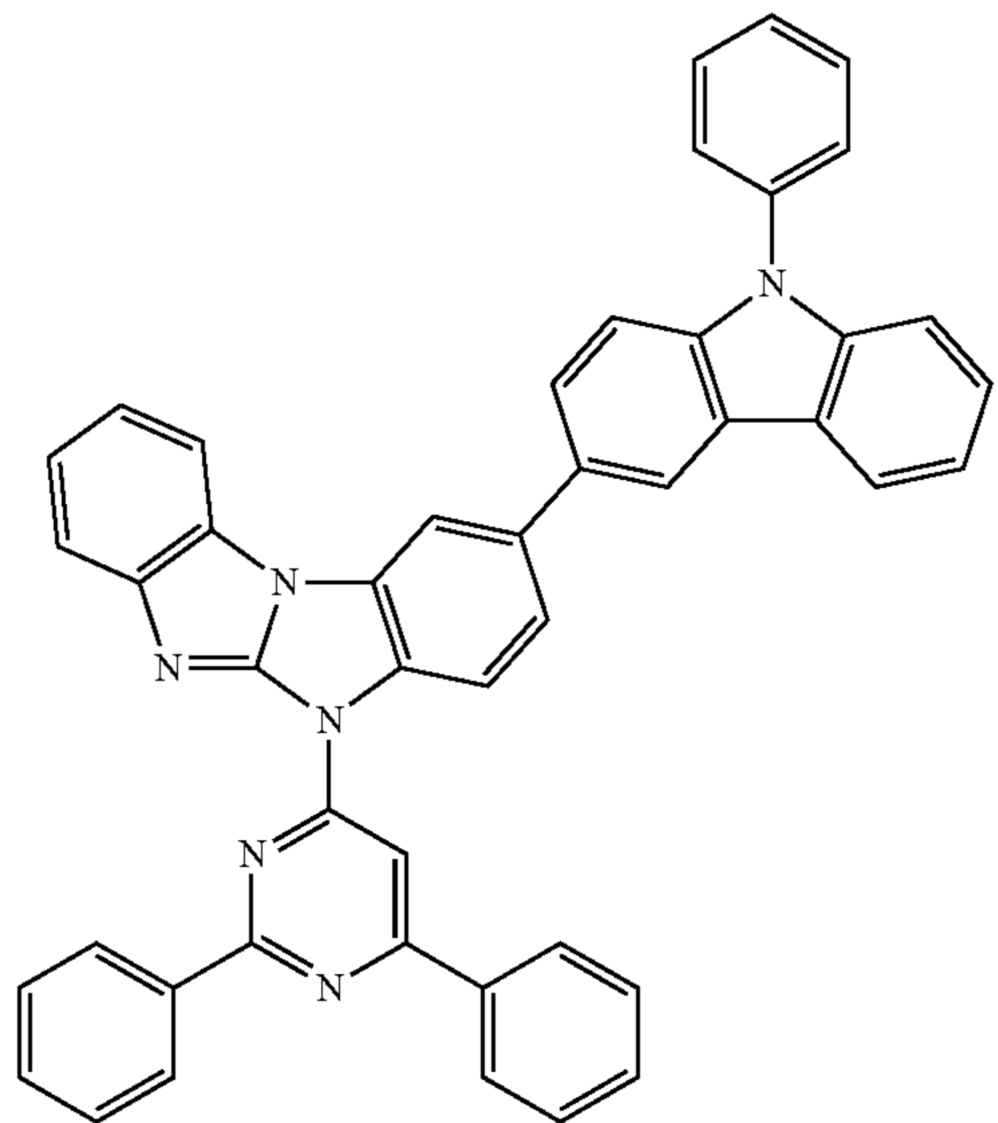
Compound 60
