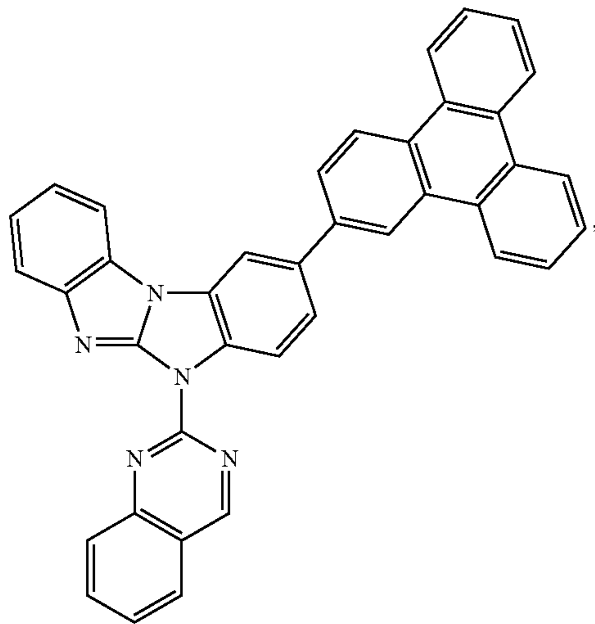
Compound 81
