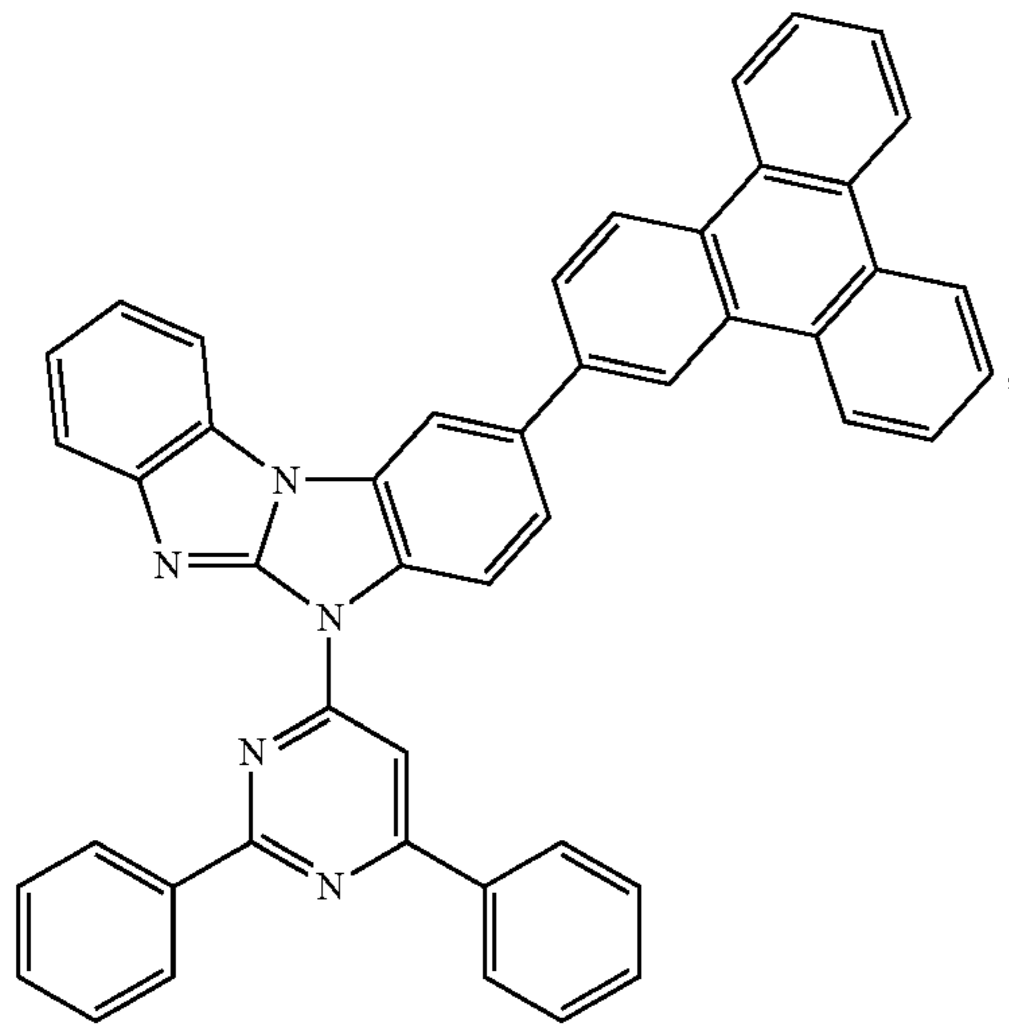
Compound 61
