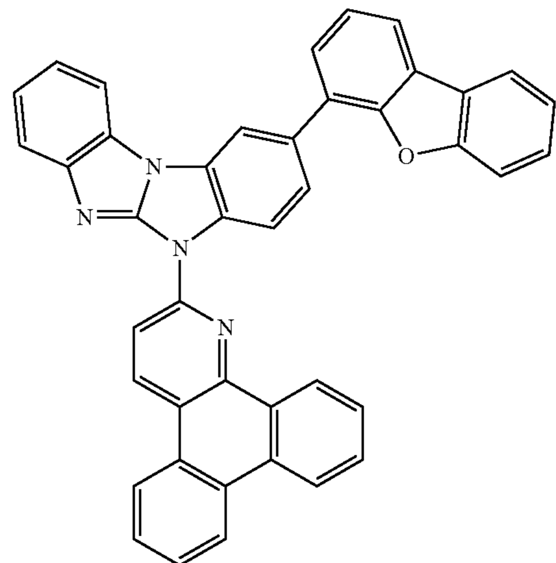
Compound 86
