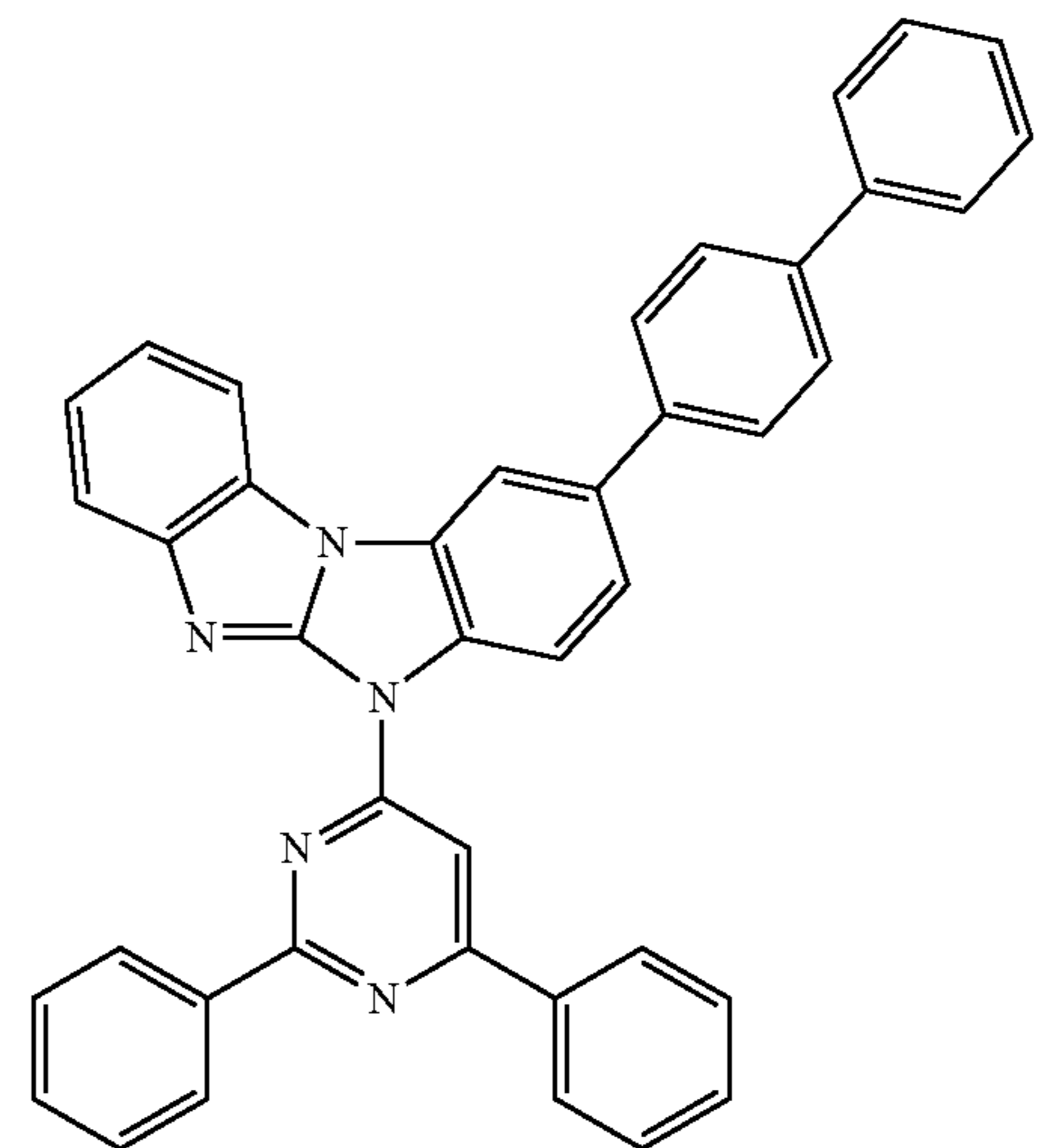
Compound 52
