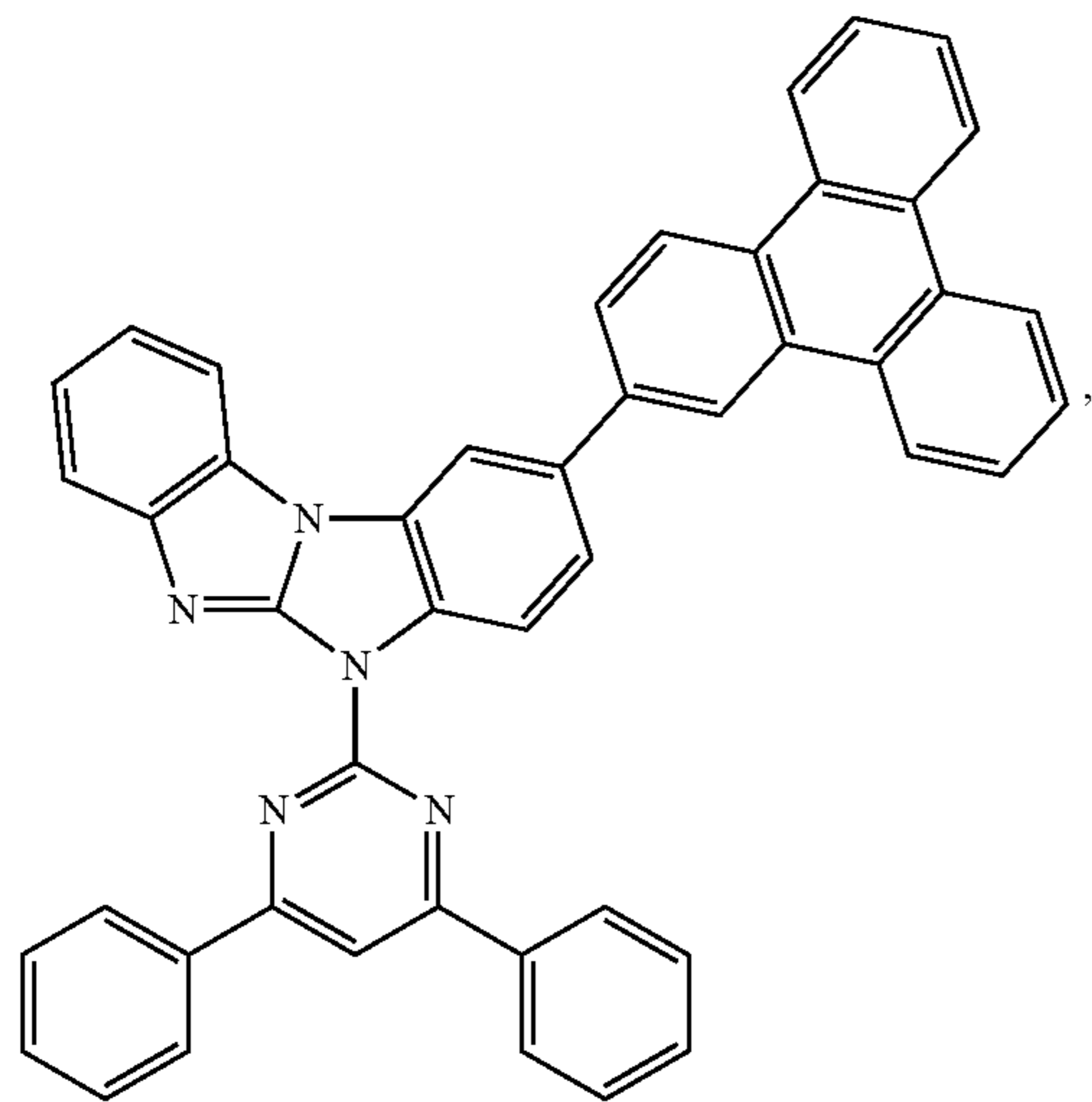
Compound 49
