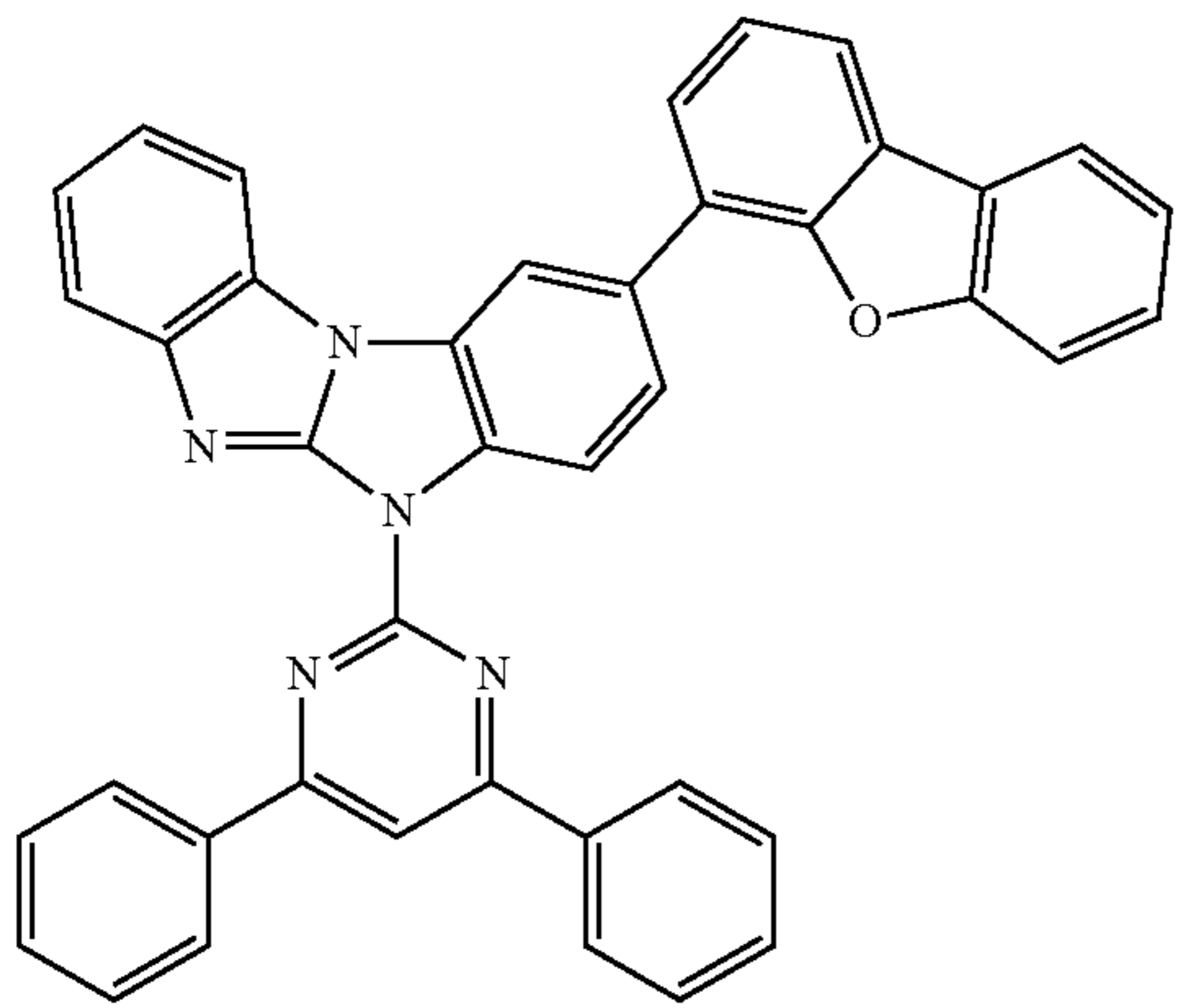
Compound 42
