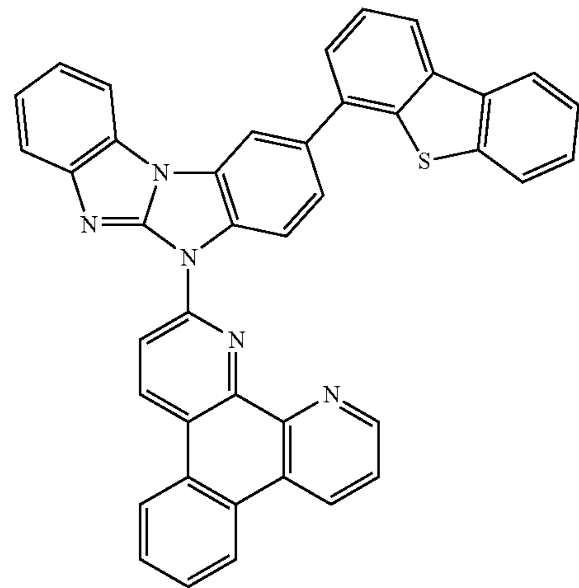
Compound 92
