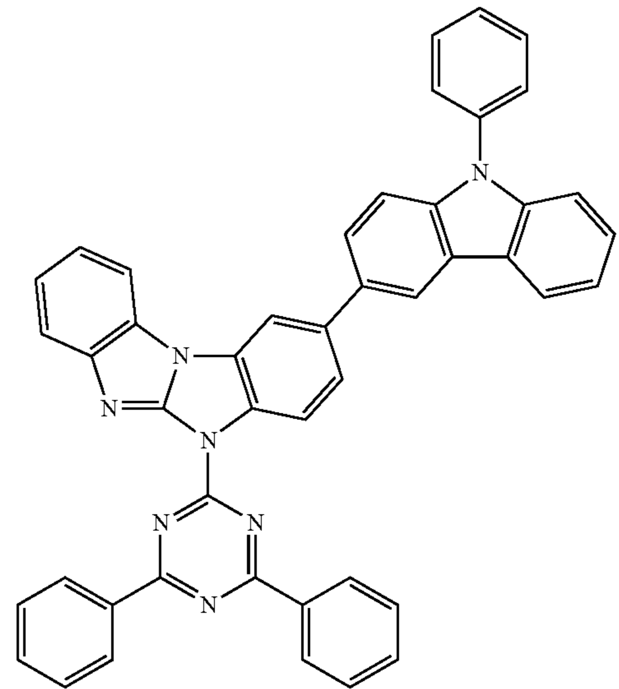
Compound 16
