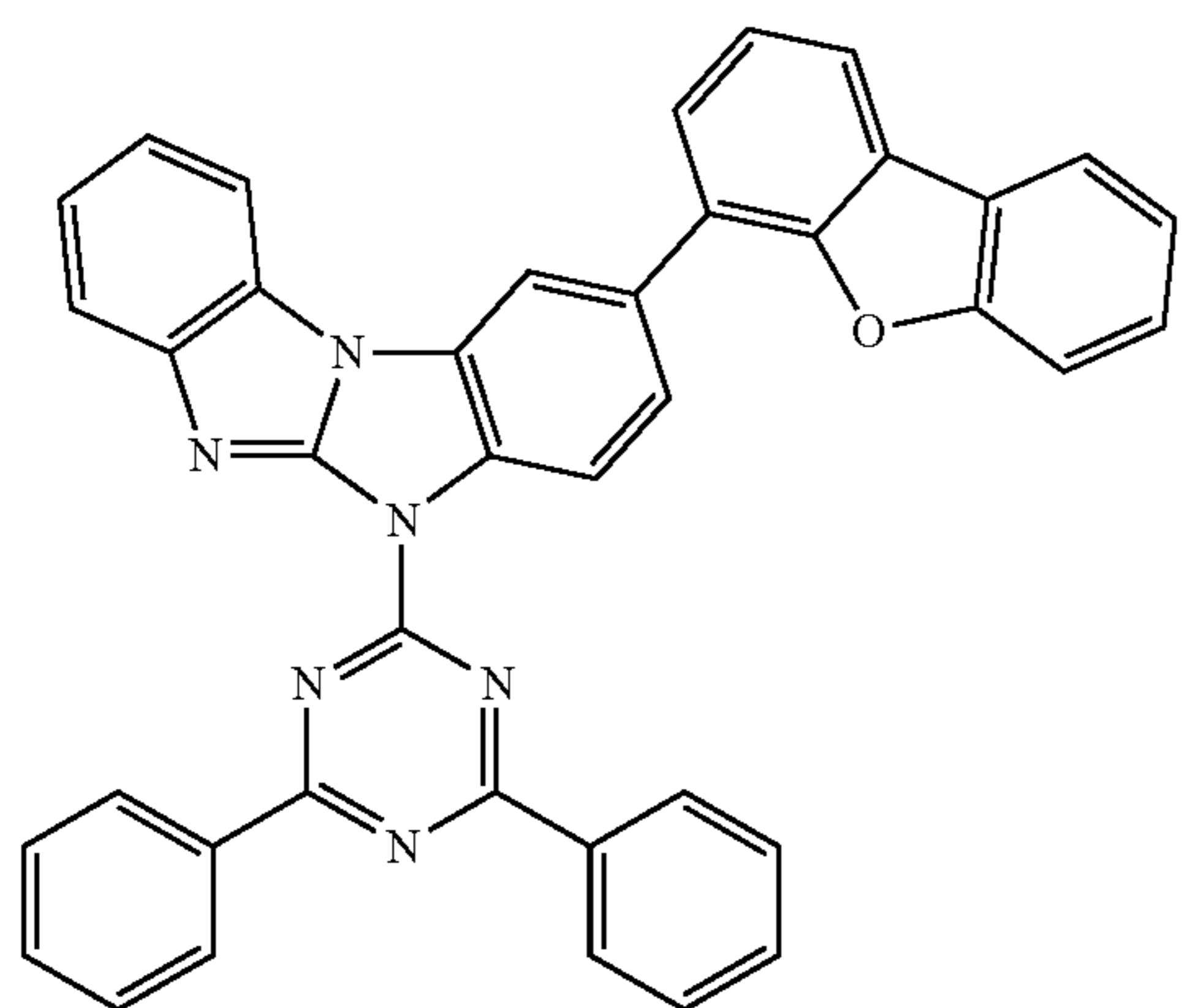
Compound 10
