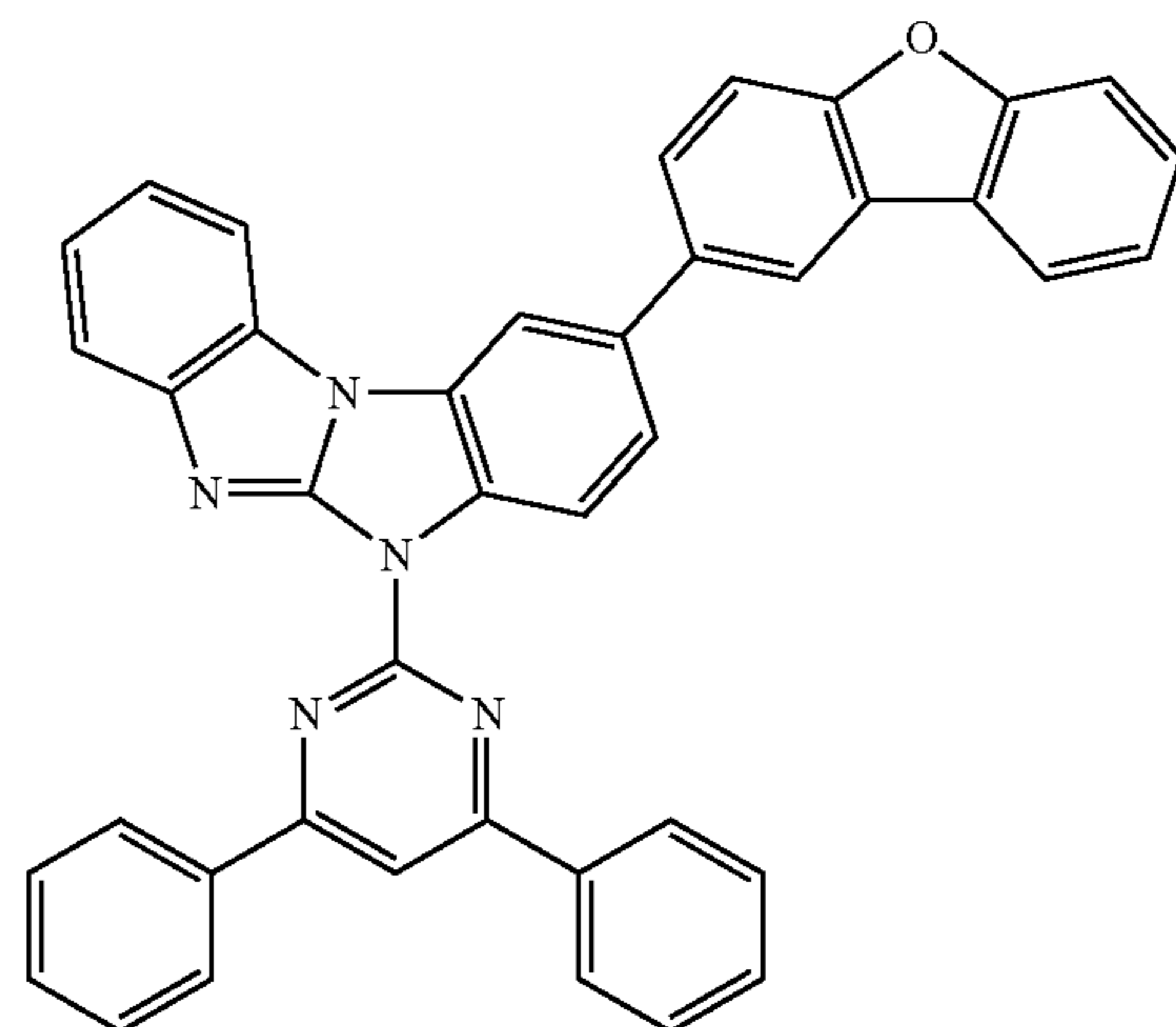
Compound 46
