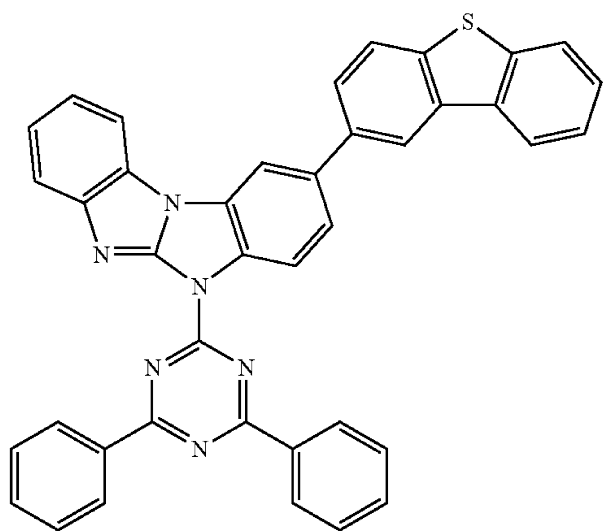
Compound 14
