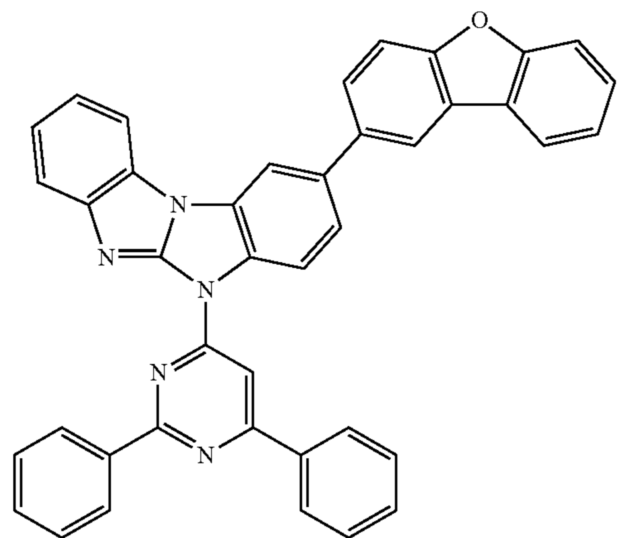
Compound 59
