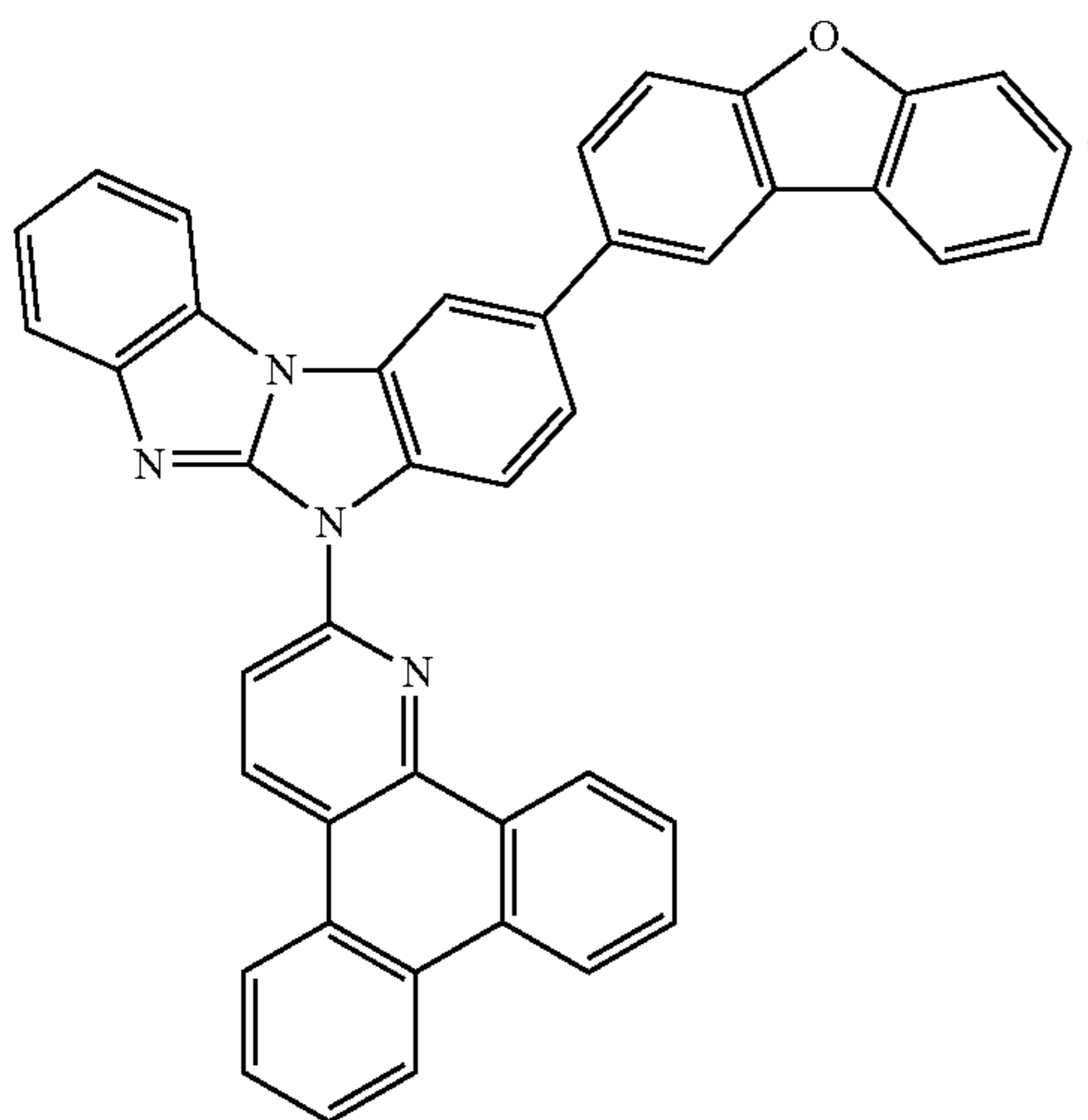
Compound 89
