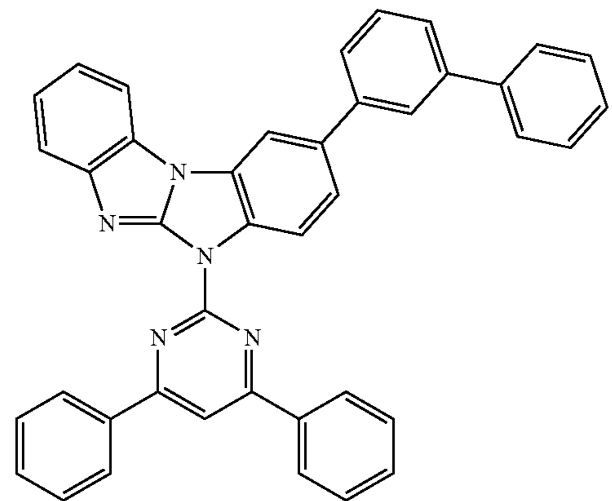
Compound 39
