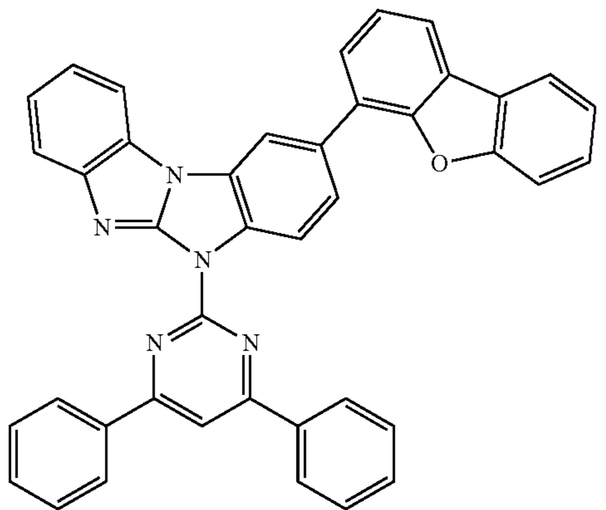
Compound 42
