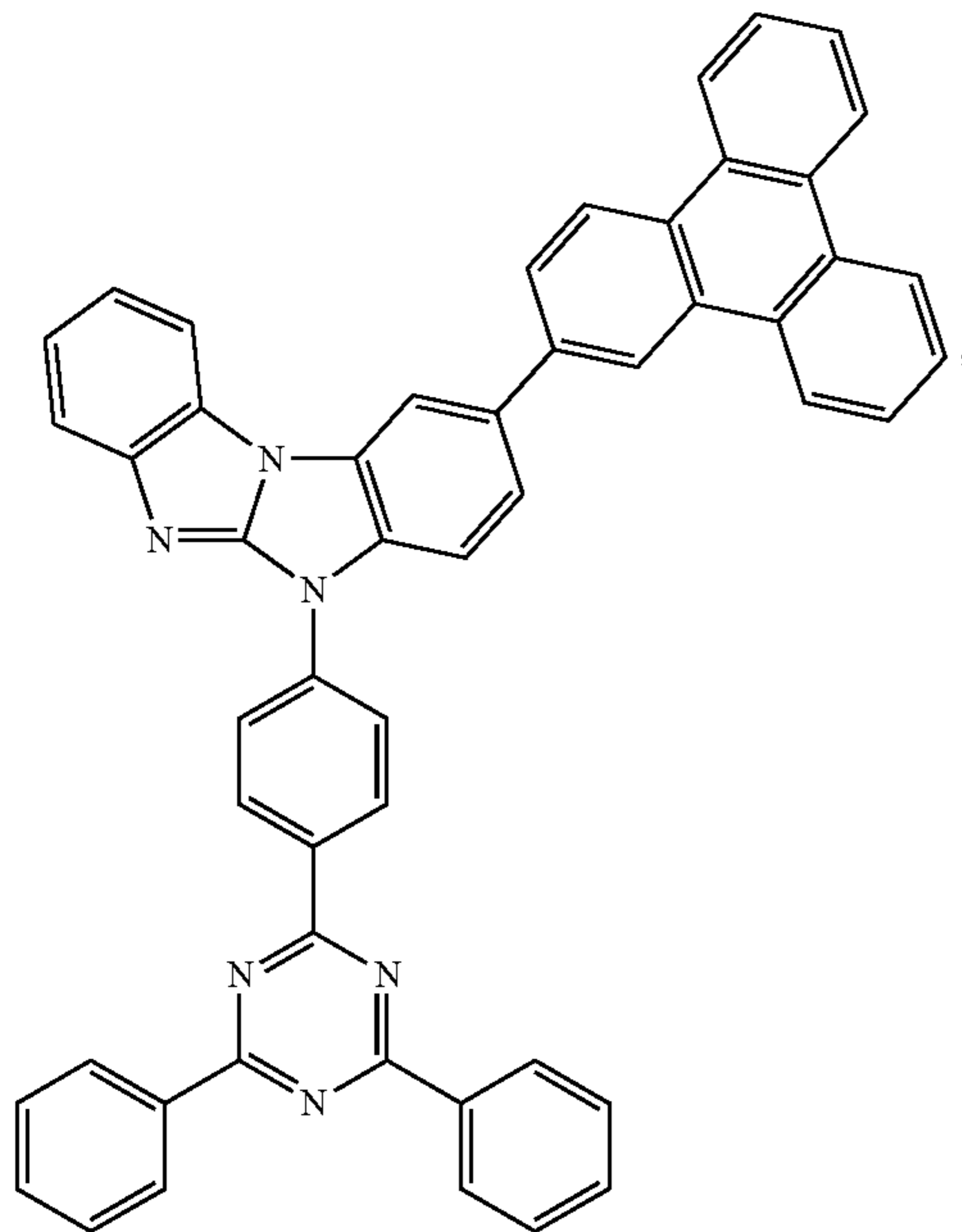
Compound 35
