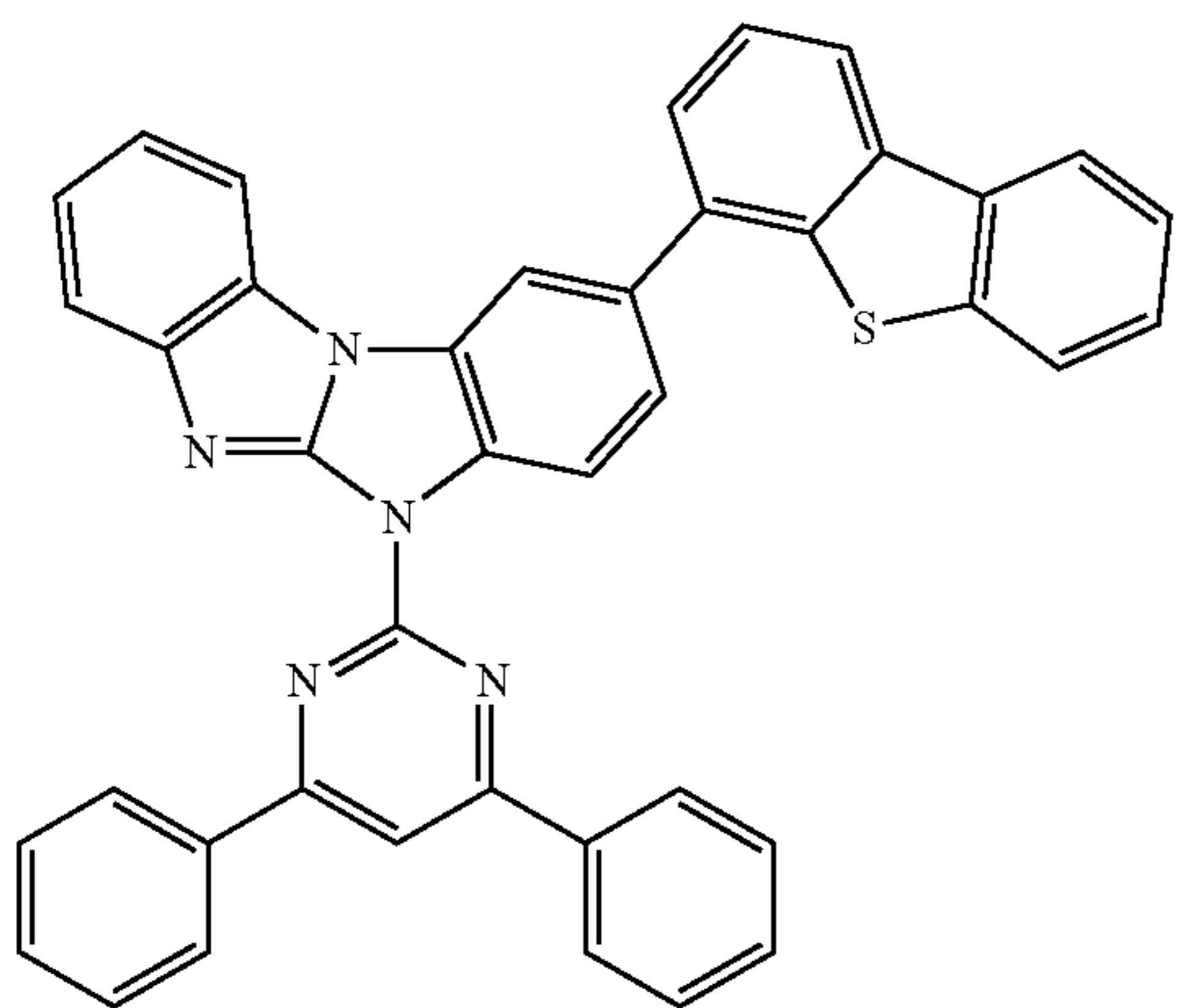
Compound 43
