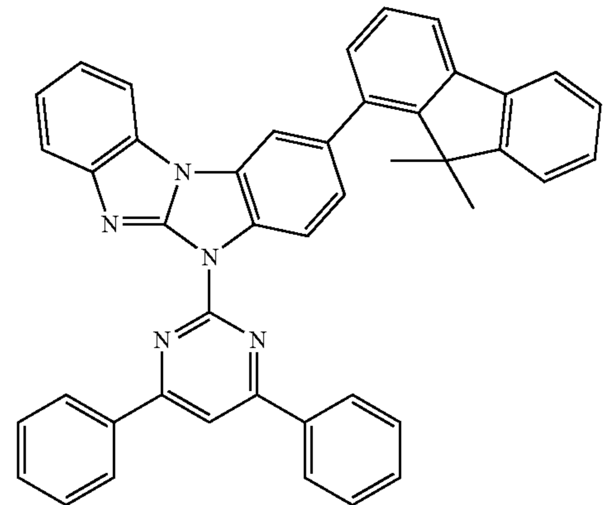
Compound 44
