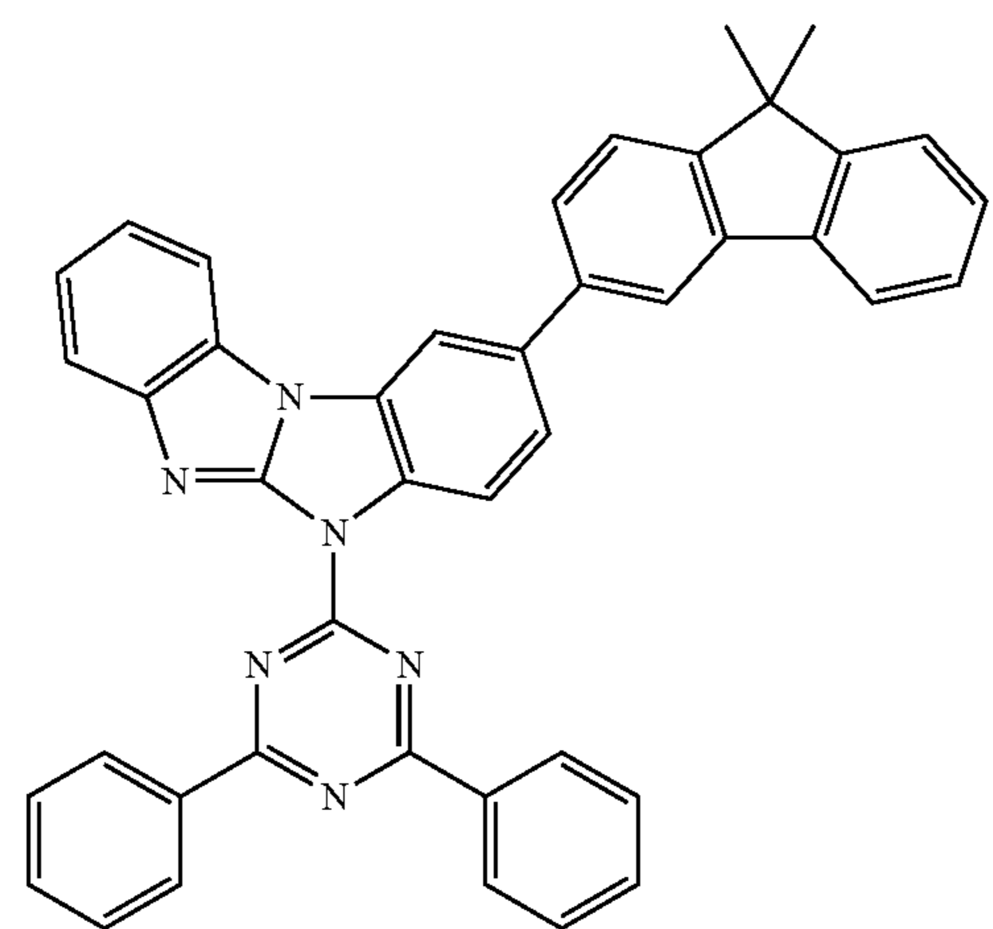
Compound 17
