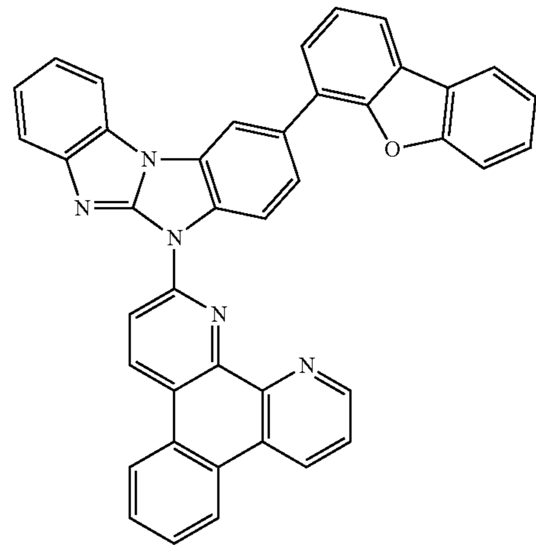
Compound 93
