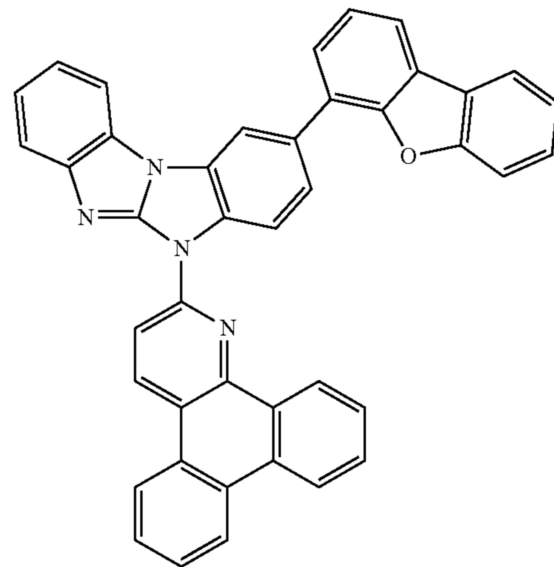
Compound 86
