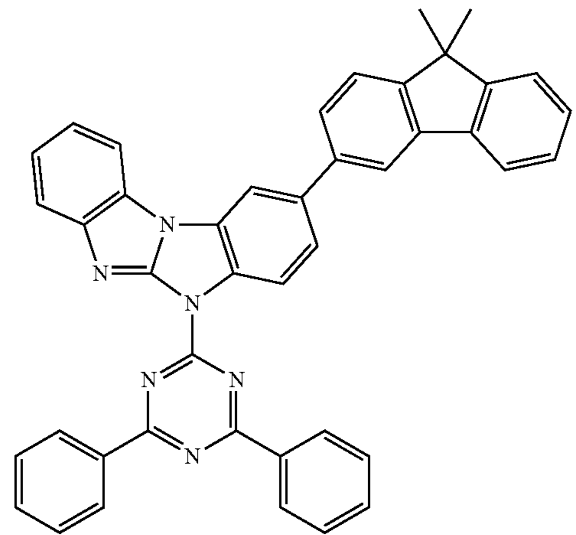
Compound 17
