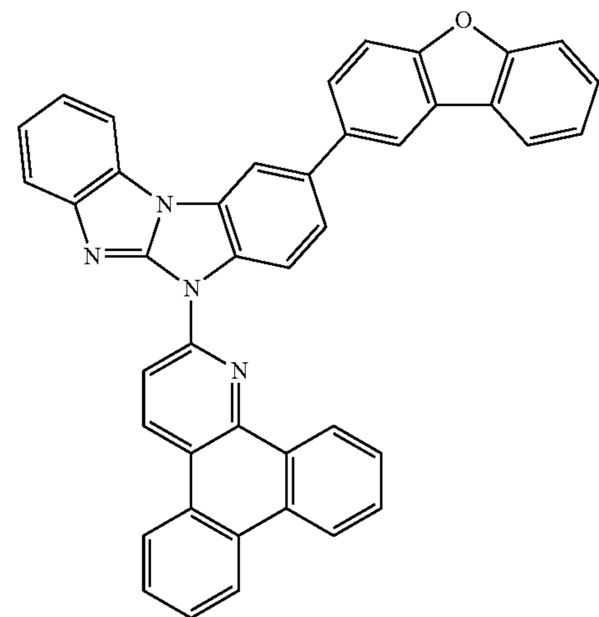
Compound 88
