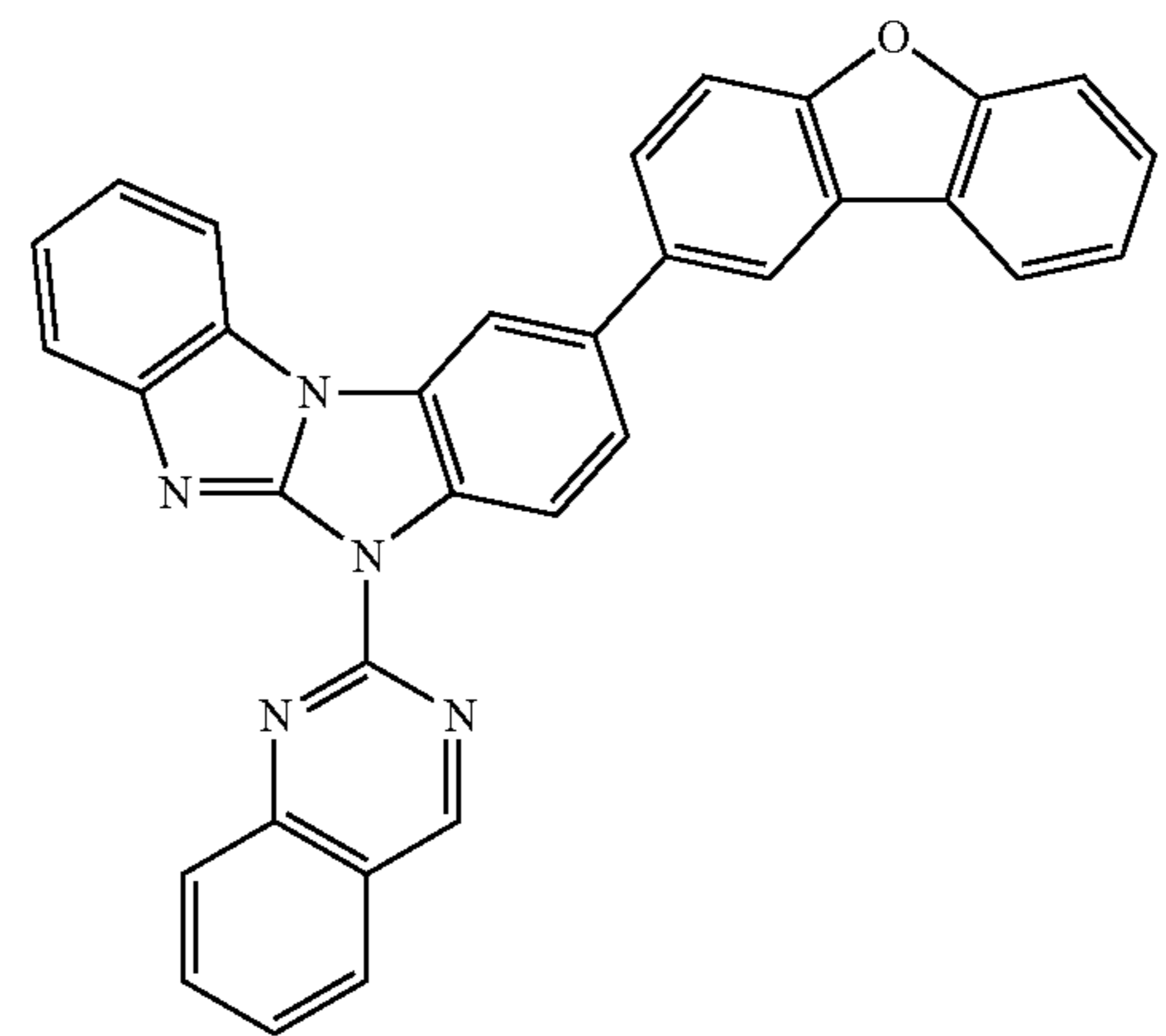
Compound 79
