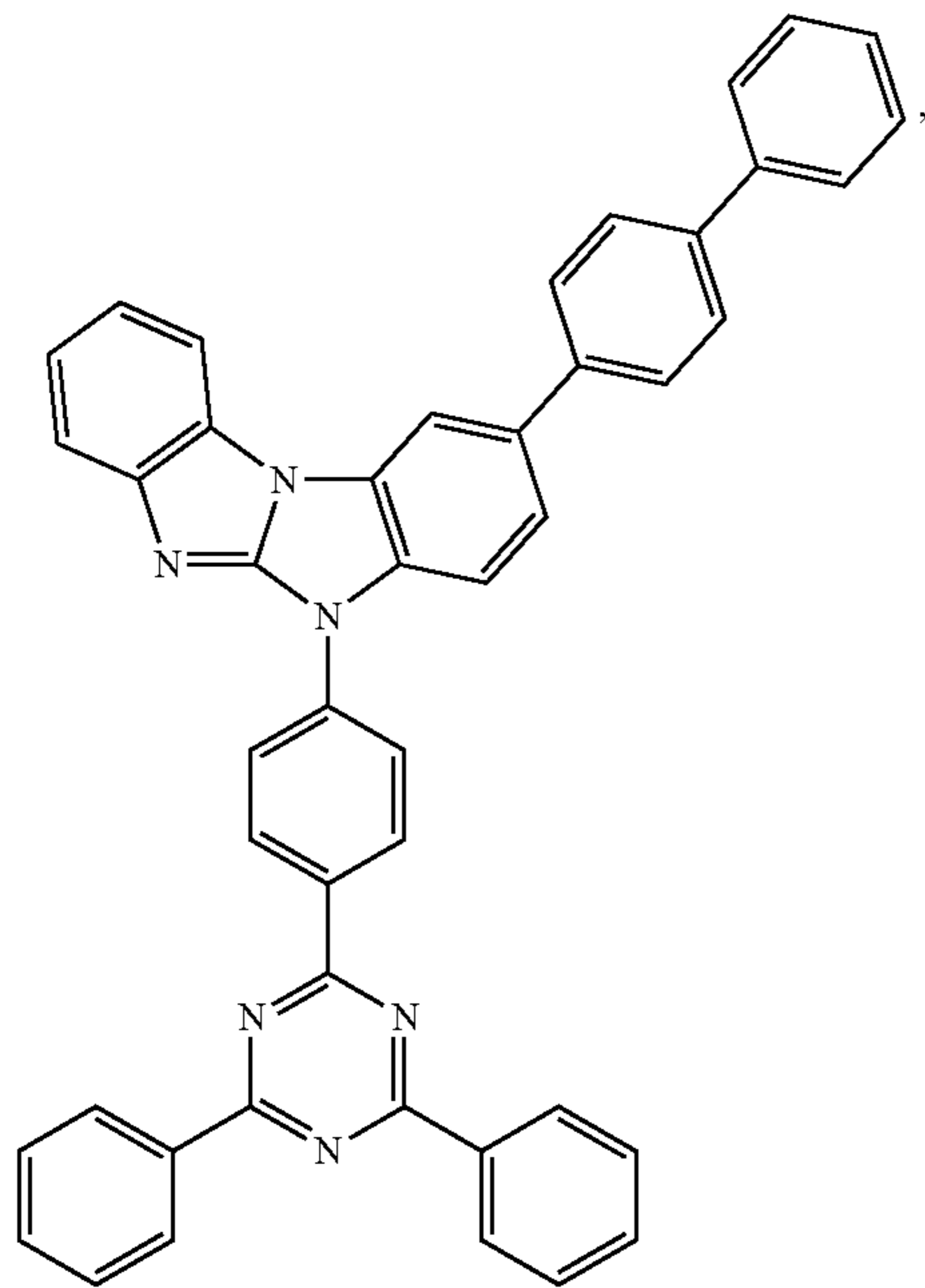
Compound 26
