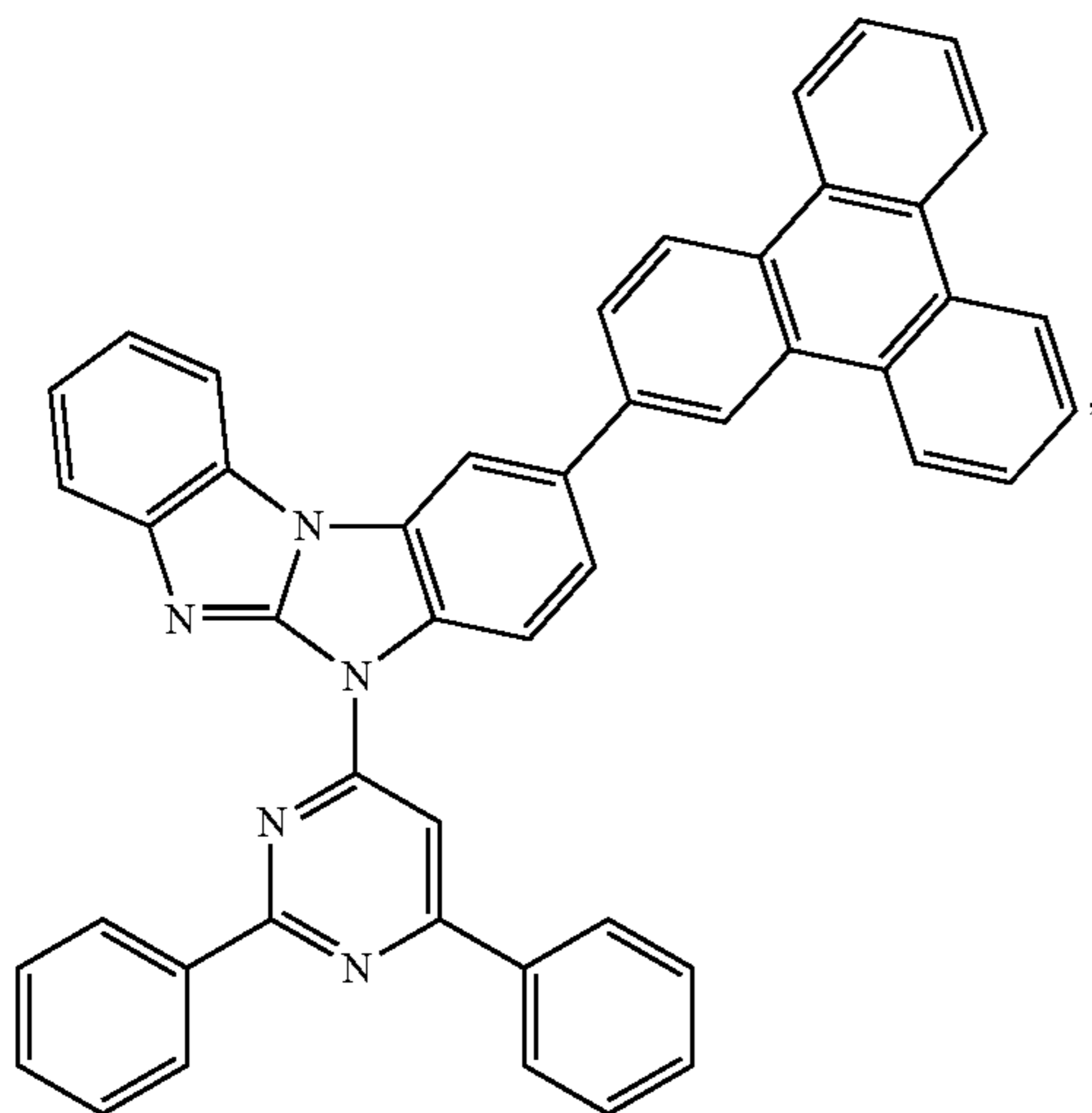
Compound 61
