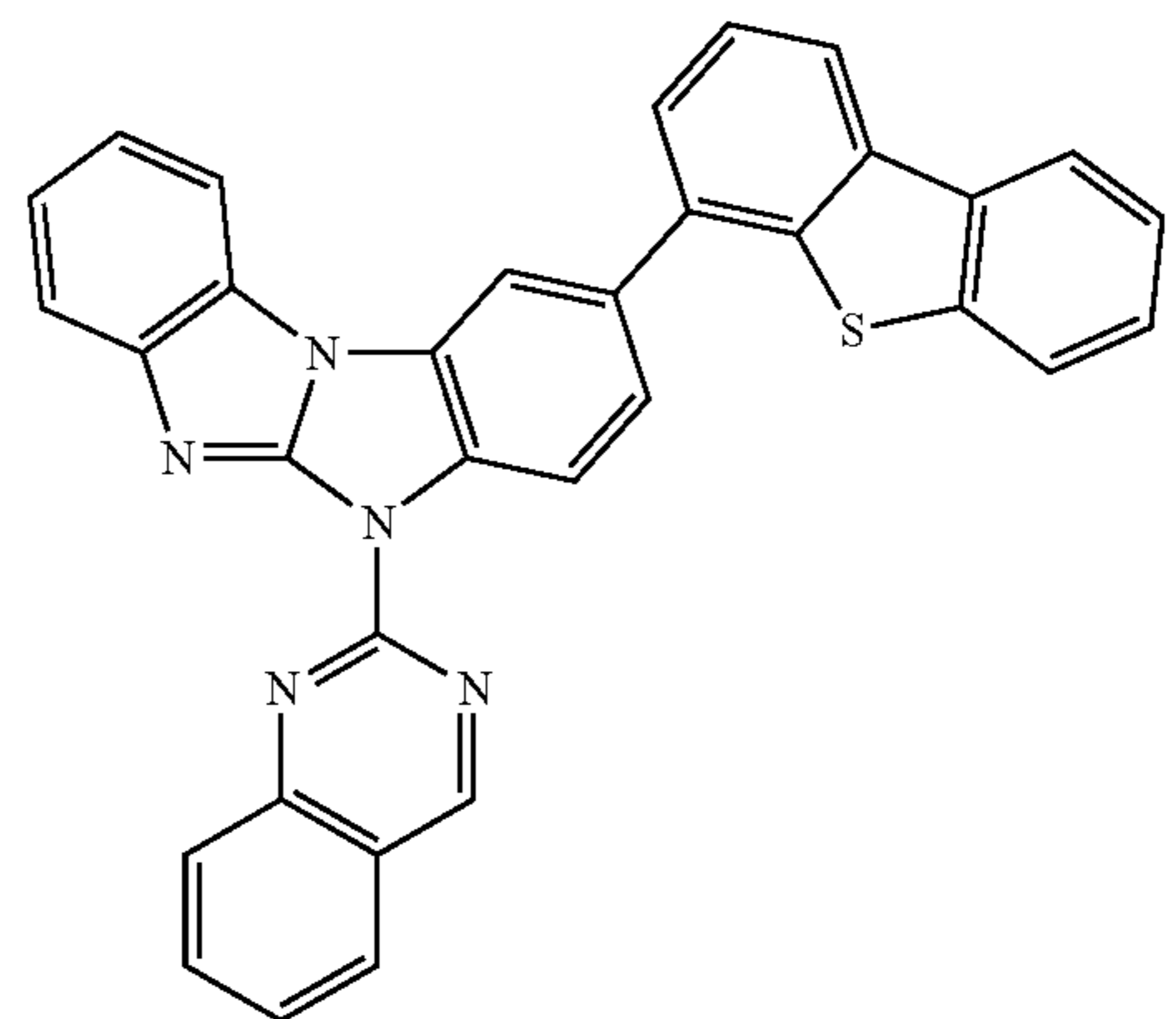
Compound 76
