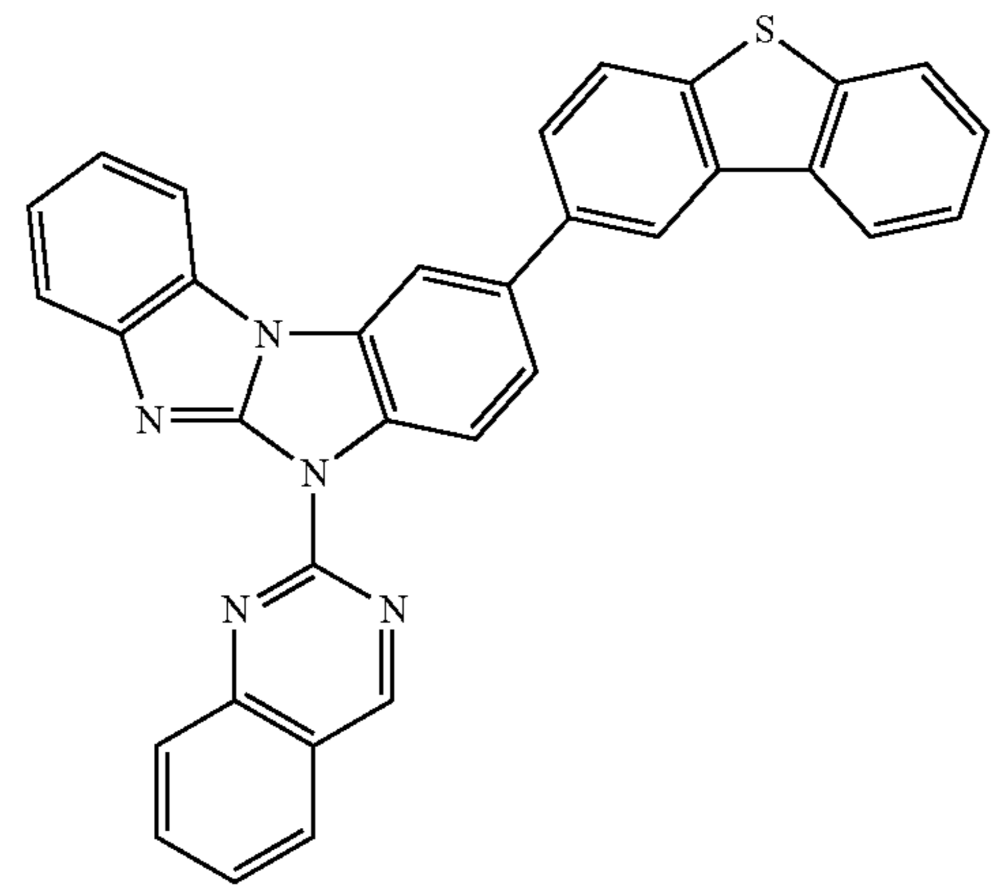
Compound 78
