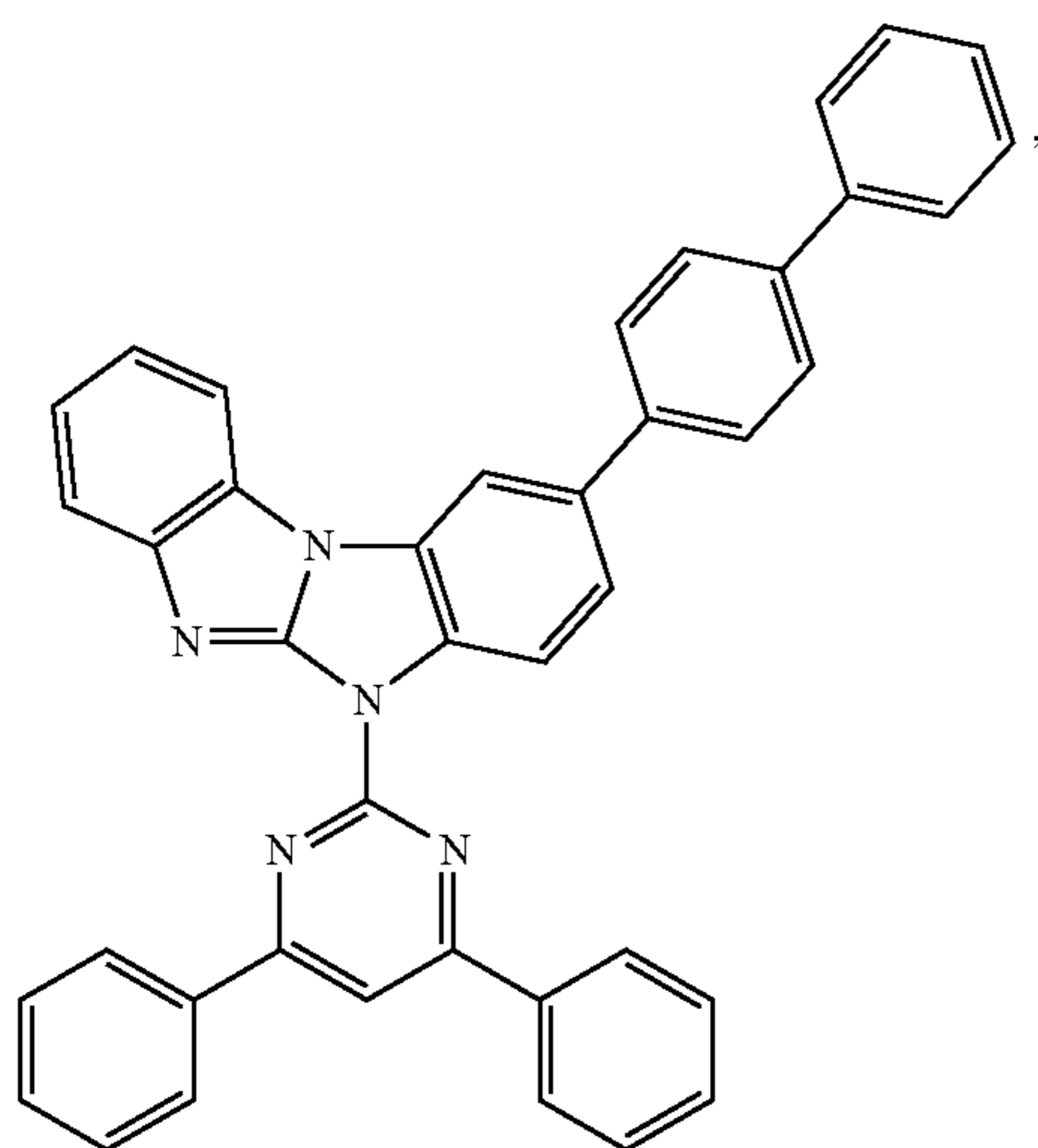
Compound 38
