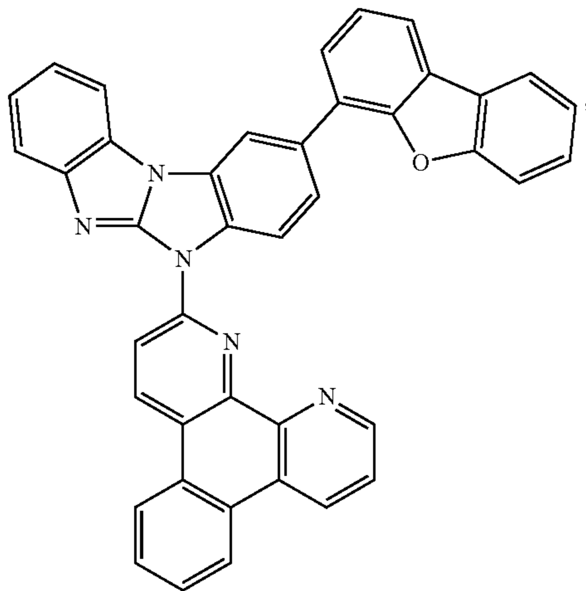
Compound 93
