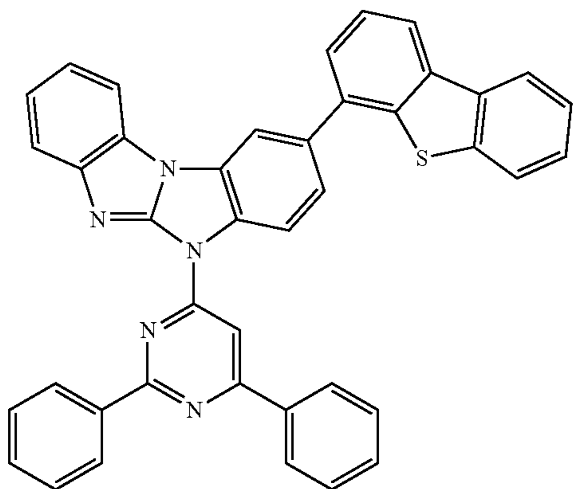
Compound 57
