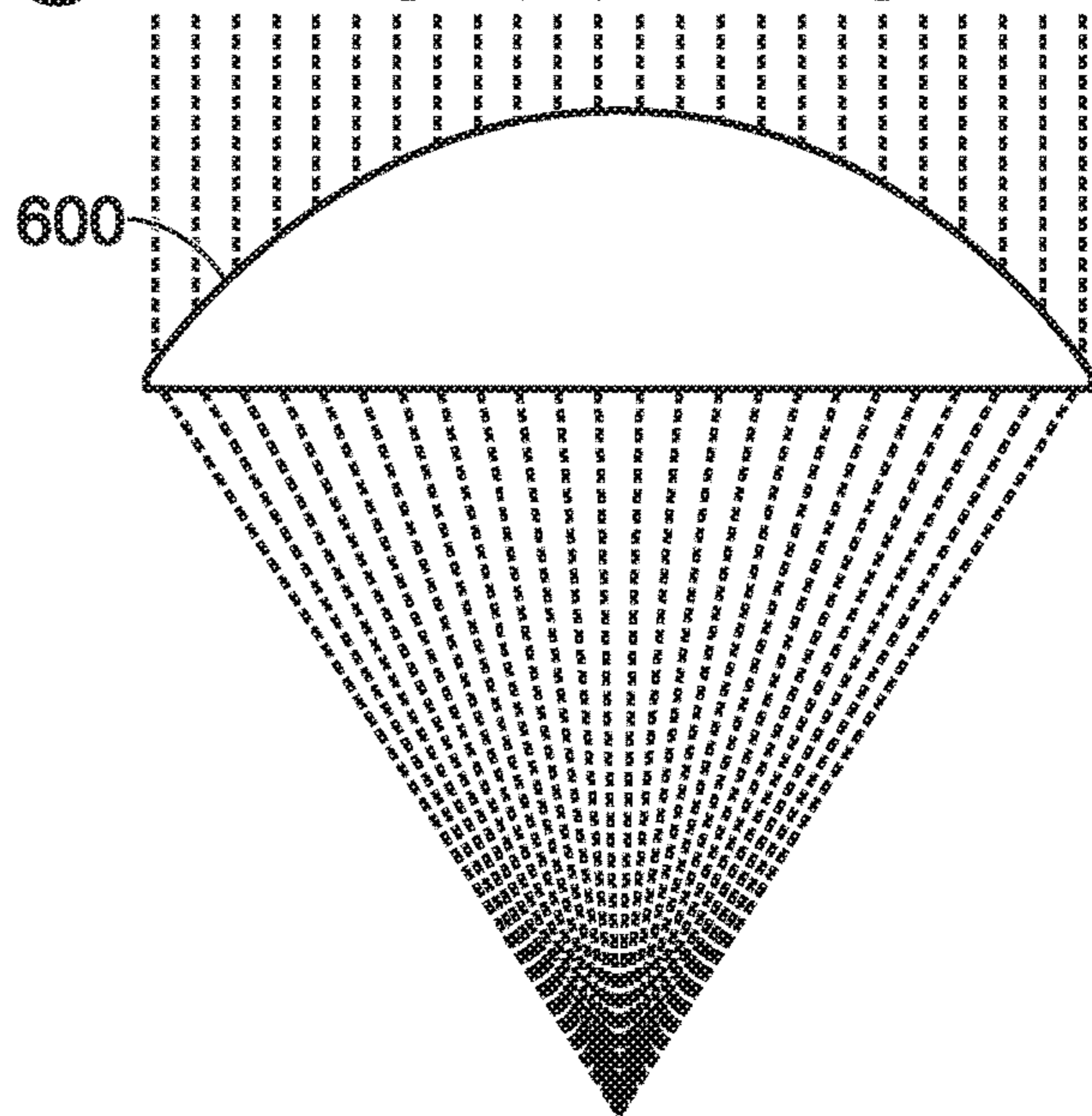
Fig. 8B ACYLINDER LENS
