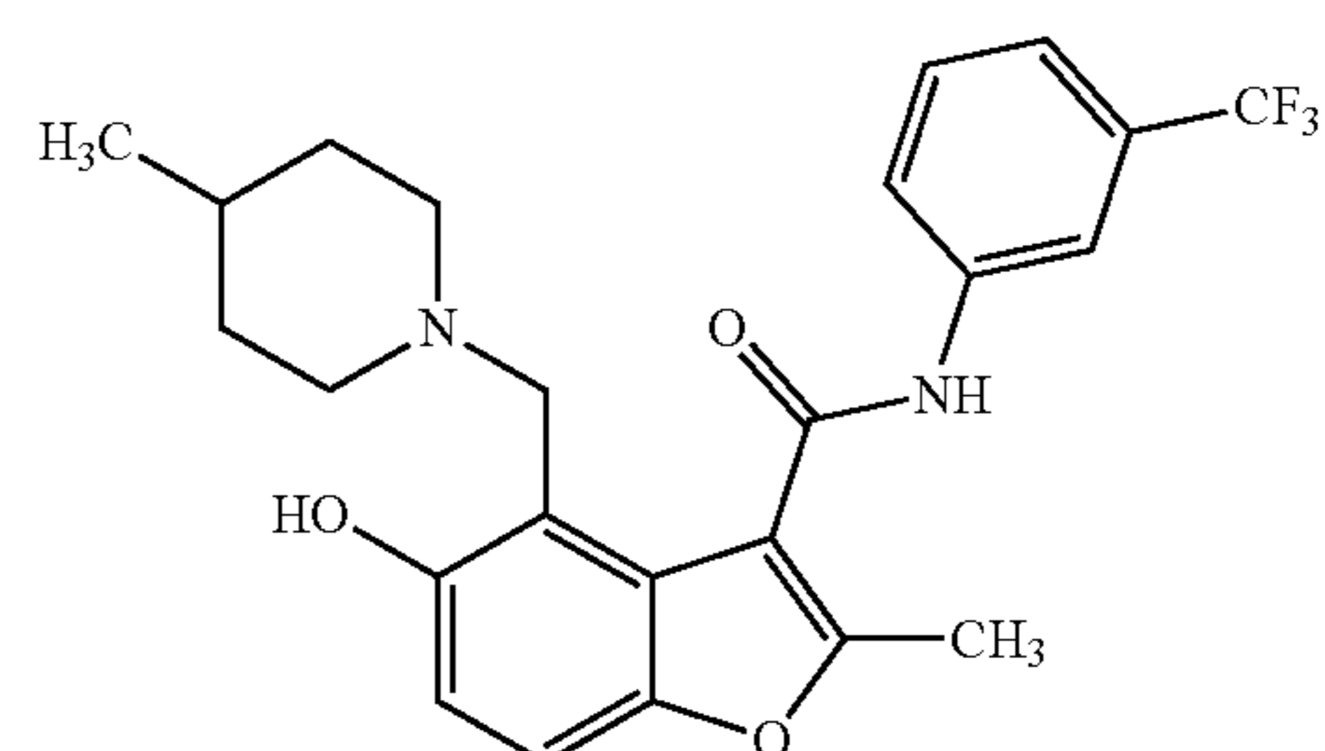
Compound 12
