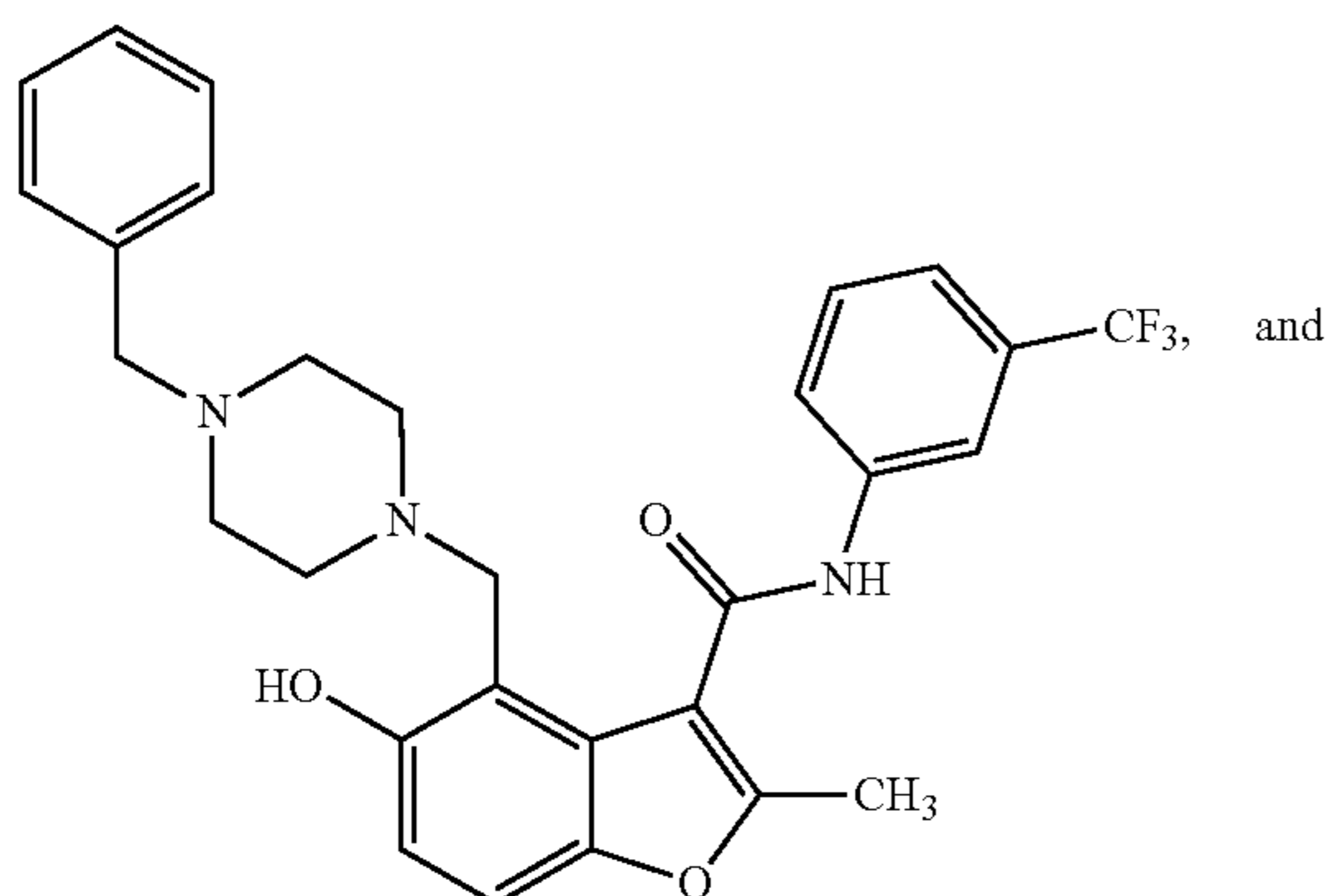
Compound 41
