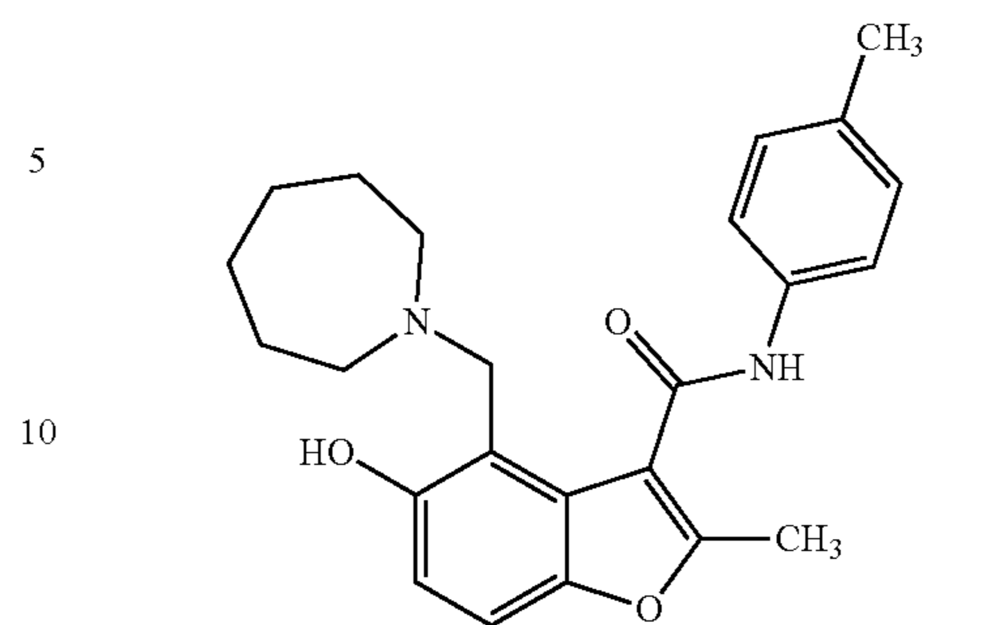
Compound 14
