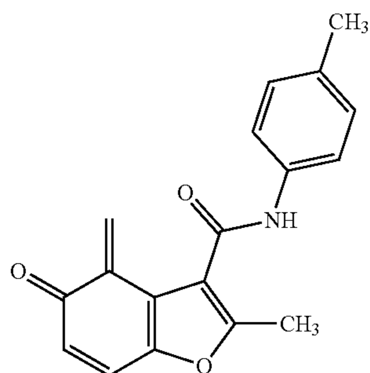
o-quinone methide
