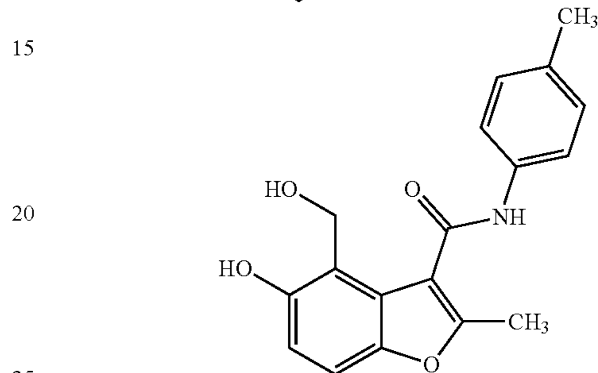
Hydrolyzed Compound
