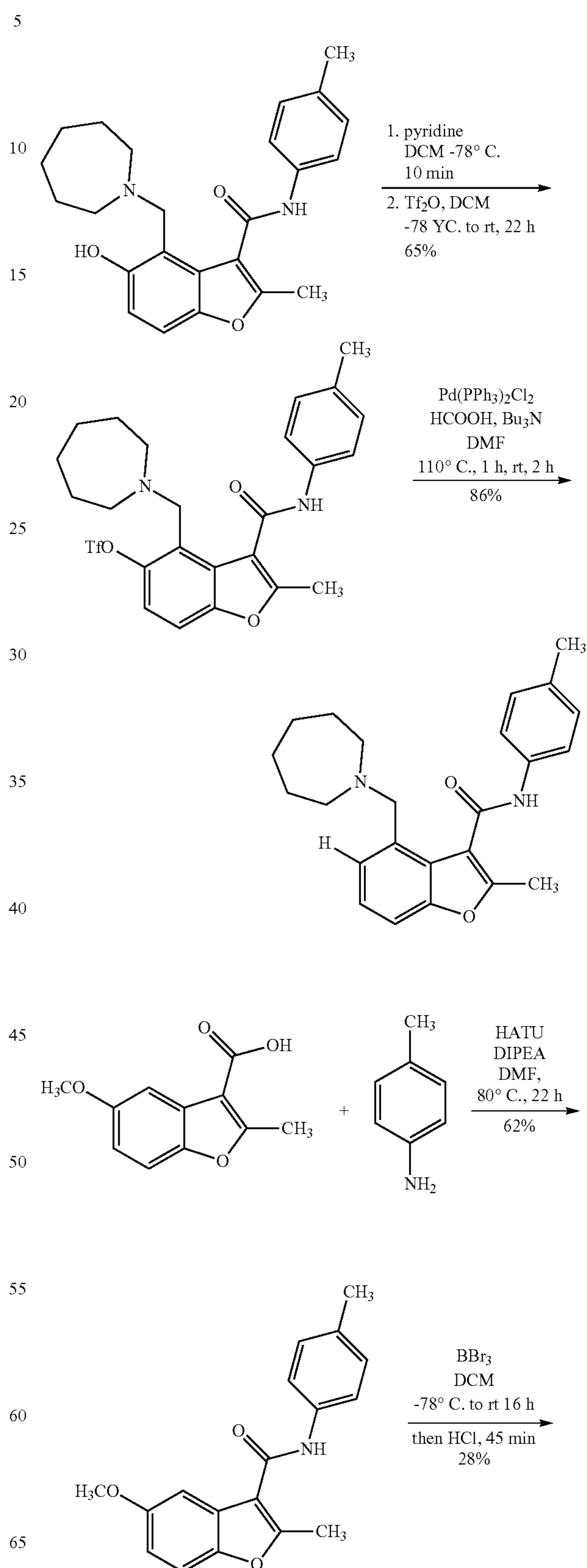
compound 1
