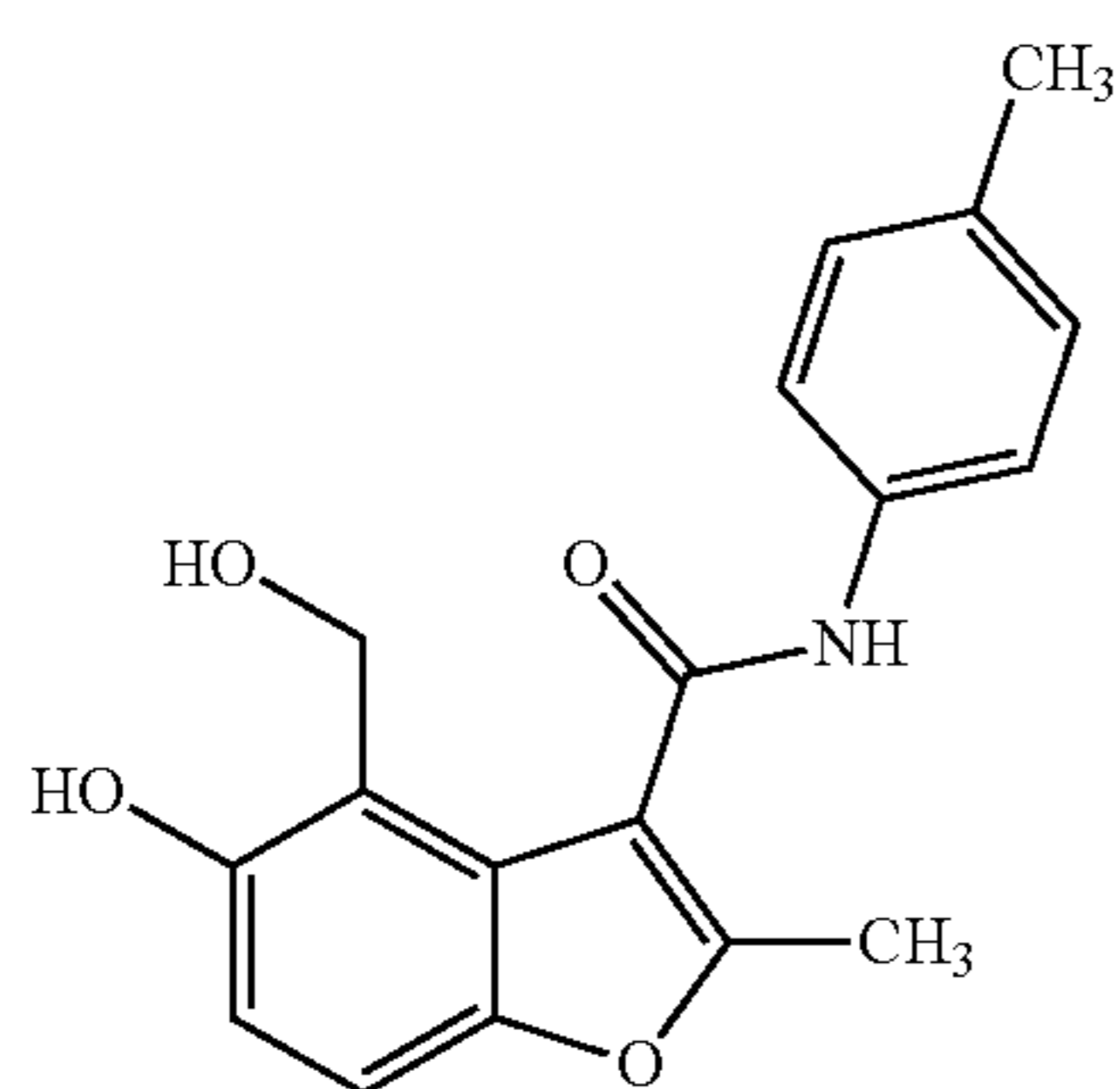
hydrolyzed compound
