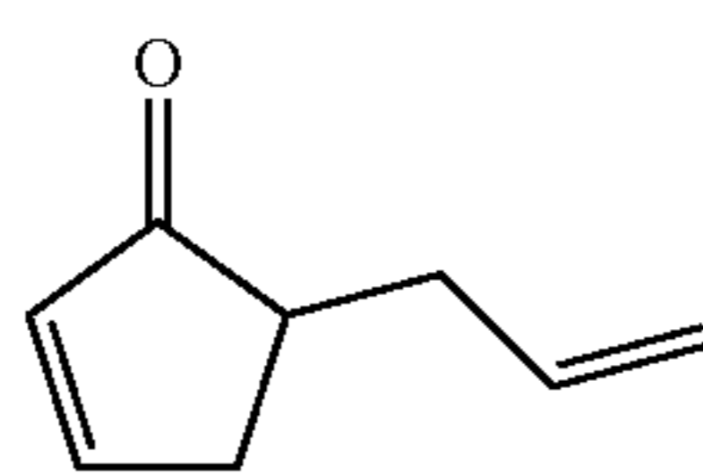
Step 3: 5-allylcyclopent-2-enone
