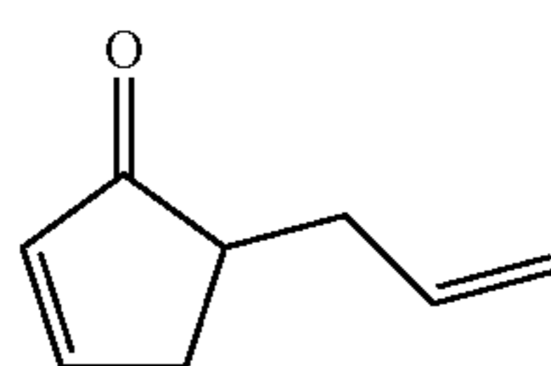
Step 3: 5-allylcyclopent-2-enone
