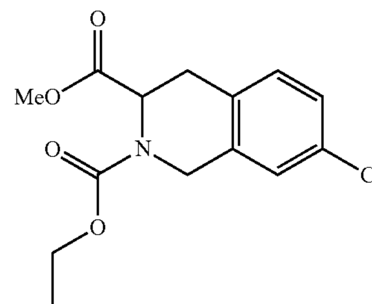
Step 3: 2-Ethyl 3-methyl 7-chloro-3,4-dihydroisoquinoline-2,3(1H)-dicarboxylate
