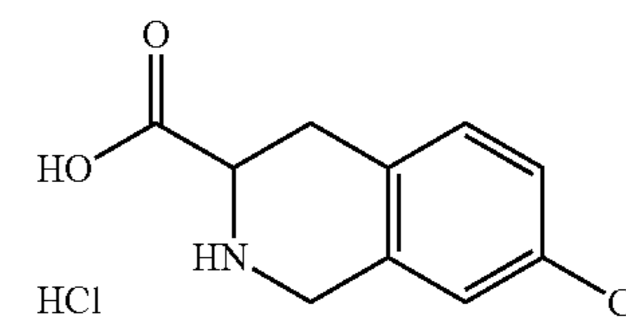
Step 4: 7-chloro-1,2,3,4-tetrahydroisoquinoline-3-carboxylic acid hydrochloride
