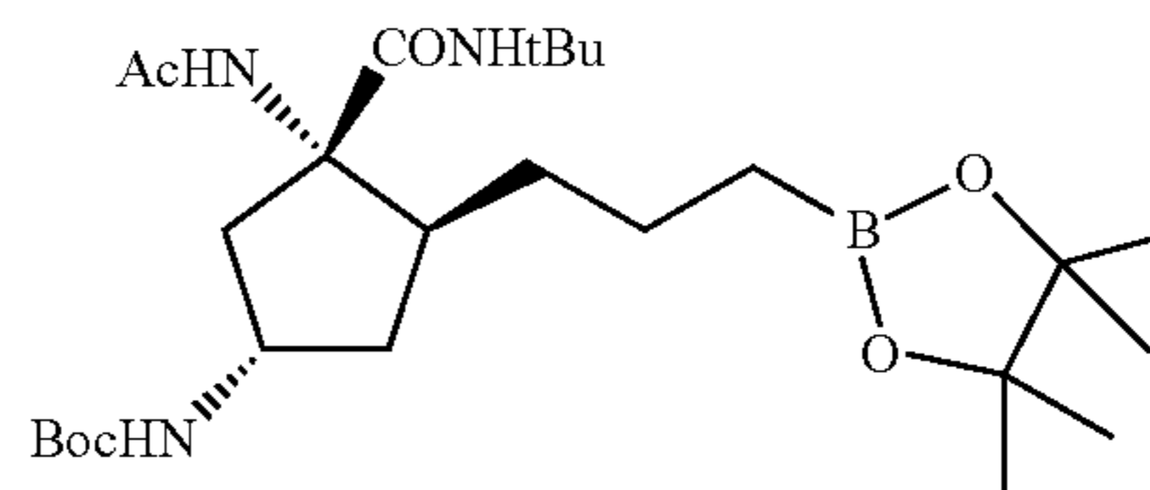
Step 6: tert-butyl (1S,3S,4S)-3-acetamido-3-(tert-butylcarbamoyl)-4-(3-(4,4,5,5-tetramethyl-1,3,2-dioxaborolan-2-yl)propyl)cyclopentylcarbamate
