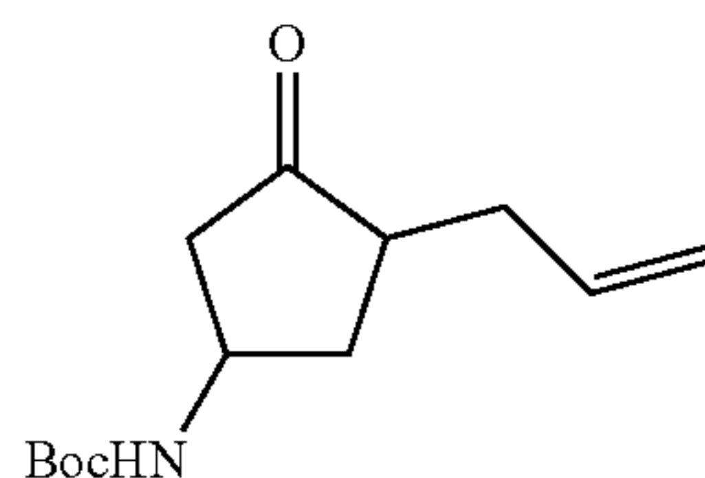
Step 4. tert-butyl 3-allyl-4-oxocyclopentylcarbamate
