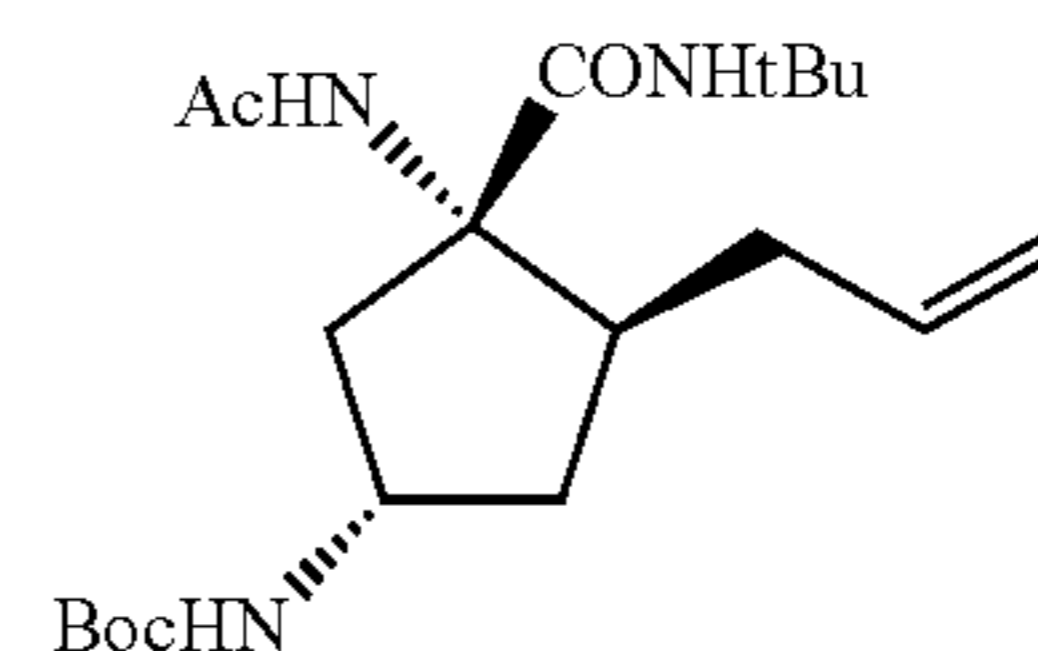
Step 5: tert-butyl (1S,3S,4S)-3-acetamido-4-allyl-3-(tert-butylcarbamoyl)cyclopentylcarbamate
