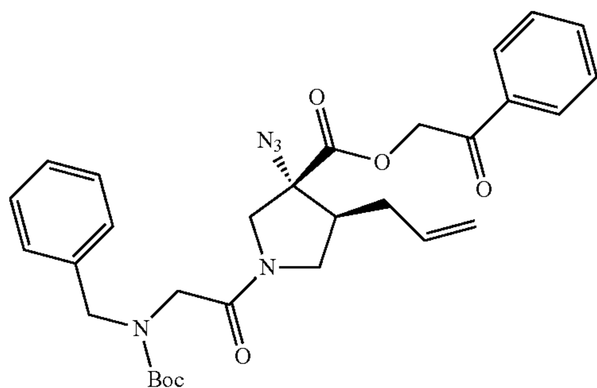
Step 2: 2-Oxo-2-phenylethyl (3R,4S)-4-allyl-3-azido-1-[N-benzyl-N-(tert-butoxycarbonyl)glycyl]pyrrolidine-3-carboxylate
