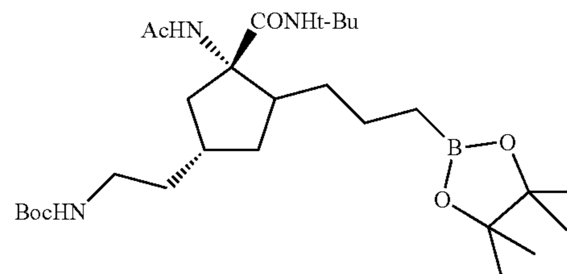
Step 5: tert-butyl 2-((1R,3S)-3-acetamido-3-(tert-butylcarbamoyl)-4-(3-(4,4,5,5-tetramethyl-1,3,2-dioxaborolan-2-yl)propyl)cyclopentyl)ethylcarbamate
