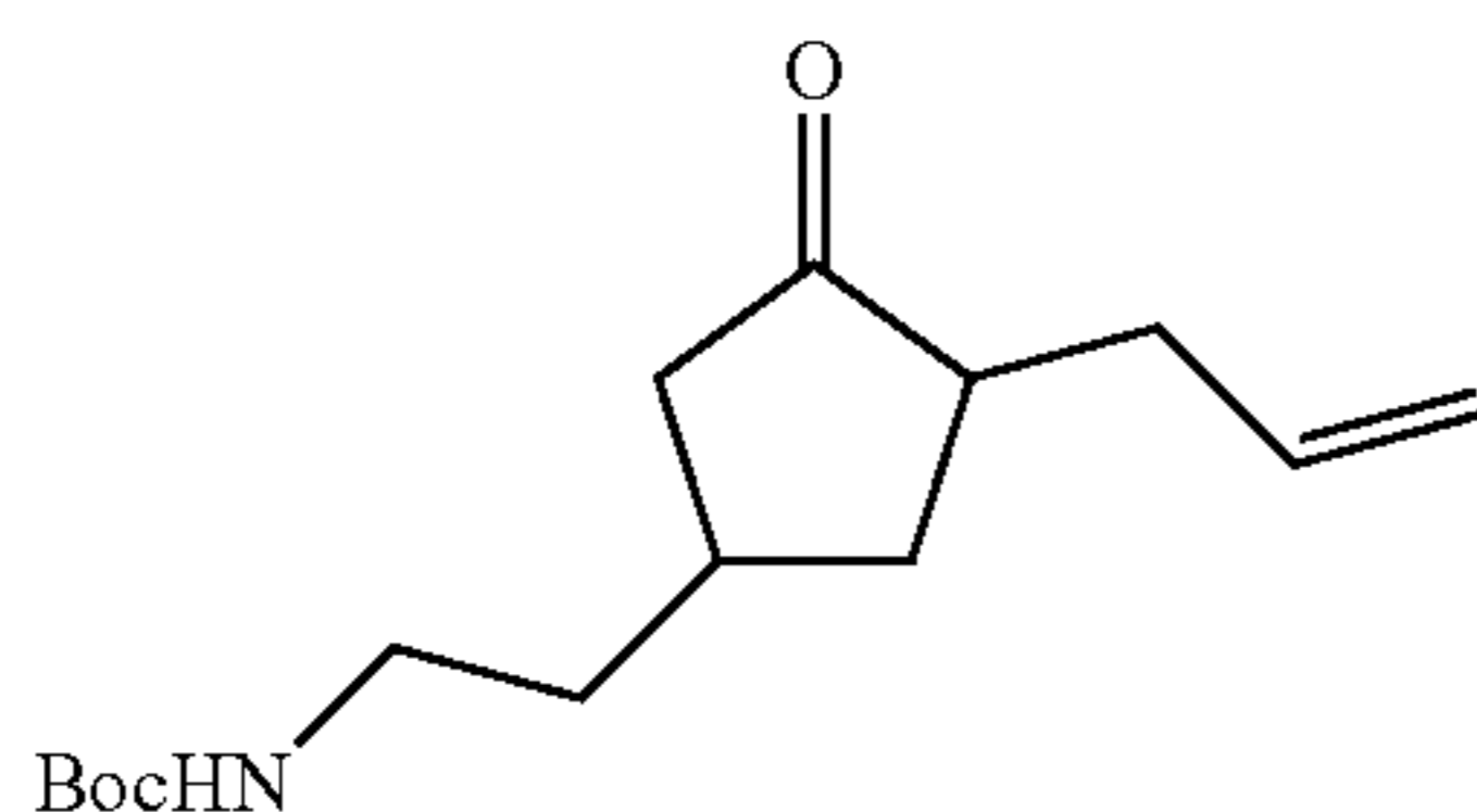
Step 3: tert-butyl 2-(3-allyl-4-oxocyclopentyl)ethylcarbamate
