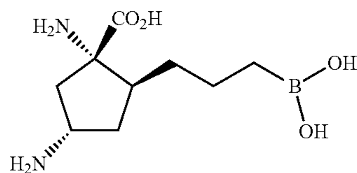
Step 7: (1S,2S,4S)-1,4-diamino-2-(3-boronopropyl)cyclopentanecarboxylic acid (Racemic)
