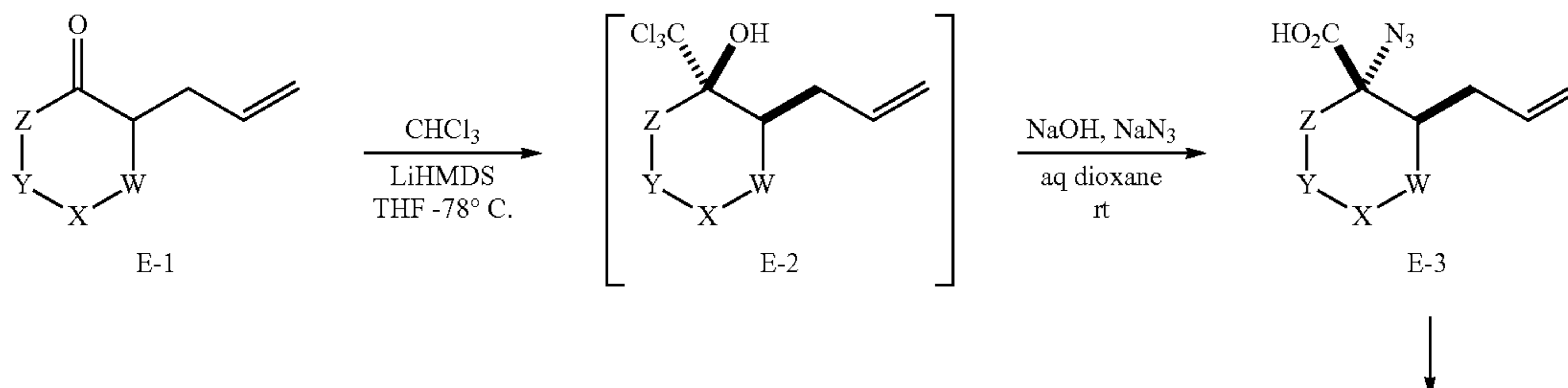
Scheme E
