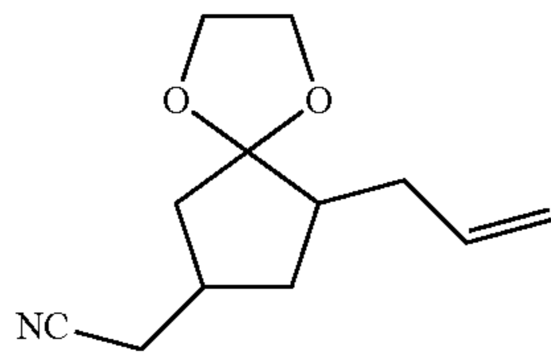
Step 2: 2-(9-allyl-1,4-dioxaspiro[4.4]nonan-7-yl)acetonitrile
