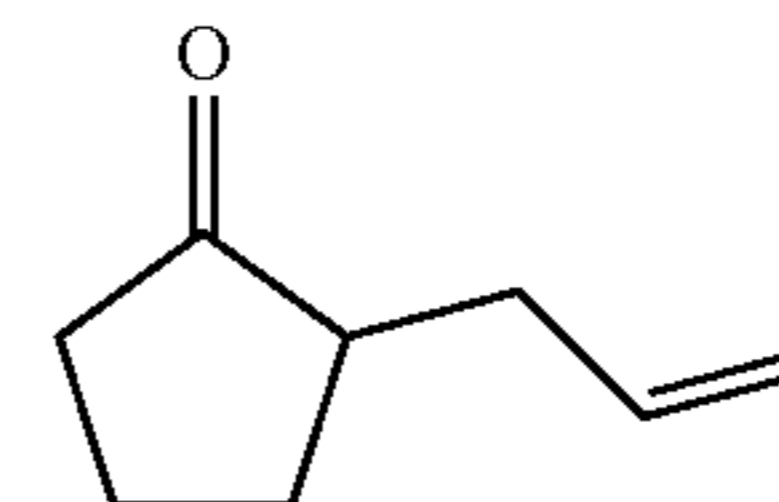
Step 1: 2-allylcyclopentanone
