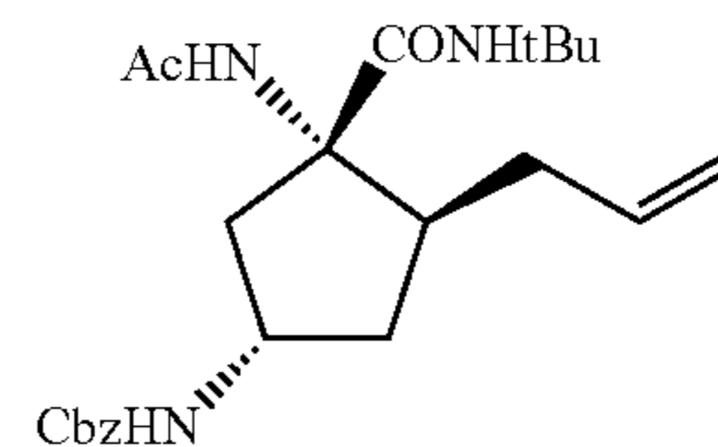
Step 2: benzyl (1S,3S,4S)-3-acetamido-4-allyl-3-(tert-butylcarbamoyl)cyclopentylcarbamate
