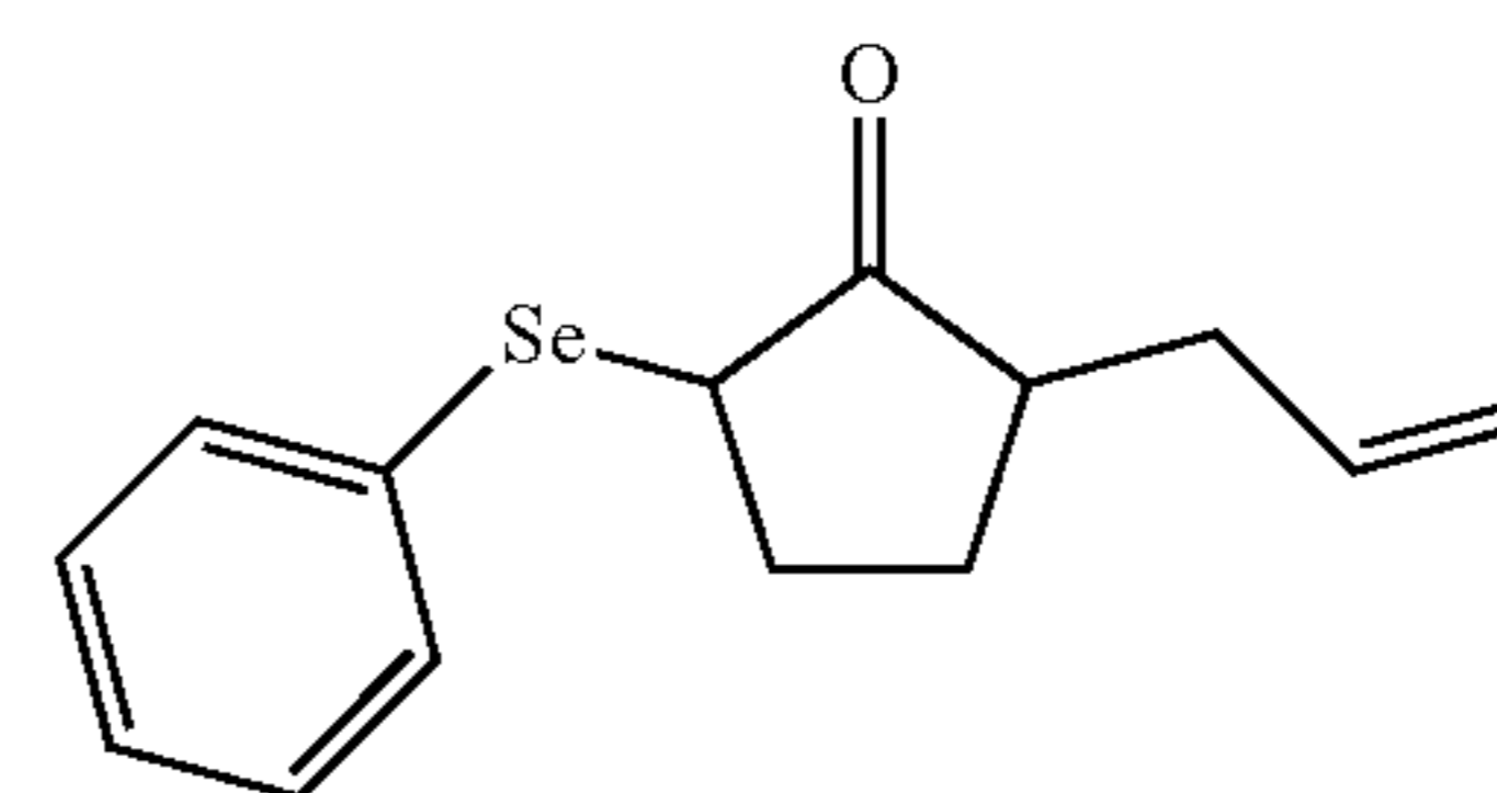
Step 2: 2-allyl-5-(phenylselanyl)cyclopentanone
