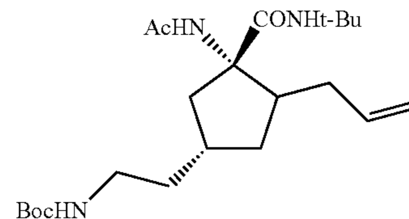
Step 4: tert-butyl 2-((1R,3S)-3-acetamido-4-allyl-3-(tert-butylcarbamoyl) cyclopentyl) ethylcarbamate
