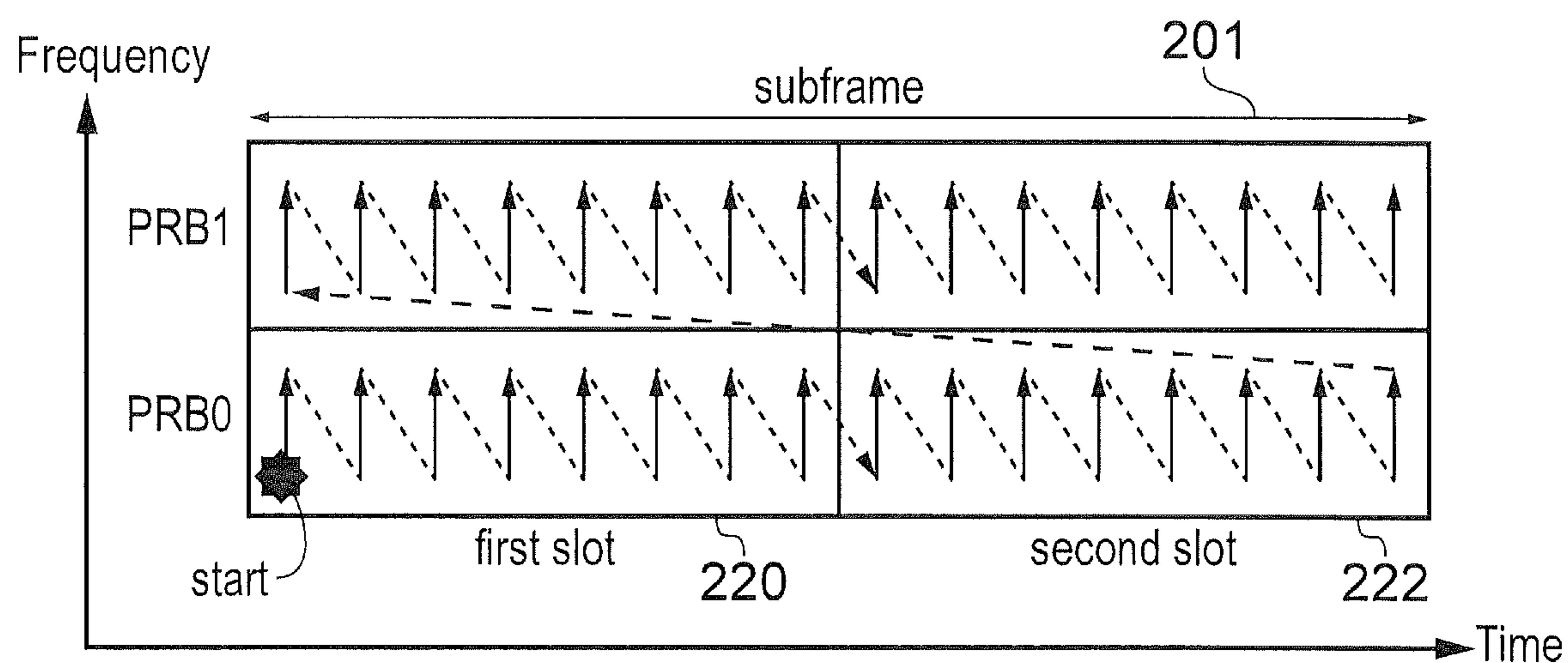
RE mapping order due to I-Interleaver
