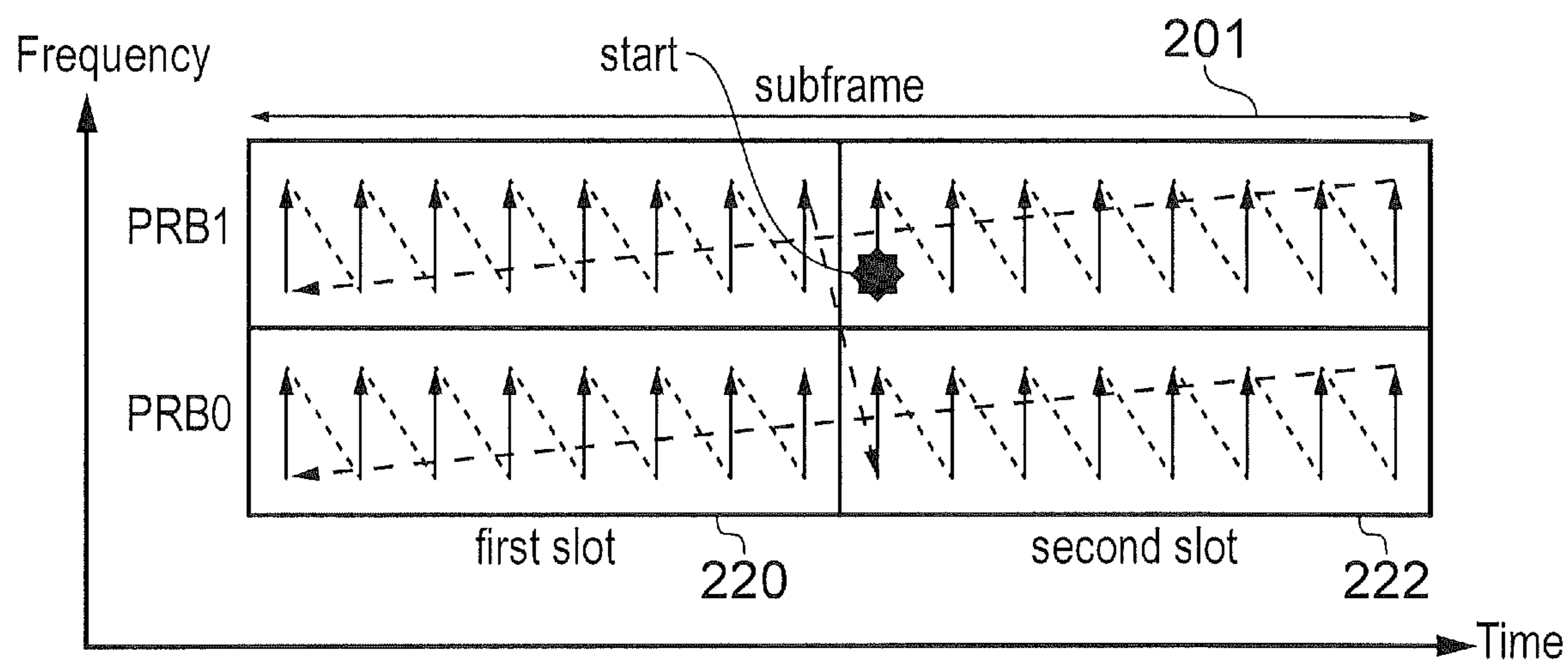
RE mapping order due to Q-Interleaver
