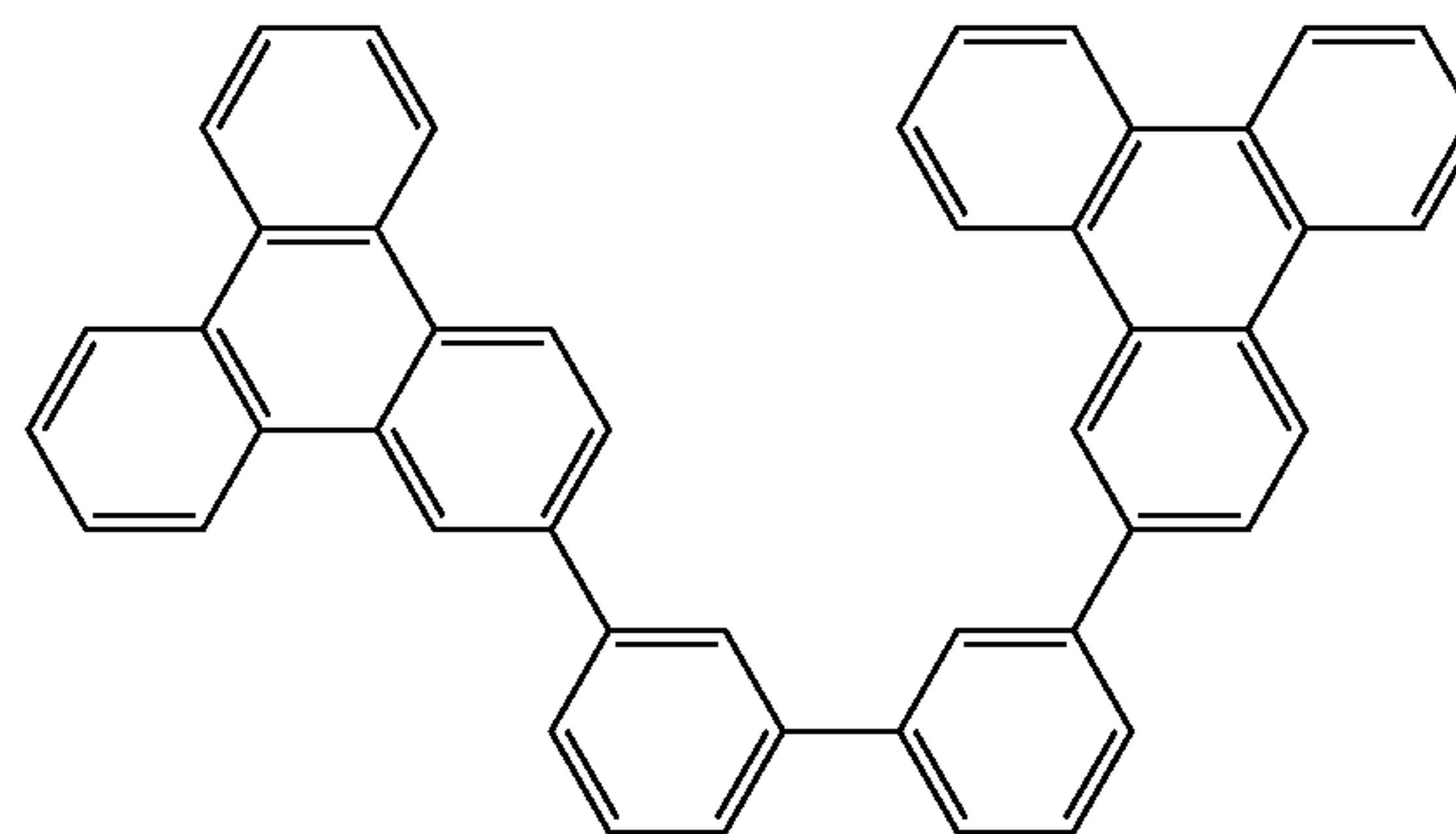
Compound C
