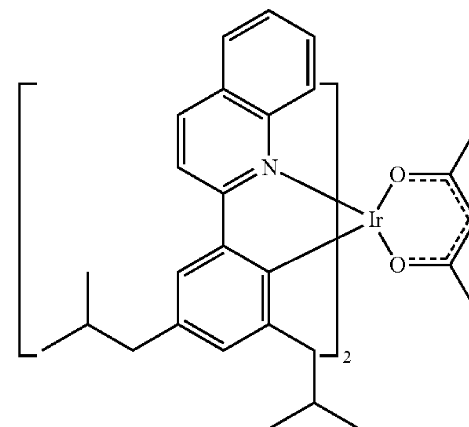
Compound 23
