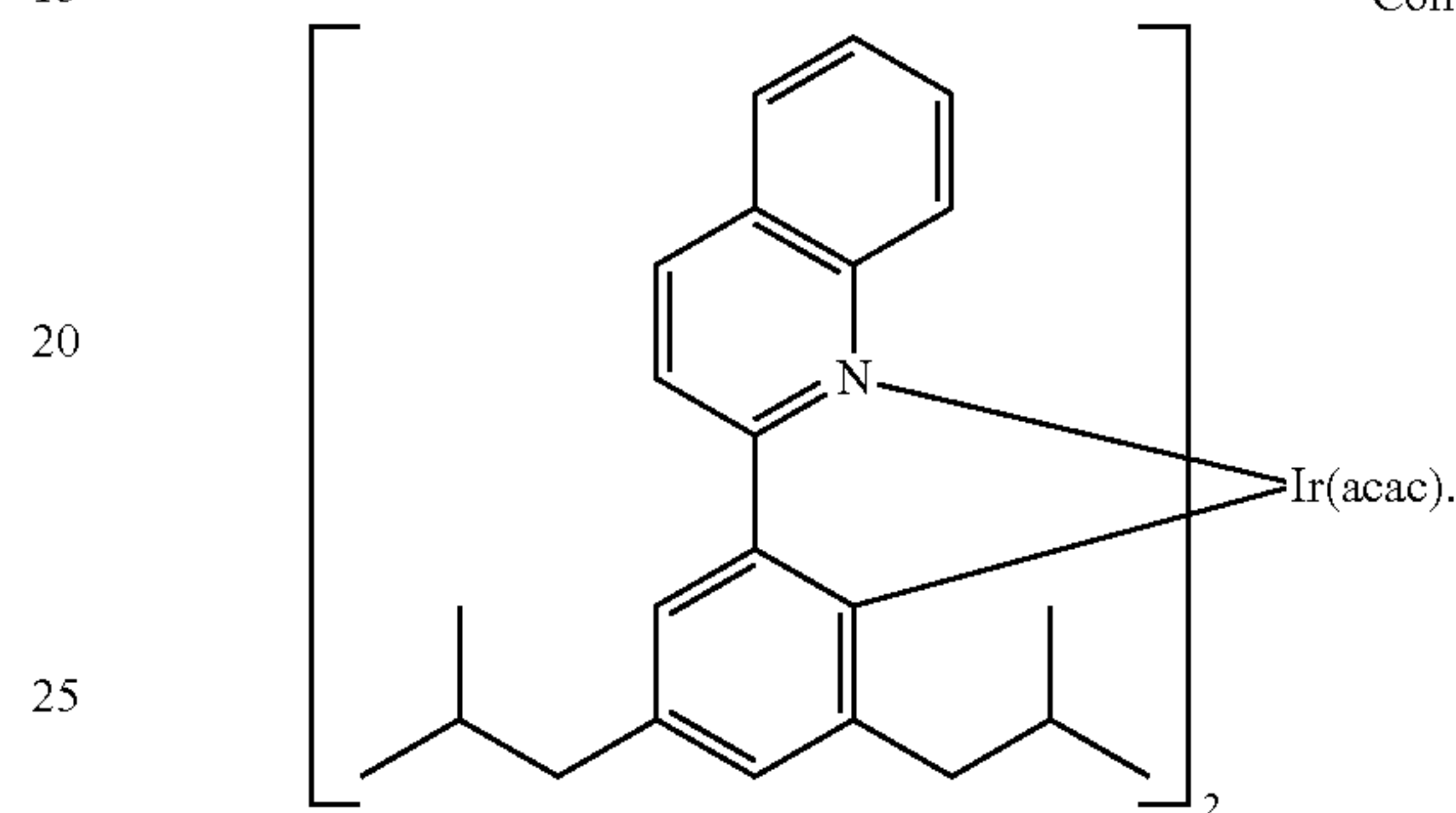
Compound 23
