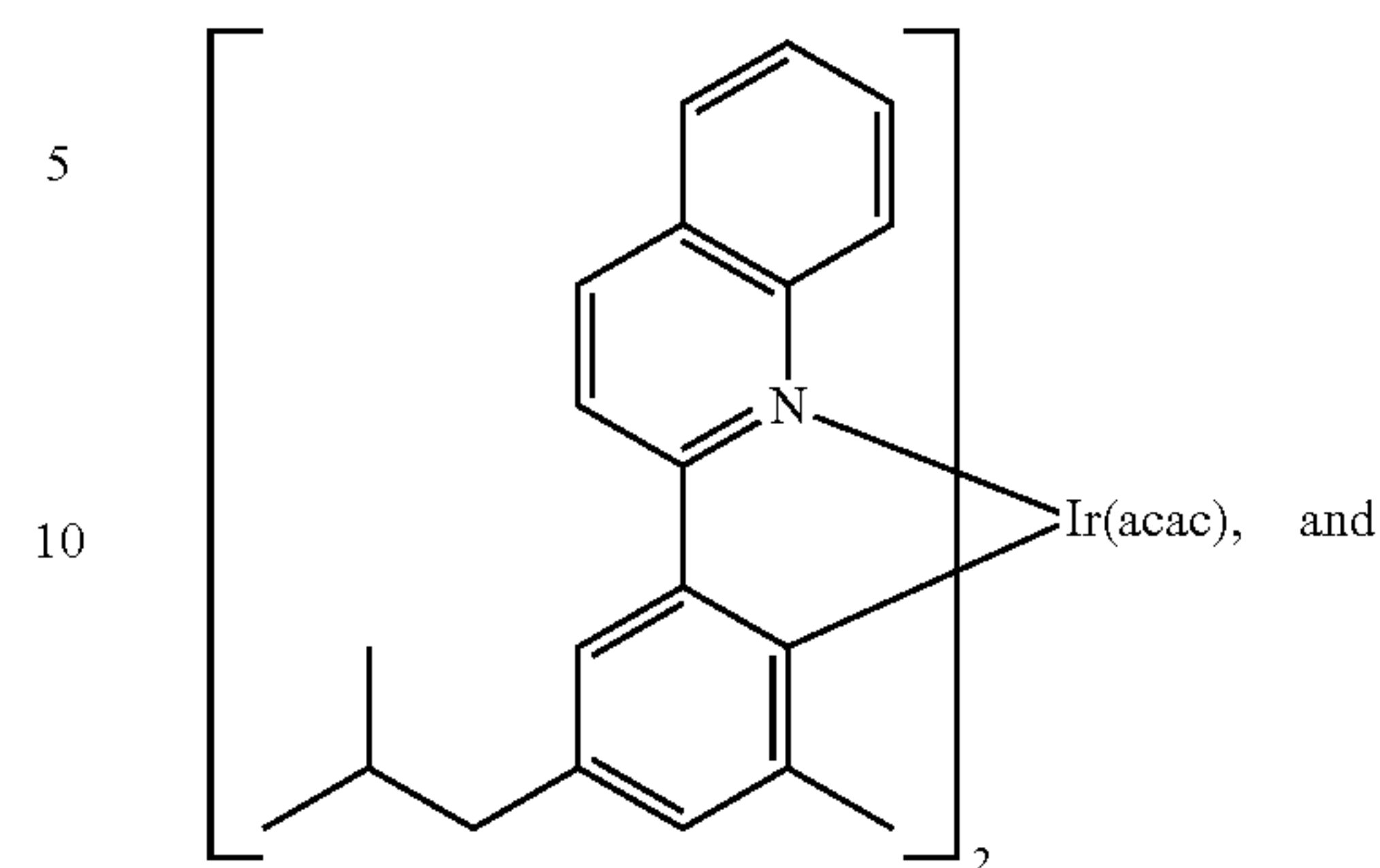
Compound 23
