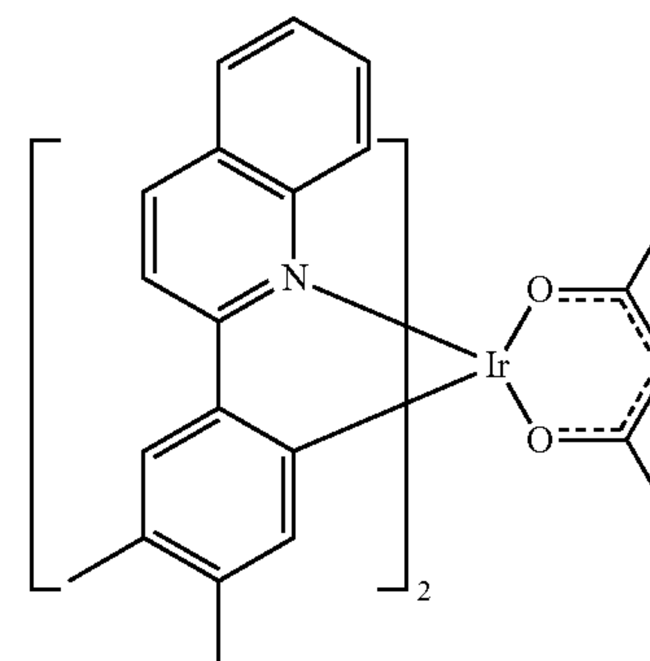
Compound 13
