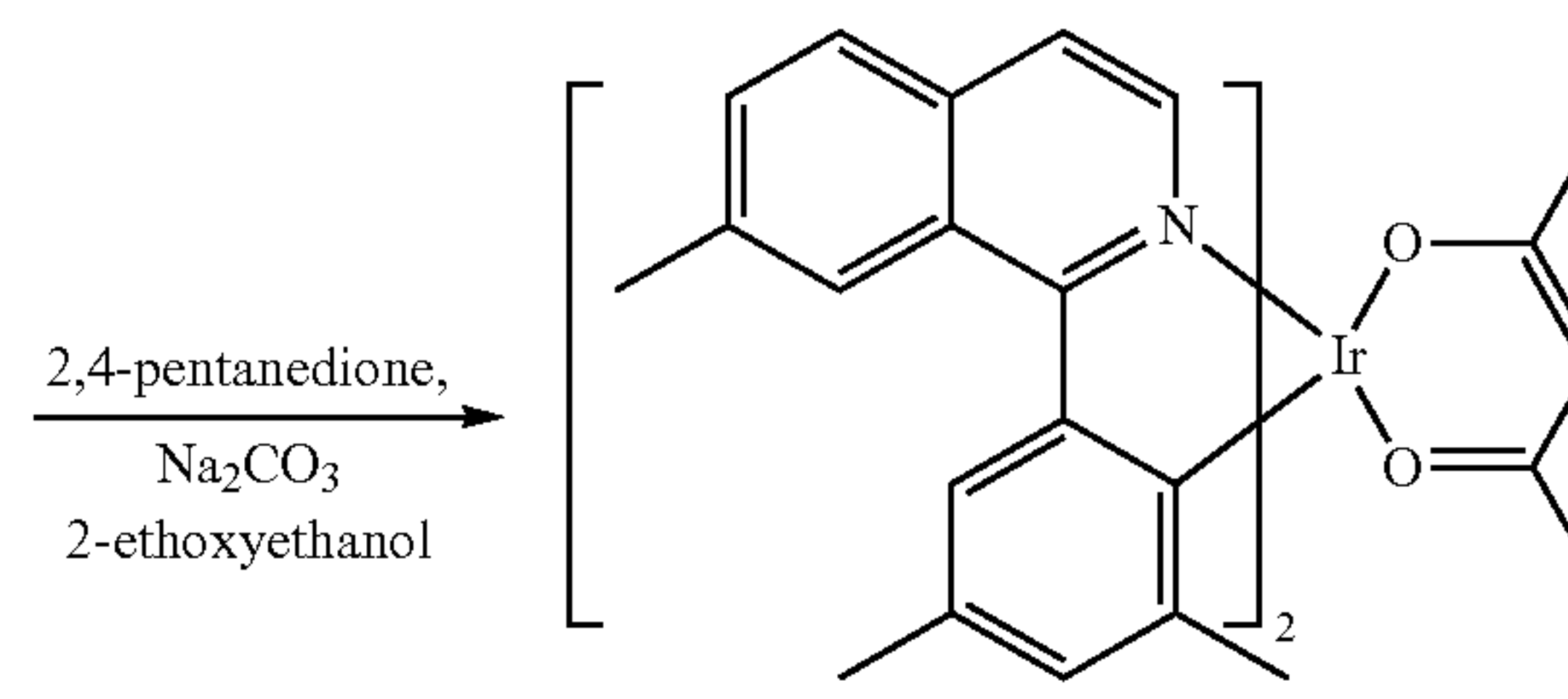
Compound 24
