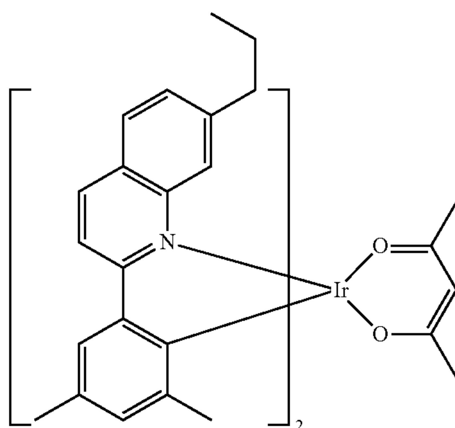
Compound 16
