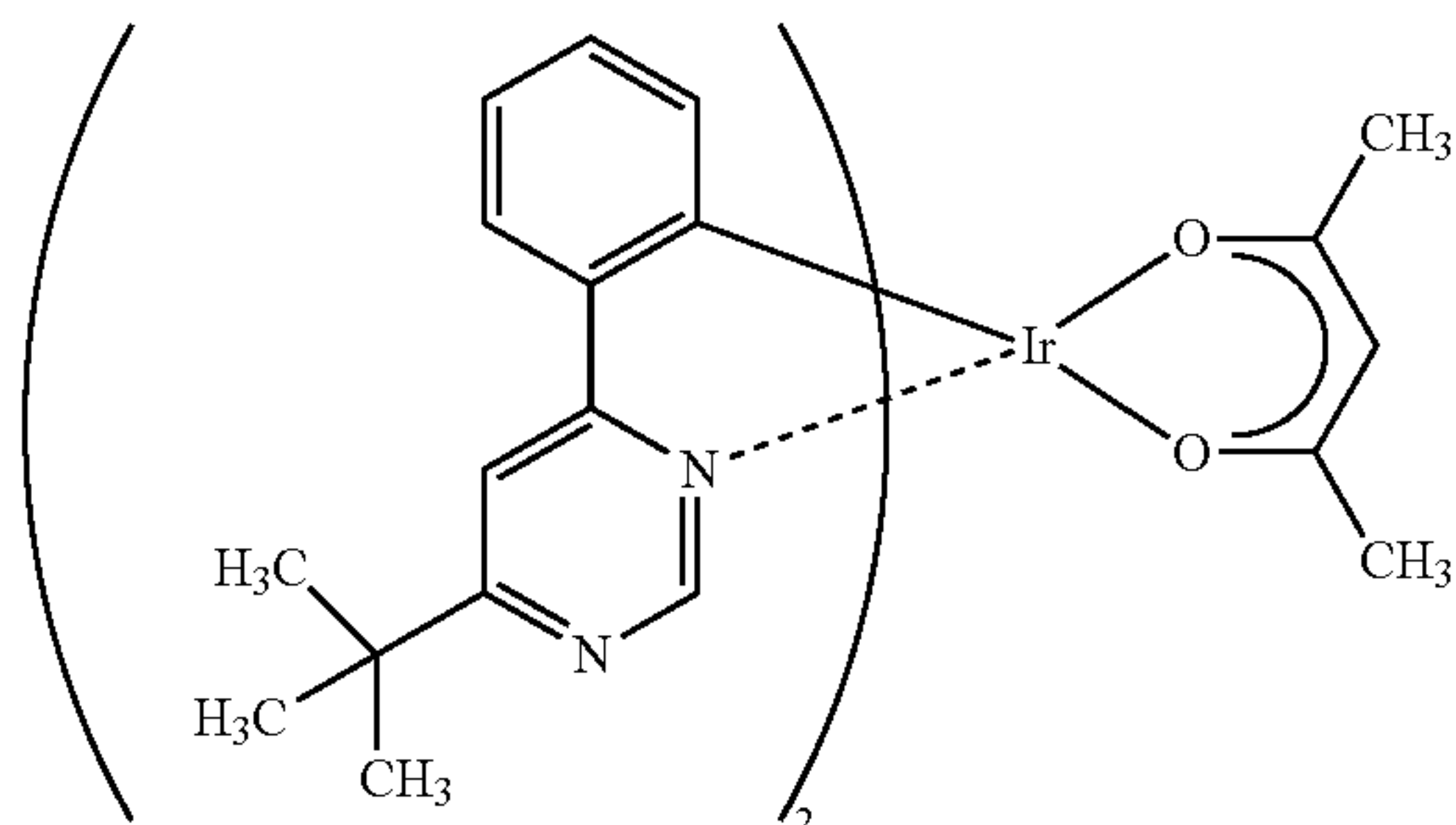
[\text{Ir}(\text{tBuppm})_2(\text{acac})]
