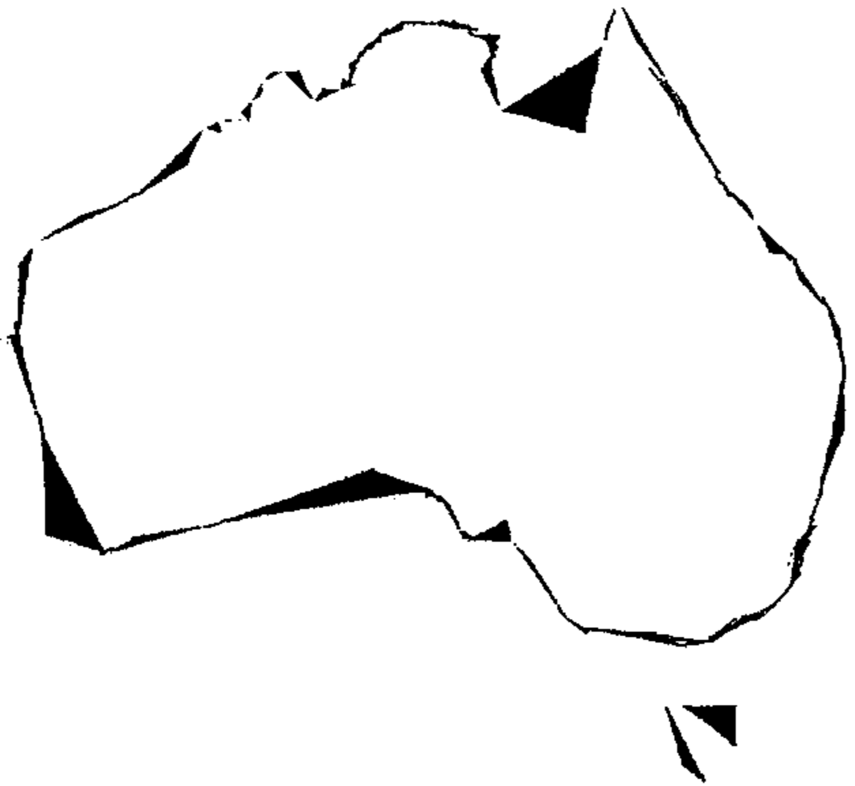
Figure 9c Step size = 16
