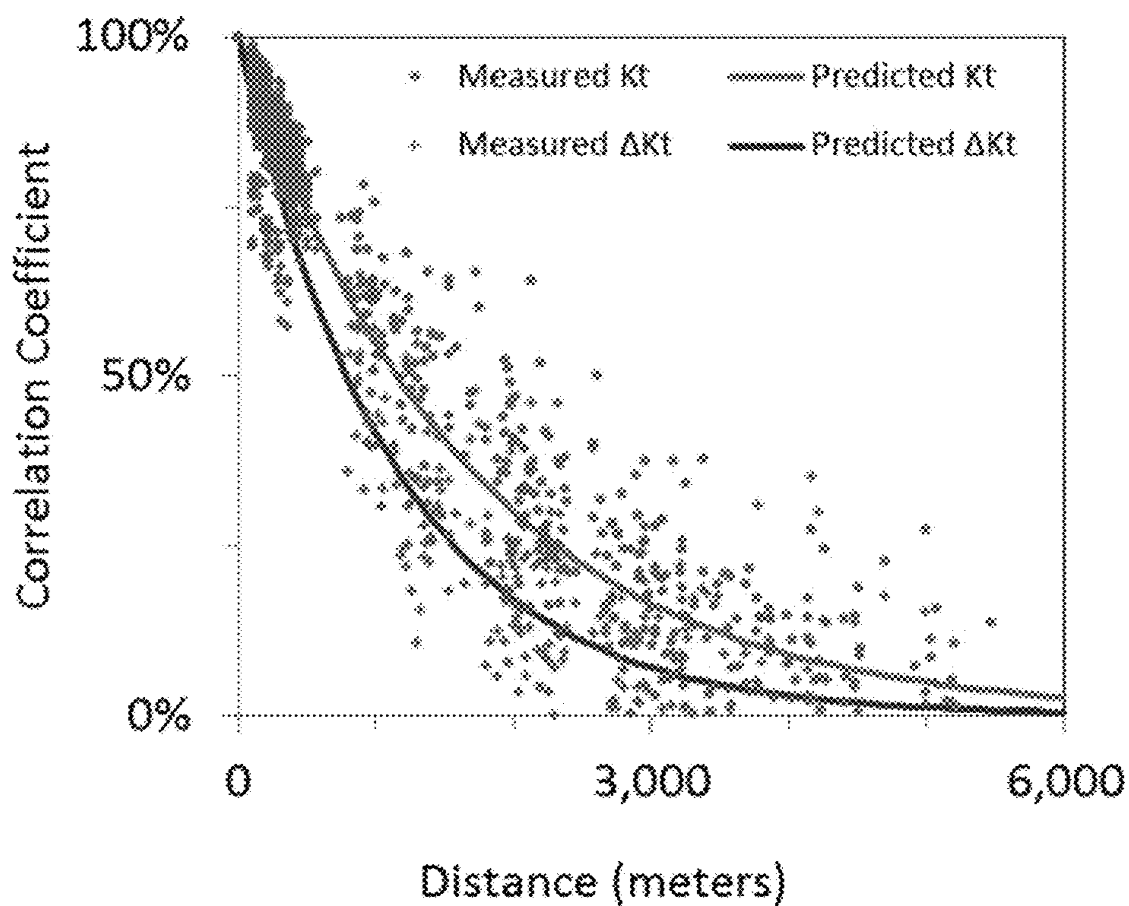
Fig. 10F Correlation vs. Distance ( \Delta t=300 )
