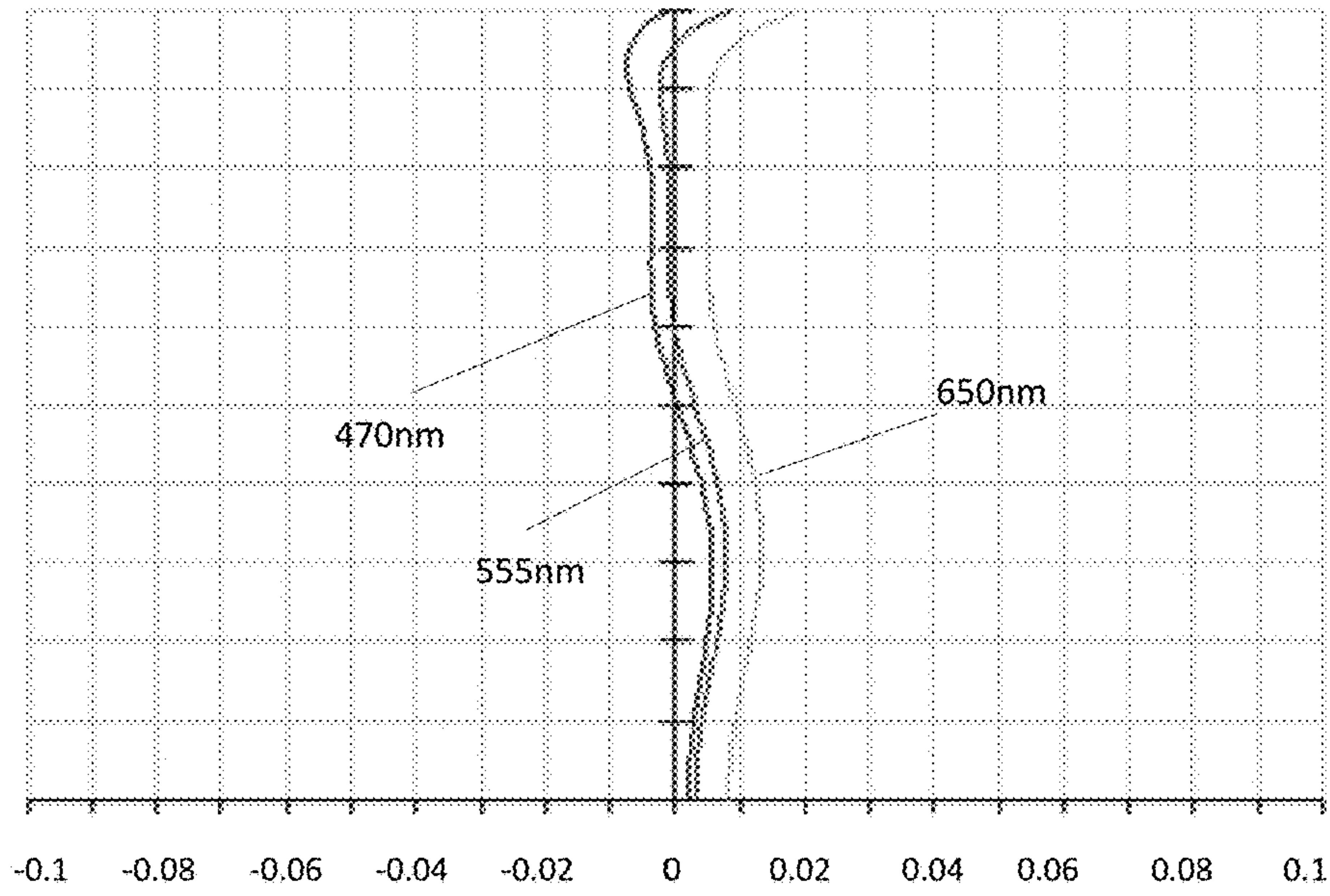
Longitudinal aberration
