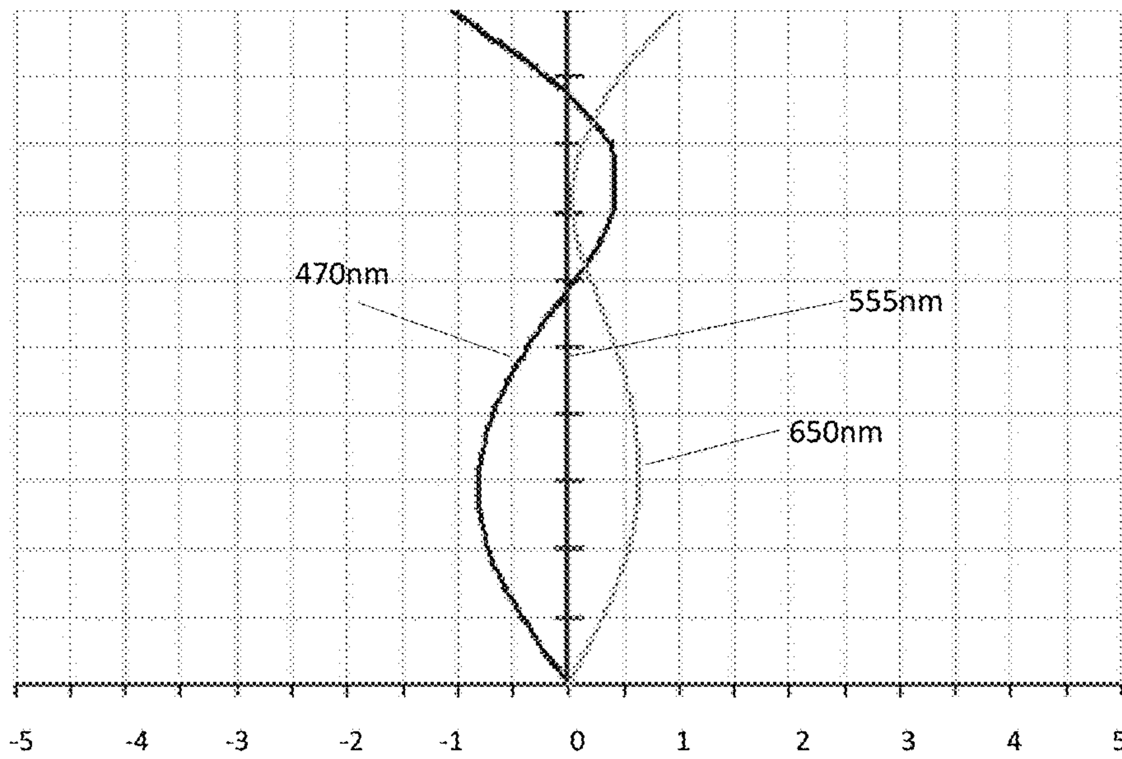
Lateral color
