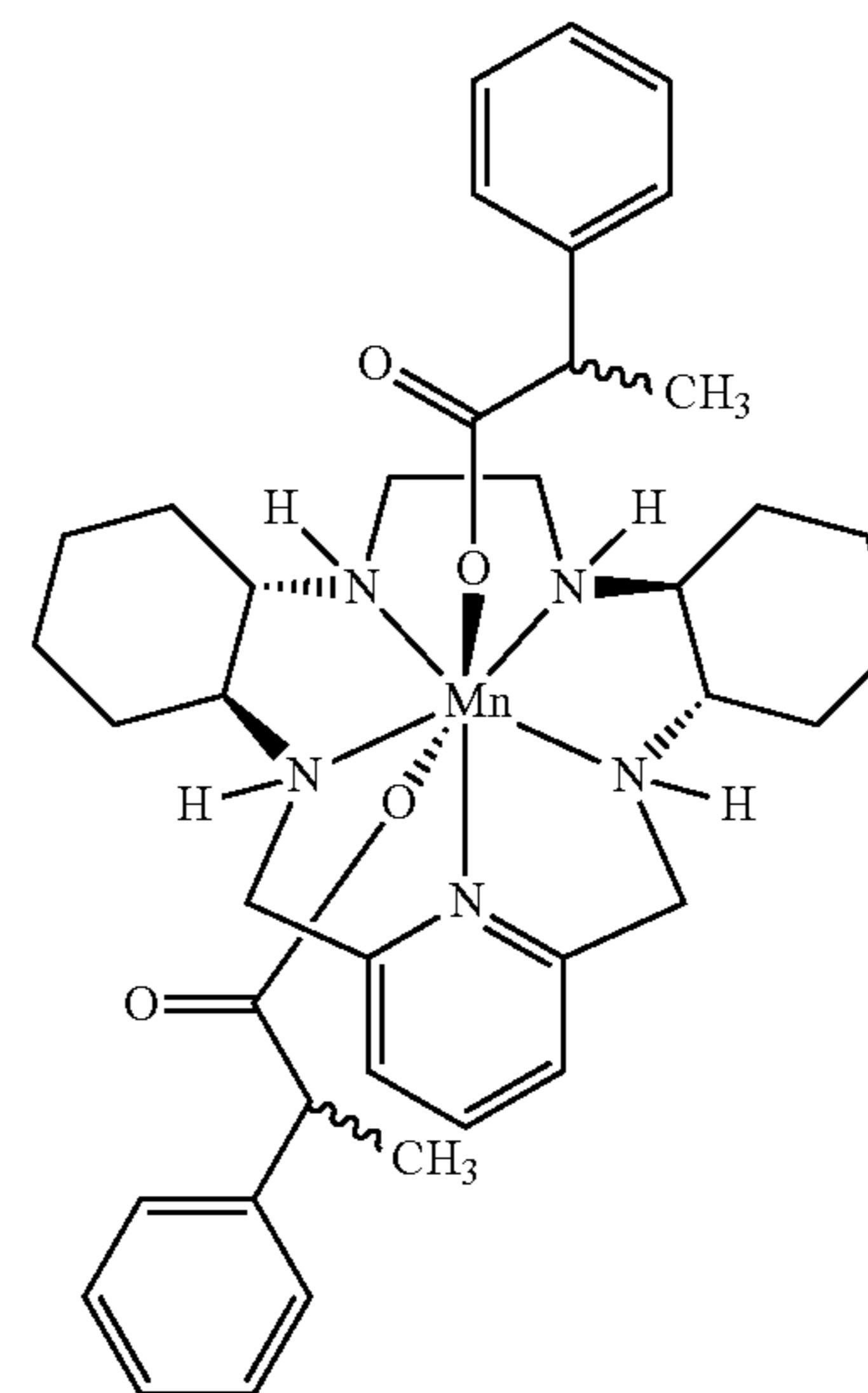
[Bis-(rac)-Phenylpropionato(GC4419)] C 39 H 53 MnN 7 O 4 MW 710.82
