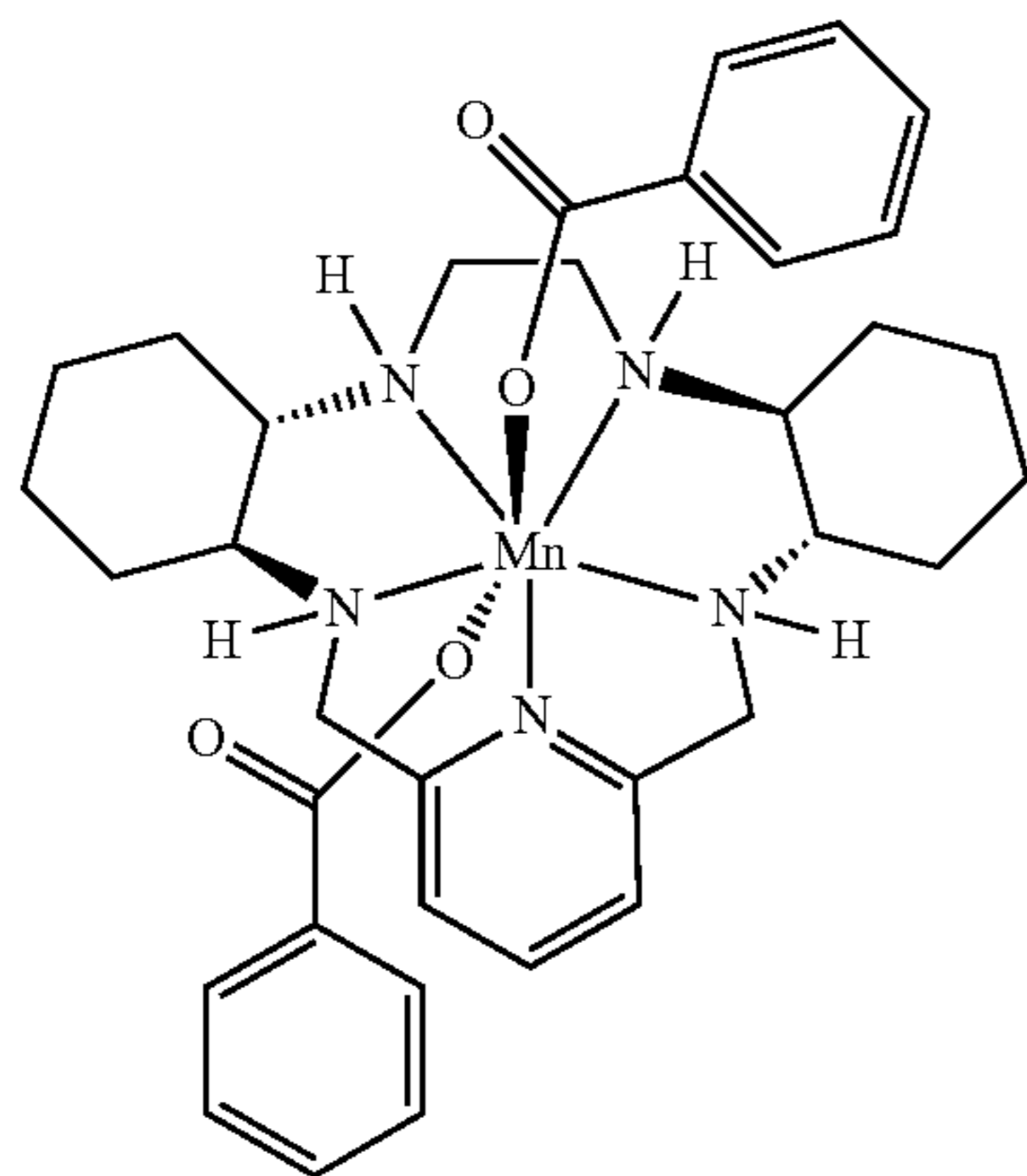
[Bis-Benzoato(GC4419)] C 35 H 45 MnN 5 O 4 MW 654.71
