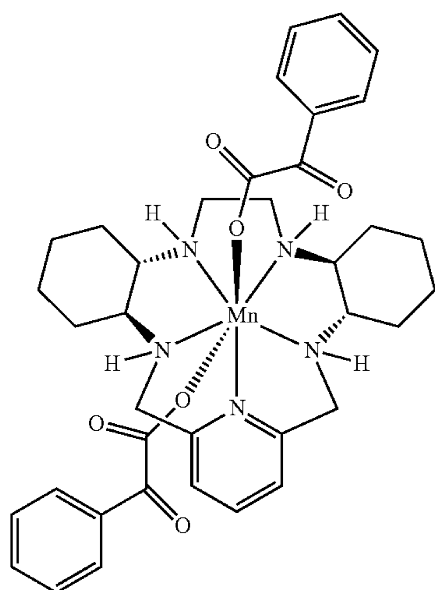
[Bis-Phenylglyoxylato(GC4419)] C_{37}H_{45}MnN_5O_6 MW 710.73
