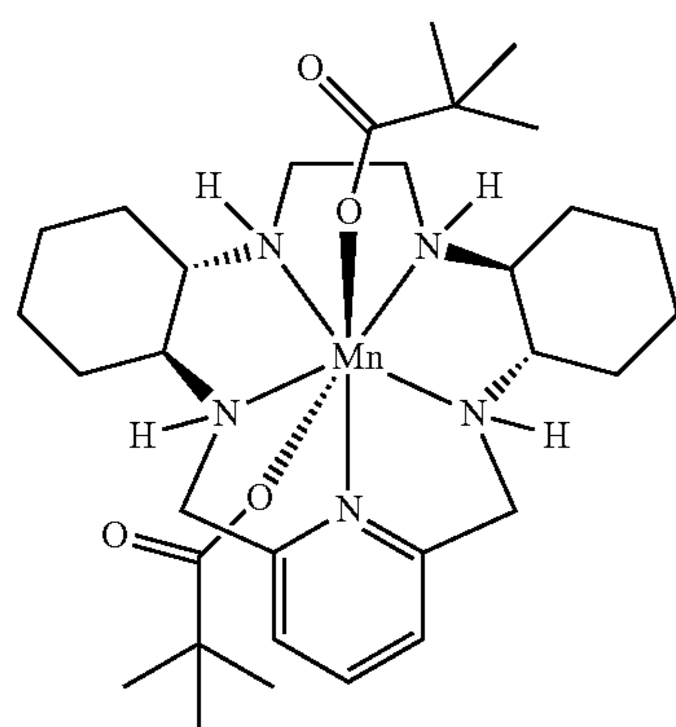
[Bis-Pivaloato(GC4419)] C_{31}H_{53}MnN_5O_4 MW 614.73
