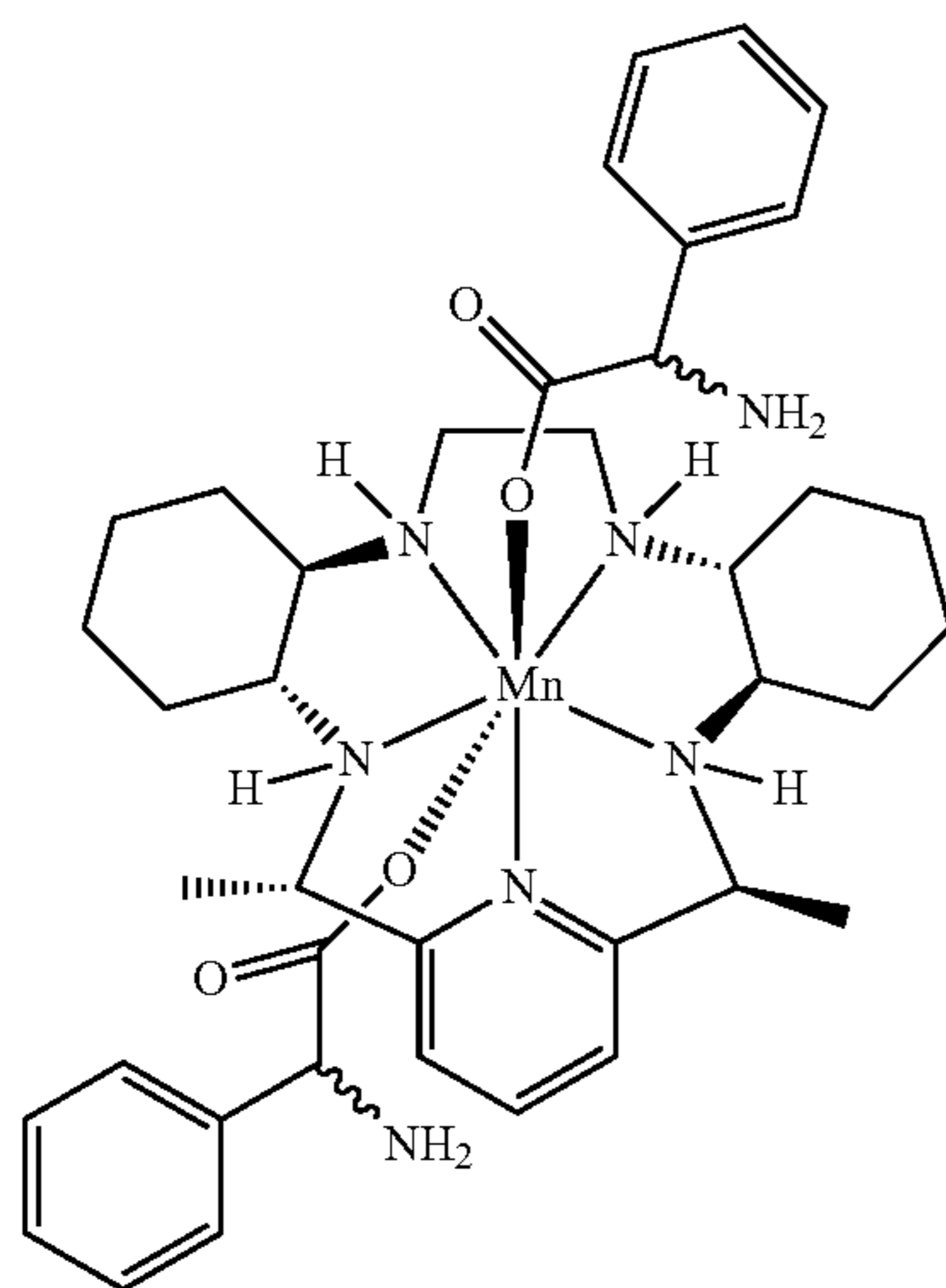
[Bis-(rac)-Phenylglycinato(GC4401)] C_{39}H_{53}MnN_7O_4 MW 740.85
