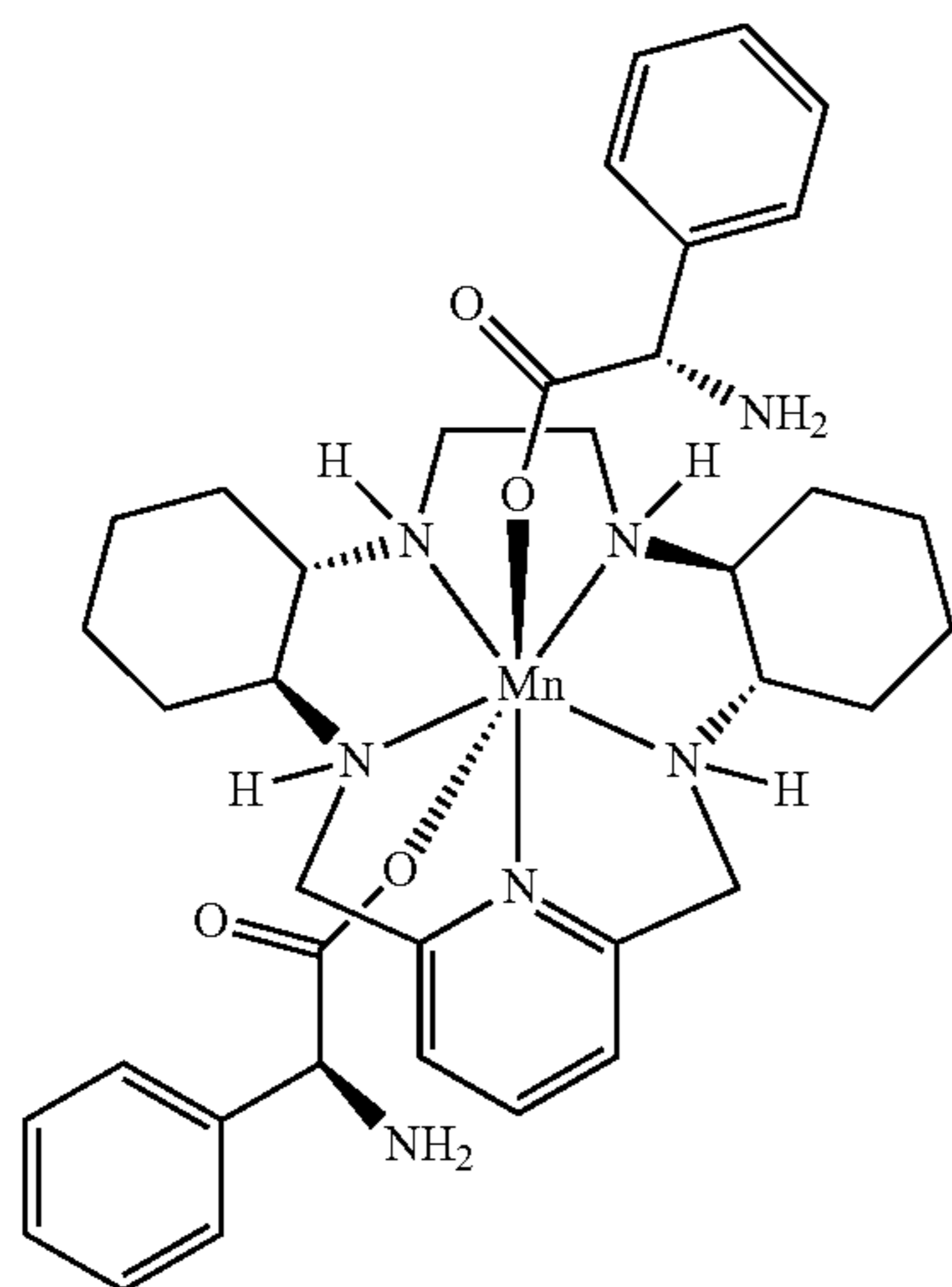
[Bis-(L)-Phenylglycinato(GC4419)] C 37 H 51 MnN 7 O 4 MW 712.80
