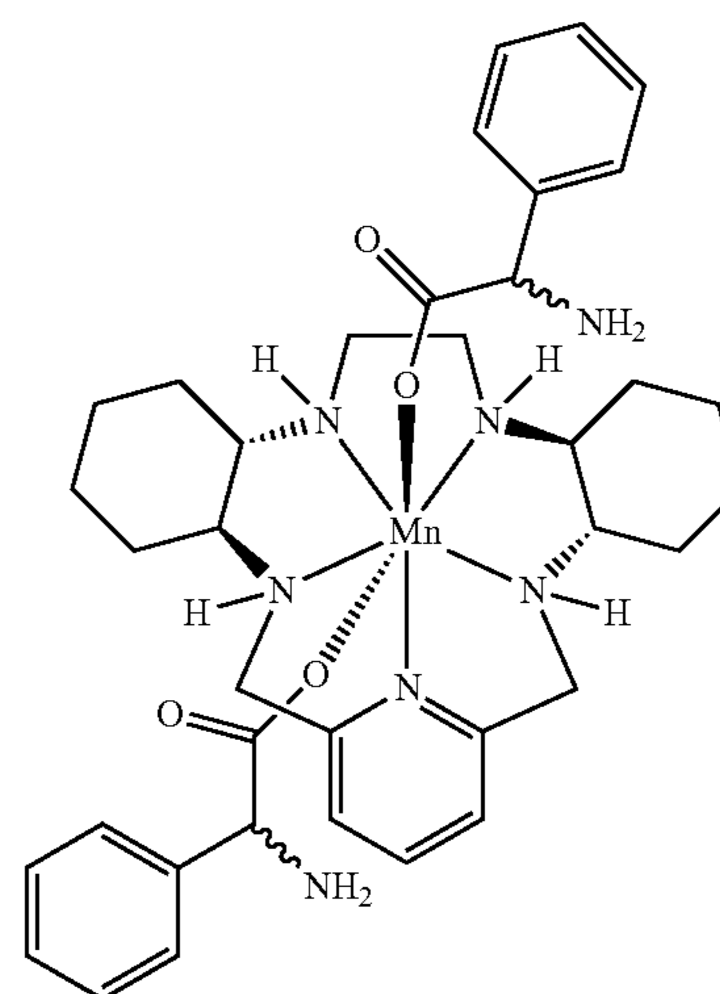
[Bis-(rac)-Phenylglycinato(GC4419)] C 37 H 51 MnN 7 O 4 MW 712.80
