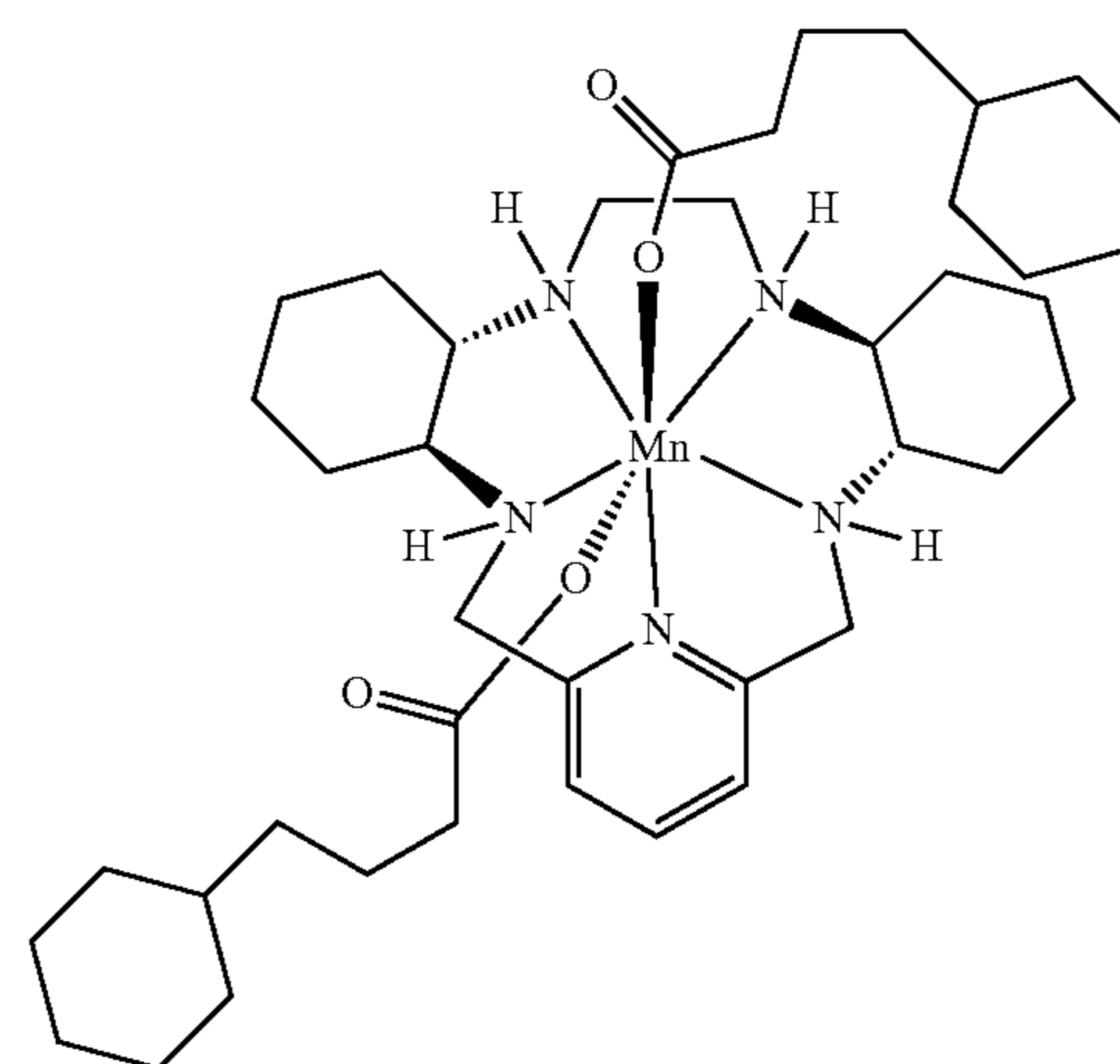
[Bis-Cyclohexanebutyrato(GC4419)] C_{41}H_{69}MnN_5O_4 MW 750.97
