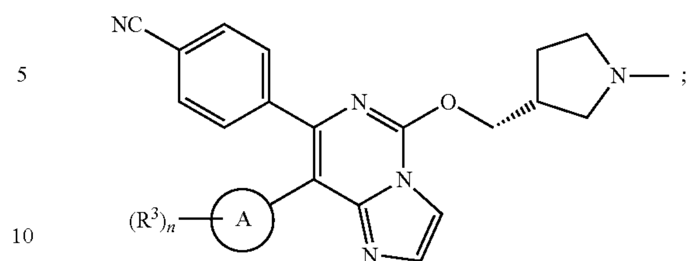
Formula (XVIIIf)
