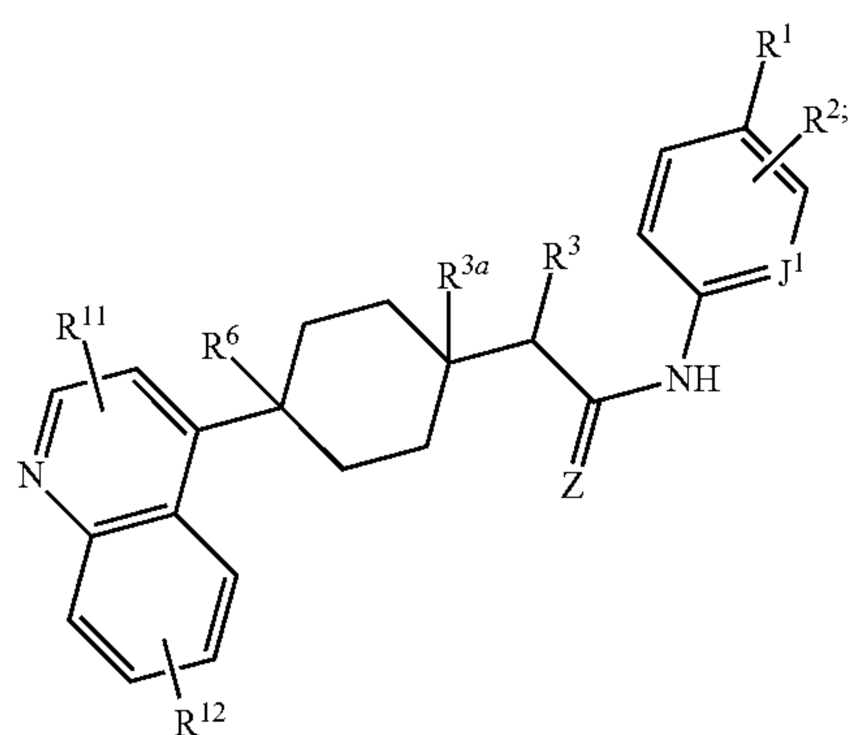
Formula (XLIIIIm)
