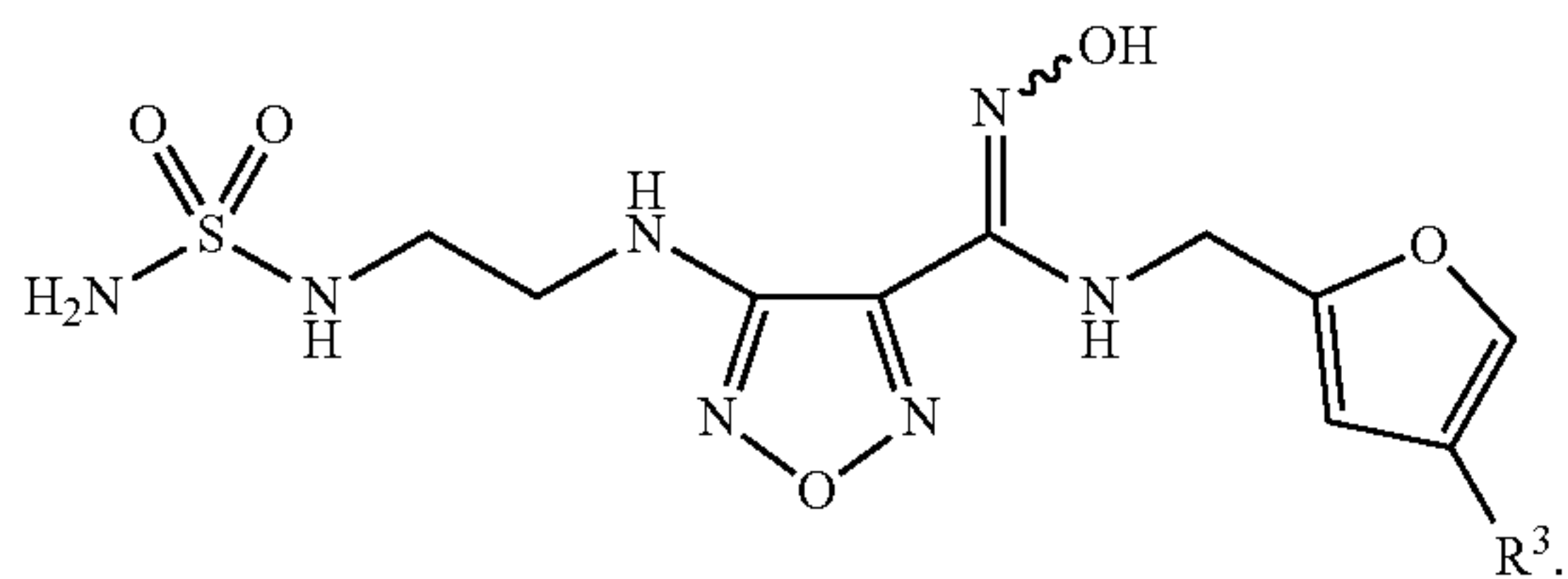
Formula (LIII)
