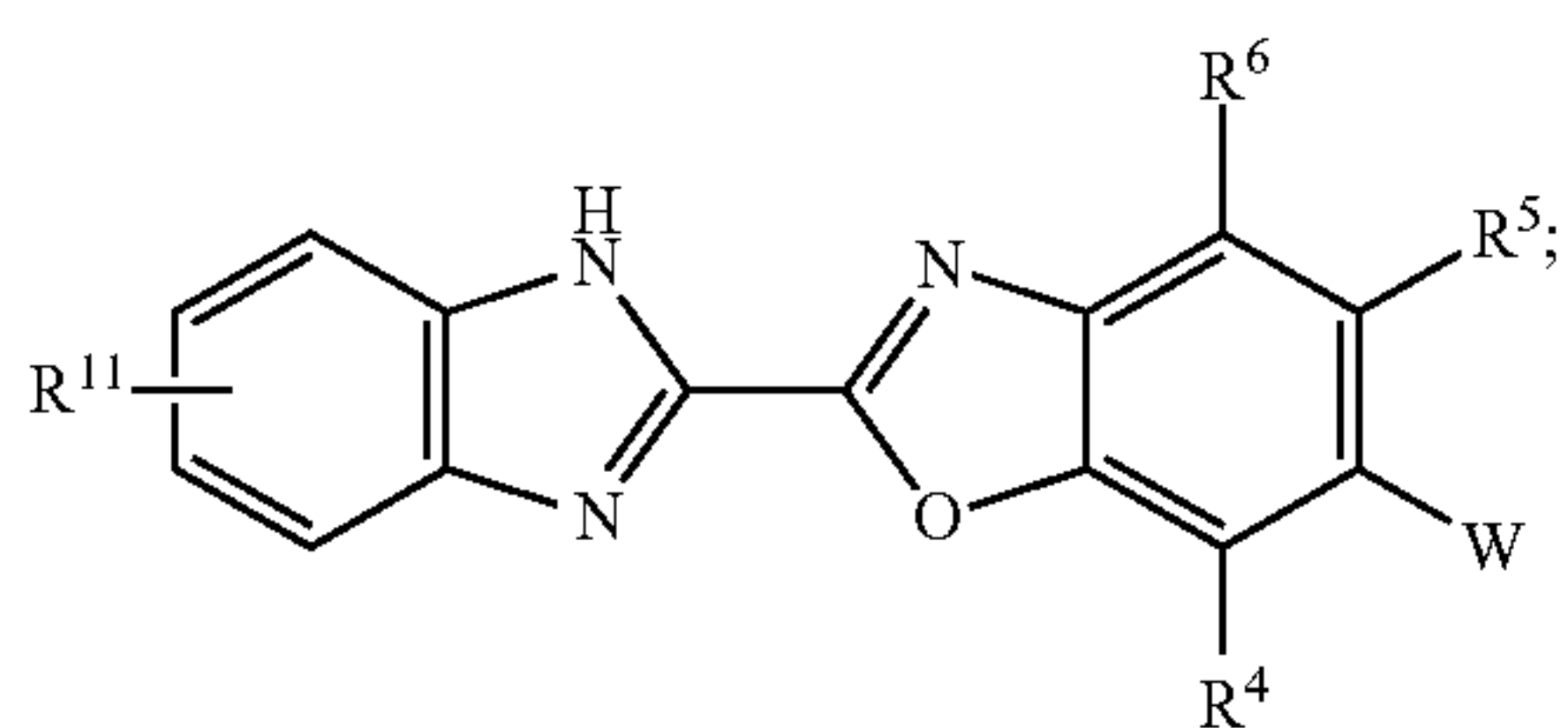
Formula (XIXg)
