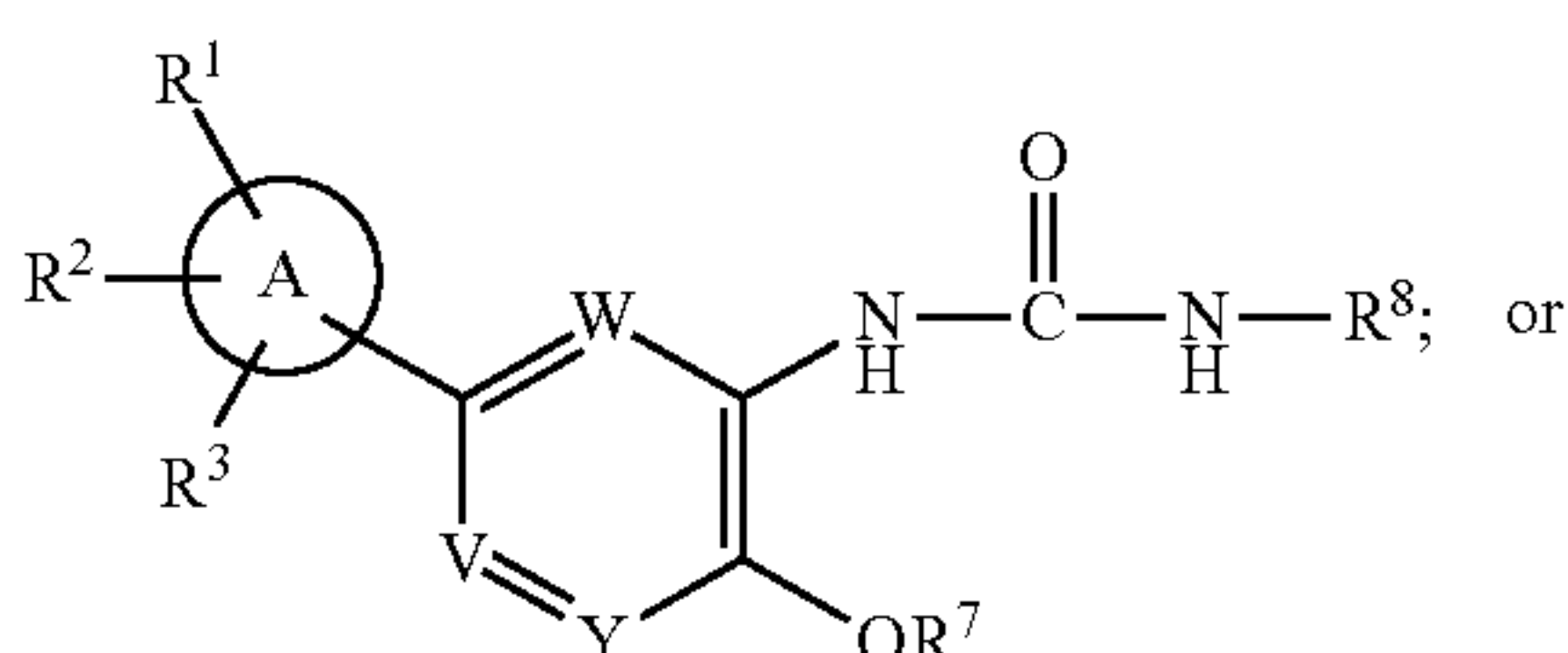
Formula (XXXVI)
