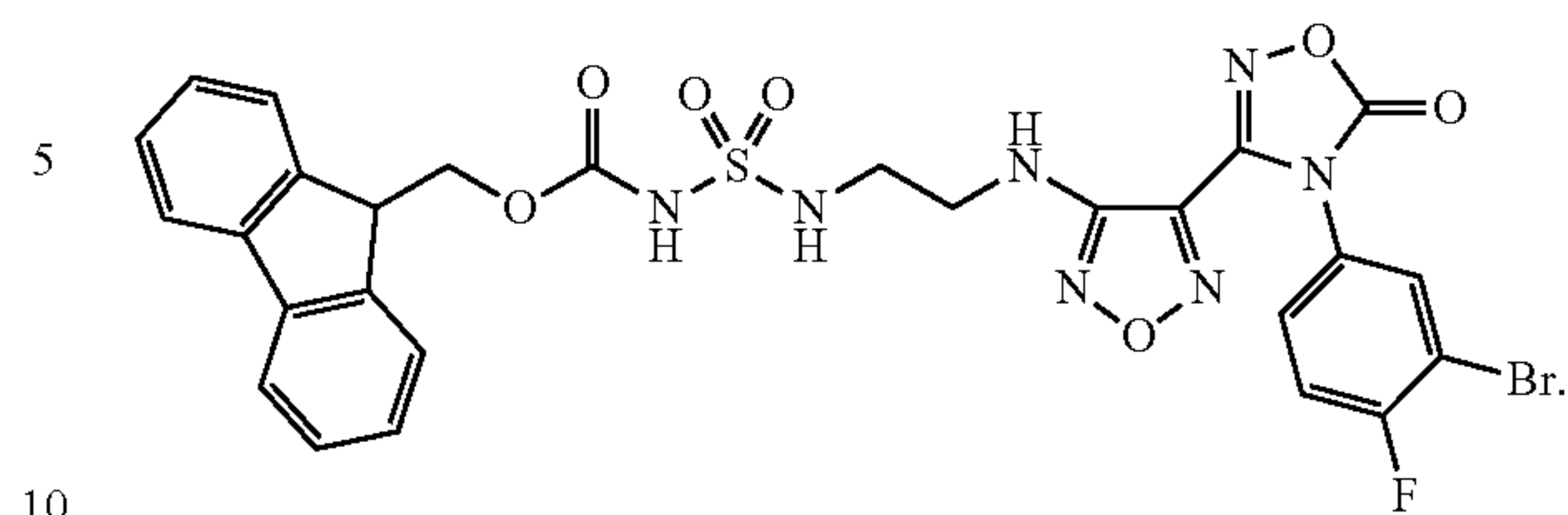
Formula F20
