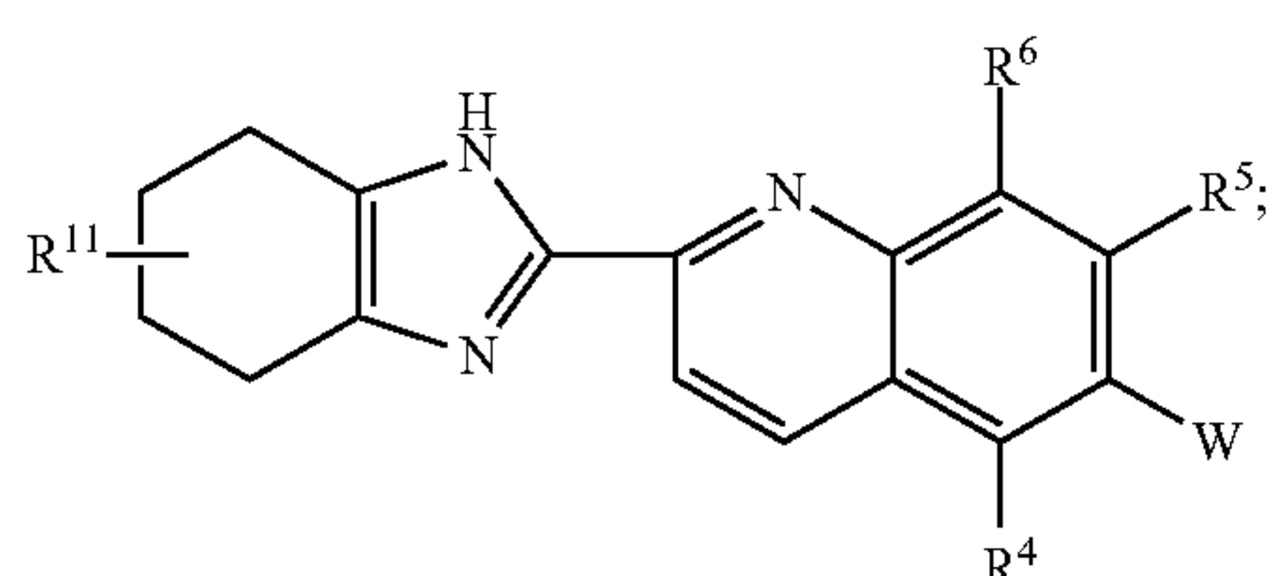
Formula (XIXq)
