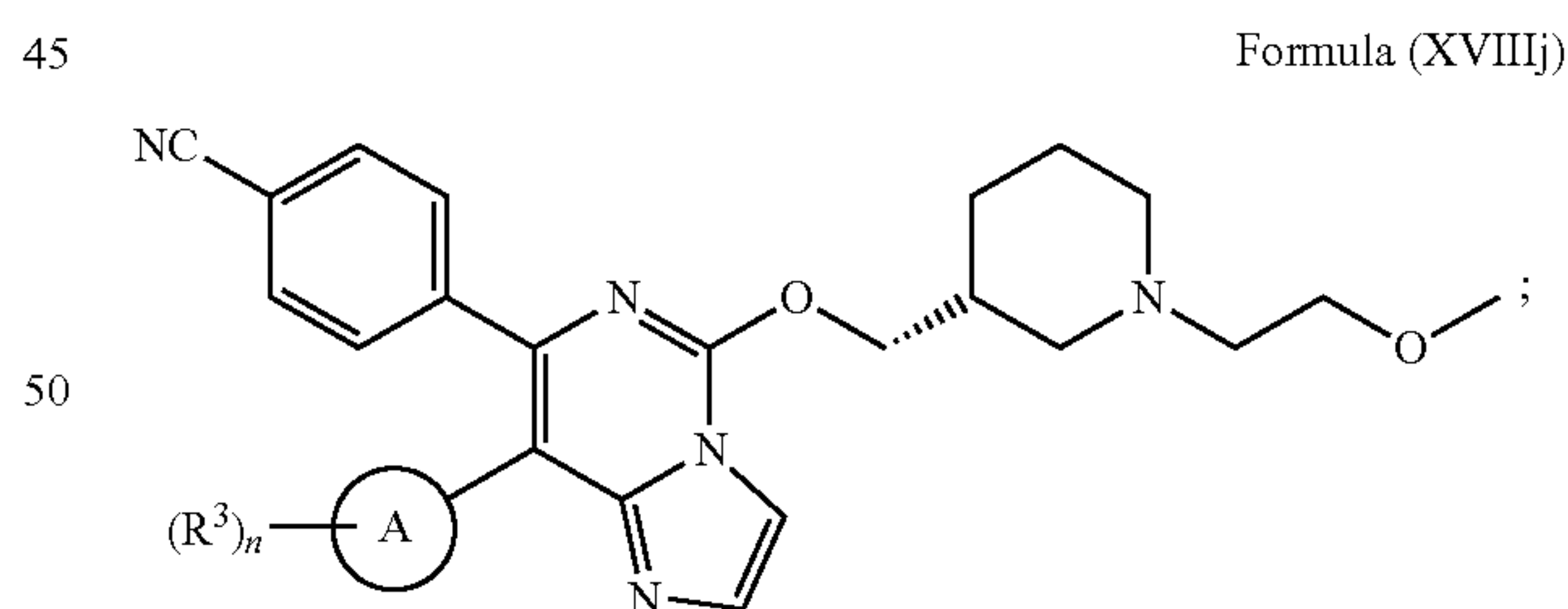
Formula ( )
