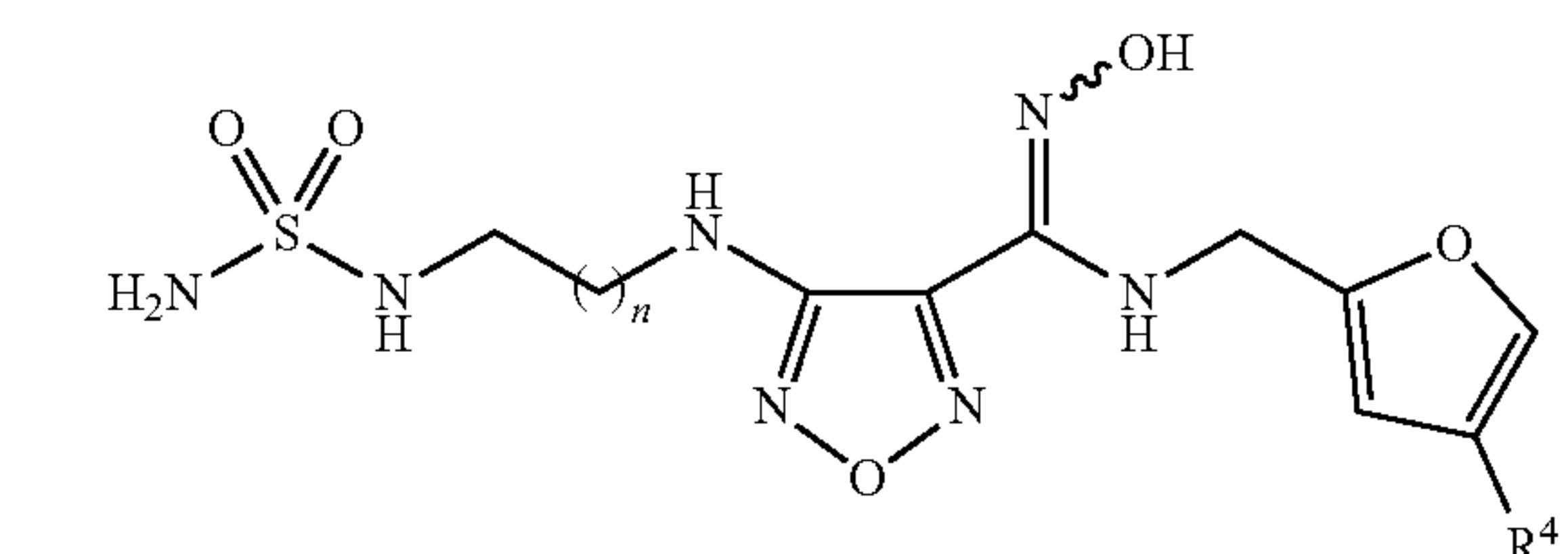
Formula F28
