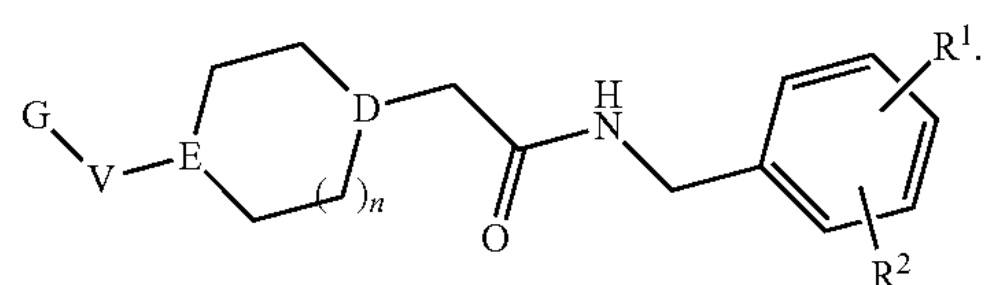
Formula (XLIVn)
