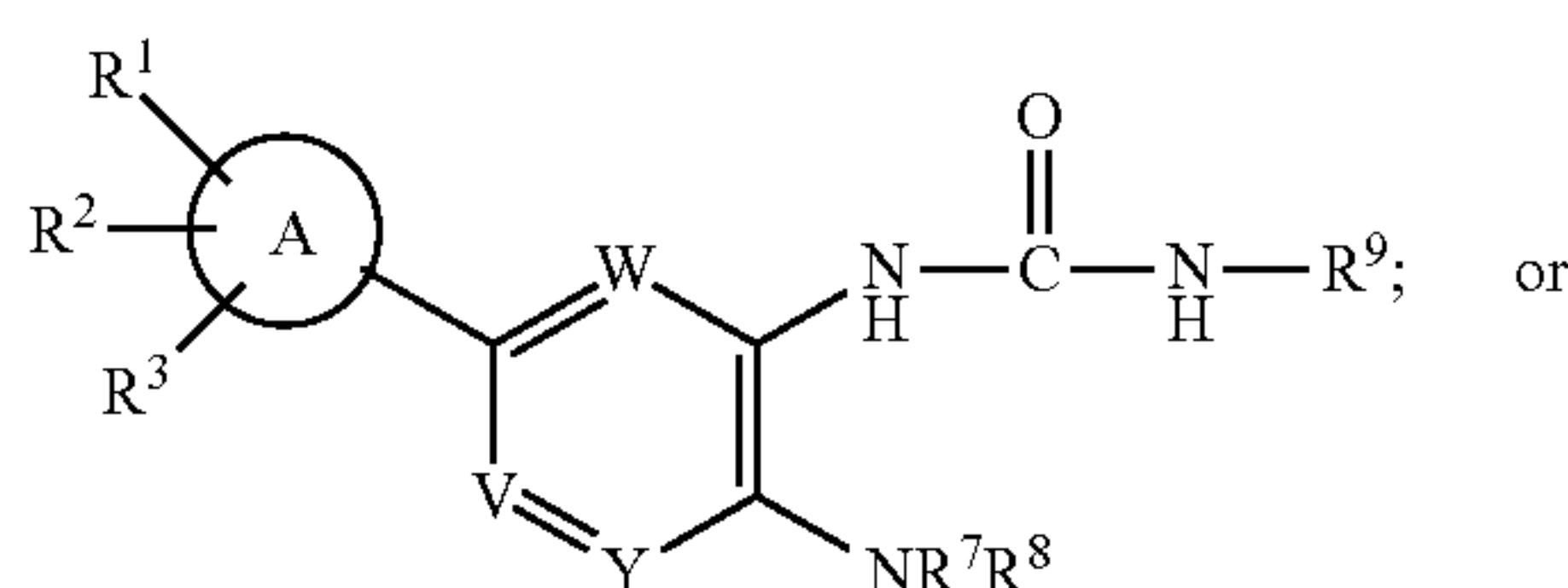
Formula (XL)
