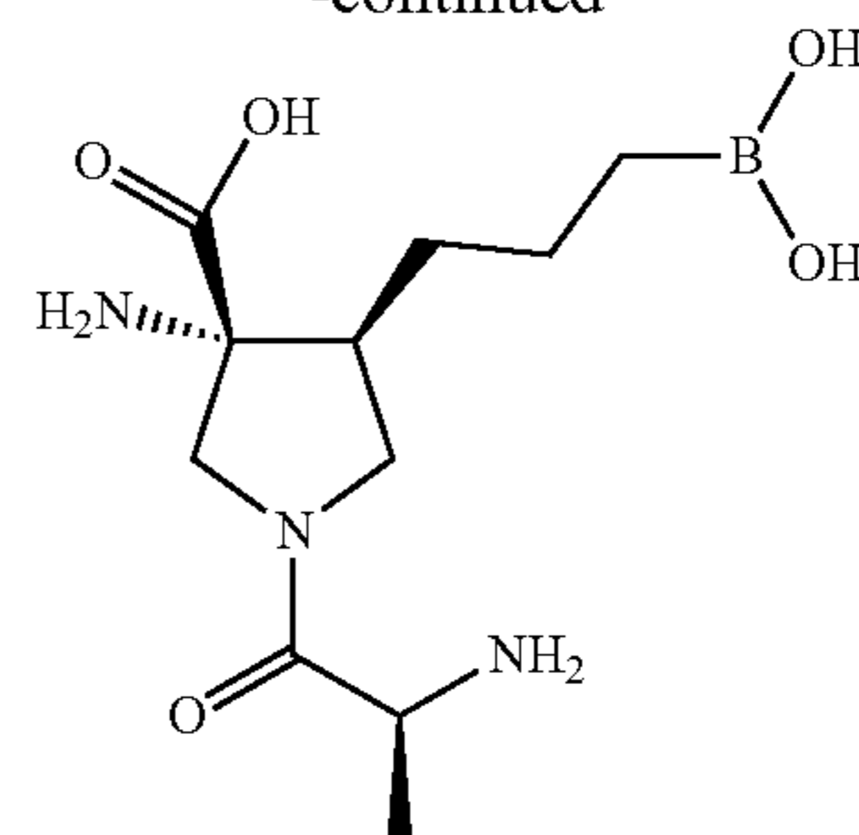
Alanine AUC = 13727 \text{IC}_{50} = 93 nM
