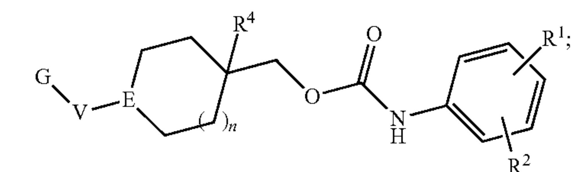
Formula (XLIVg)
