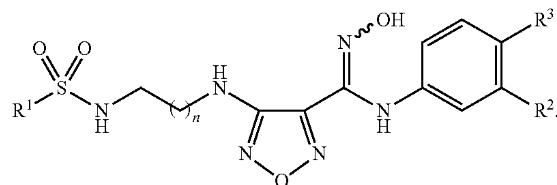
Formula (III)
