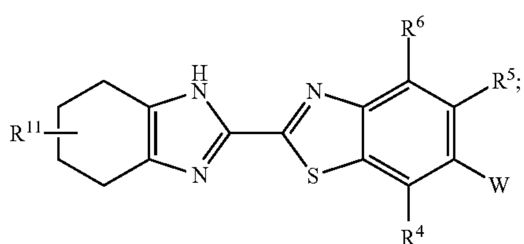
Formula (XIXm)
