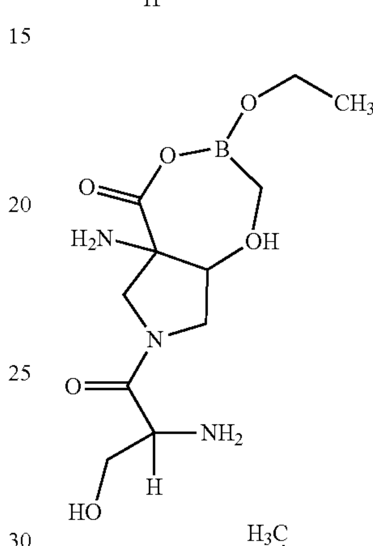
Formula (LVc)
