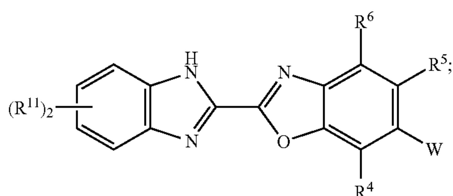
Formula (XIXi)
