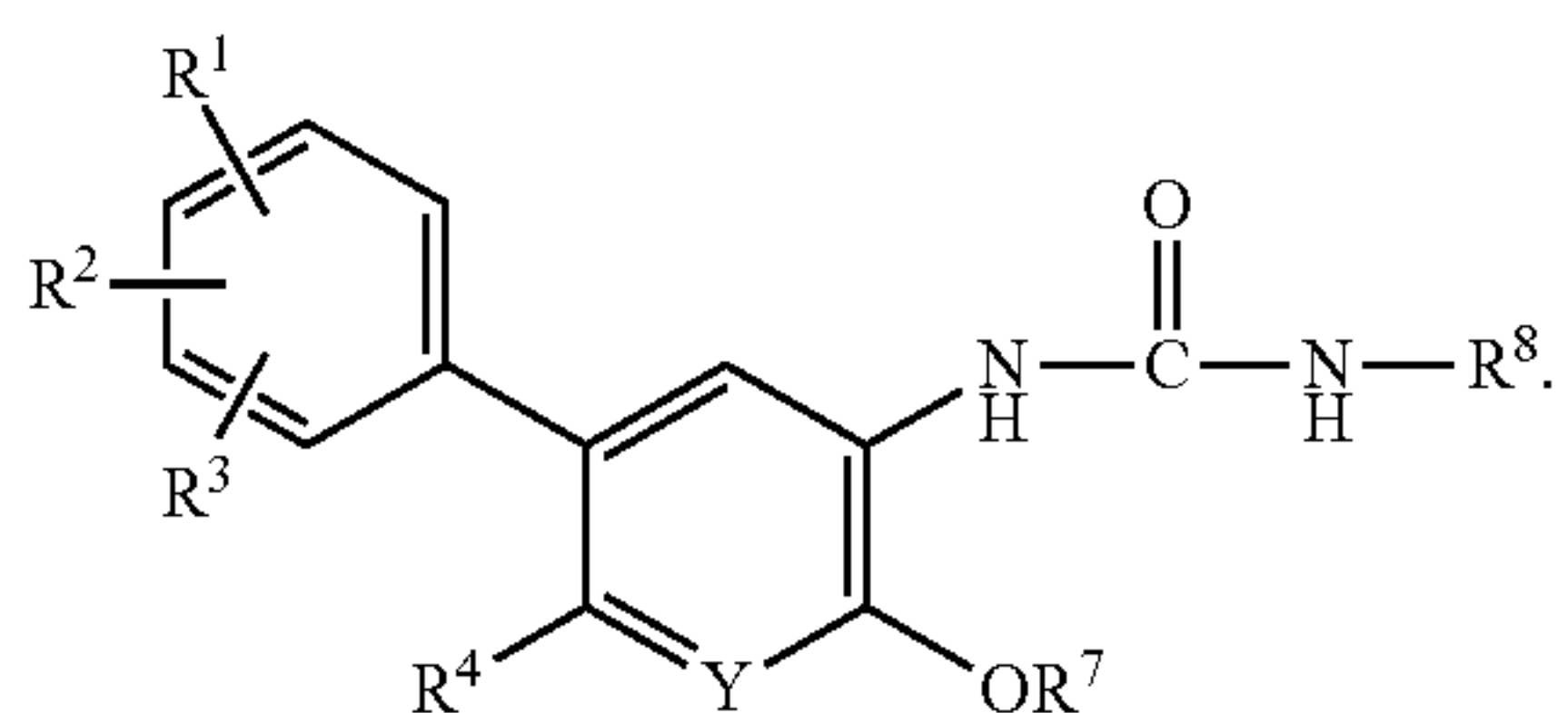
Formula (XXXVI)
