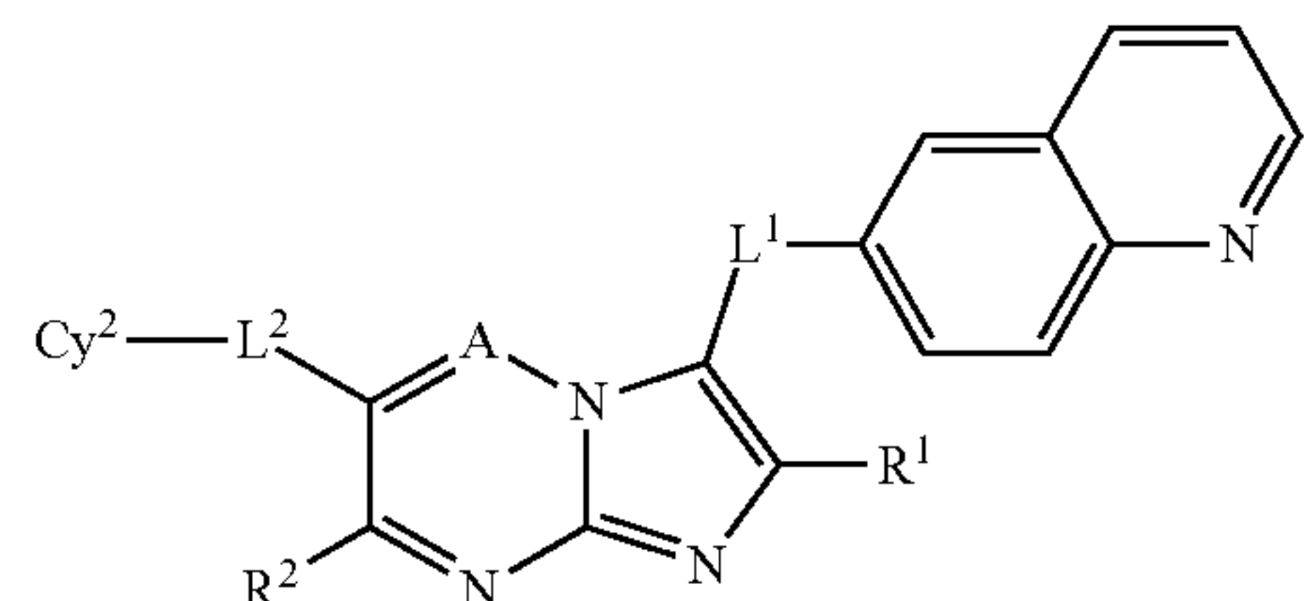
Formula (IIg)
