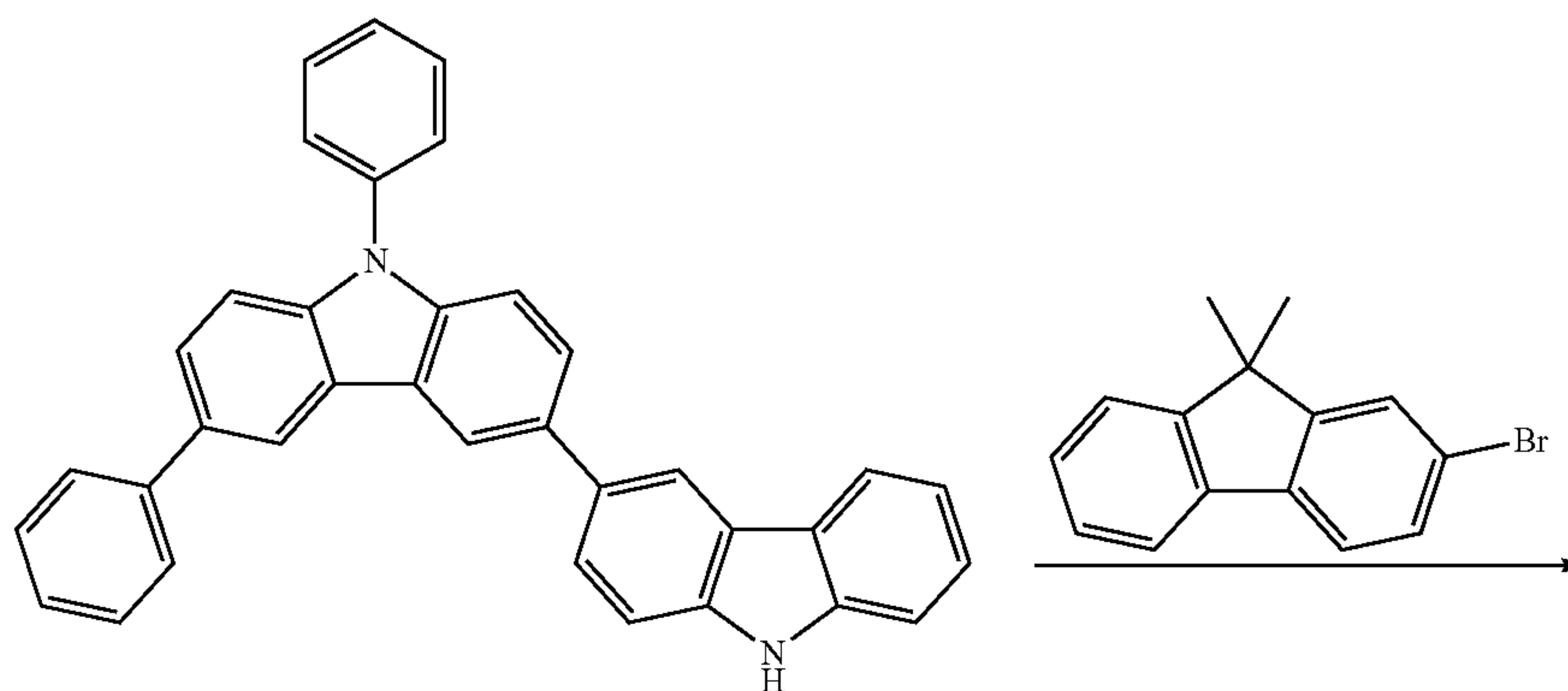
Intermediate C
