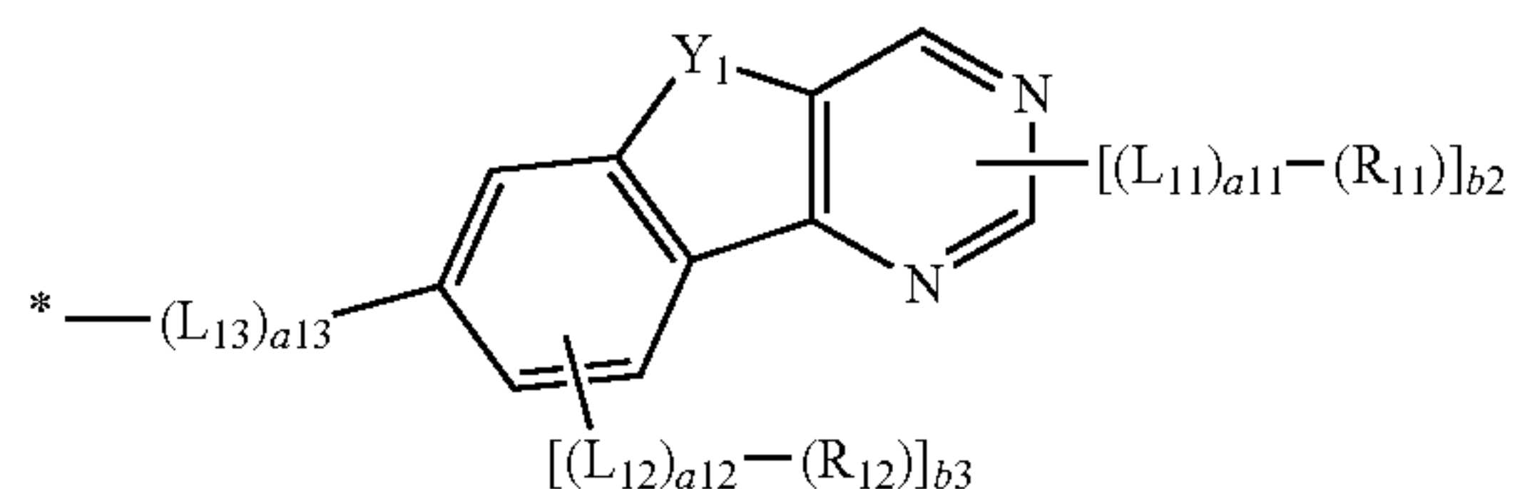
Formula (3)-5
