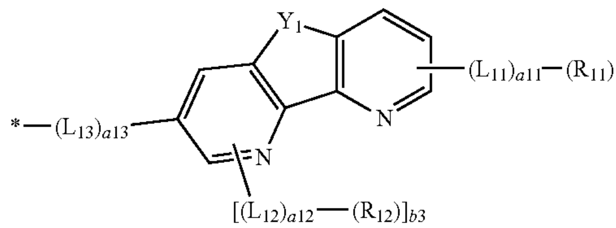
Formula (3)-11
