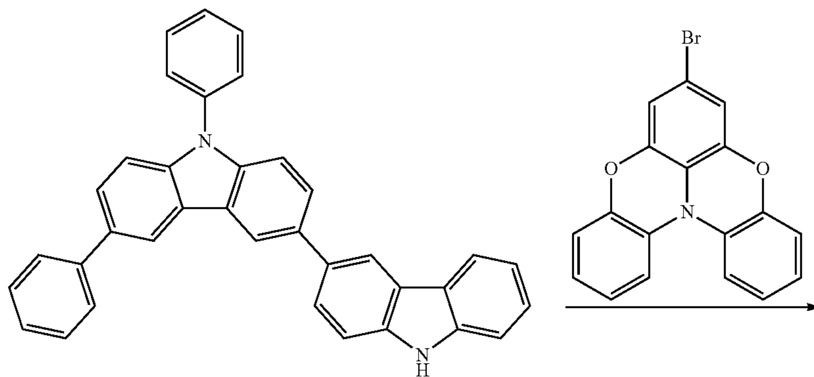
Intermediate C
