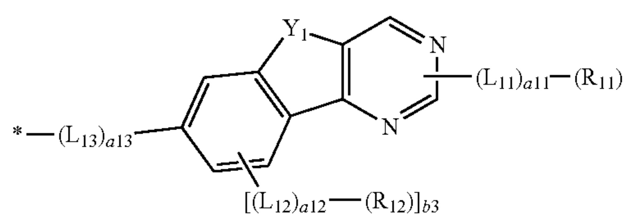
Formula (3)-5
