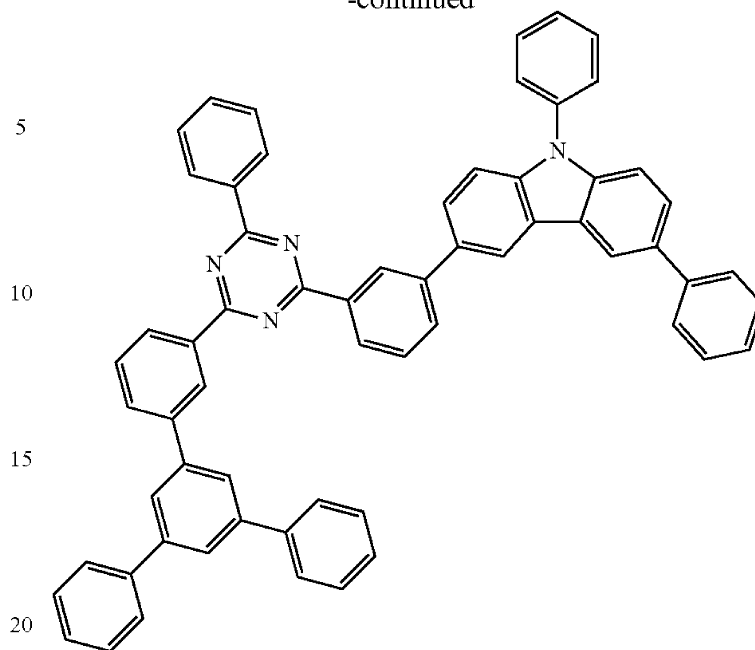
Compound 1-79
