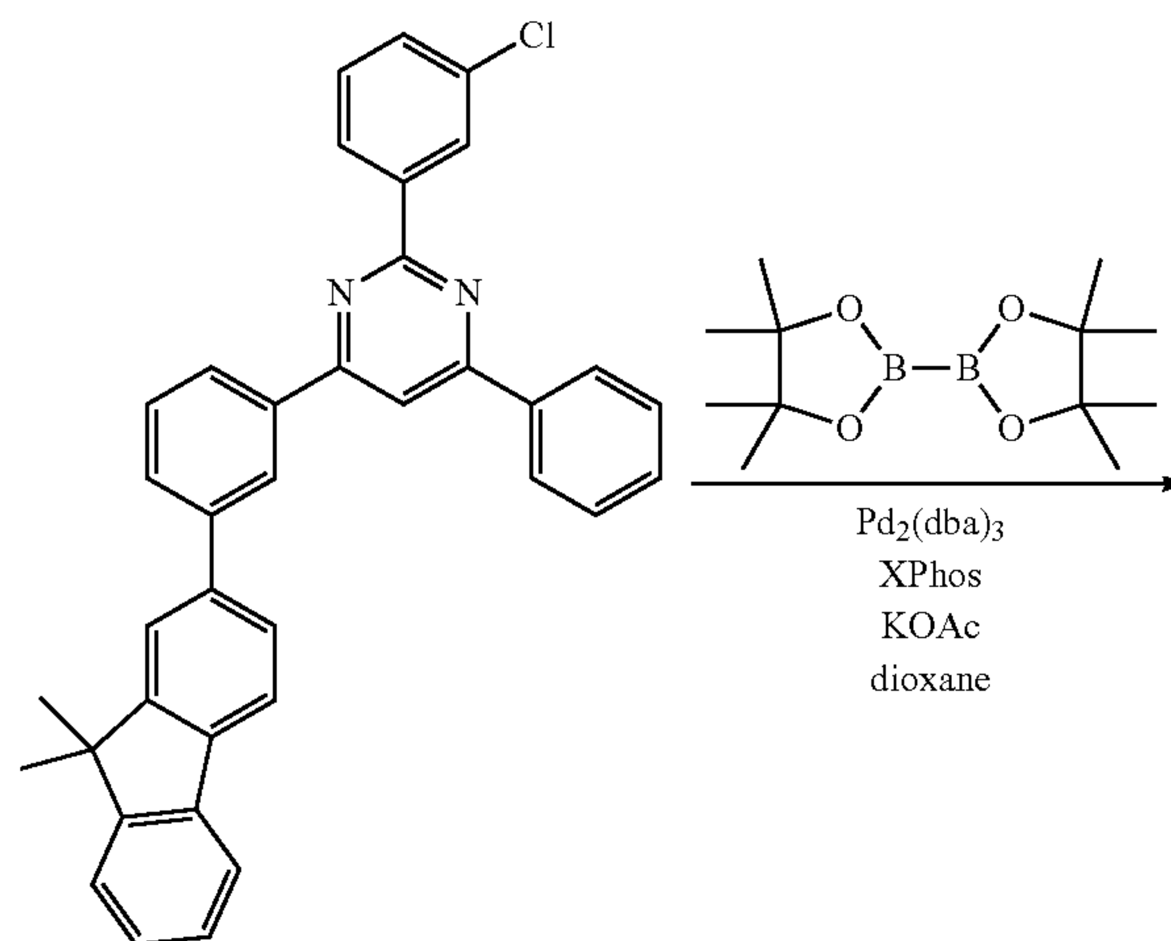
Intermediate 1-24a
