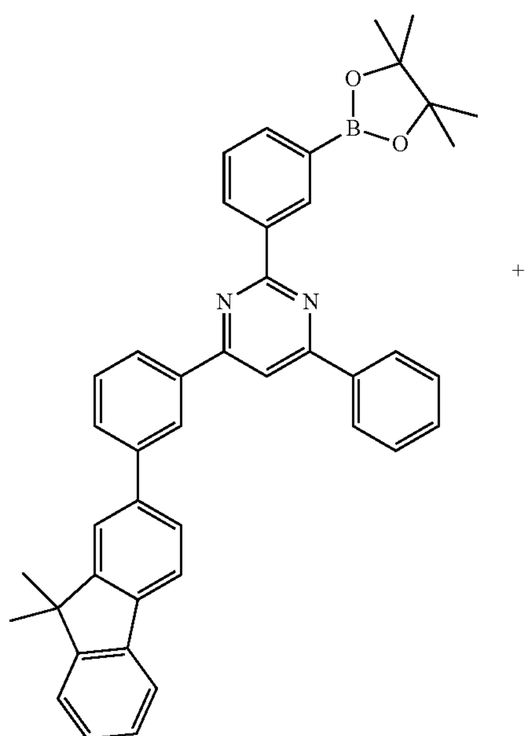
Intermediate 1-24b
