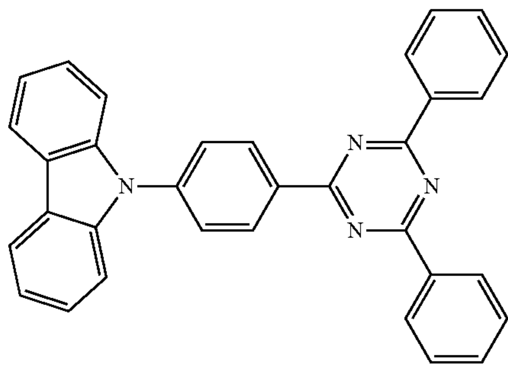
Compound h-1
