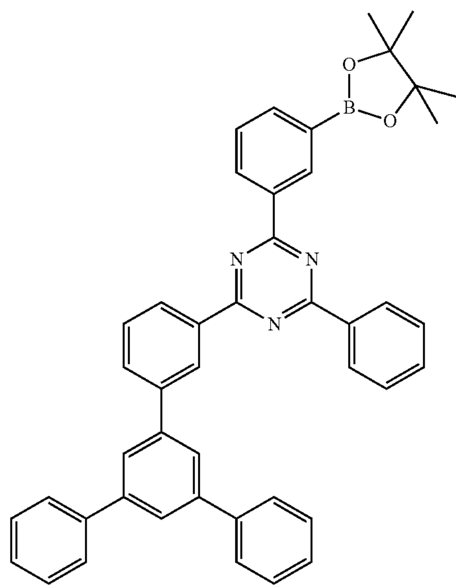
Intermediate b
