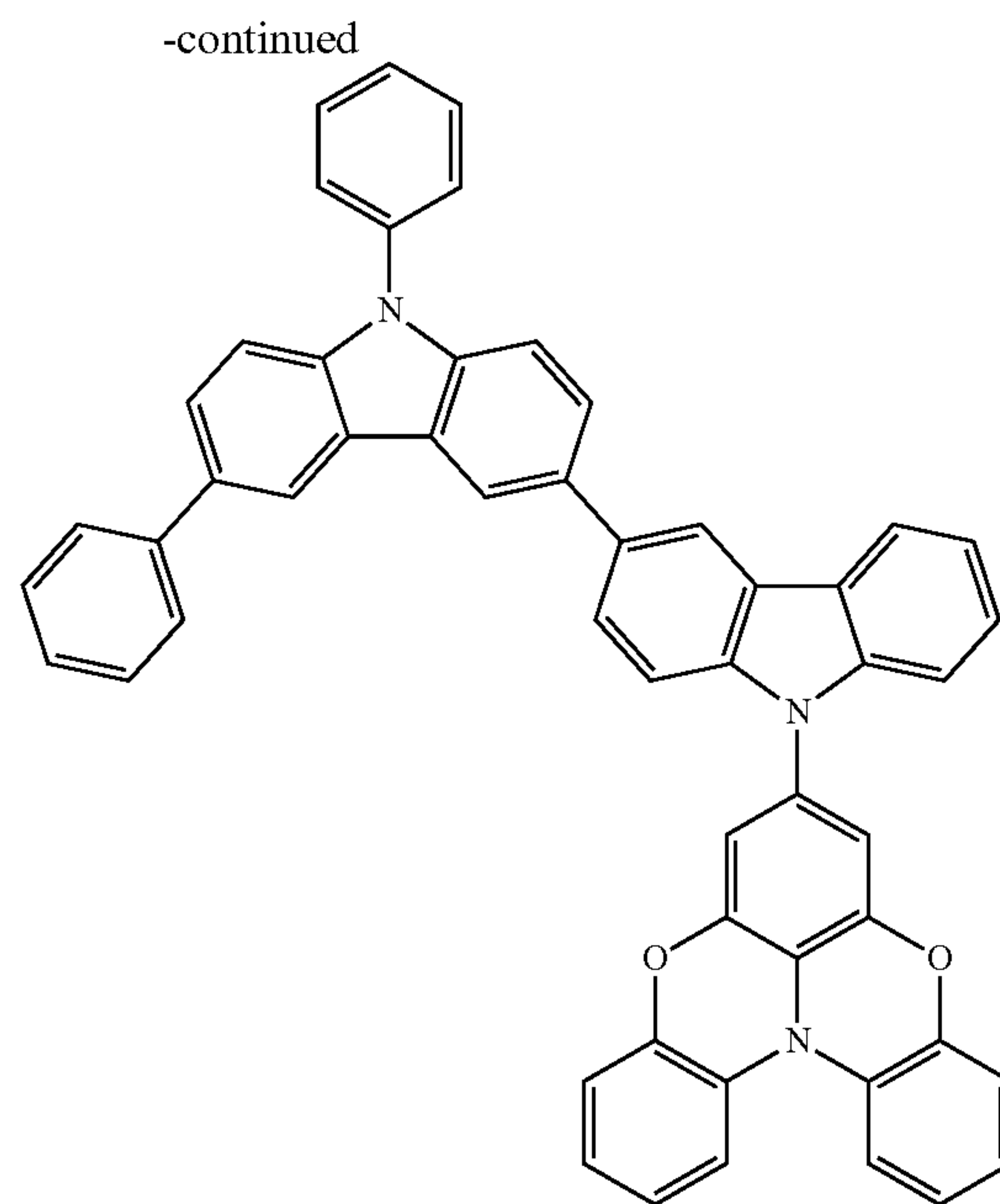
Compound 6-31
