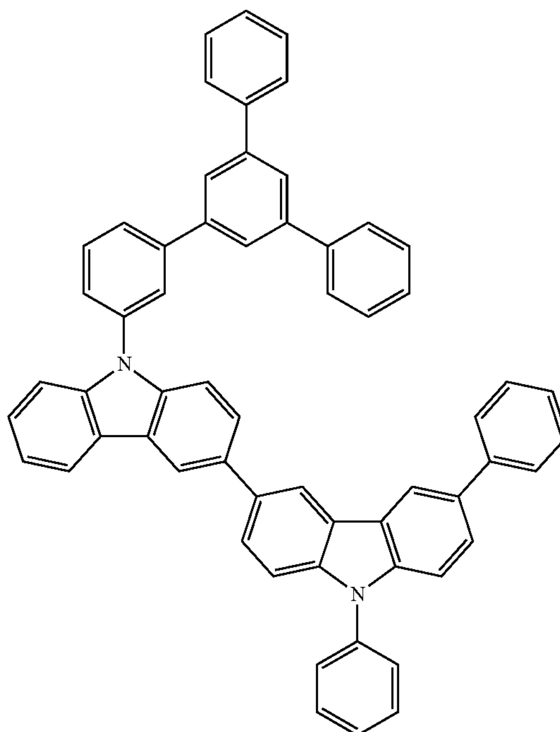
Compound 6-5
