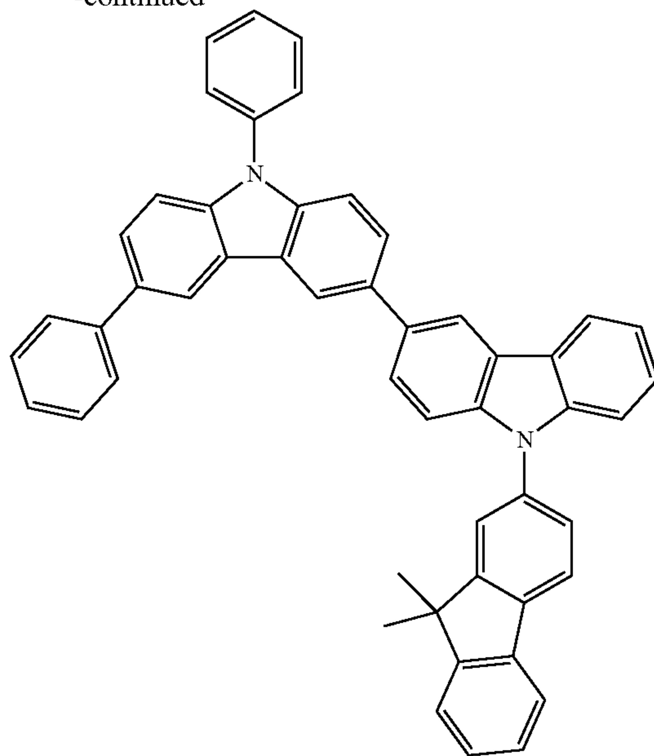
Compound 6-12
