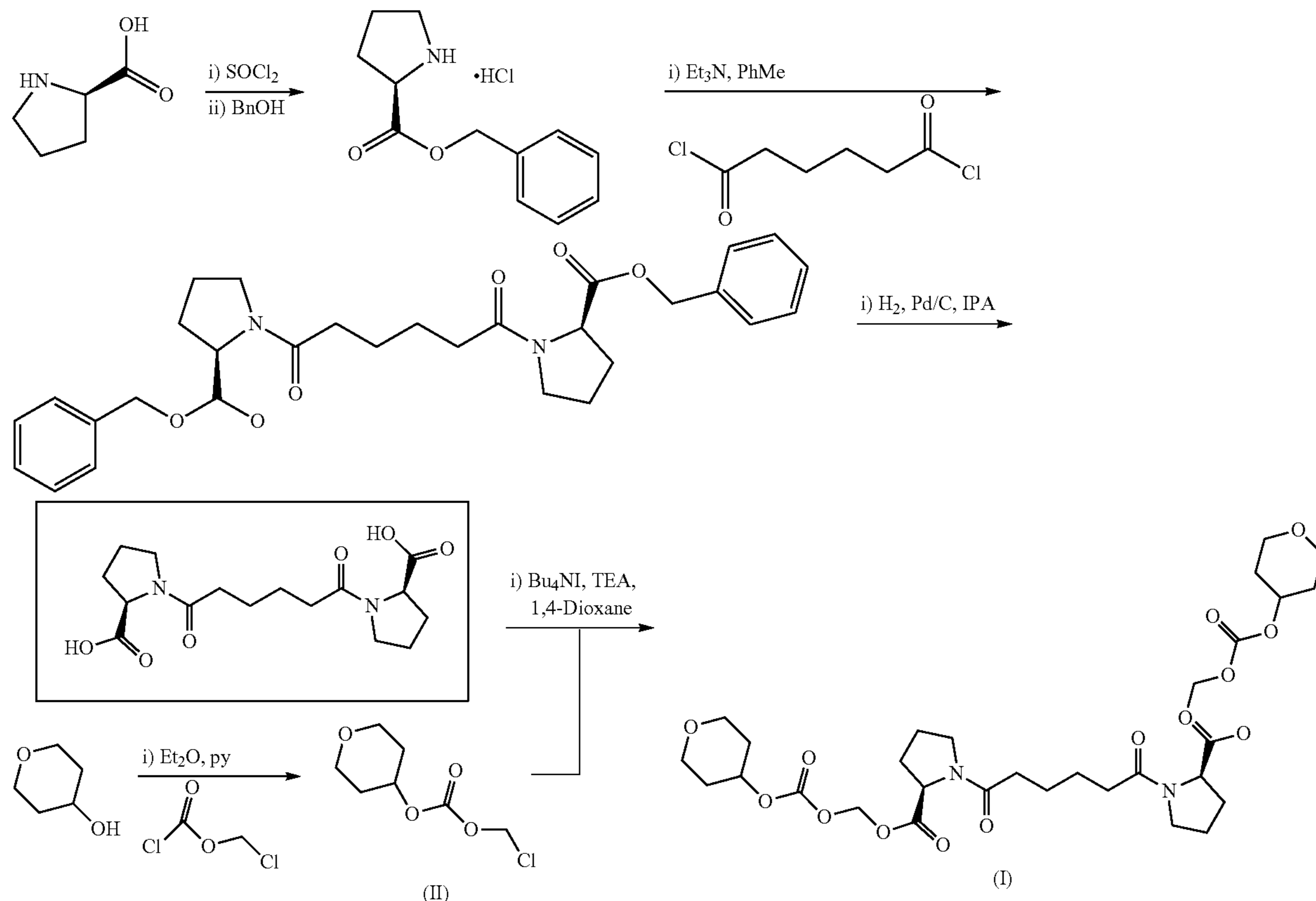
Reaction Scheme 2
