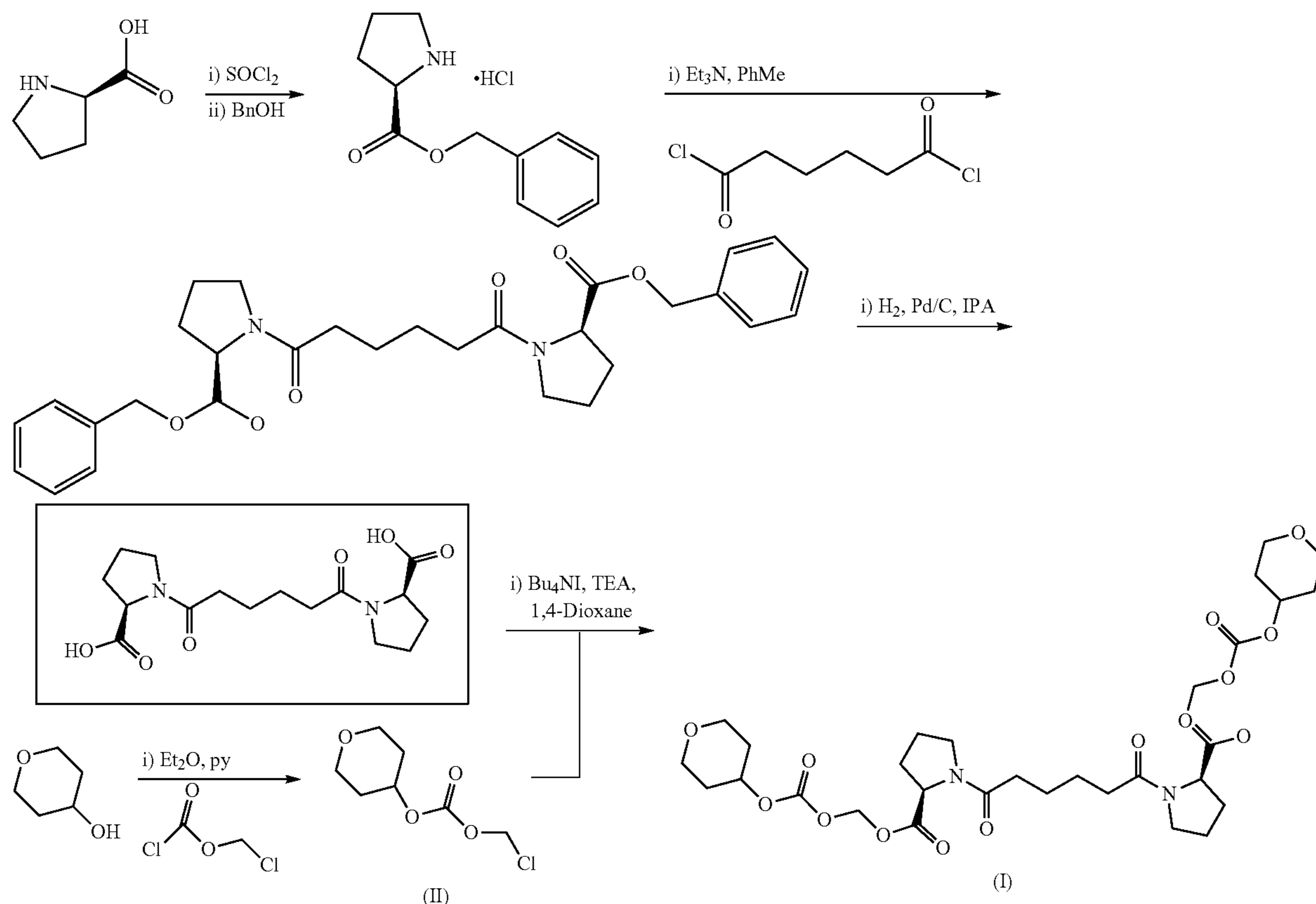
Reaction Scheme 2
