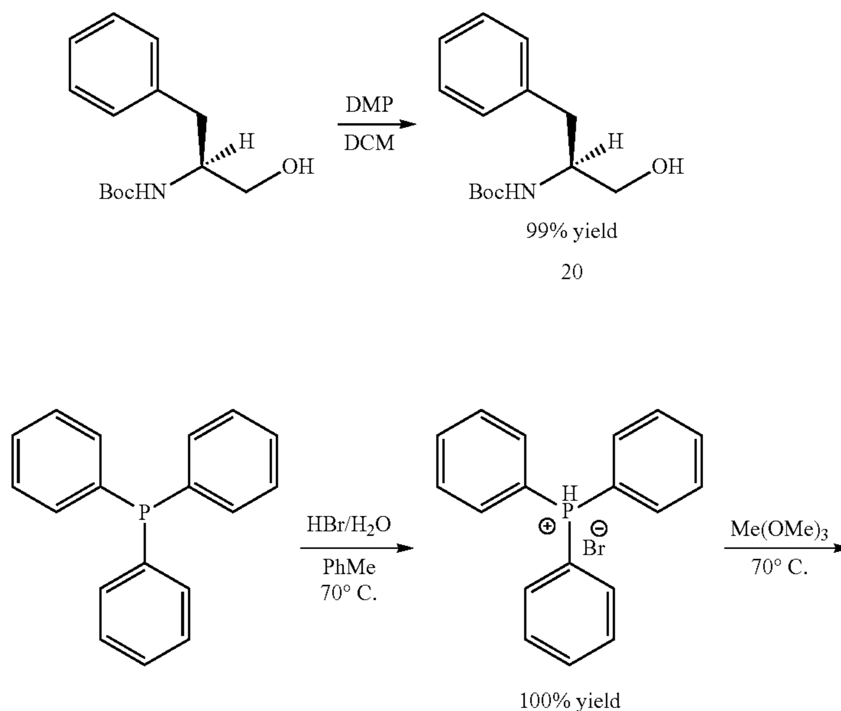
Scheme 1
