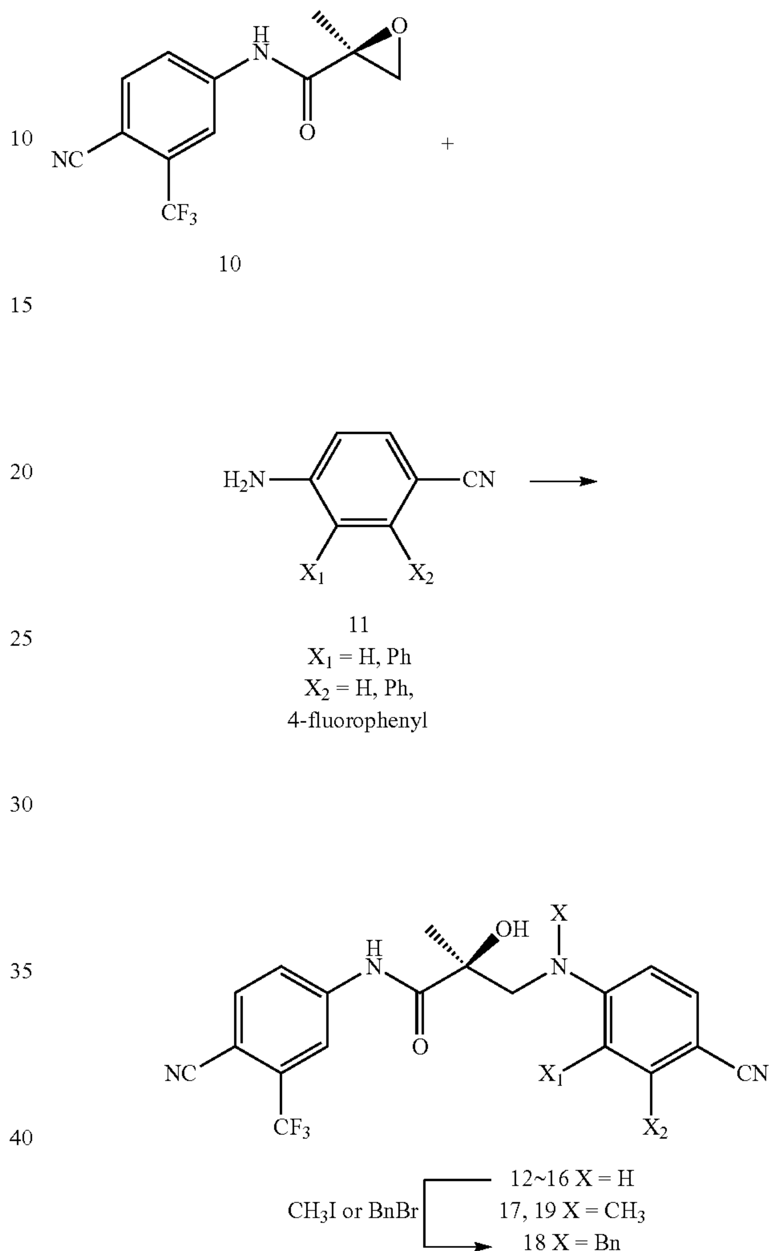
Scheme 3. Preparation of SARDs 12-19.
