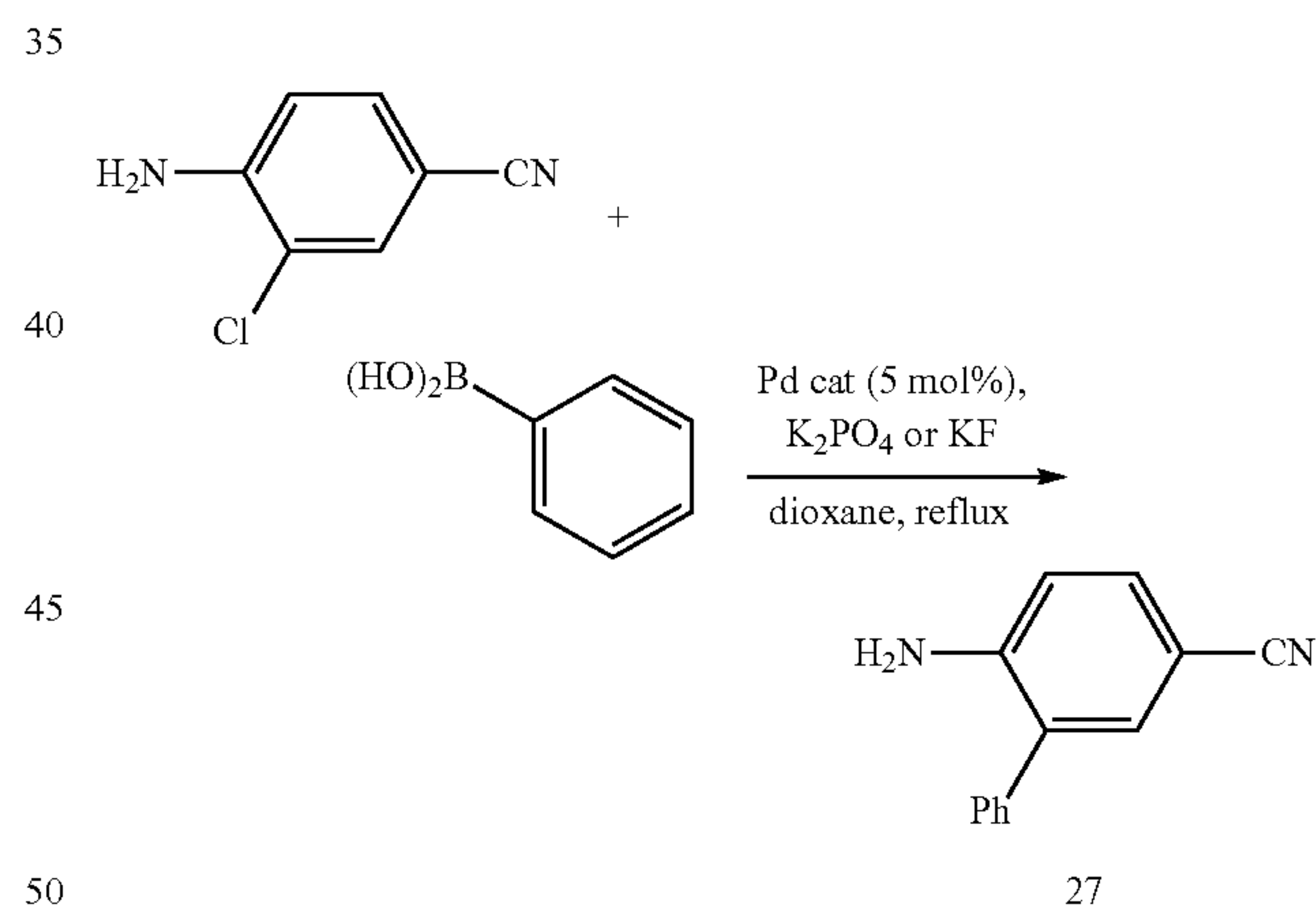
Scheme 2. Preparation of 4-cyano 2,3-substituted anilines (26-28).
