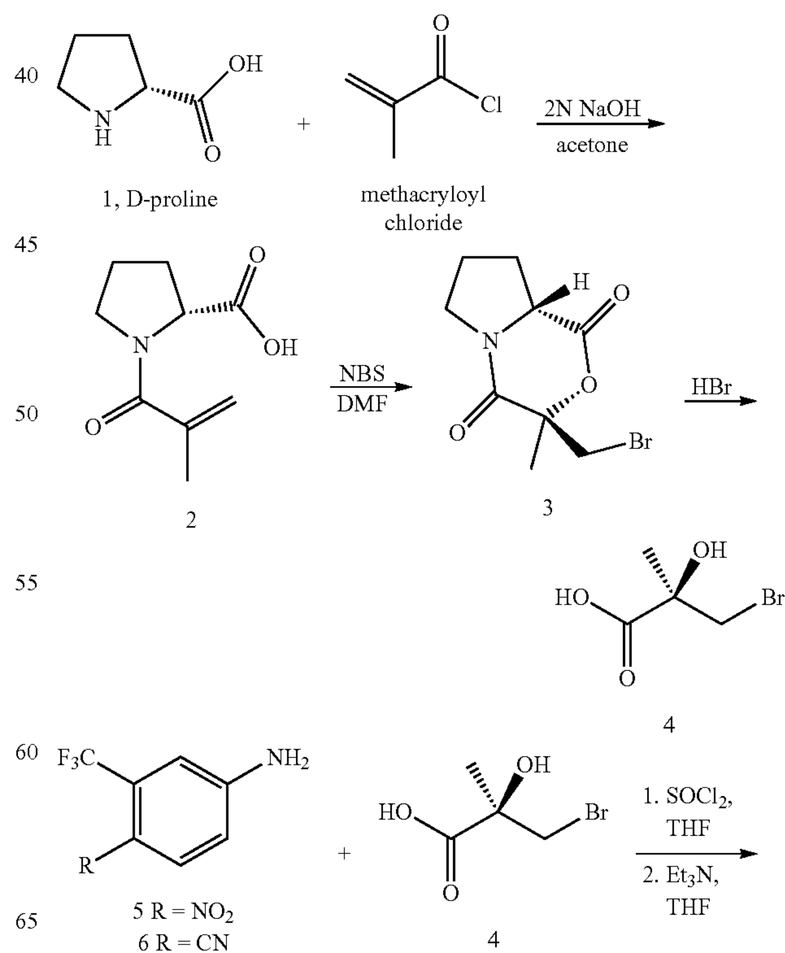
Scheme 1. Synthesis of (S)-3-(substituted phenyl amino)-N-(4-nitro- or 4-cyano-3-(trifluoromethyl)phenyl)-2-hydroxy-2-methylpropanamides (12~19).
