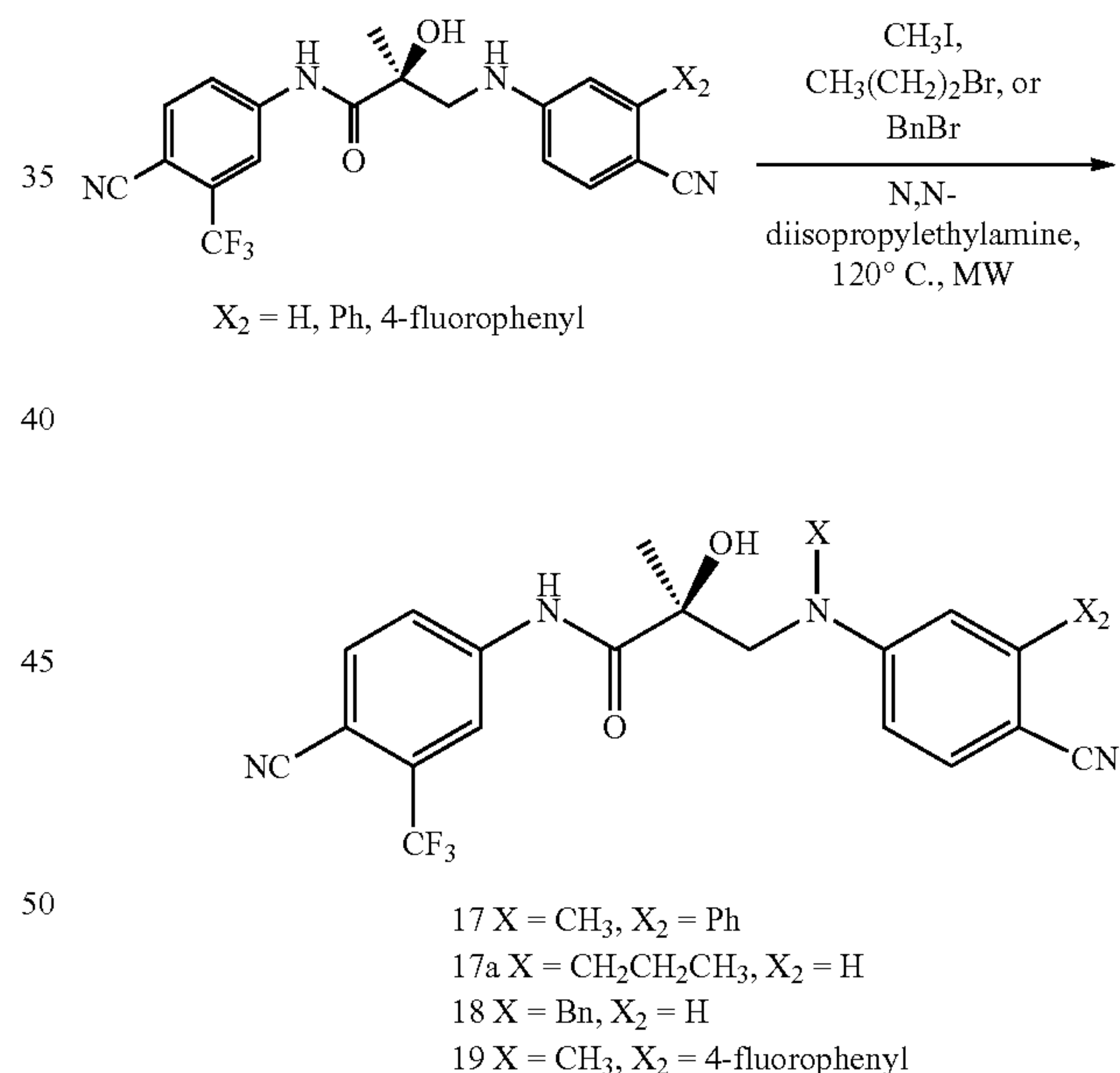
Scheme 4. Preparation of SARDs 17-19 and 17a.
