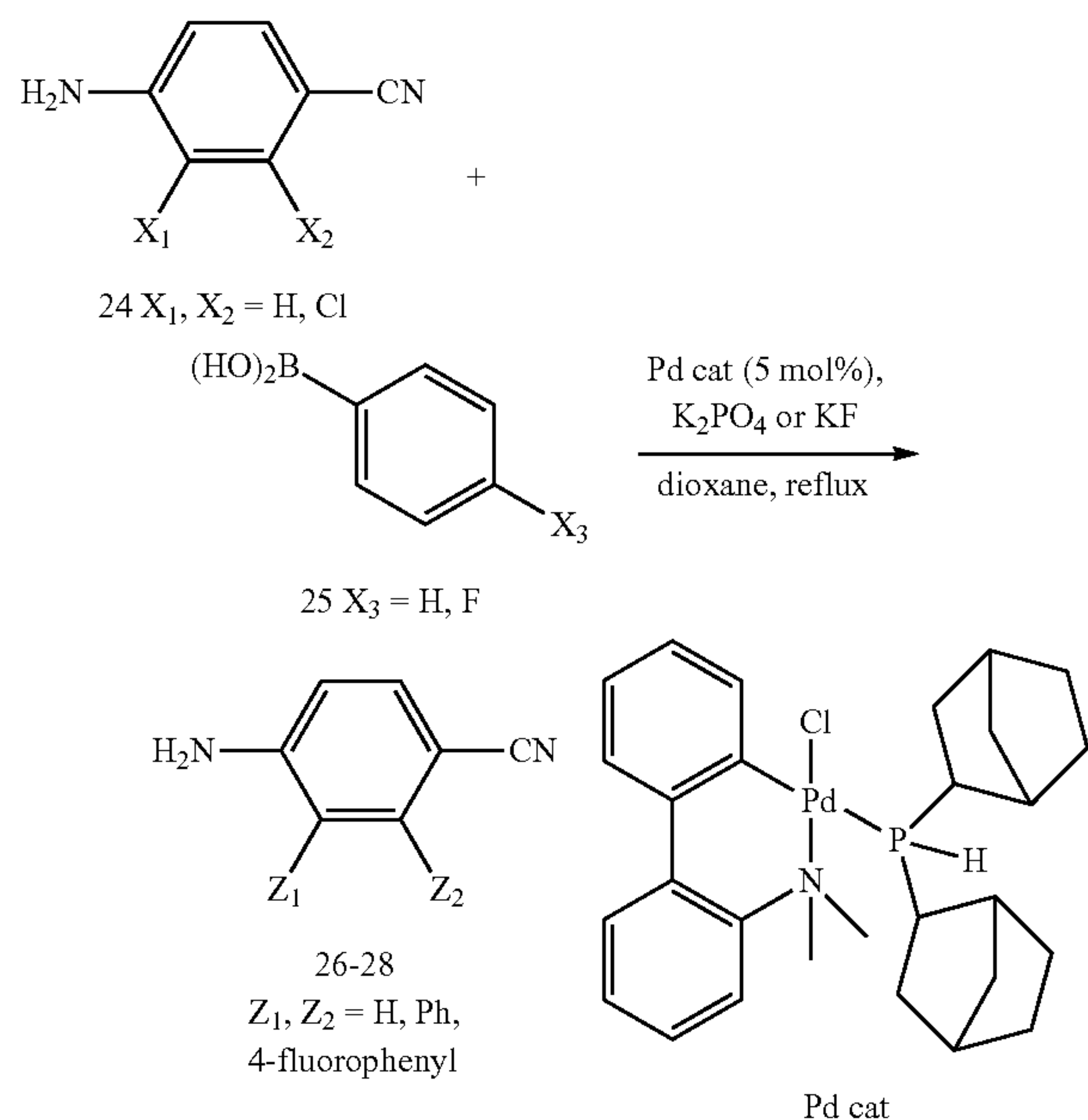
Scheme 2. Preparation of 4-cyano 2,3-substituted anilines (26-28).
