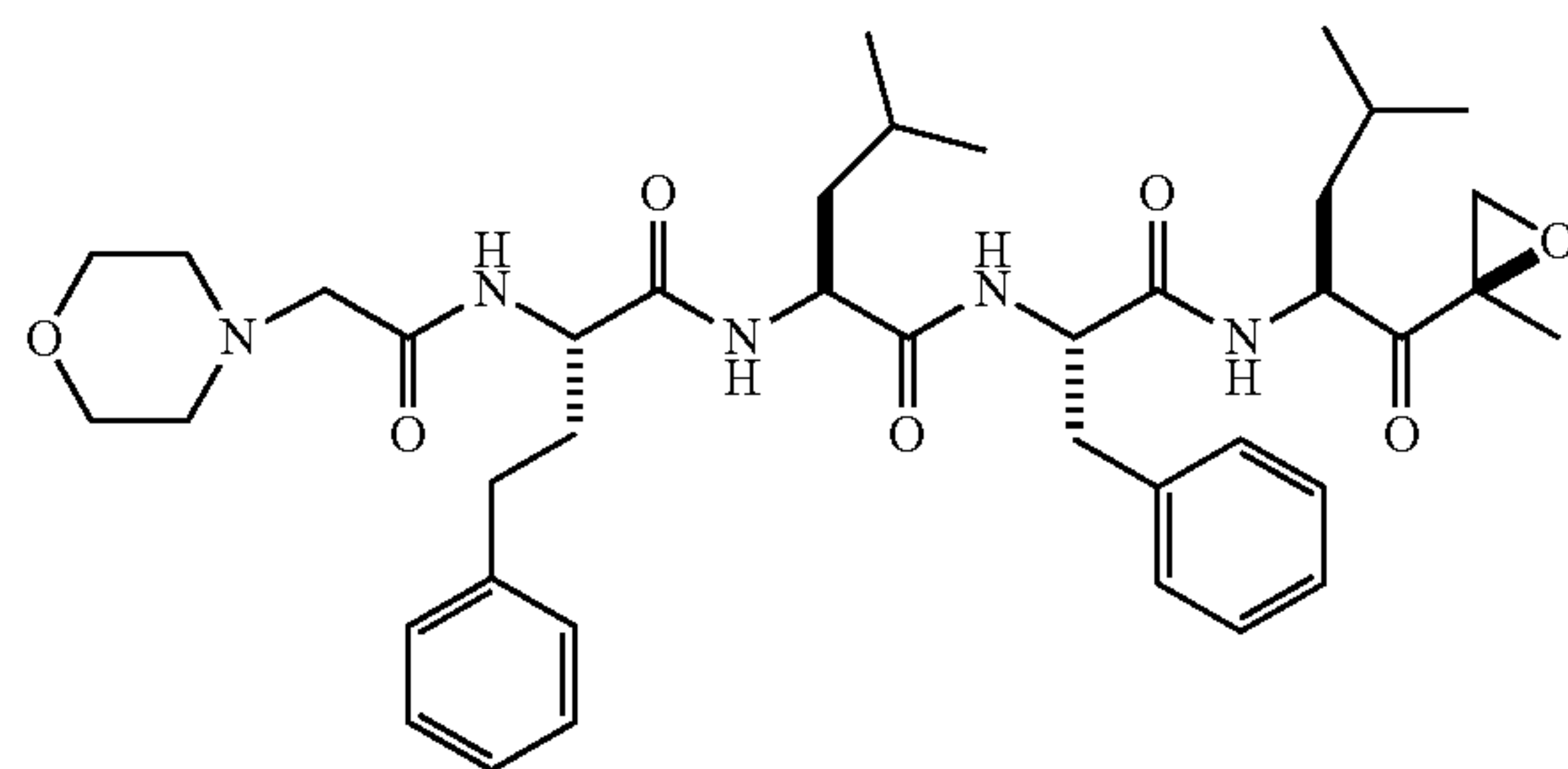
Compound 1
