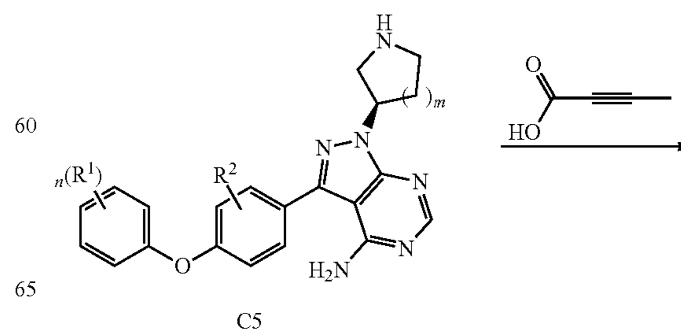
Scheme 6
