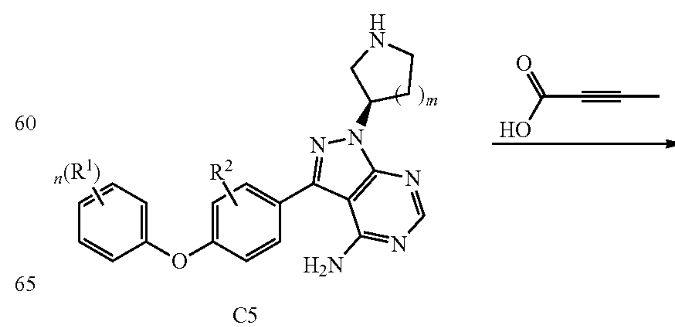
Scheme 6
