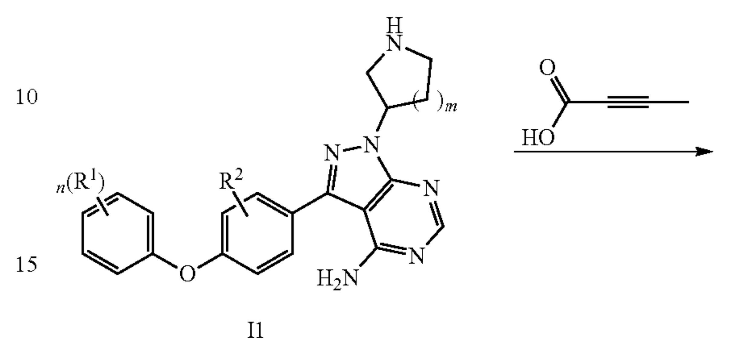
Scheme 4
