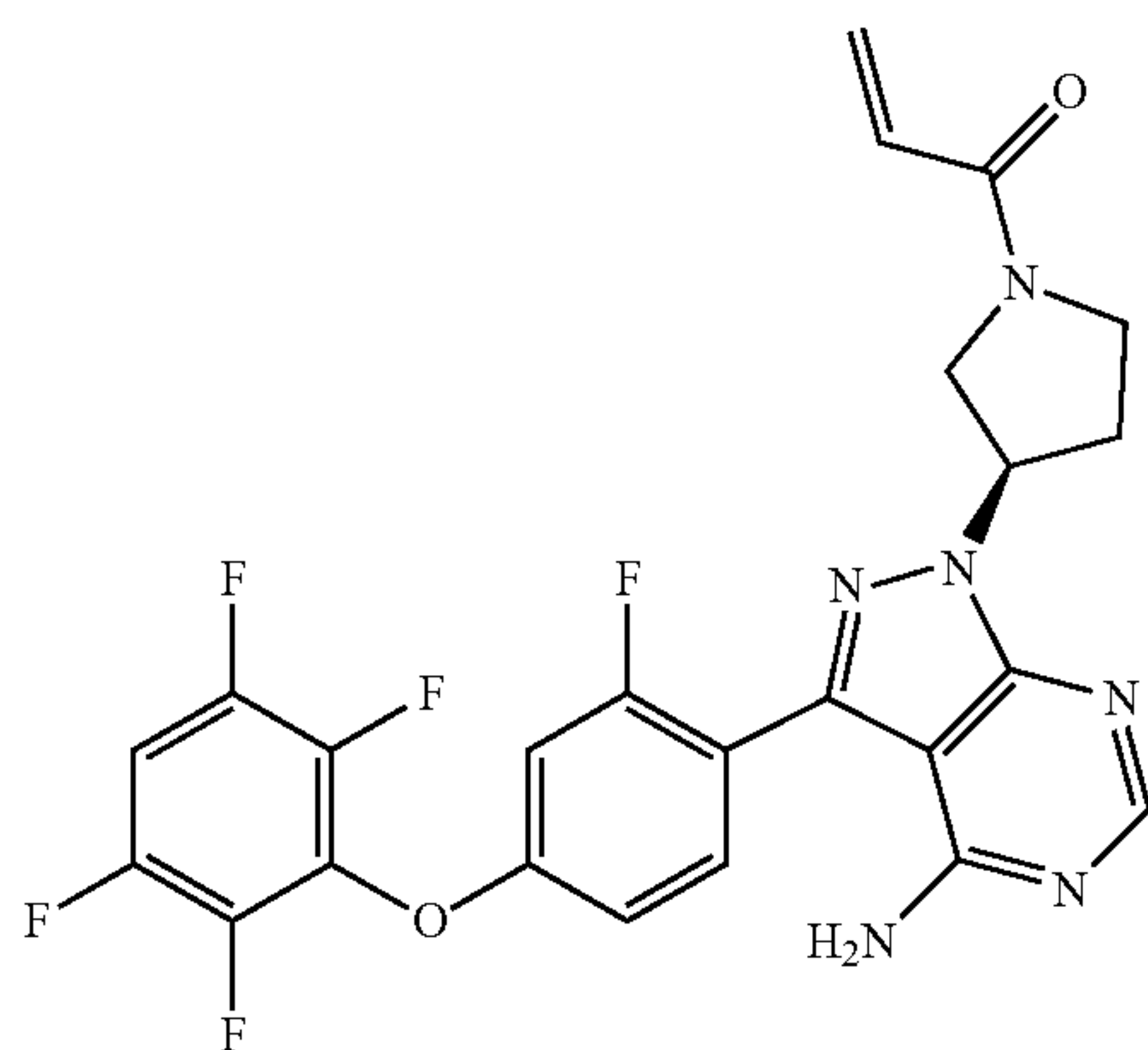
1-((R)-3-(4-amino-3-(2-fluoro-4-(2,3,5,6-tetrafluorophenoxy)phenyl)-1H-pyrazolo[3,4-d]pyrimidin-1-yl)pyrrolidin-1-yl)prop-2-en-1-one
