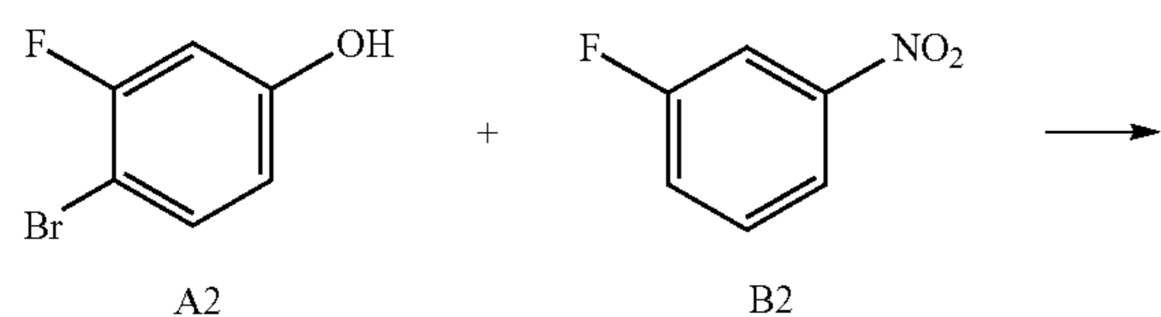
Scheme 2
