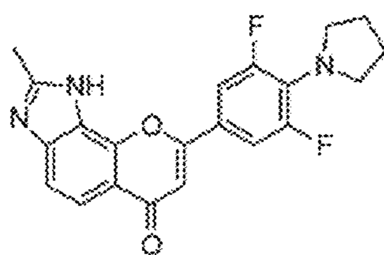
TCRS-198 MW = 381
