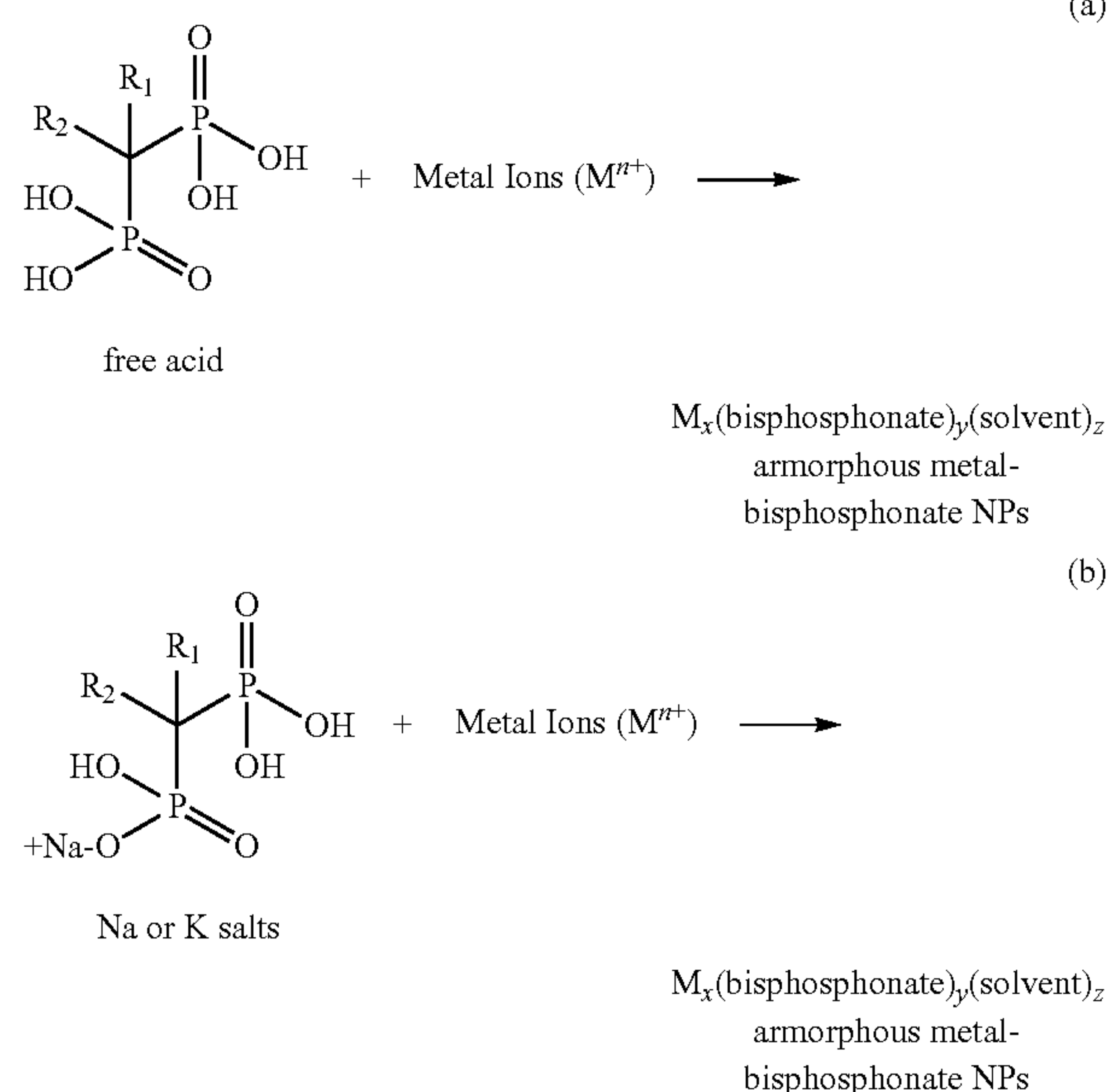
Scheme 3. Synthesis of Amorphous Metal-Bisphosphonate Nanoparticles.
