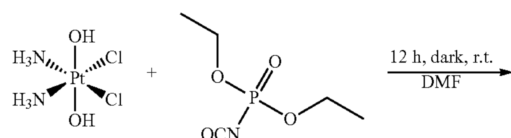
Scheme 4. Synthesis of Cisplatin Bisphosphonate Complex.
