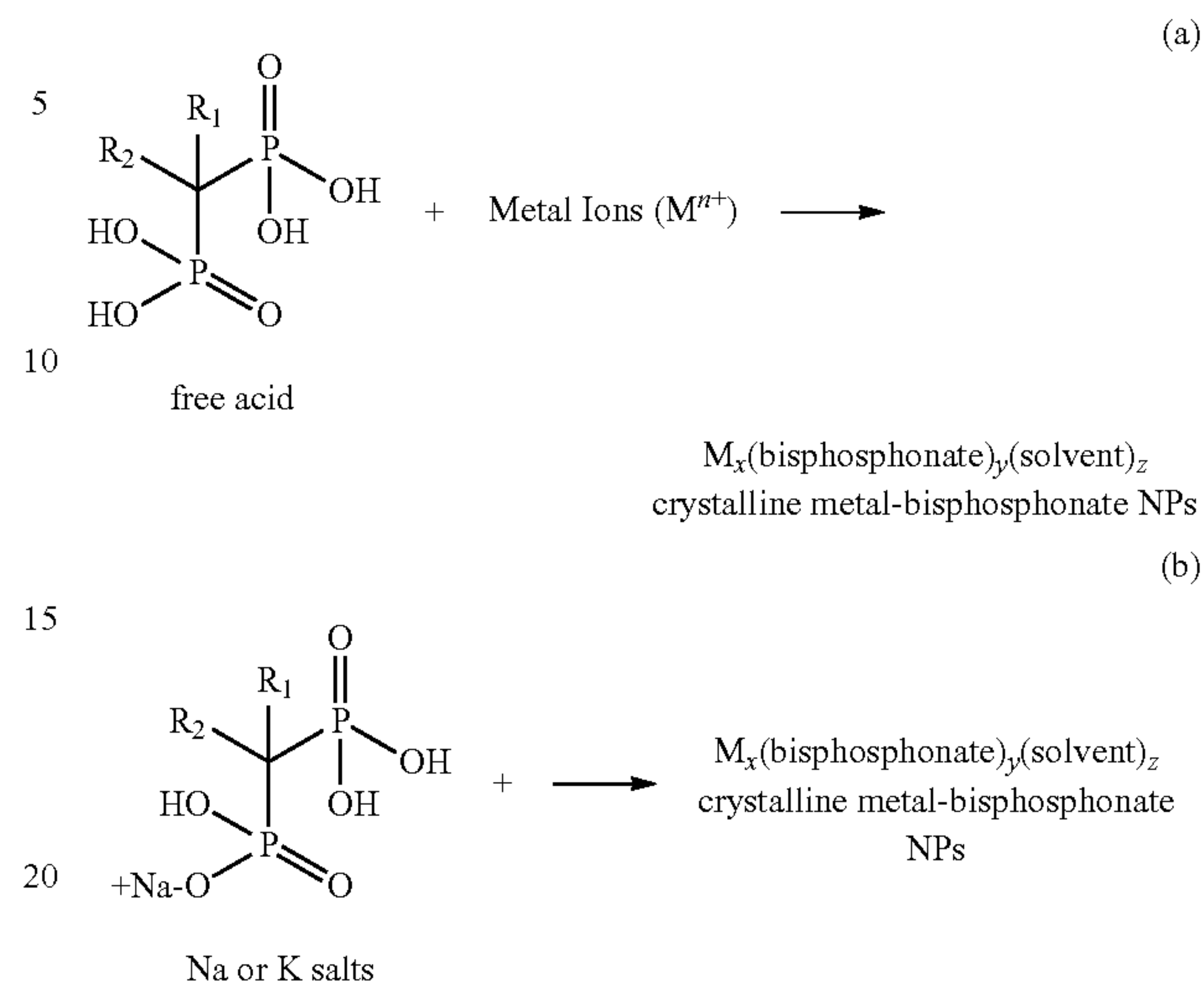
Scheme 2. Synthesis of Crystalline Metal-Bisphosphonate Nanoparticles.
