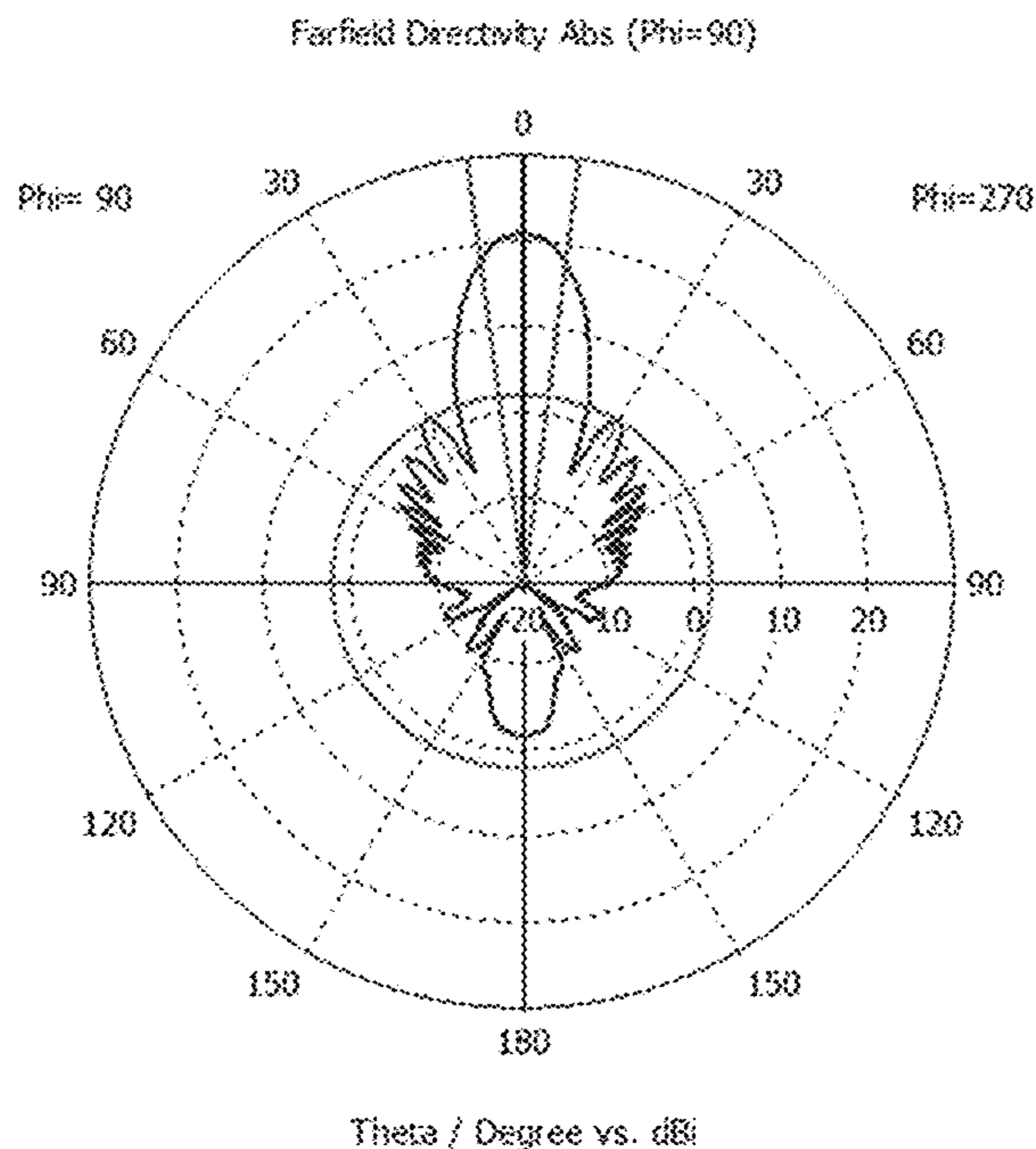
Antenna Gain Pattern
