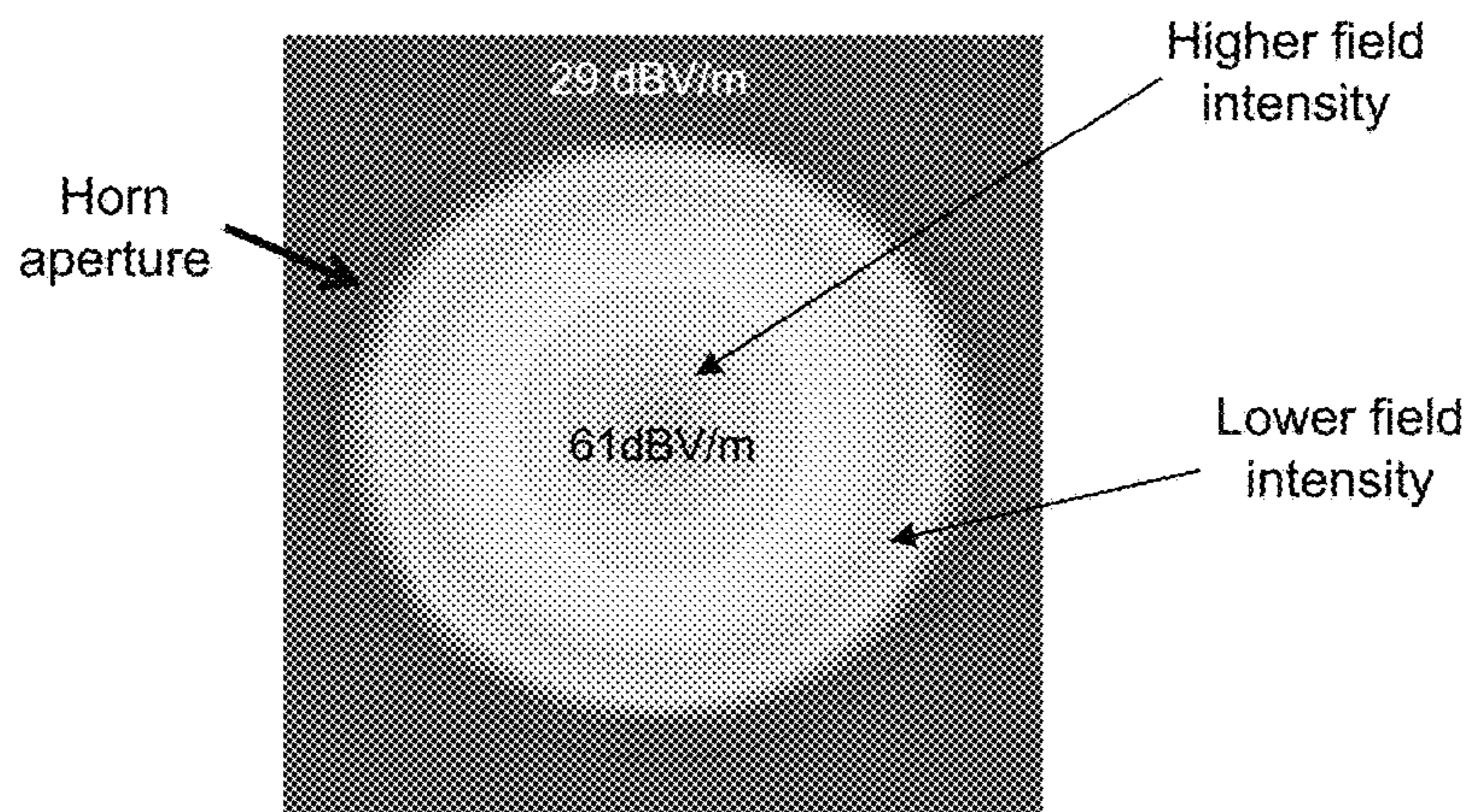
E-field Intensity Pattern
