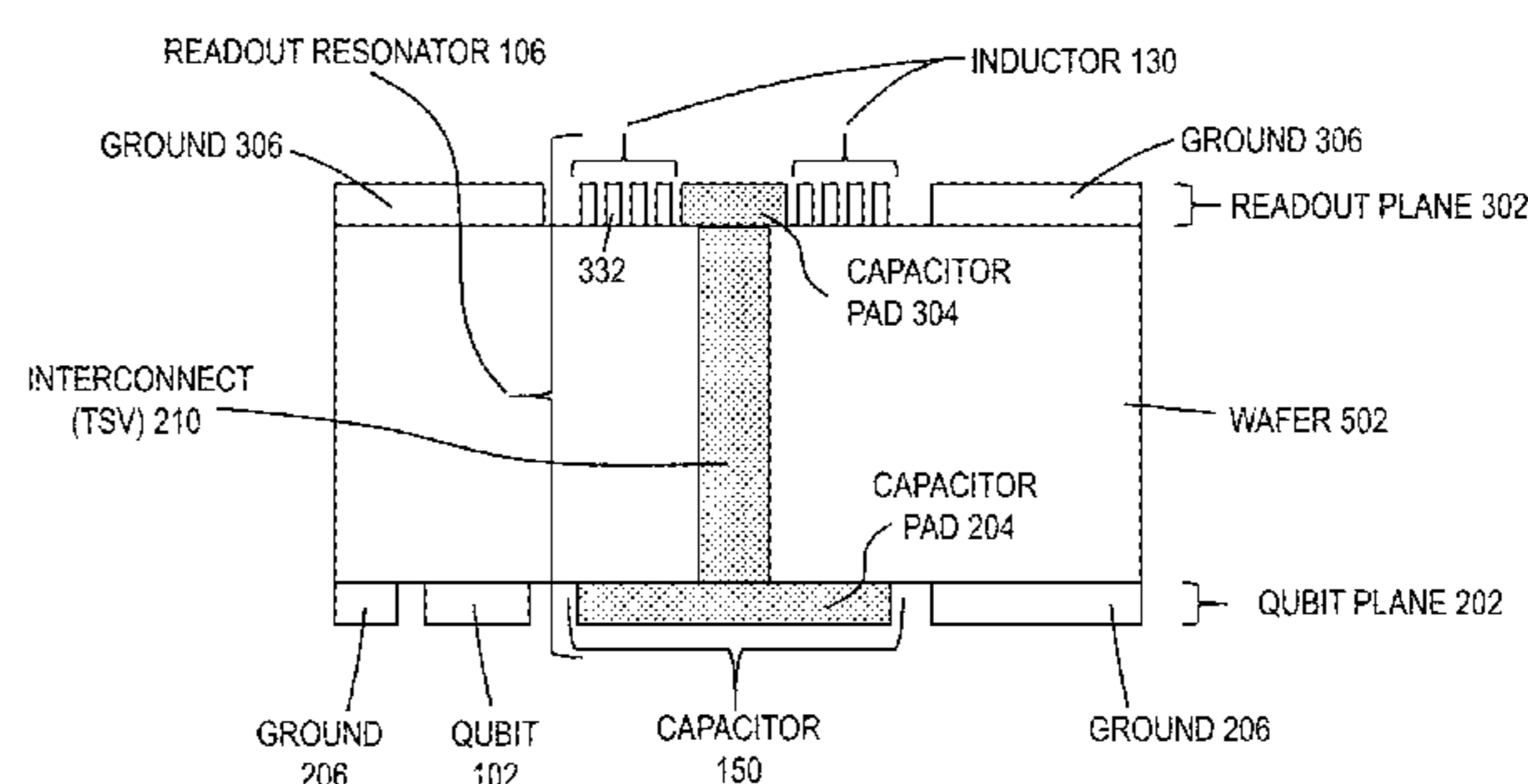
CAPACITOR PORTION:
