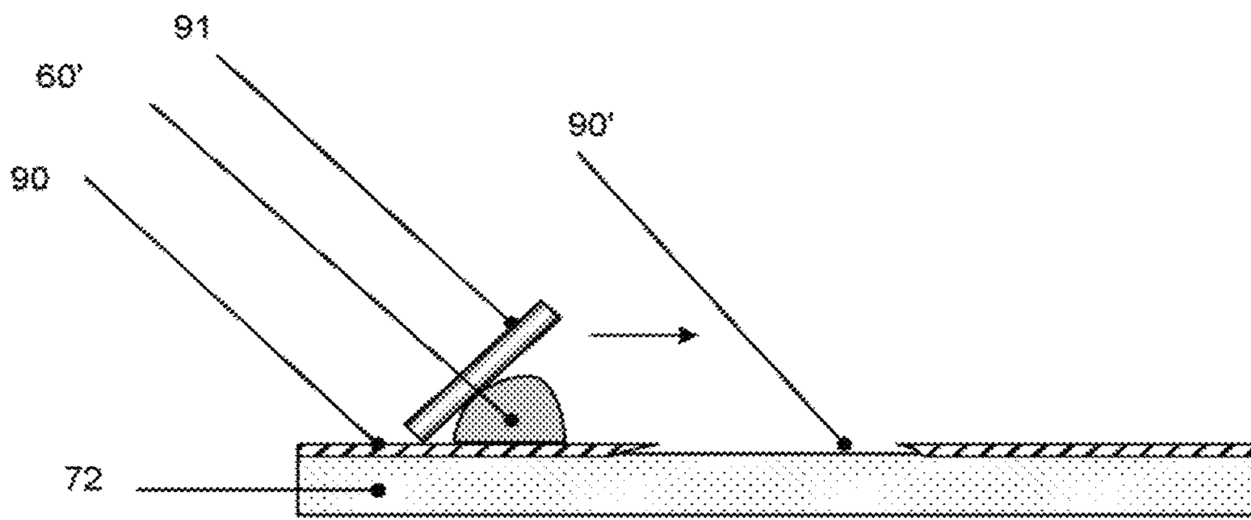
FIG. 30A - Alignment prior to screen printing
