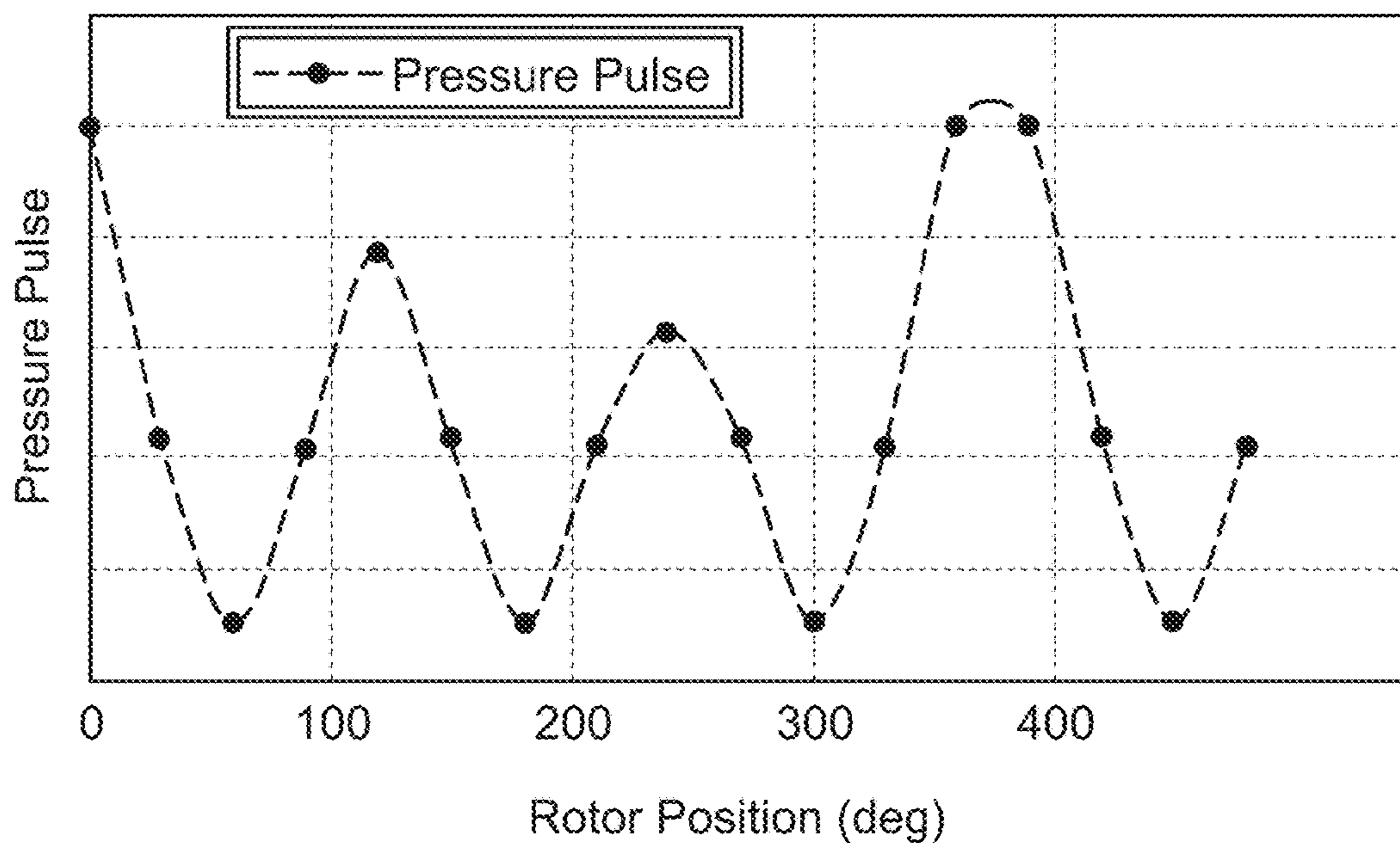
MMO - Varying Amplitude/Constant Wavelength Downhole Oscillation Tool Rotor position (time) vs Pressure Pulse
