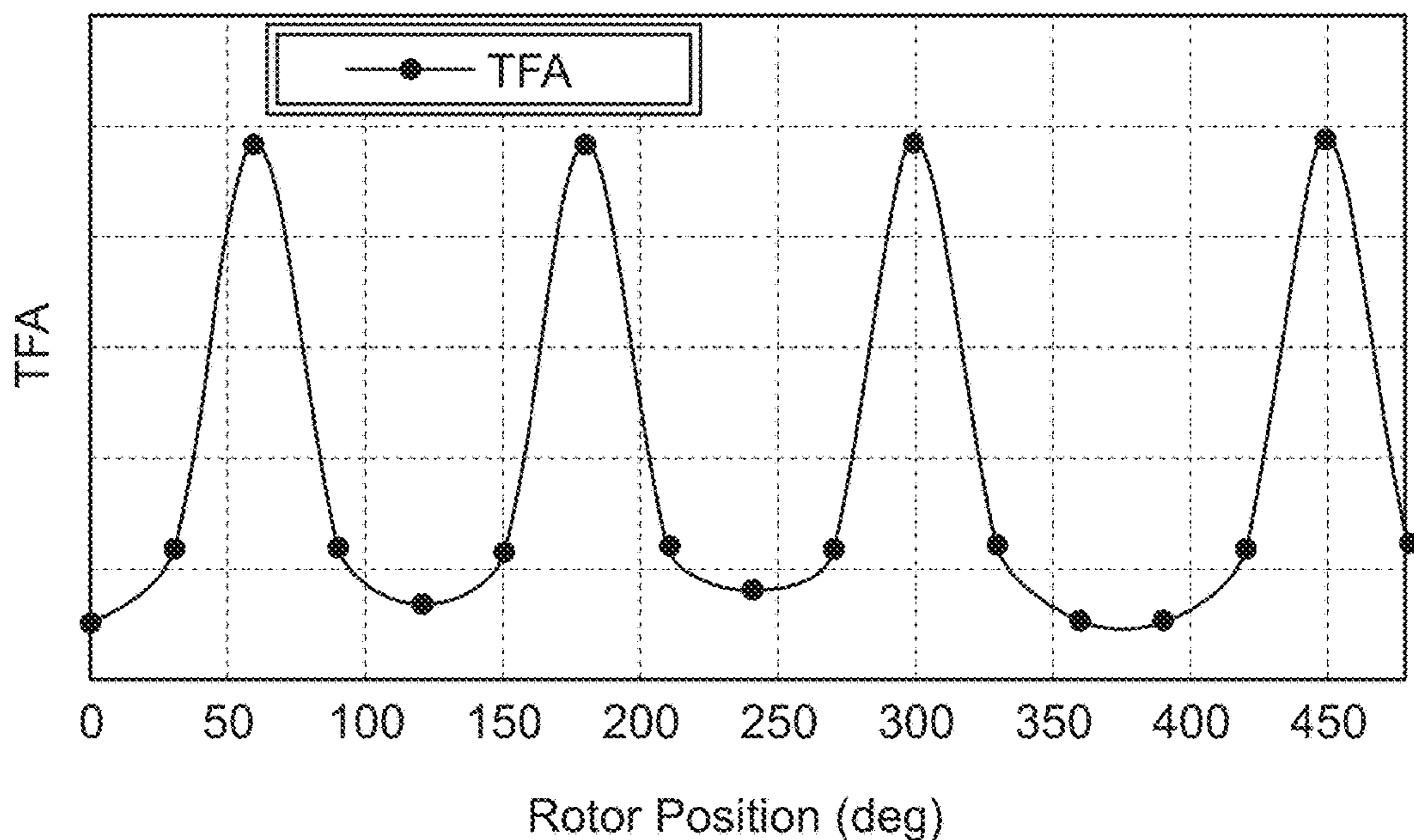
MMO - Varying Amplitude/Constant Wavelength Downhole Oscillation Tool Rotor position (time) vs TFA
