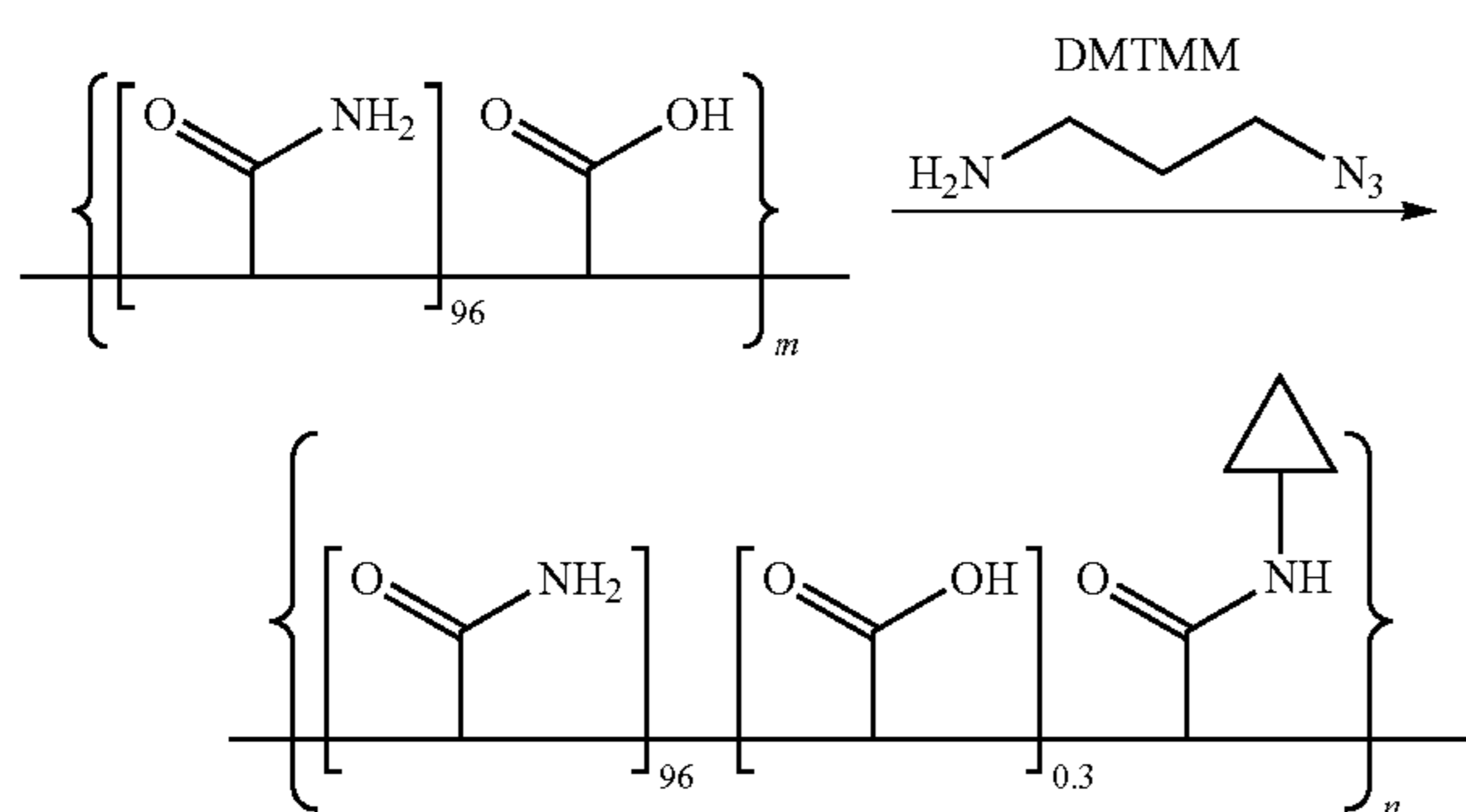
Scheme 11.
