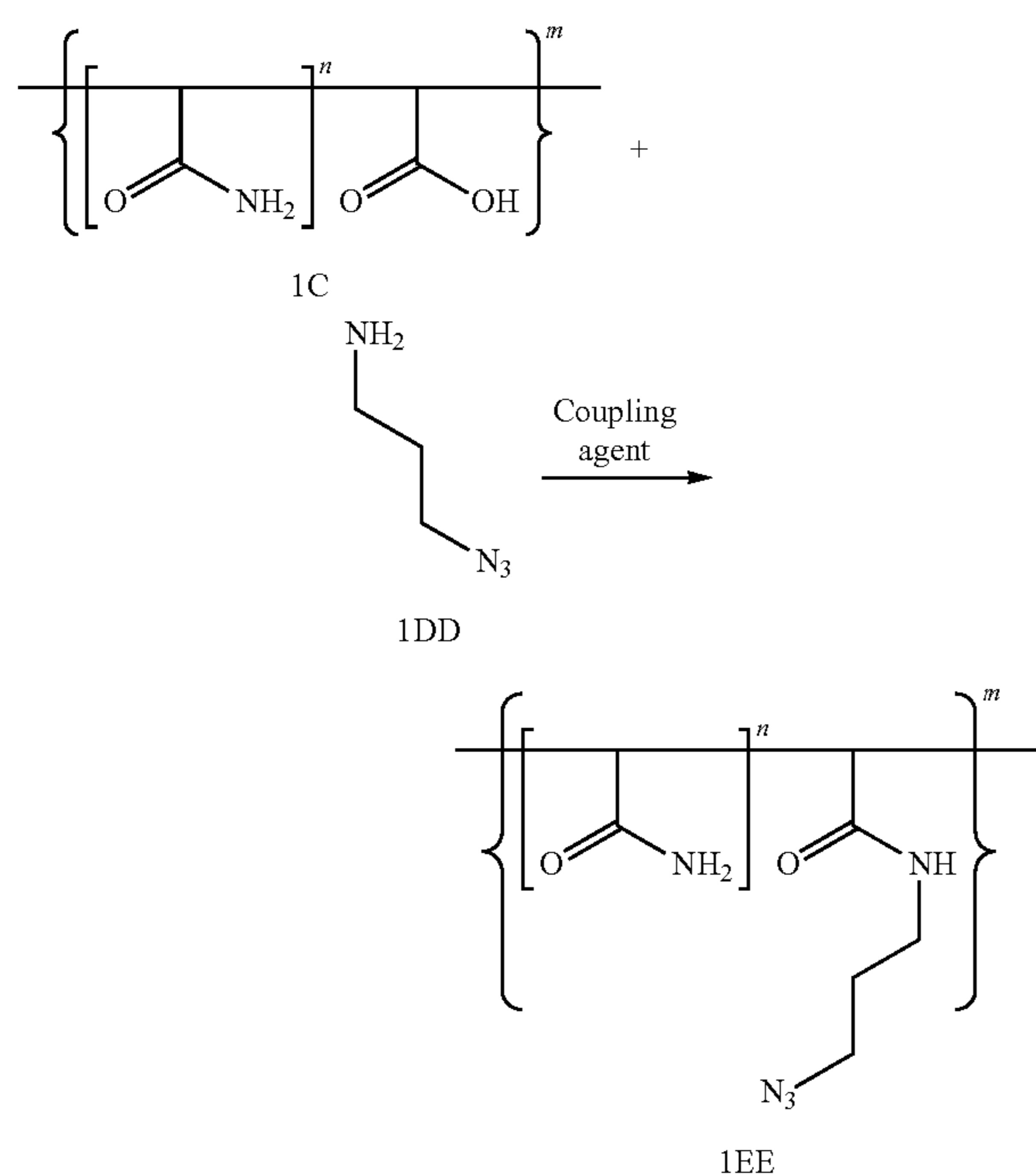
Scheme 4B.
