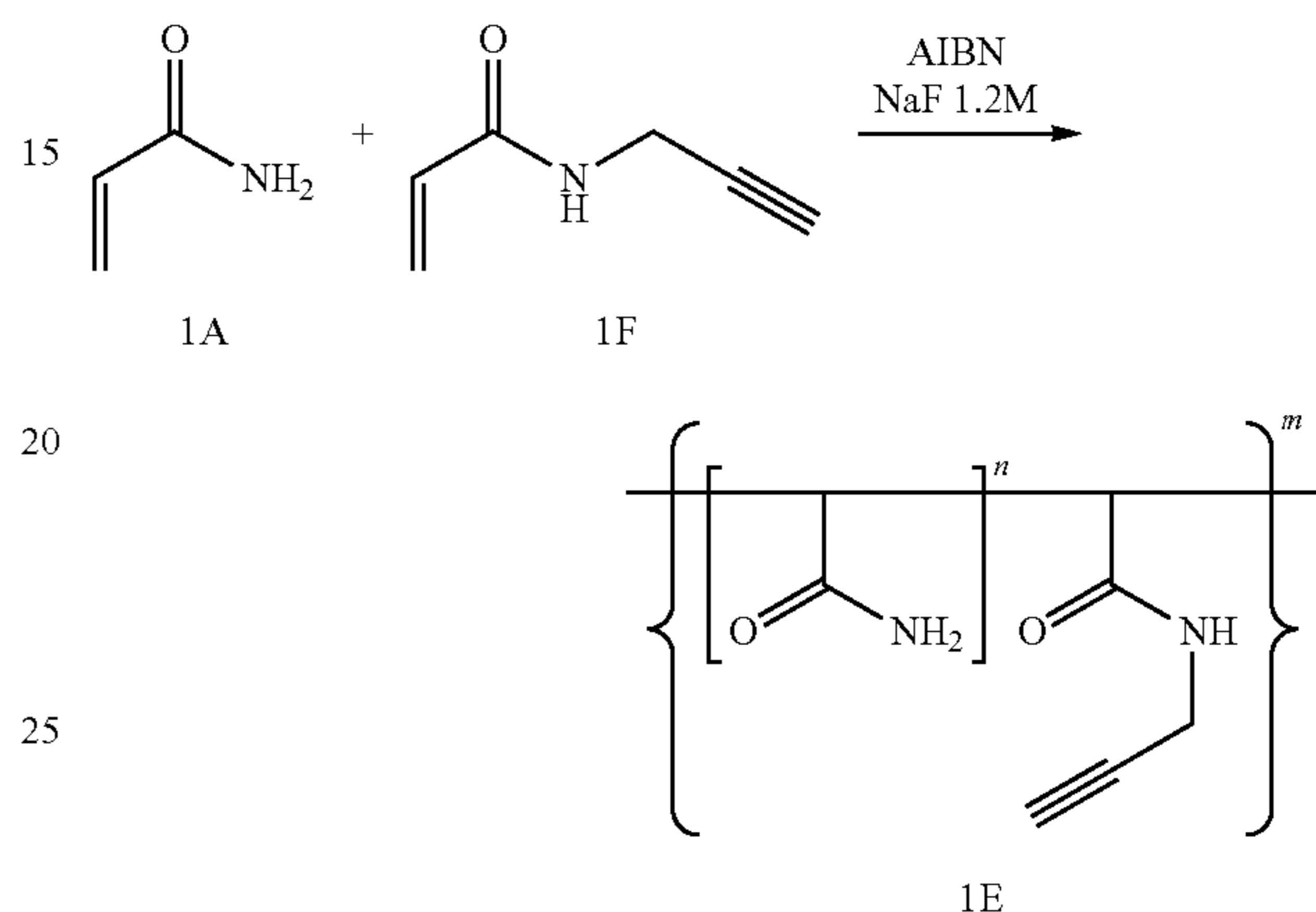
Scheme 5.
