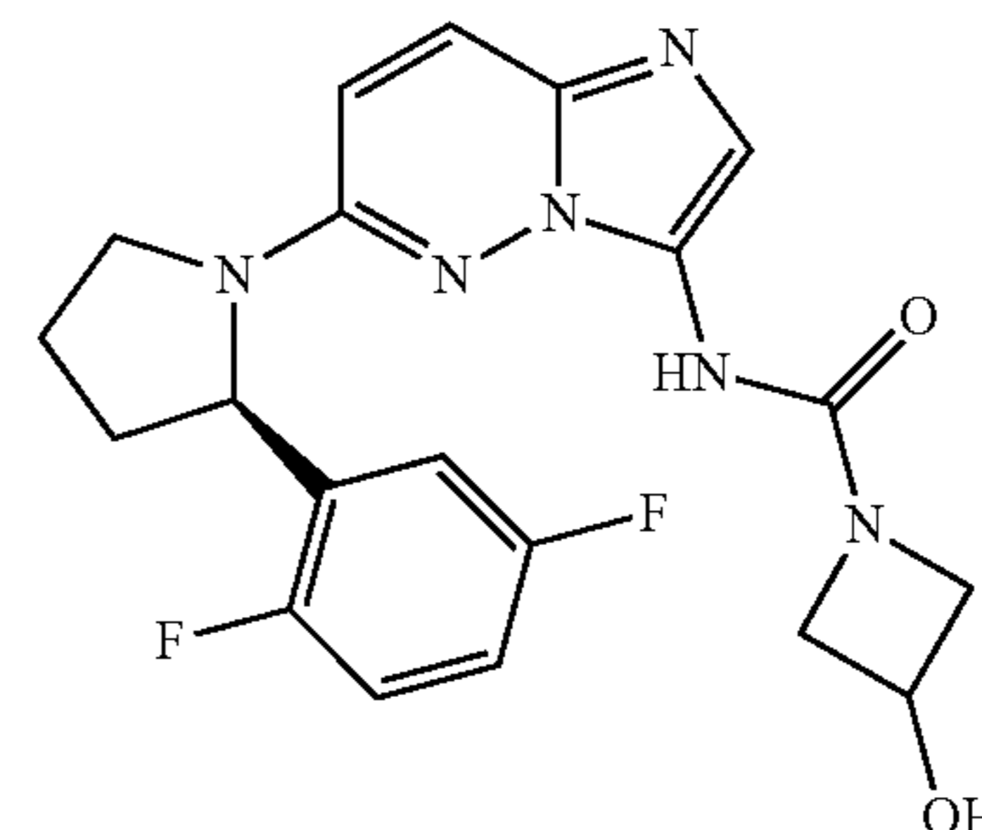
(R)—N-(6-((R)-2-(2,5-difluorophenyl)pyrrolidin-1-yl)imidazo[1,2-b]pyridazin-3-yl)-3-hydroxyazetidine-1-carboxamide
