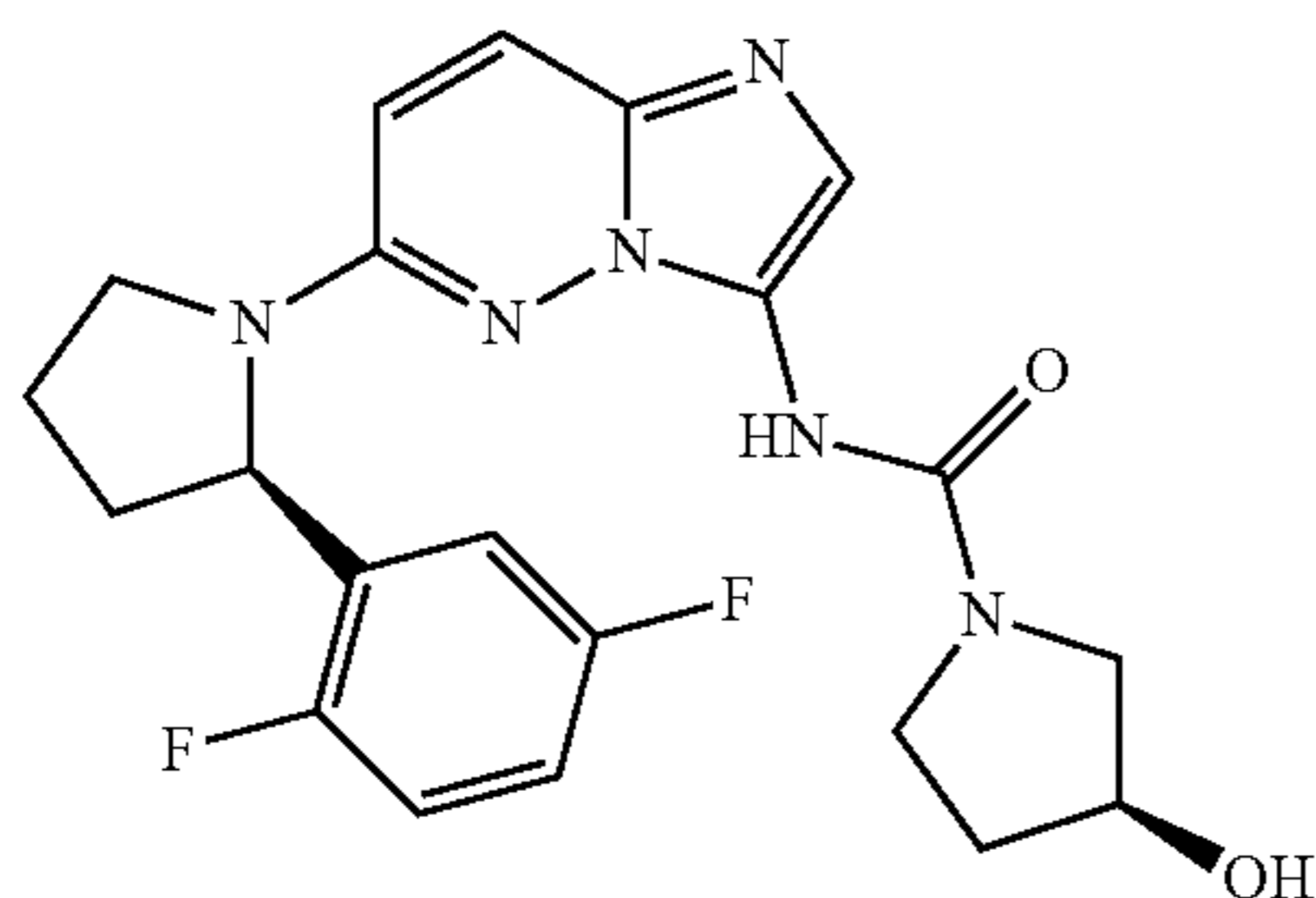
(S)—N-(6-((R)-2-(2,5-difluorophenyl)pyrrolidin-1-yl)imidazo[1,2-b]pyridazin-3-yl)-3-hydroxypyrrolidine-1-carboxamide
