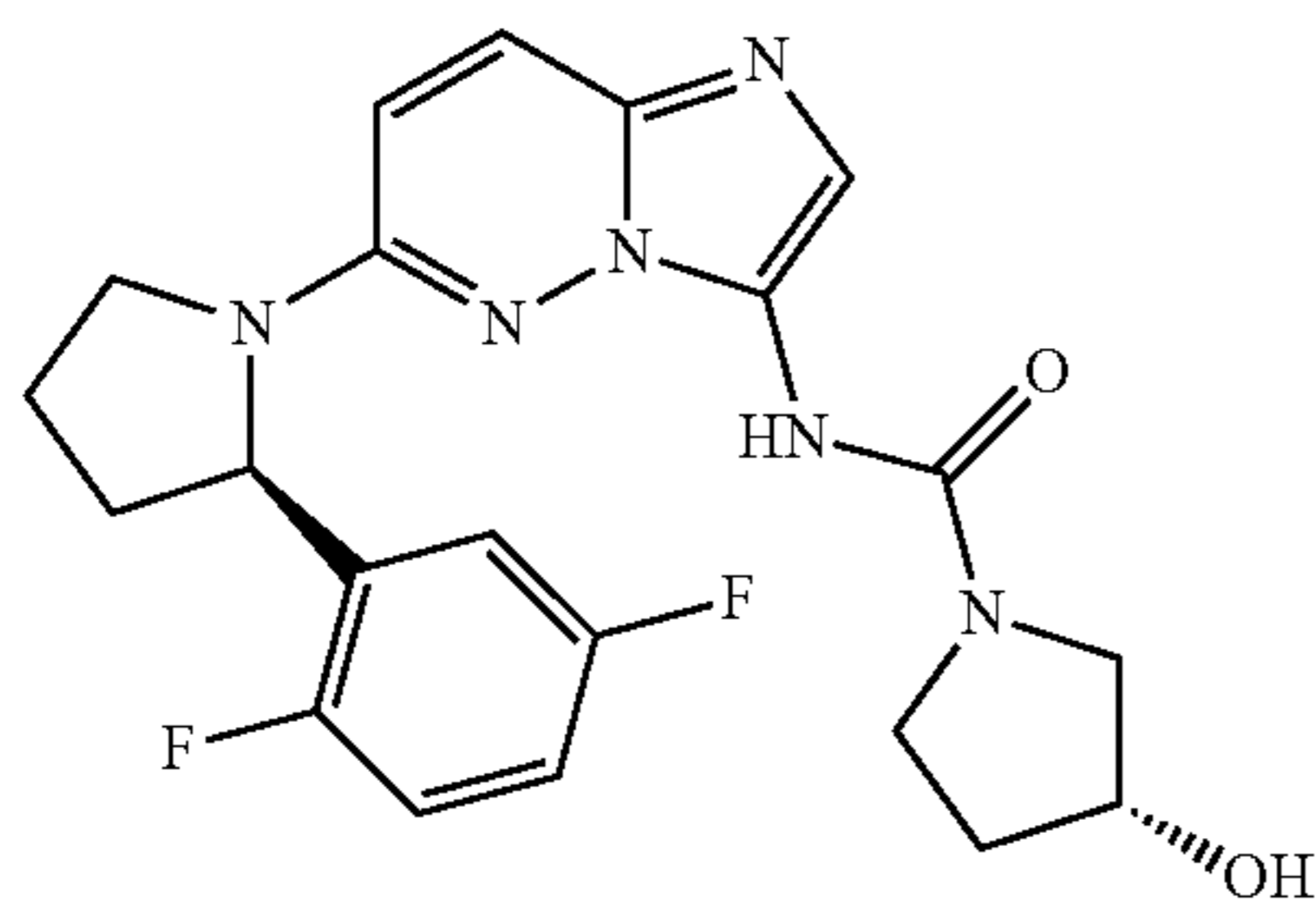
(R)—N-(6-((R)-2-(2,5-difluorophenyl)pyrrolidin-1-yl)imidazo[1,2-b]pyridazin-3-yl)-3-hydroxypyrrolidine-1-carboxamide
