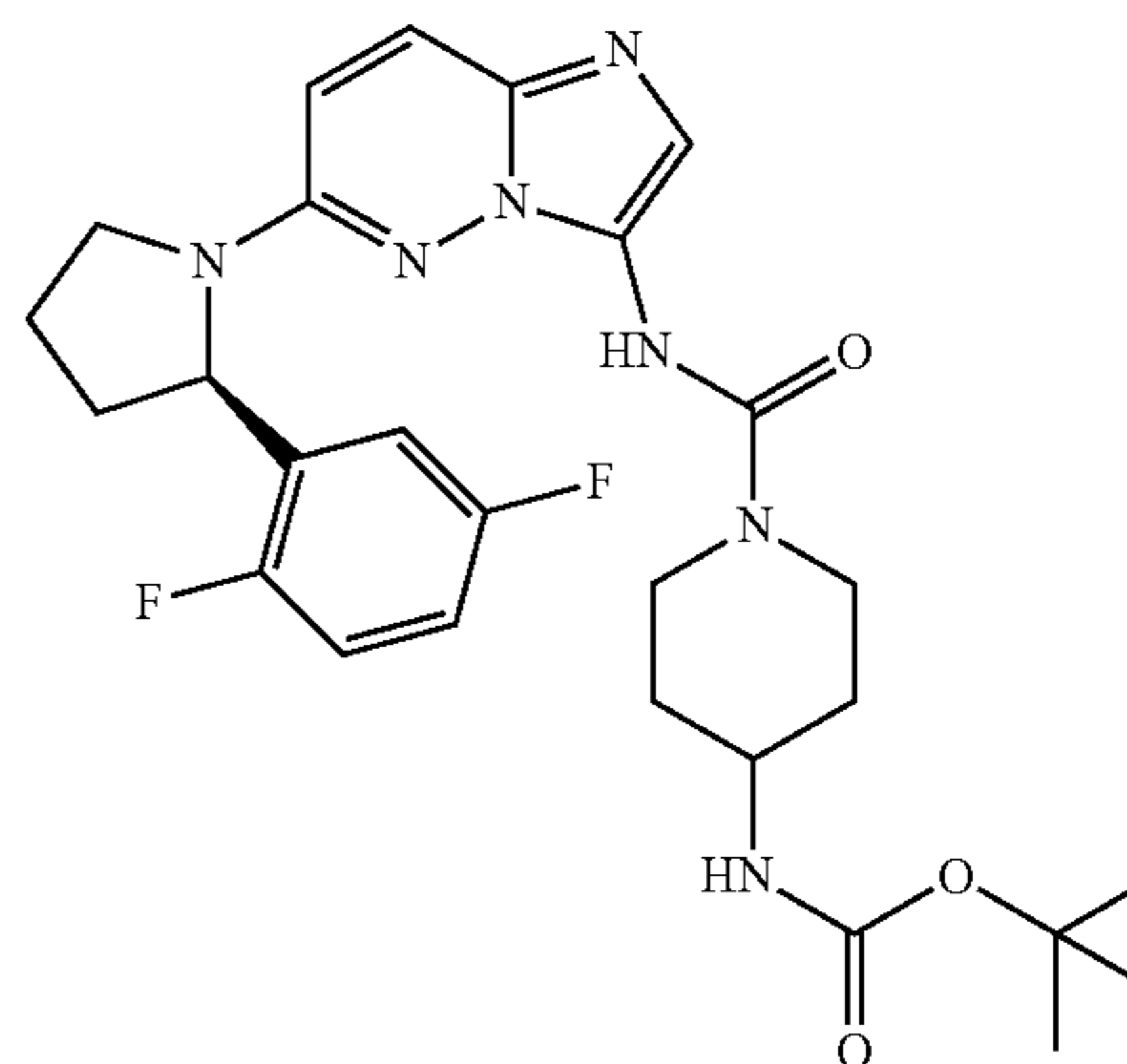
(R)-tert-butyl 1-(6-((R)-2-(2,5-difluorophenyl)pyrrolidin-1-yl)imidazo[1,2-b]pyridazin-3-yl)carbamoyl piperidin-4-ylcarbamate
