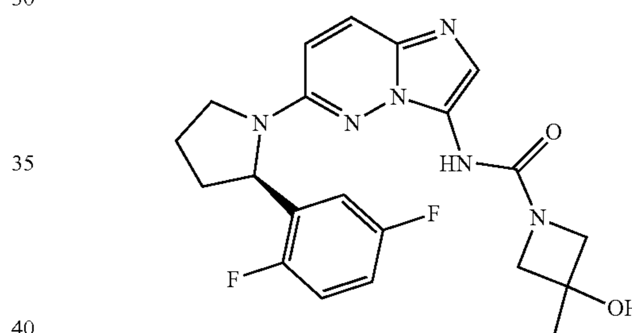
(R)—N-(6-(2-(2,5-difluorophenyl)pyrrolidin-1-yl) imidazo[1,2-b]pyridazin-3-yl)-3-hydroxy-3-methyl- azetidine-1-carboxamide
