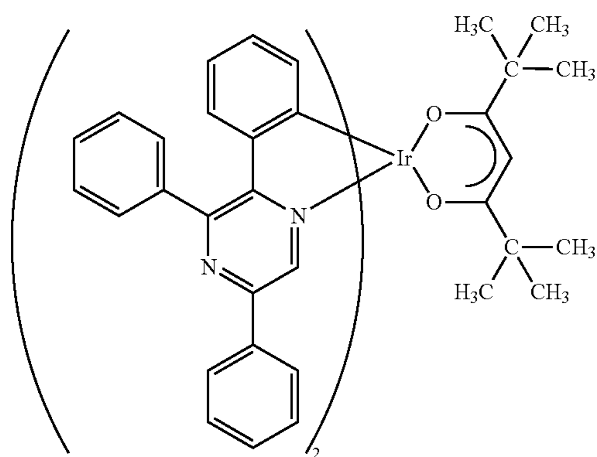
[Ir(tppr) 2 (dpm)]
