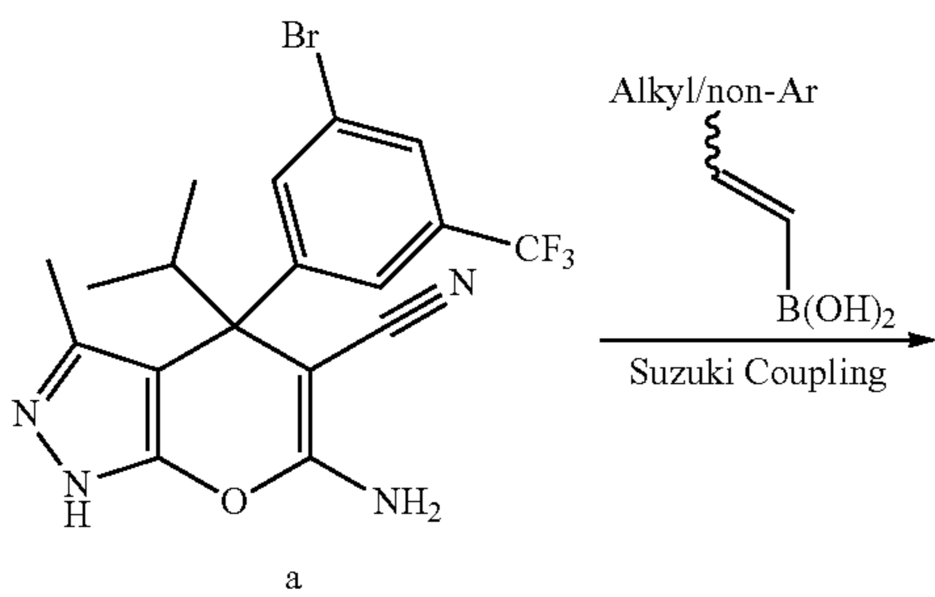
Scheme 2
