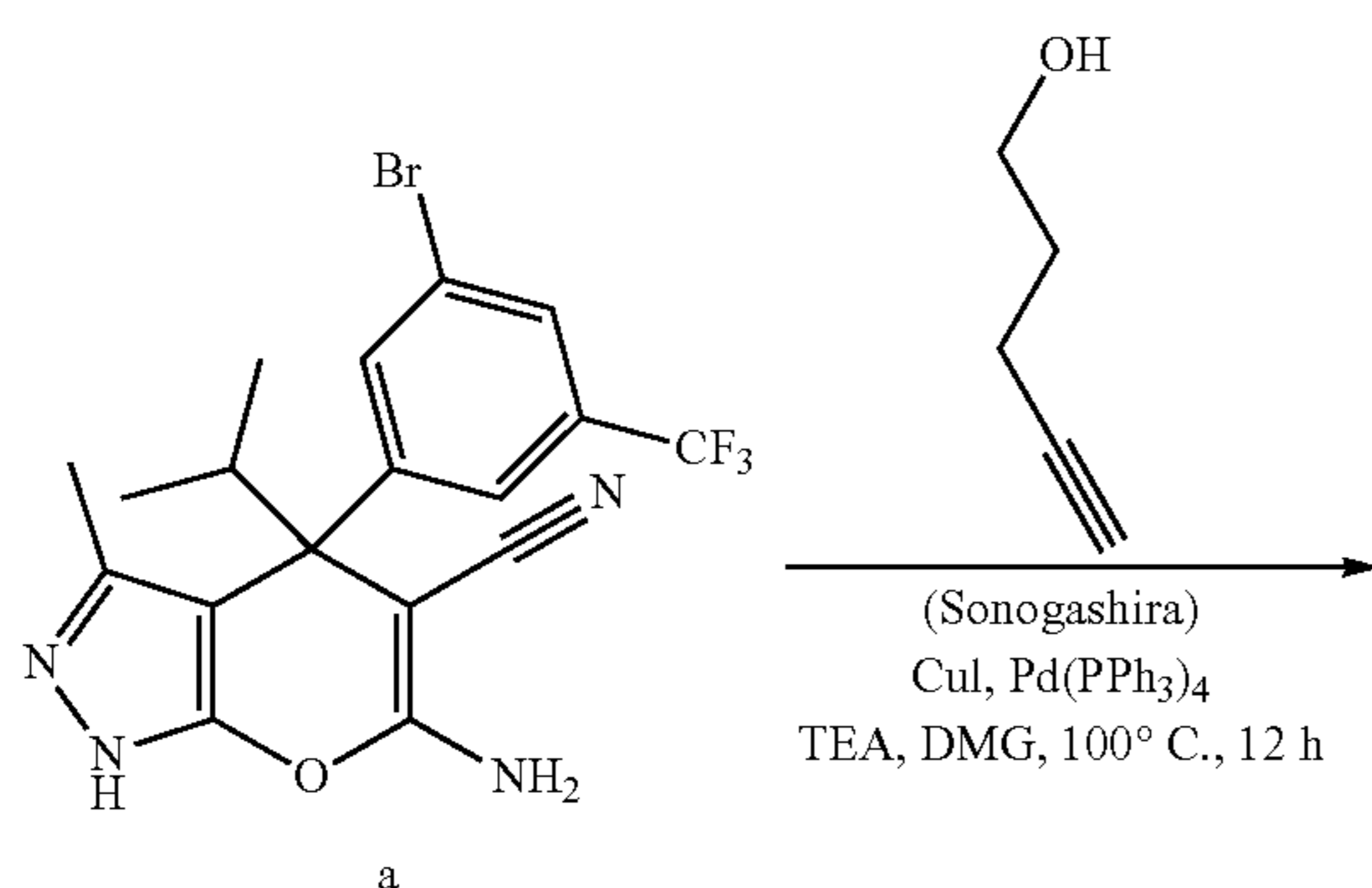
Scheme 5
