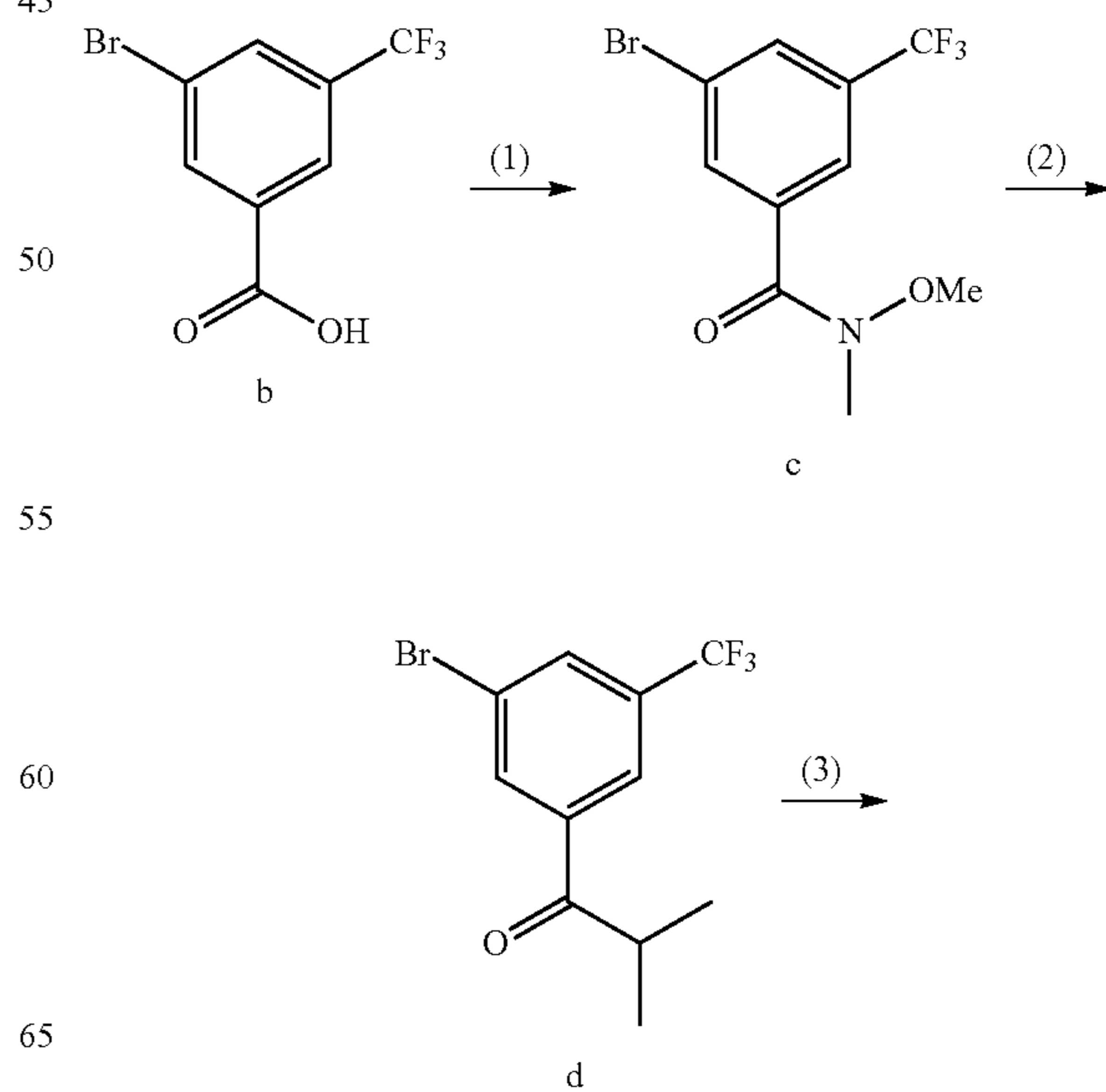
Scheme 4
