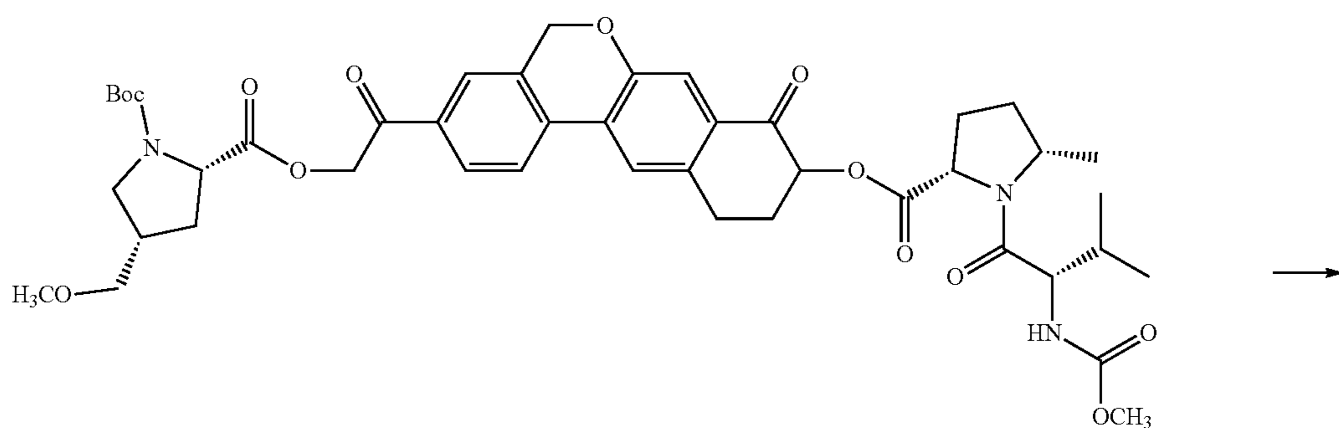
Compound (B-a)
