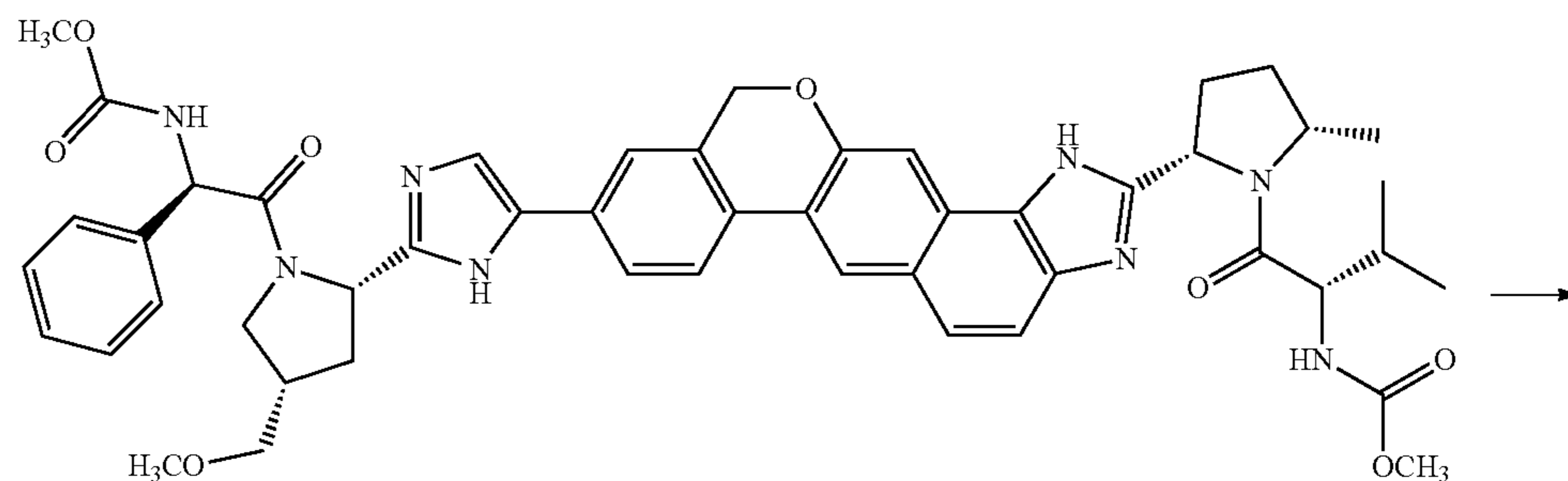
Compound (A)
