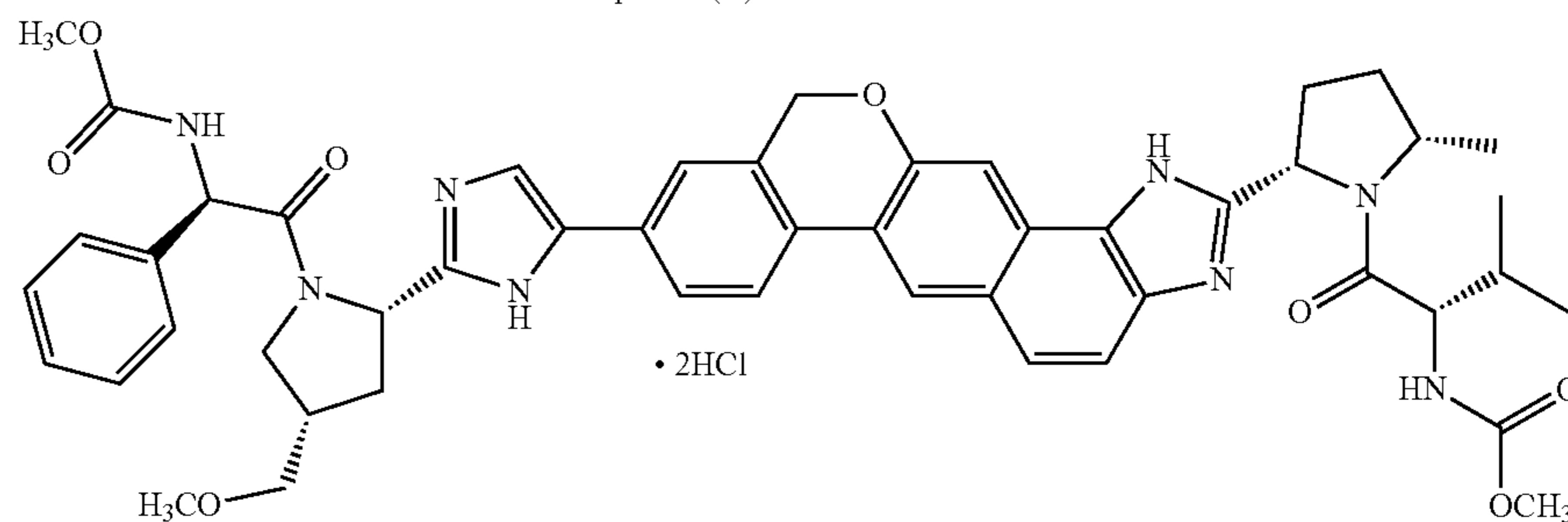
Compound (A-a)
