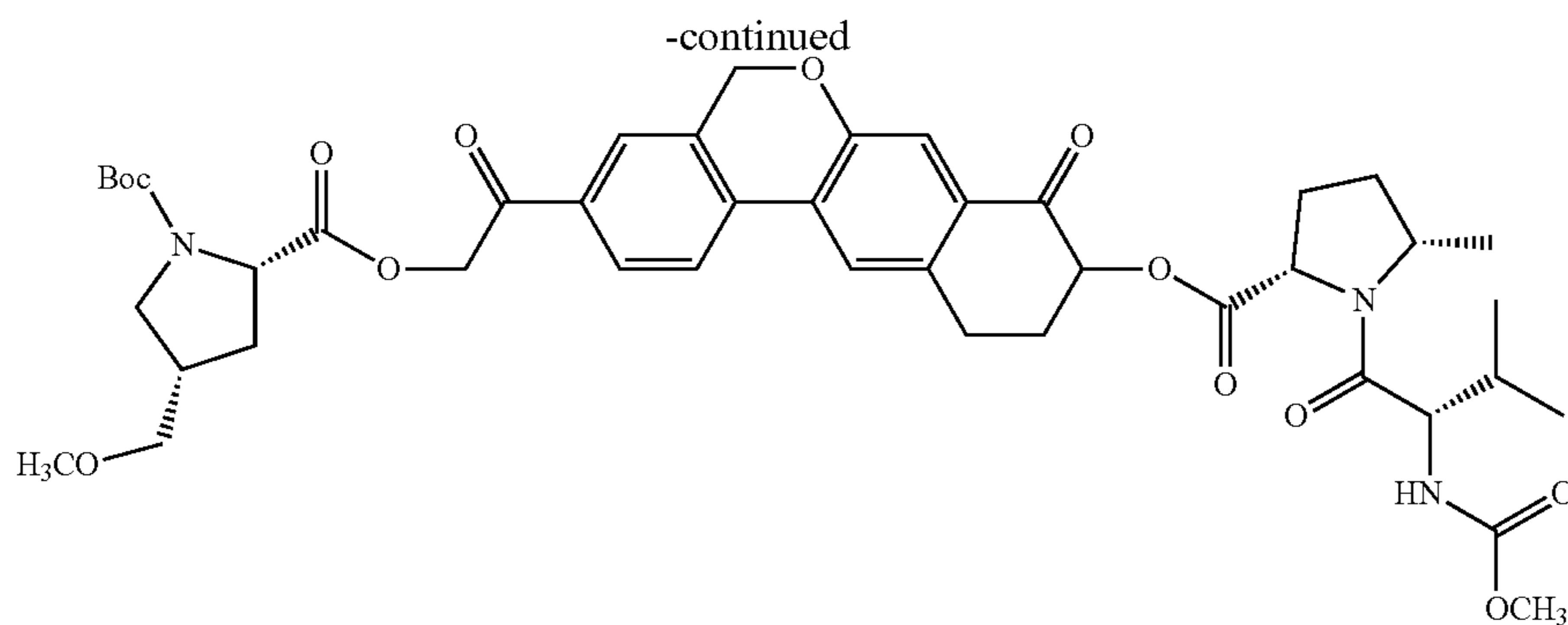
Compound (B-a)
