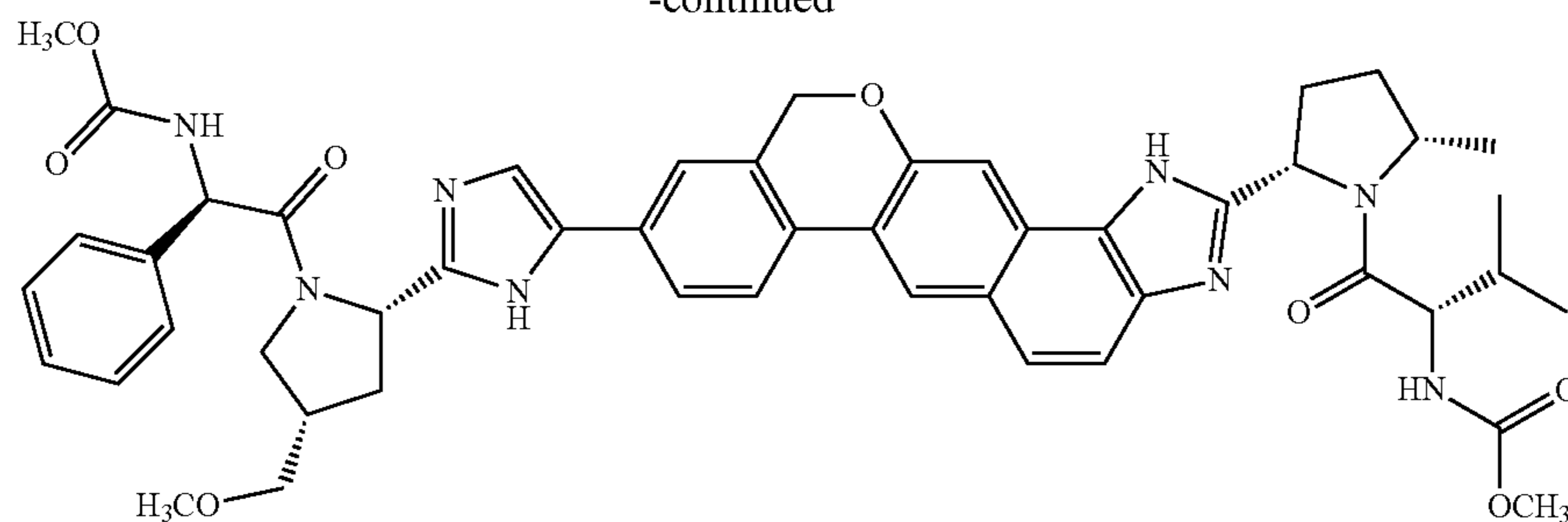
Compound (A)
