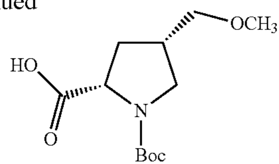
Compound (J-a)
