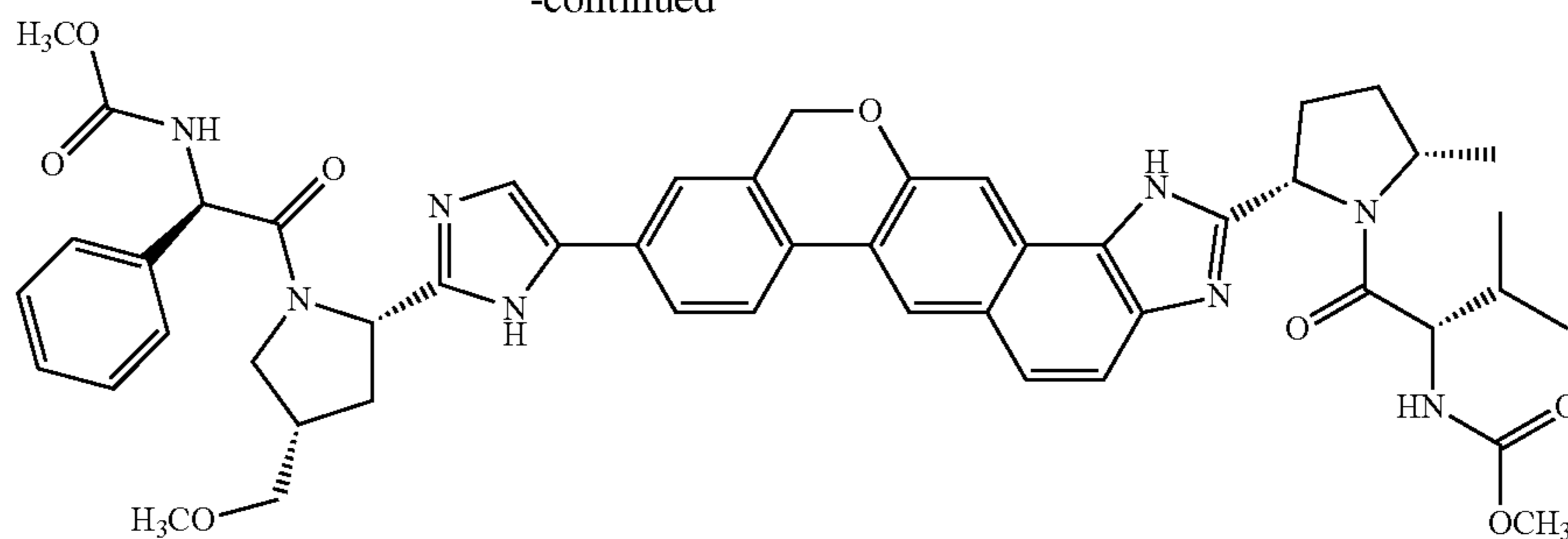
Compound (A)
