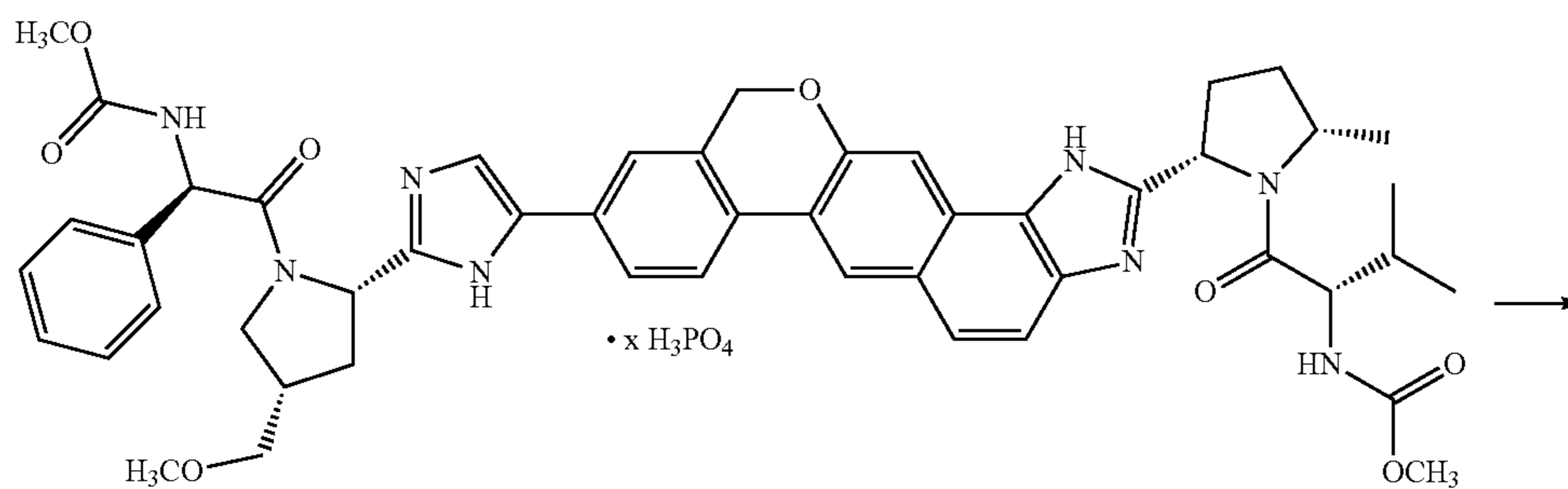
Compound (A-b)
