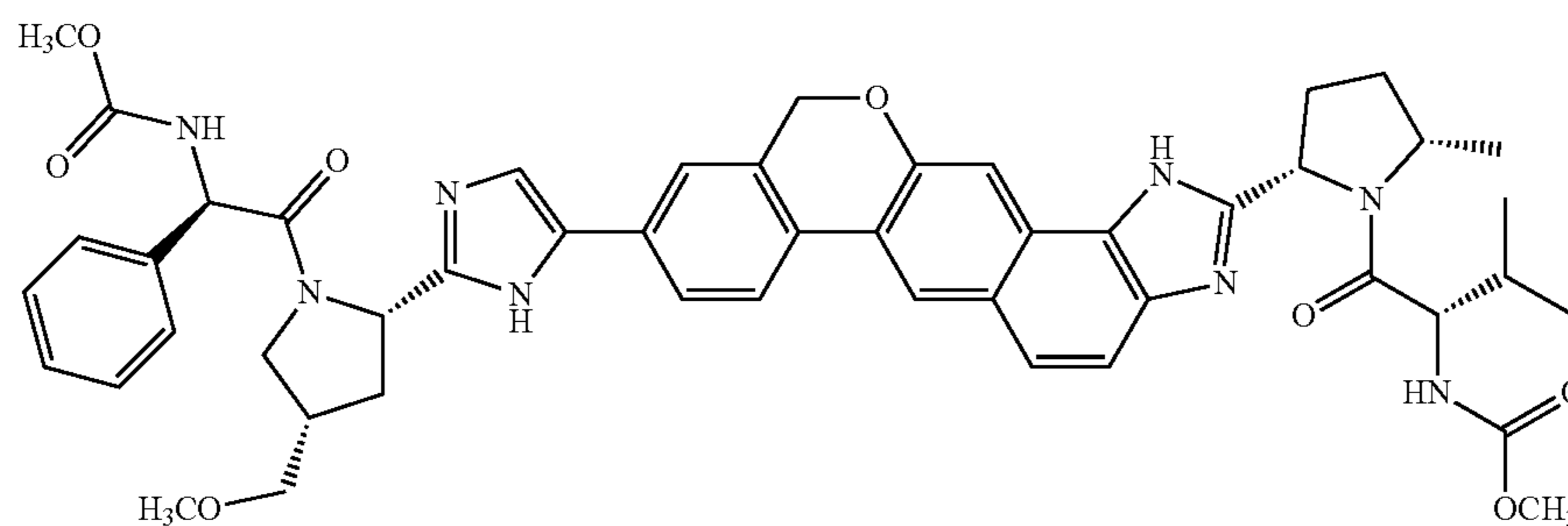
Compound (A)
