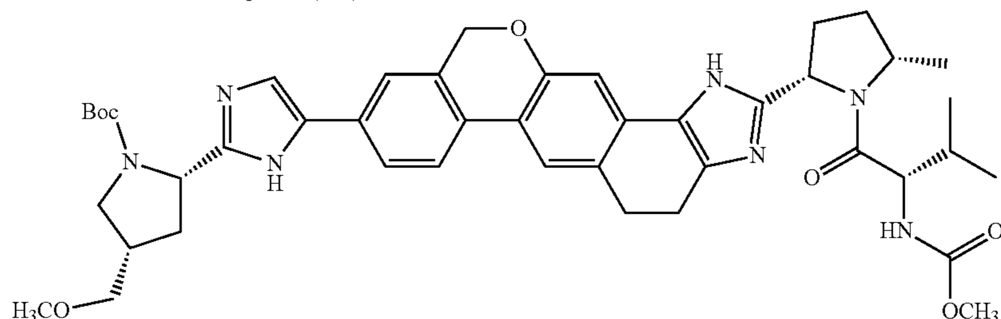
Compound (C-a)
