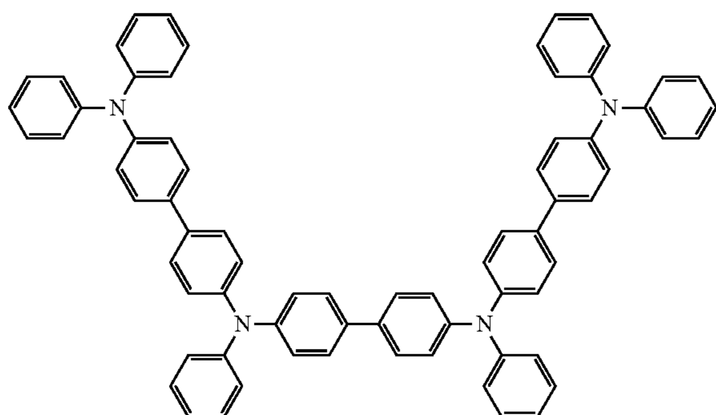
N^4,N^{4'} -([1,1'-biphenyl]-4,4'-diyl)bis( N^4,N^{4'} , N^{4''} -triphenyl-[1,1'-biphenyl]-4,4'-diamine)
