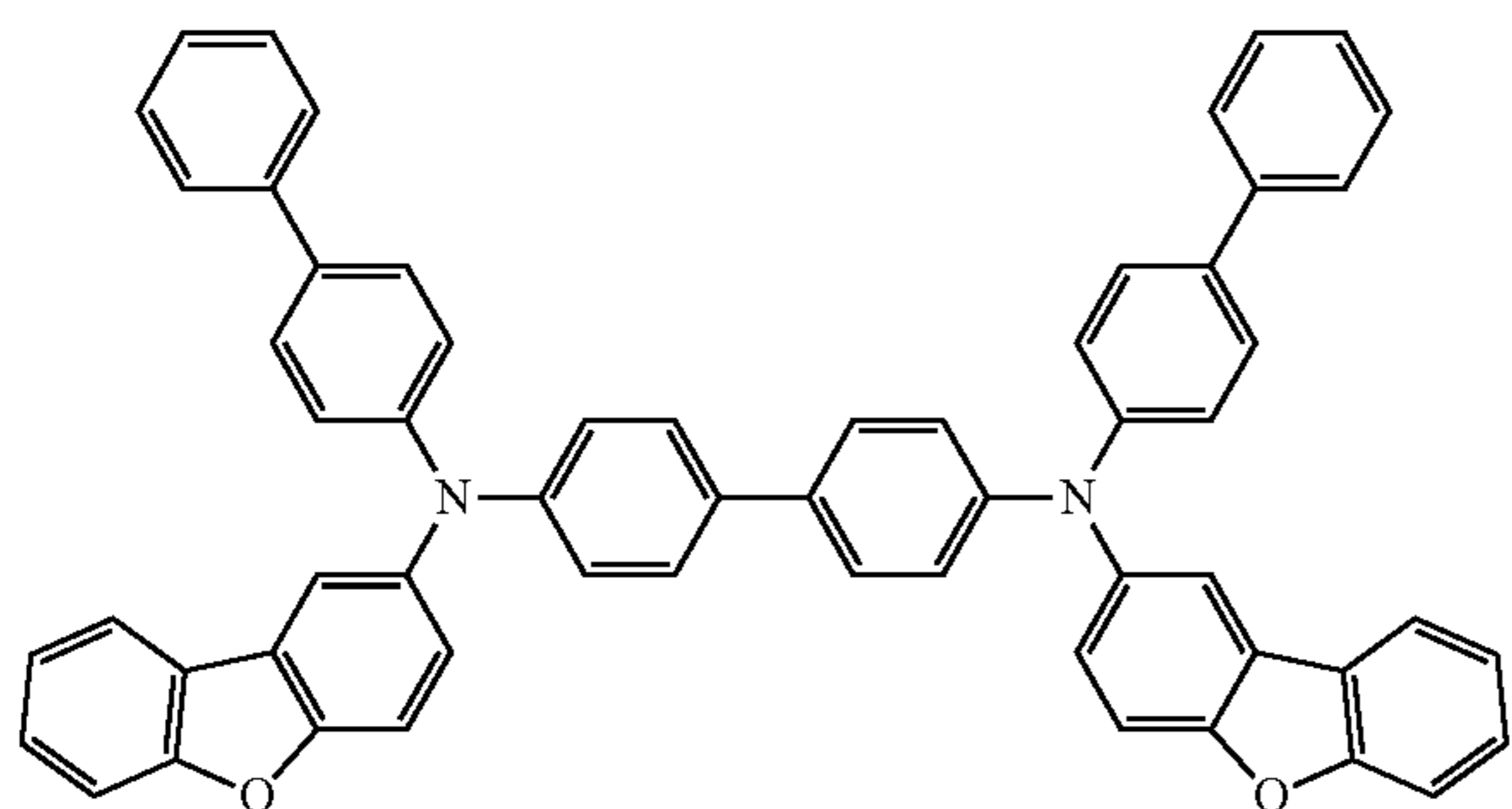
N^4,N^{4'} -di([1,1'-biphenyl]-4-yl)- N^4,N^{4'} -bis(dibenzo[b,d]furan-2-yl)-[1,1'-biphenyl]-4,4'-diamine
