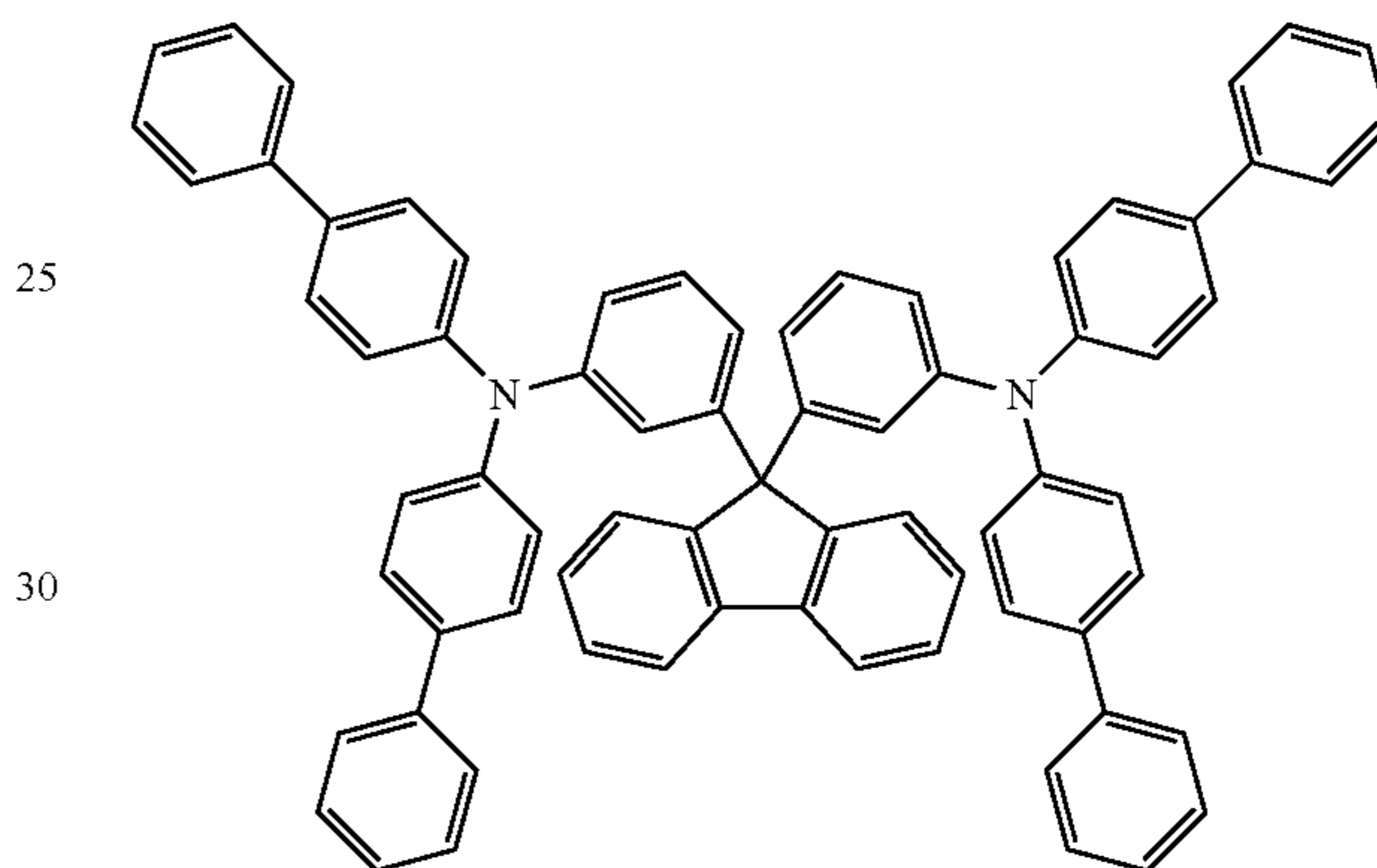
N,N'' -((9H-fluorene-9,9-diyl)bis(3,1-phenylene))bis( N -([1,1'-biphenyl]-4-yl)-[1,1'-biphenyl]-4-amine)
