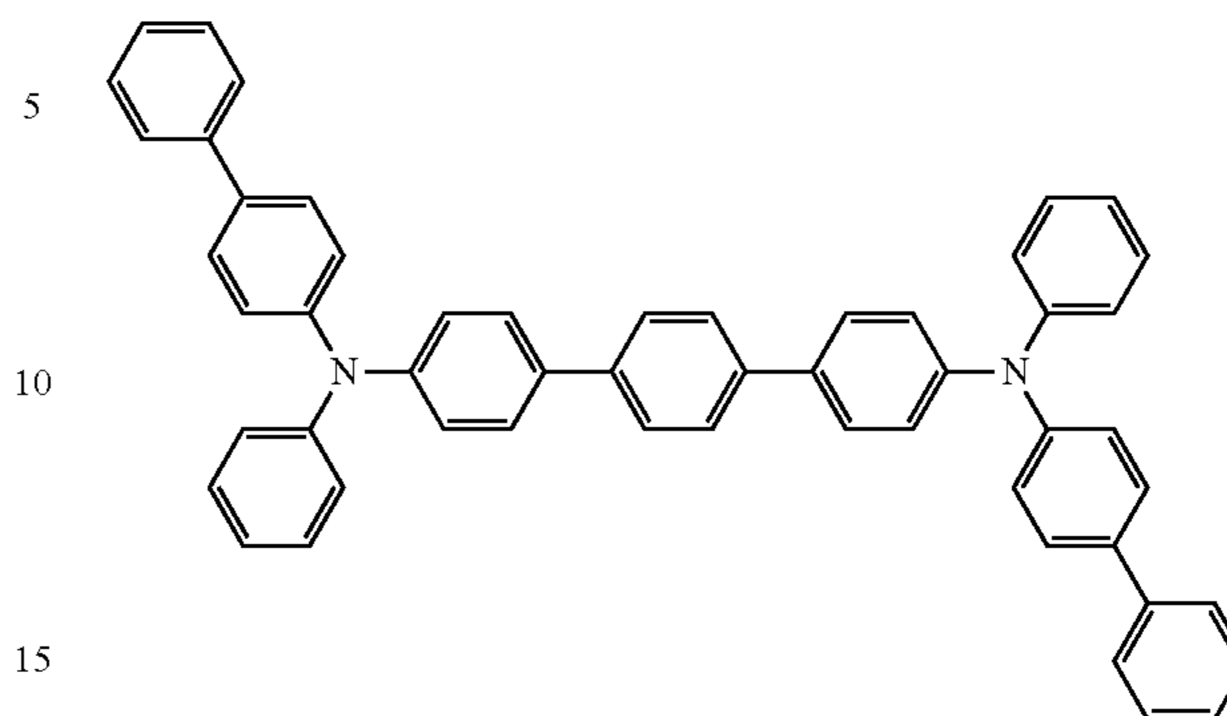
N^4,N^{4''} -di([1,1'-biphenyl]-4-yl)- N^4,N^{4''} -diphenyl-[1,1':4',1''-terphenyl]-4,4''-diamine
