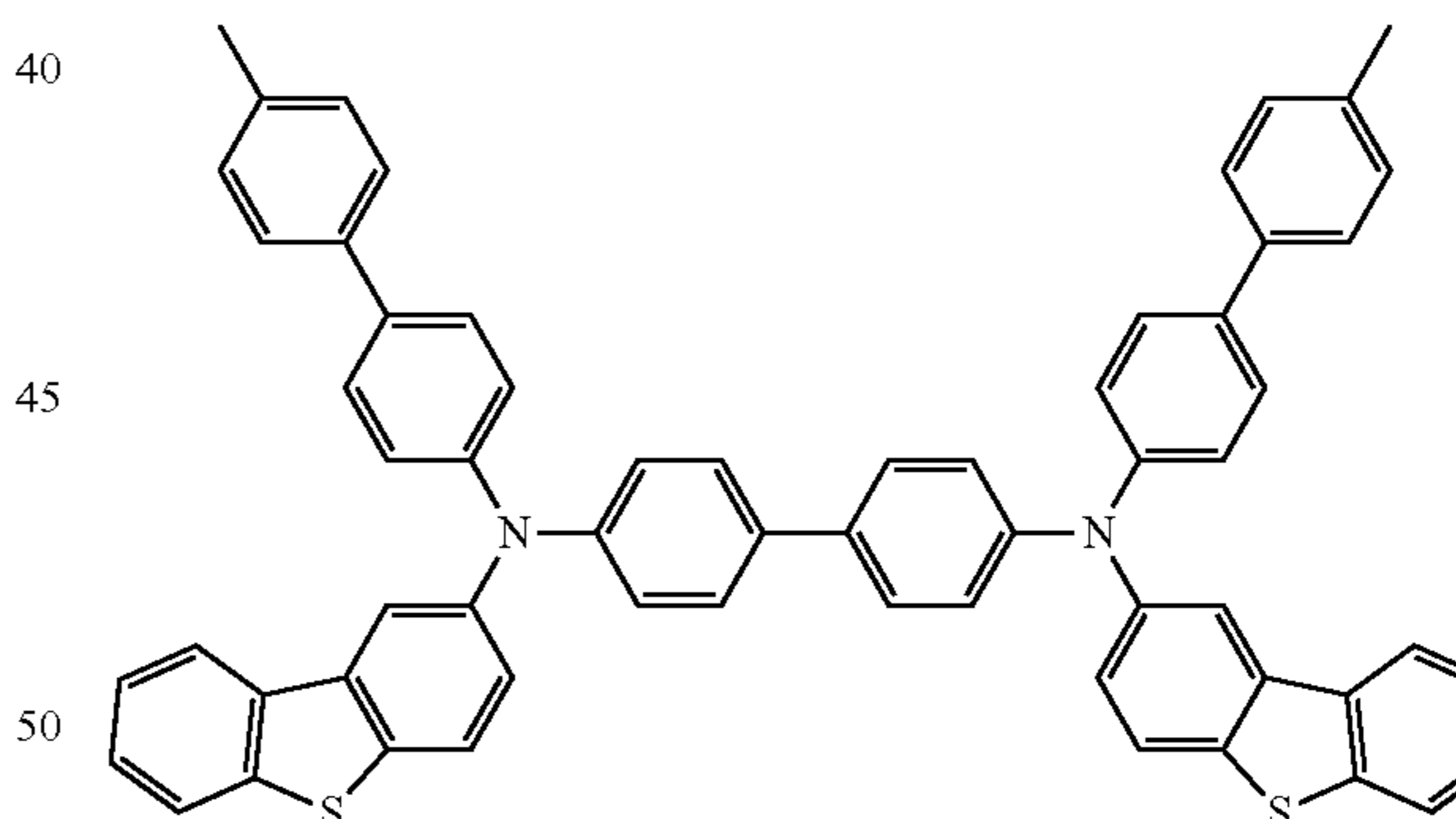
N^4,N^{4'} -bis(dibenzo[b,d]thiophen-2-yl)- N^4,N^{4'} -bis(4'-methyl-[1,1'-biphenyl]-4-yl)-[1,1'-biphenyl]-4,4'-diamine
