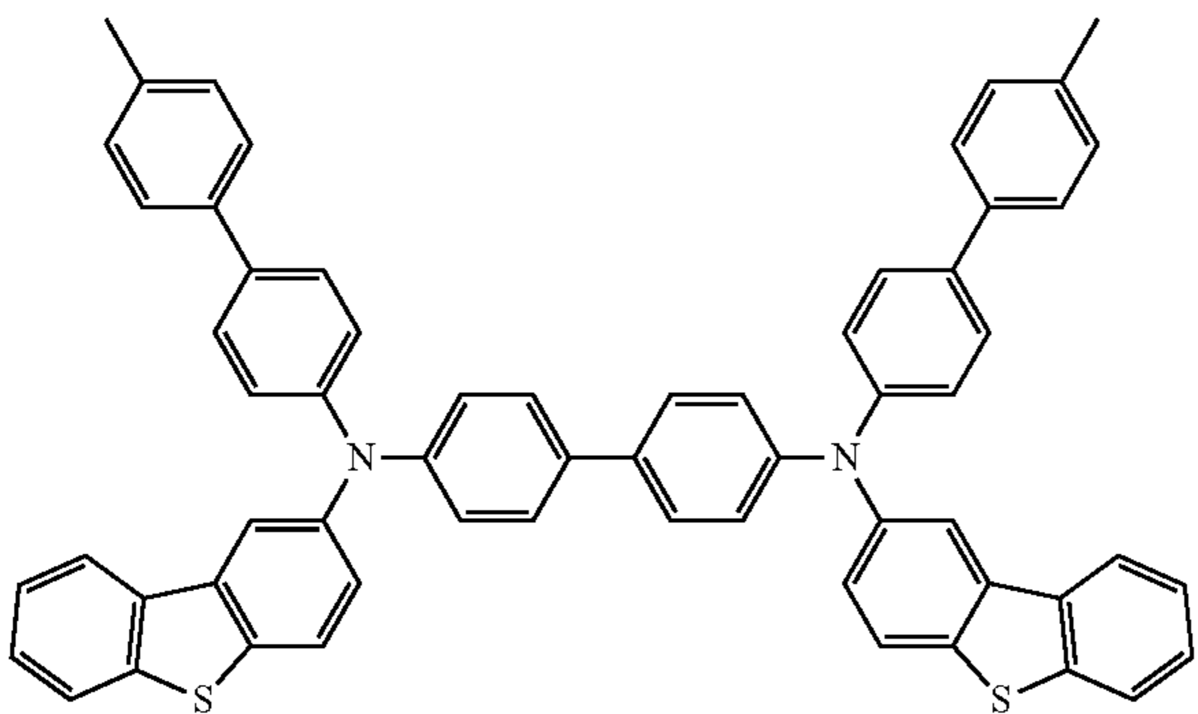
N,N'-(9H-fluorene-9,9-diyl)bis(3,1-phenylene)bis(N-([1,1'-biphenyl]-4-yl)-[1,1'-biphenyl]-4-amine)
