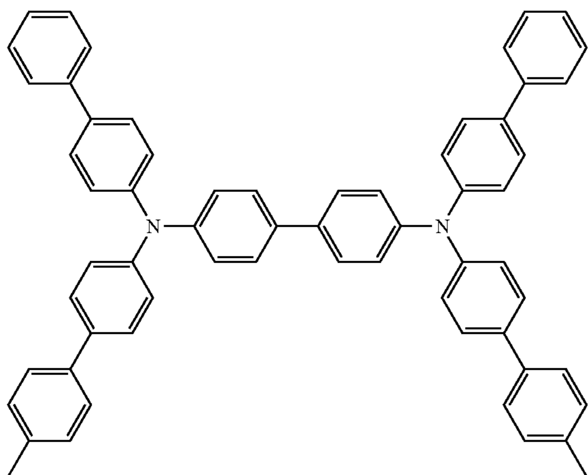
N^4,N^{4'} -di([1,1'-biphenyl]-4-yl)- N^4,N^{4'} -bis(4'-methyl-[1,1'-biphenyl]-4-yl)-[1,1'-biphenyl]-4,4'-diamine
