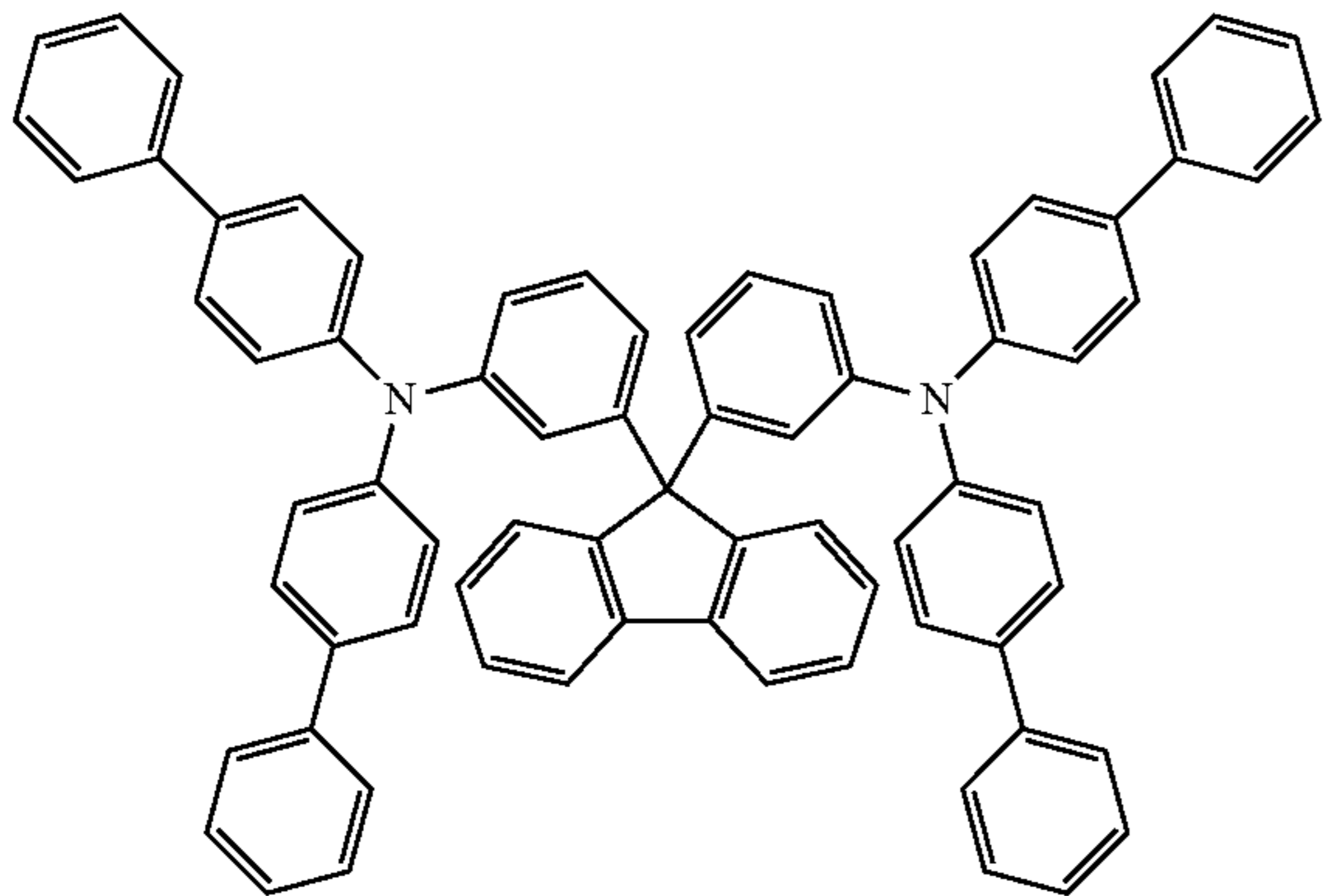
N,N'-(9H-fluorene-9,9-diyl)bis(3,1-phenylene)bis(N-([1,1'-biphenyl]-4-yl)-[1,1'-biphenyl]-4-amine)
