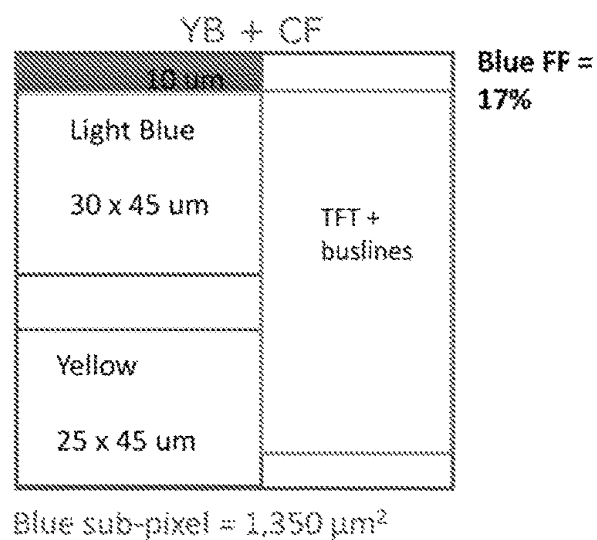
YB two-deposition
