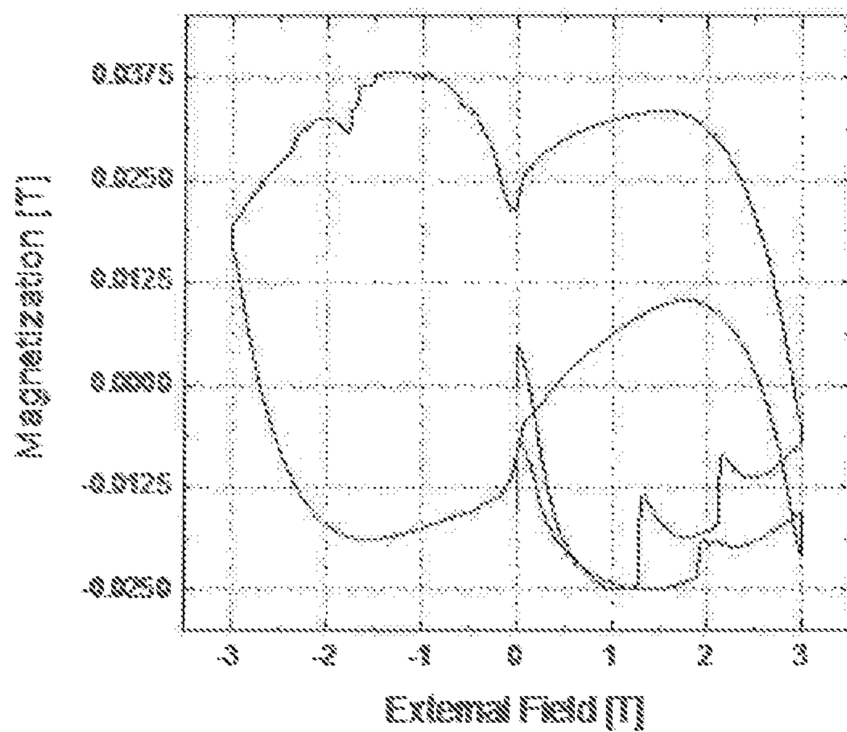
FIG. 6 (PRIOR ART)
