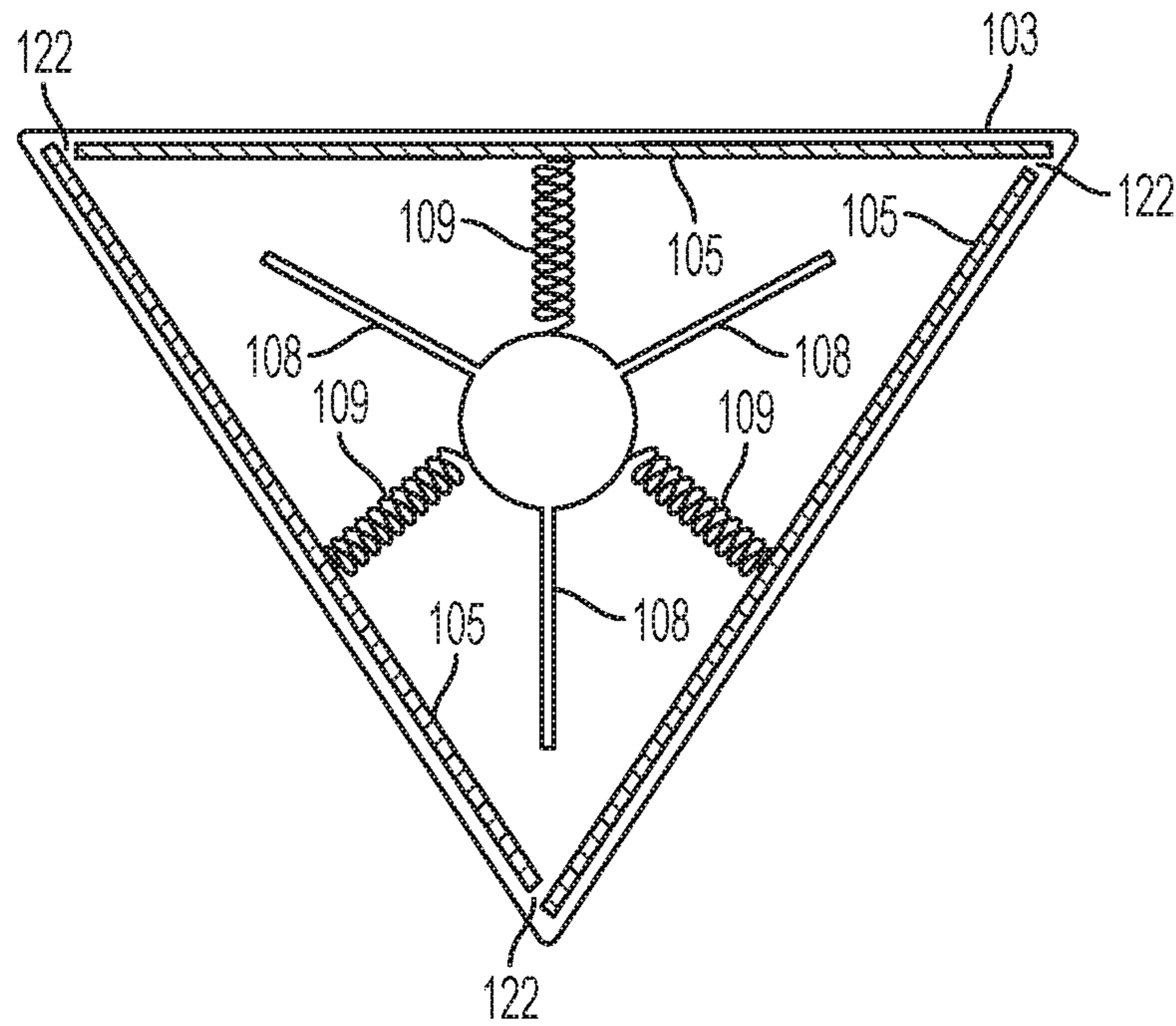
SECTION C-C
