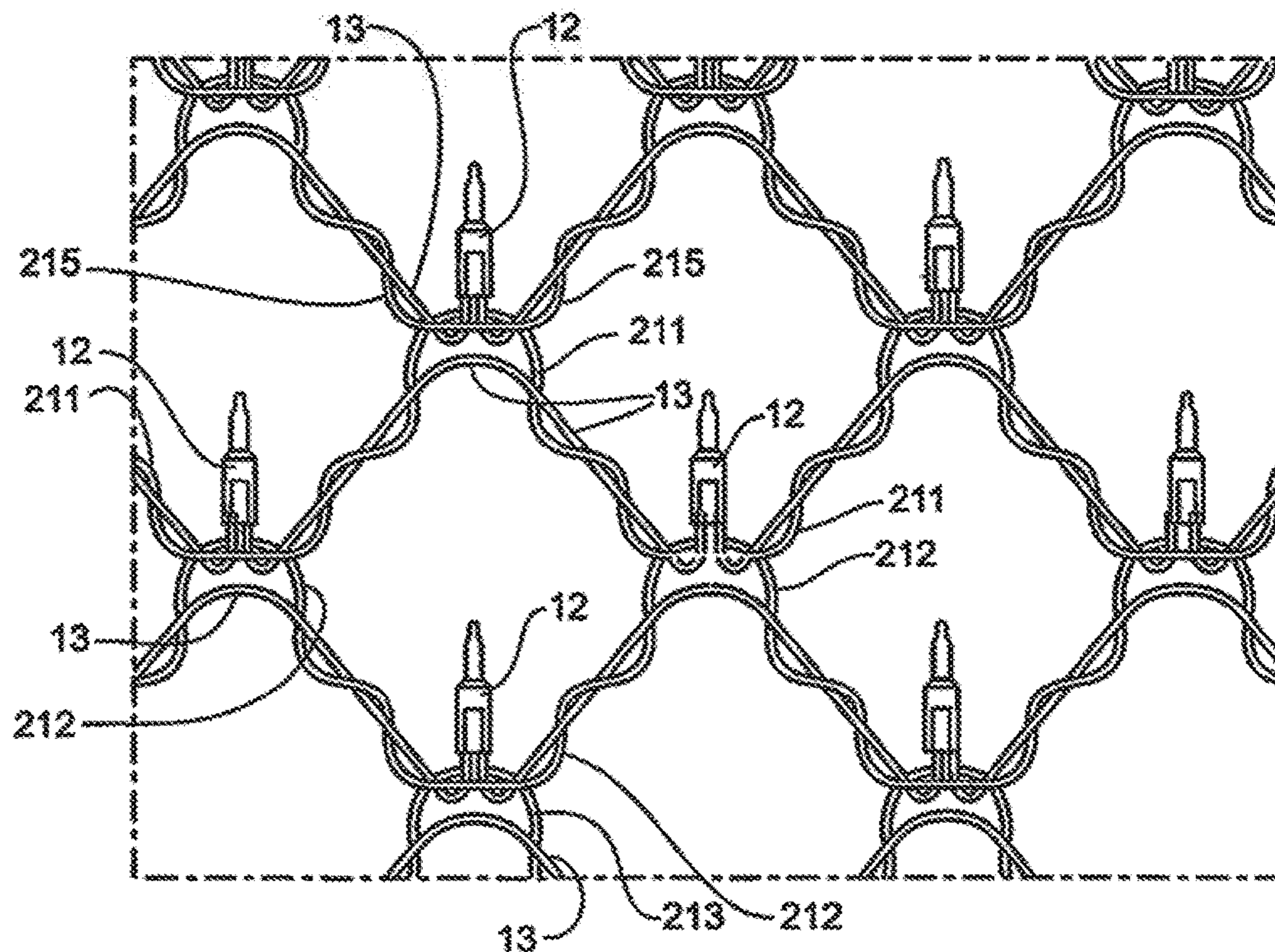
Fig. 2 Prior Art
