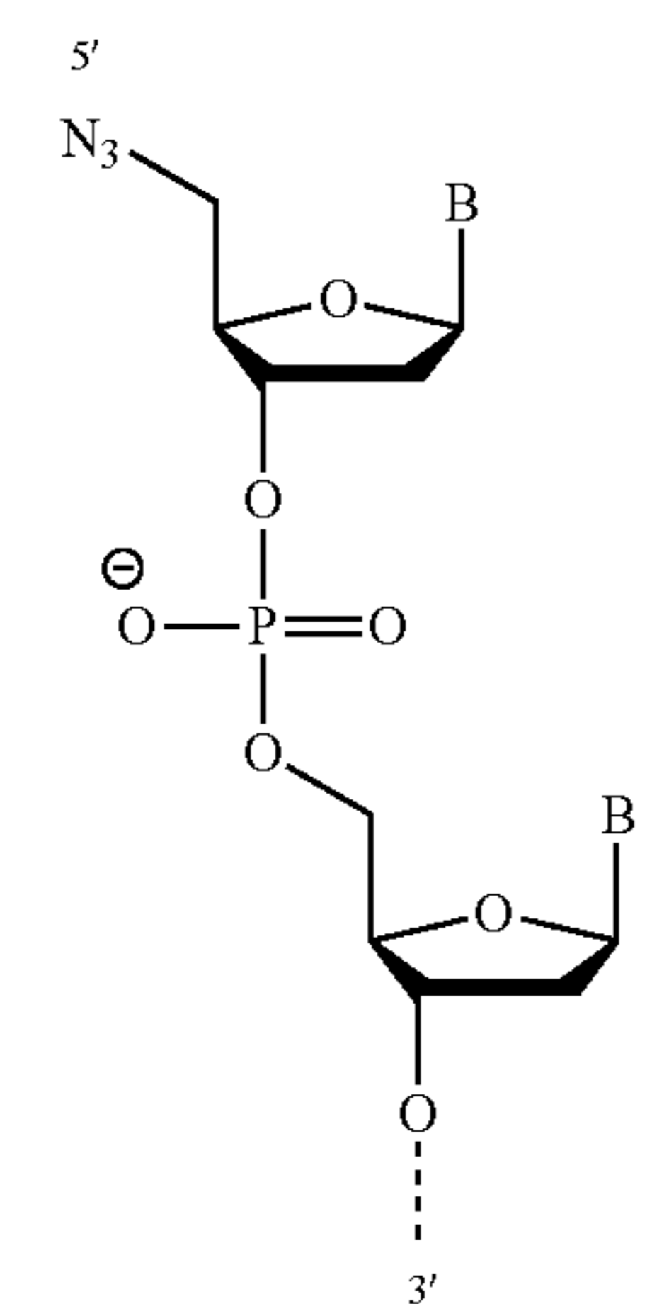
5'-azido-methyl modification
