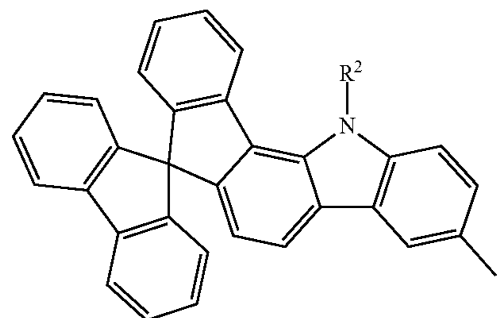
Formula (Ar-8-5-1a)
