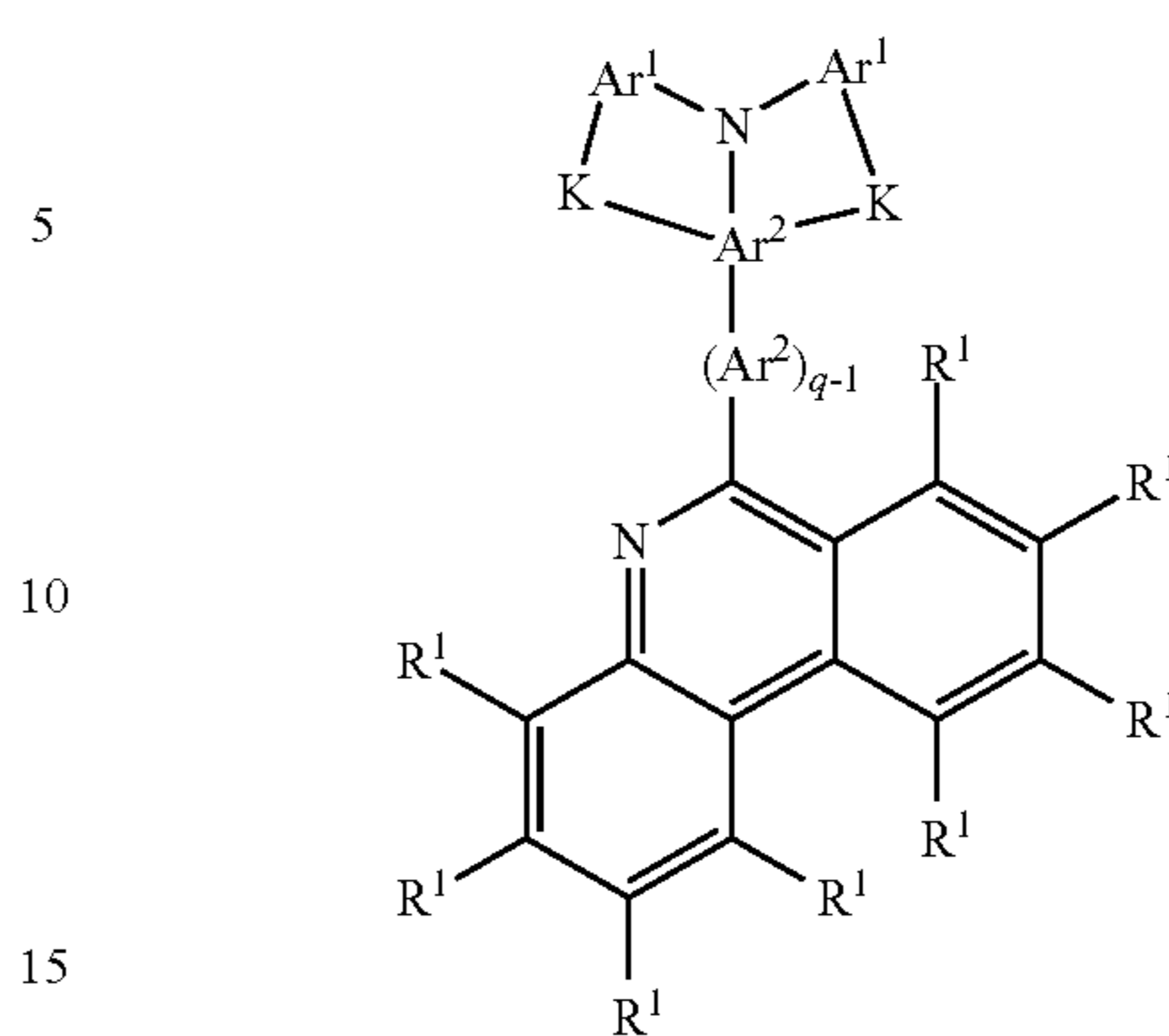
Formula (3)
