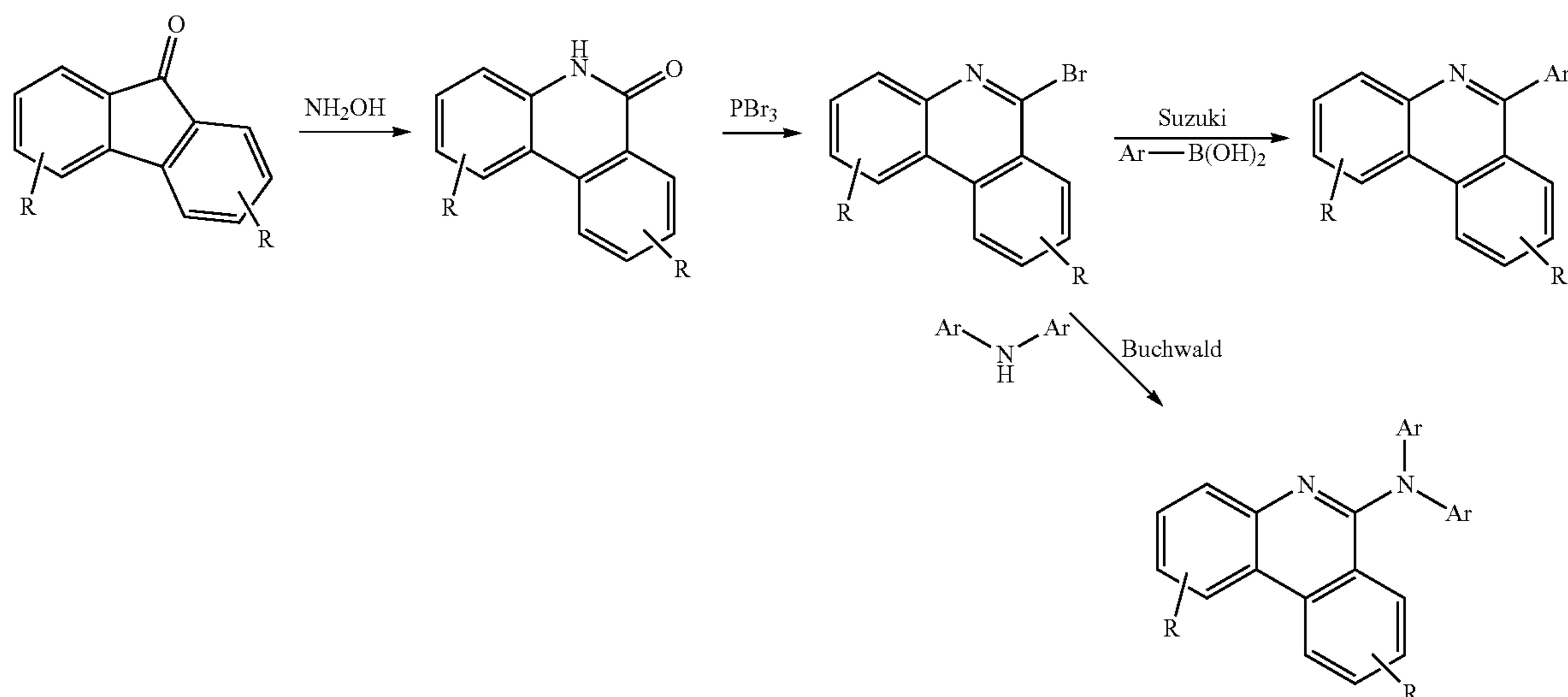
Scheme 1:
