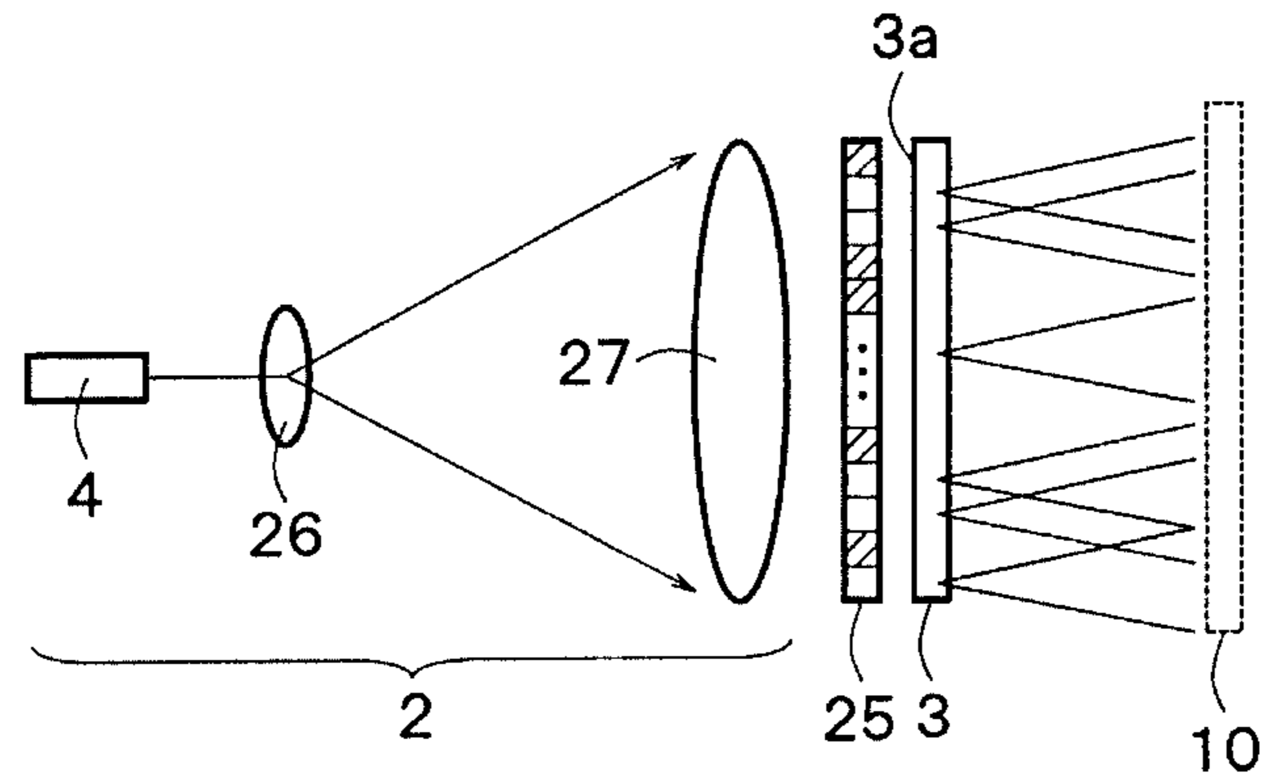
1 : ILLUMINATION DEVICE
