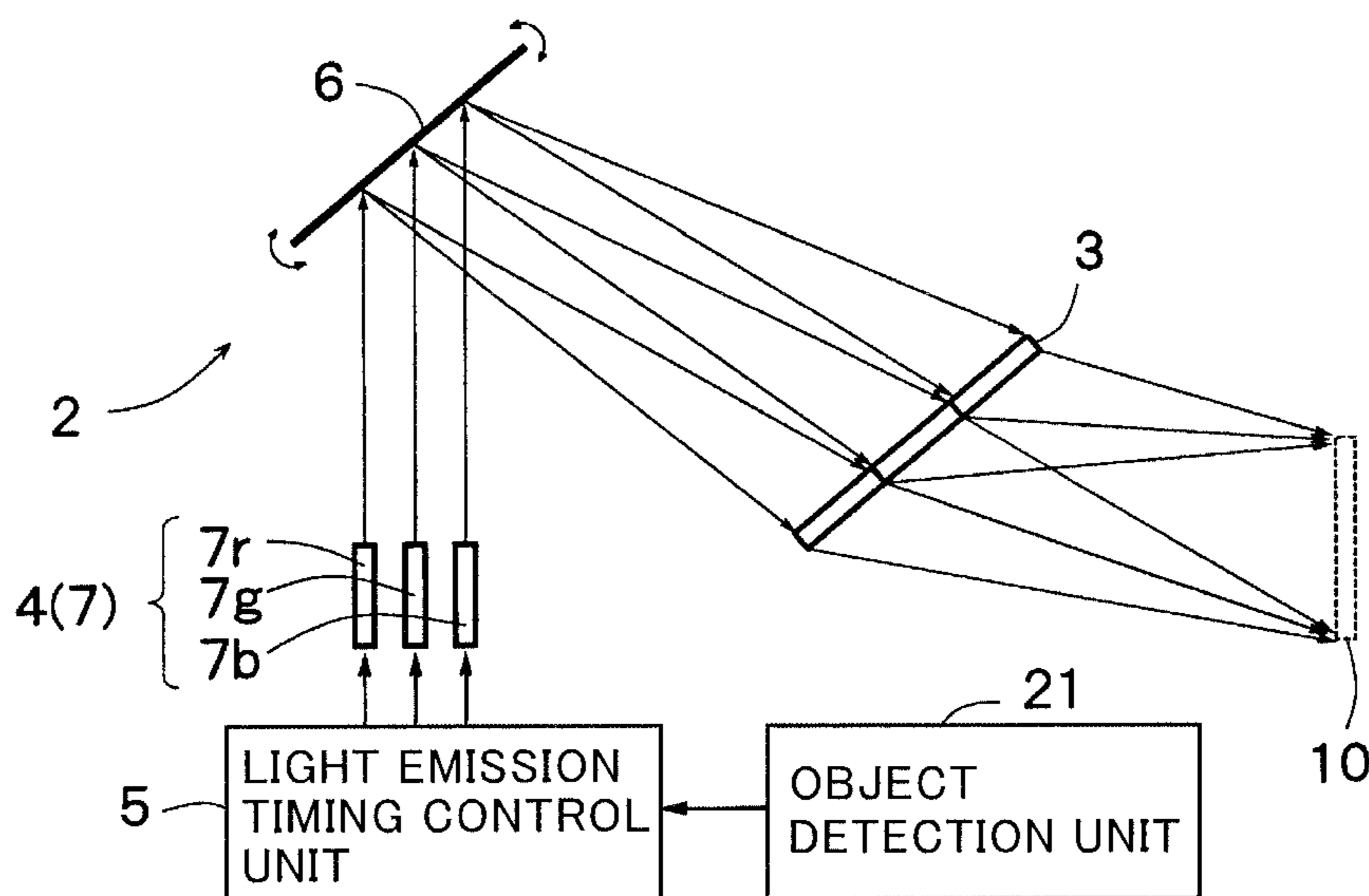
1 . ILLUMINATION DEVICE
