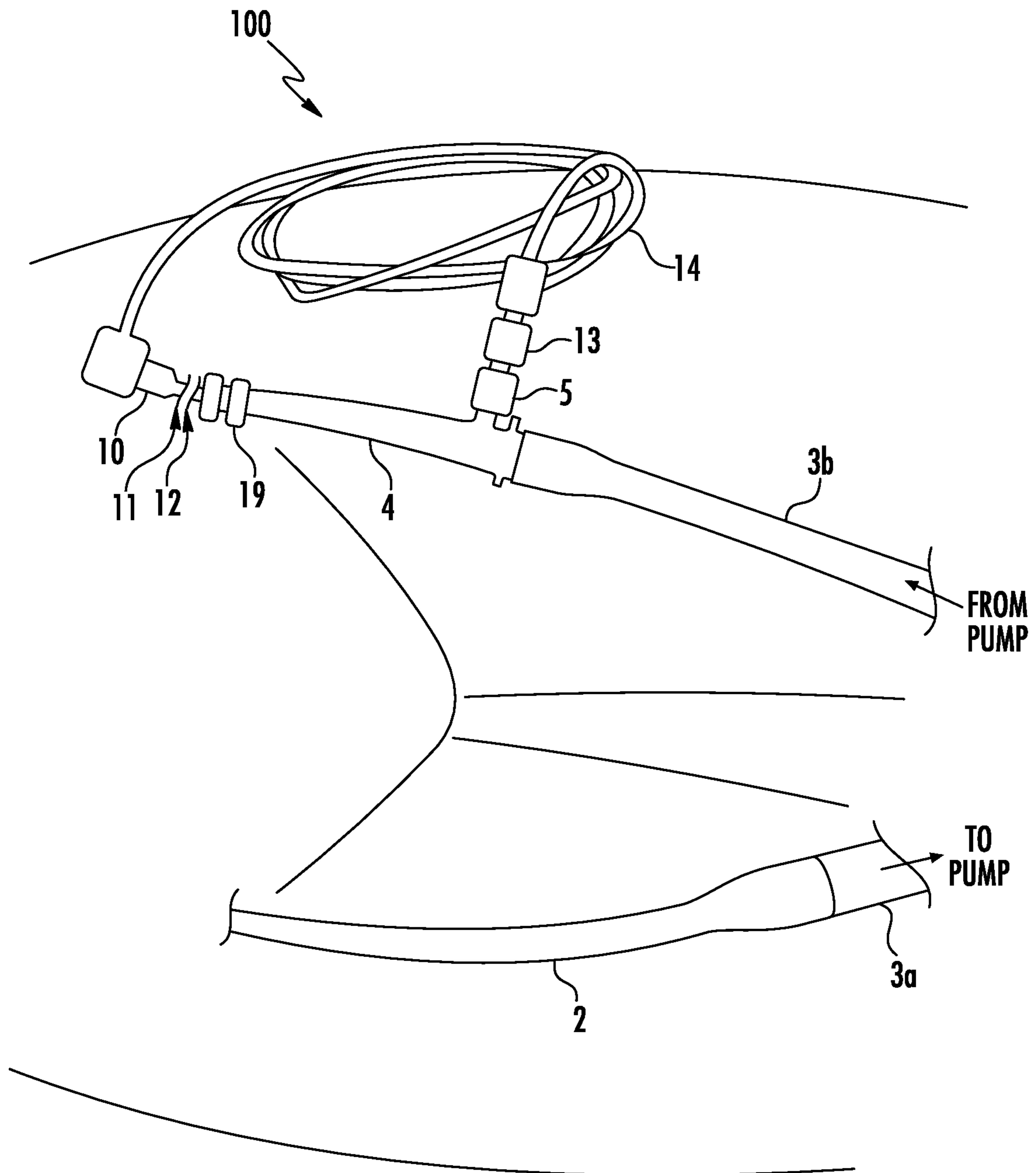
FIG. 1 (PRIOR ART)
