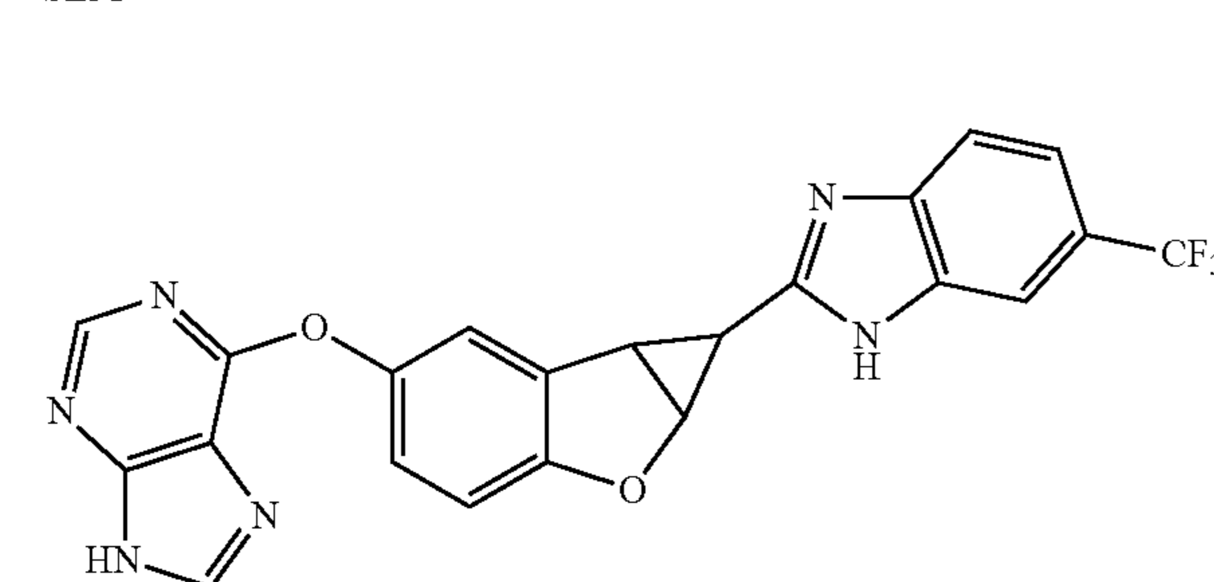
Compound 3.5
