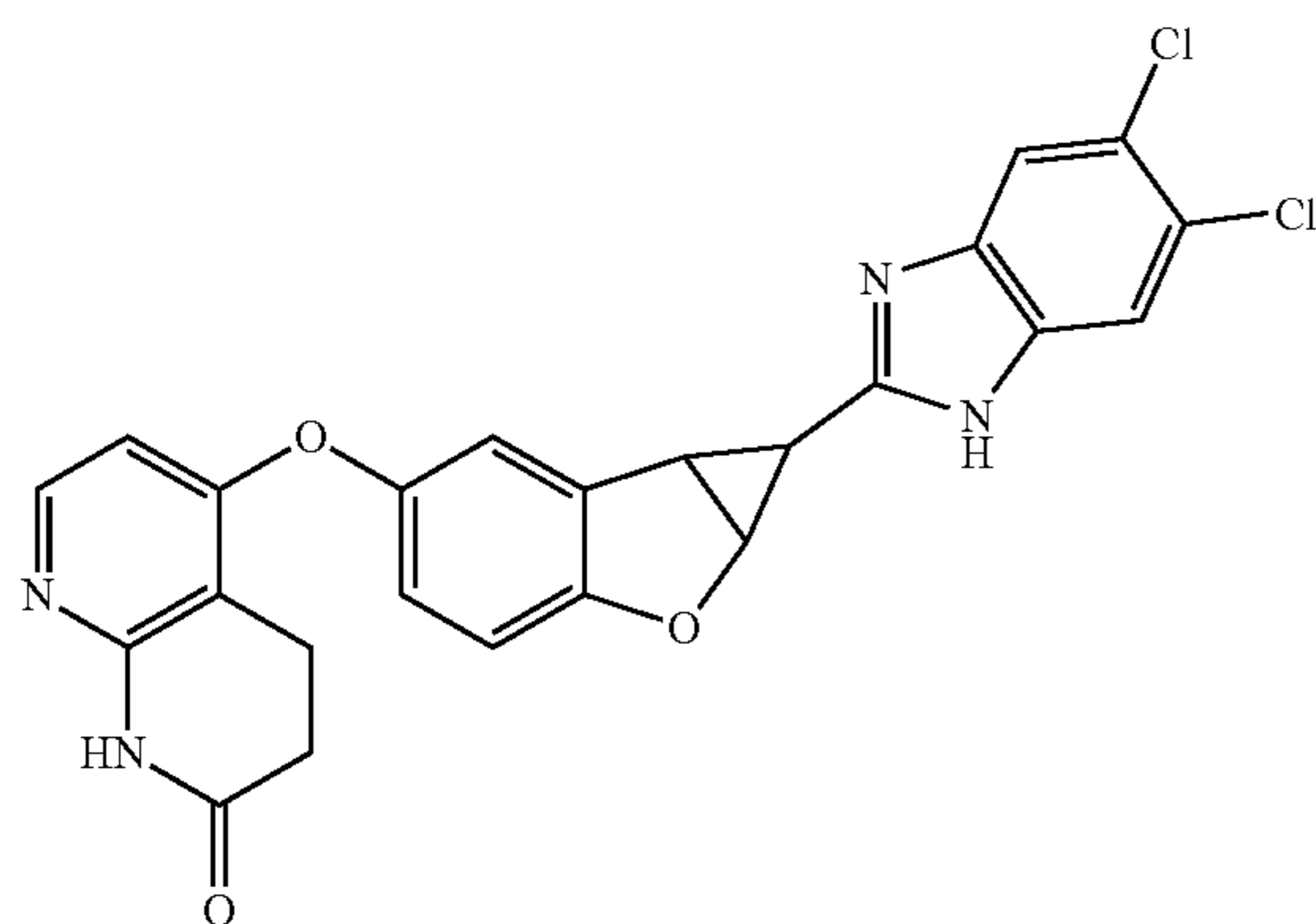
Compound 2.3
