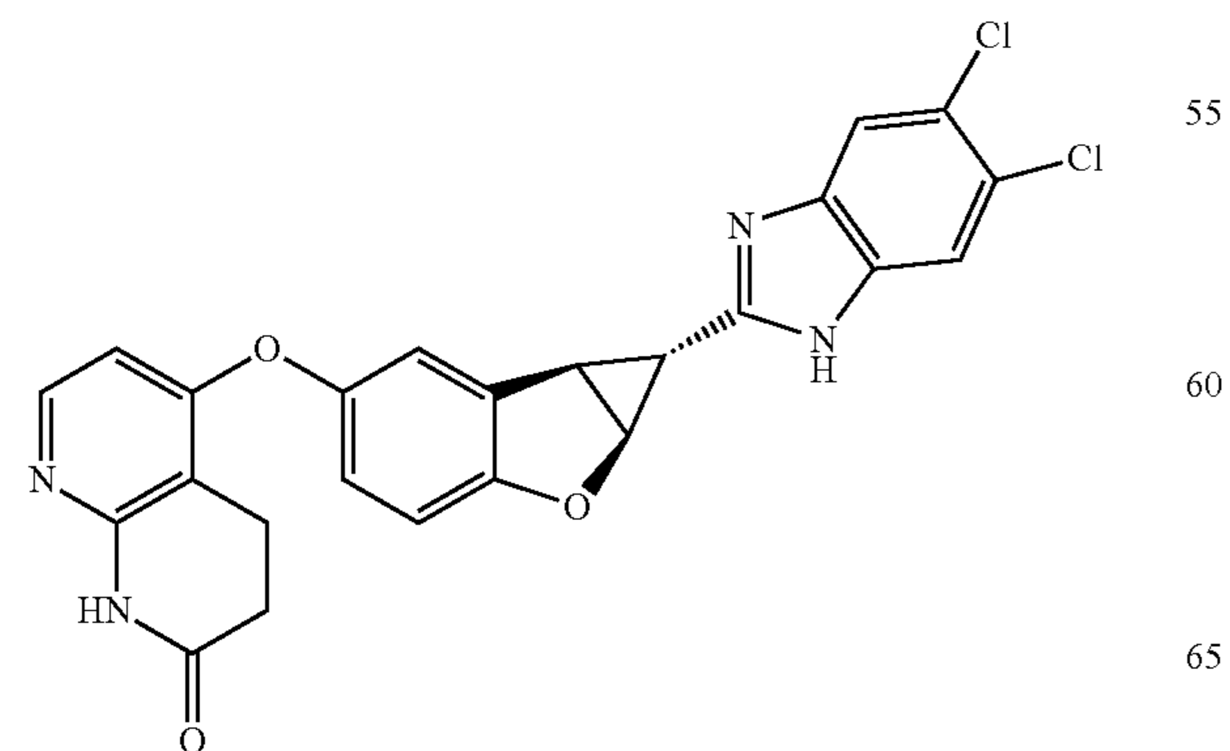
Compound 2.3a
