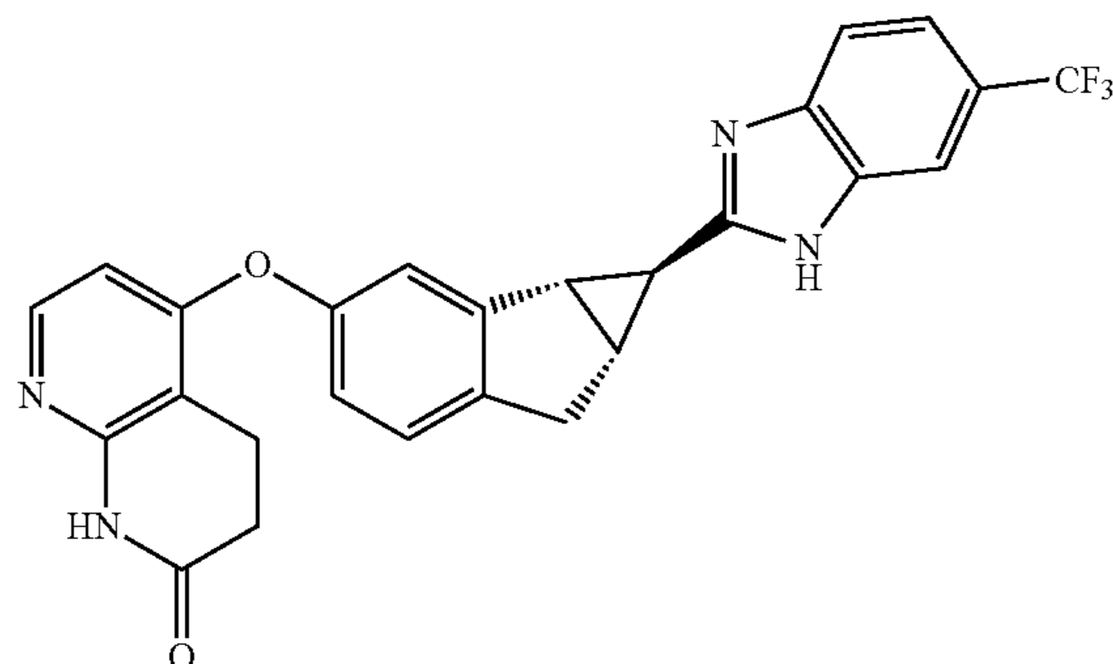
Compound 1.2b
