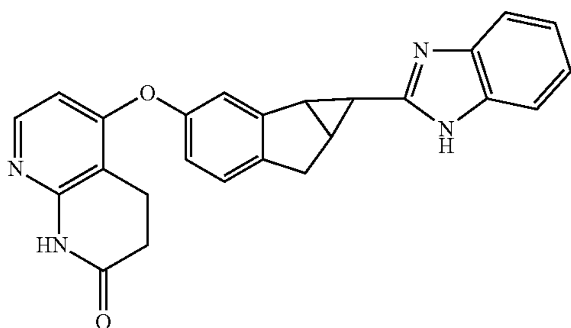
Compound 1.1
