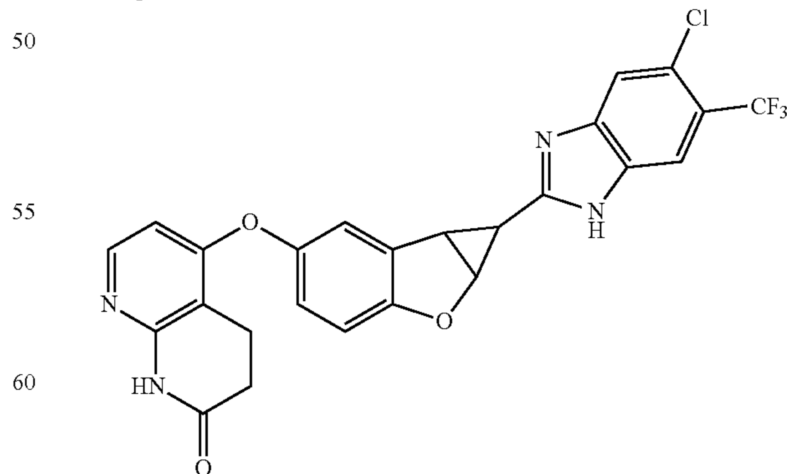
Compound 2.5
