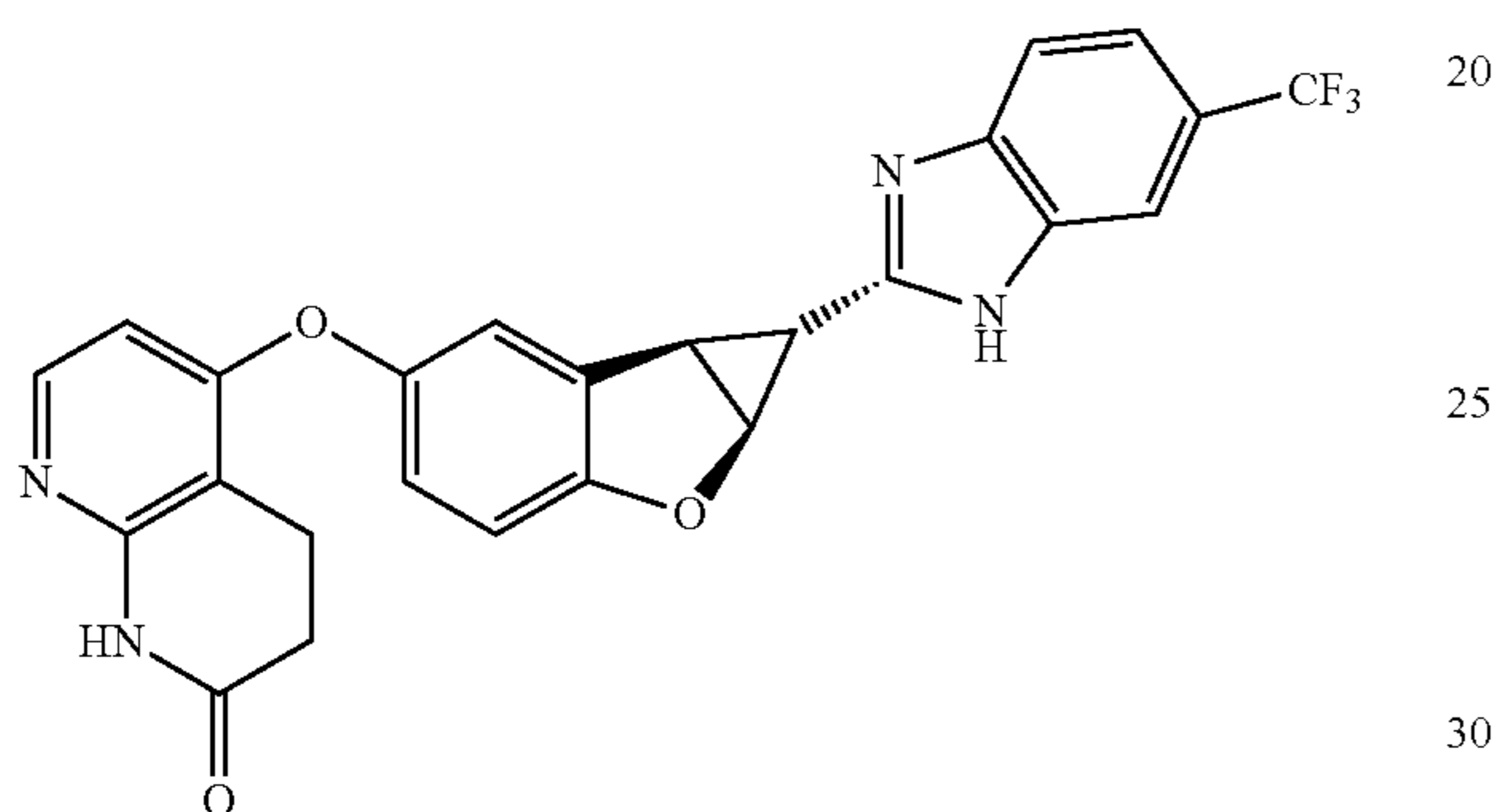
Compound 2.2b
