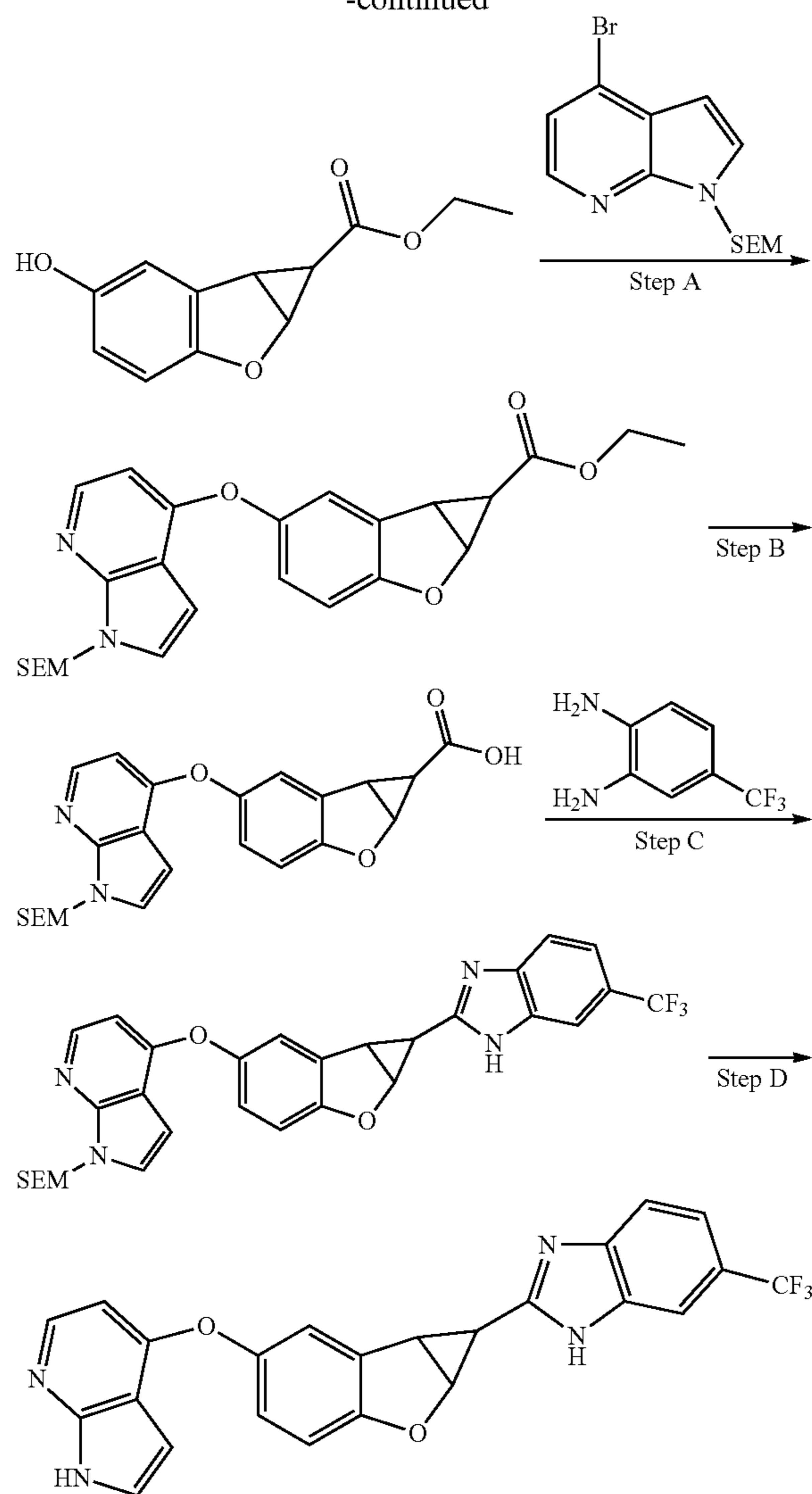
Compound 3.3
