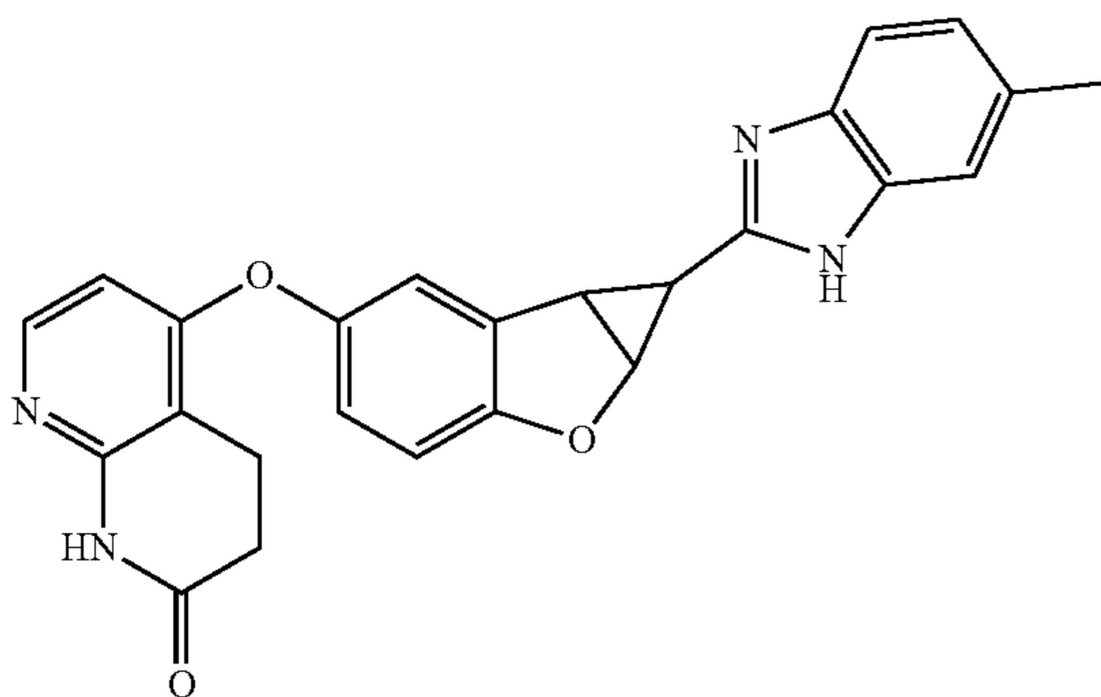
Compound 2.8
