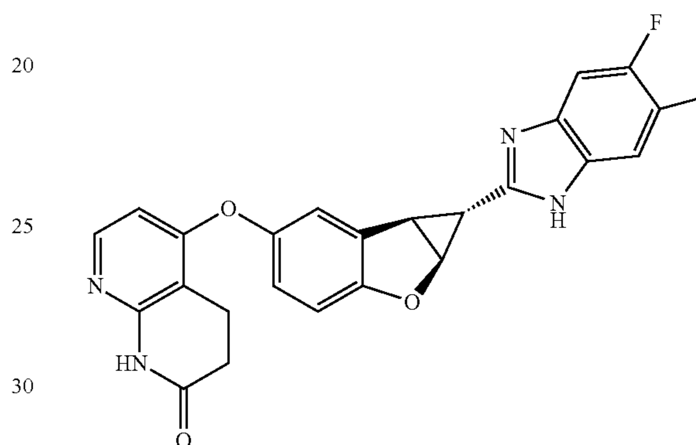
Compound 2.5b
