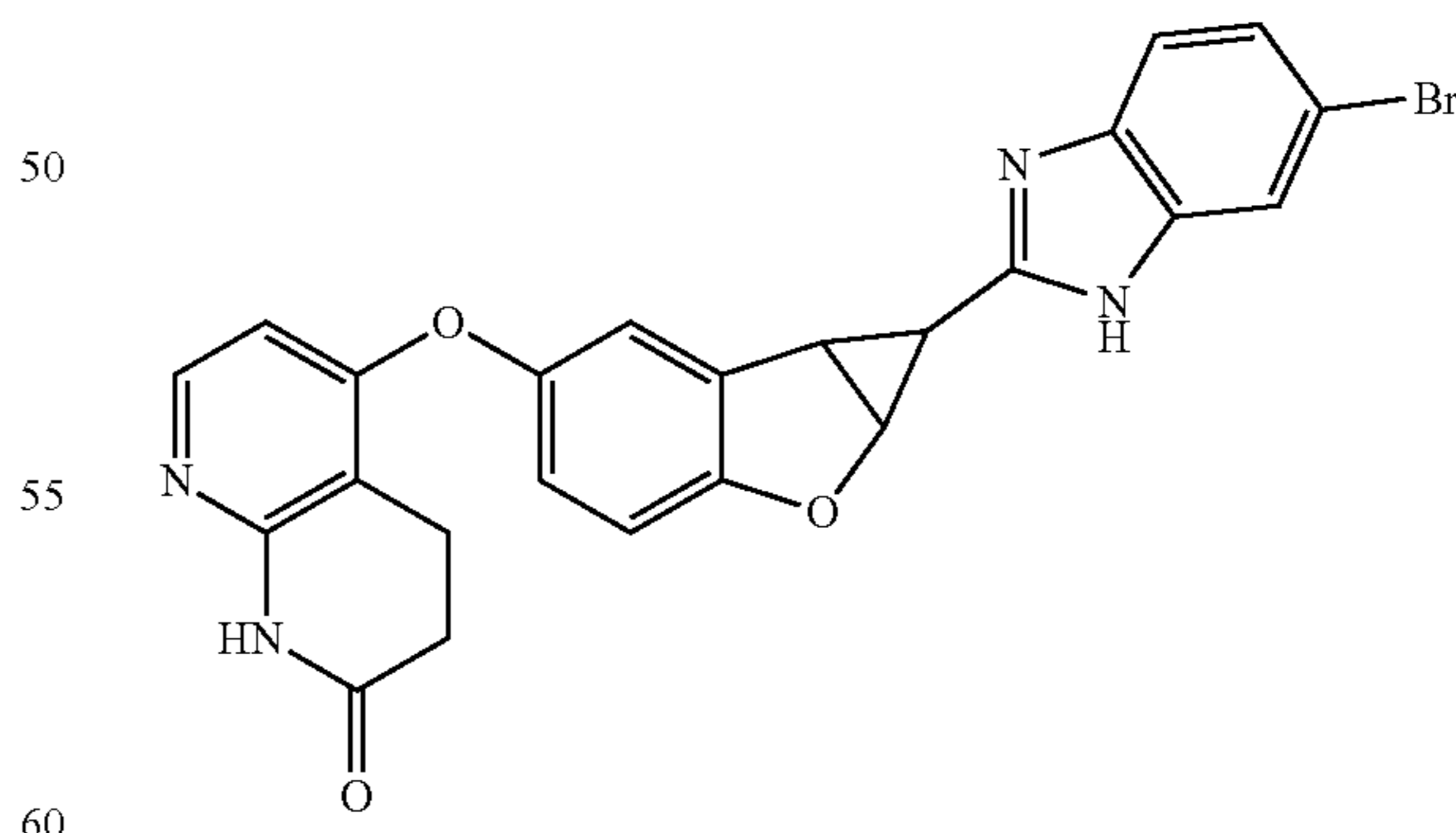
Compound 2.13
