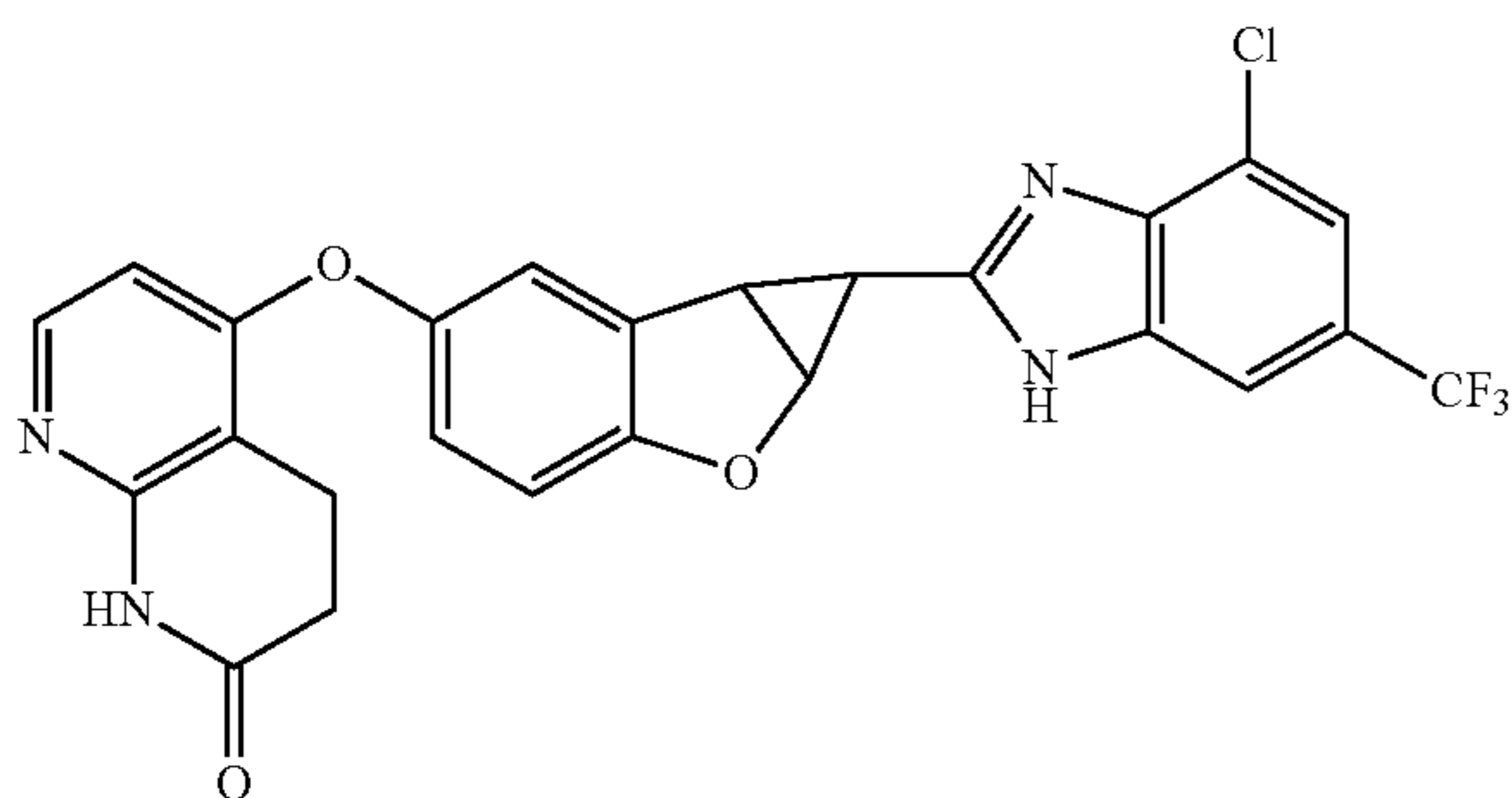
Compound 2.10
