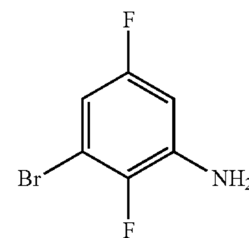
3-bromo-2,5-difluoroaniline
