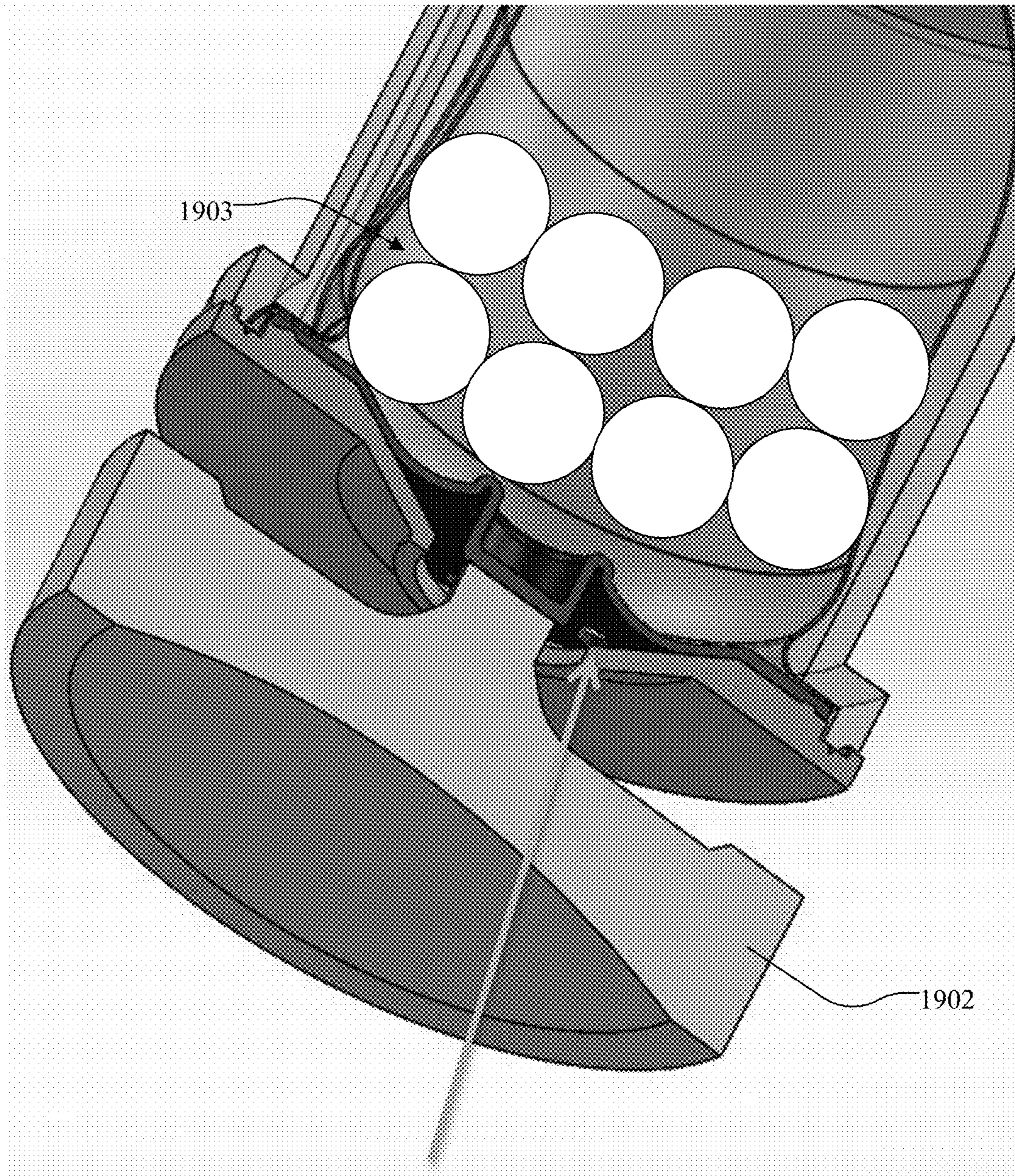
Breaking Mechanism for the Capsule(s)
