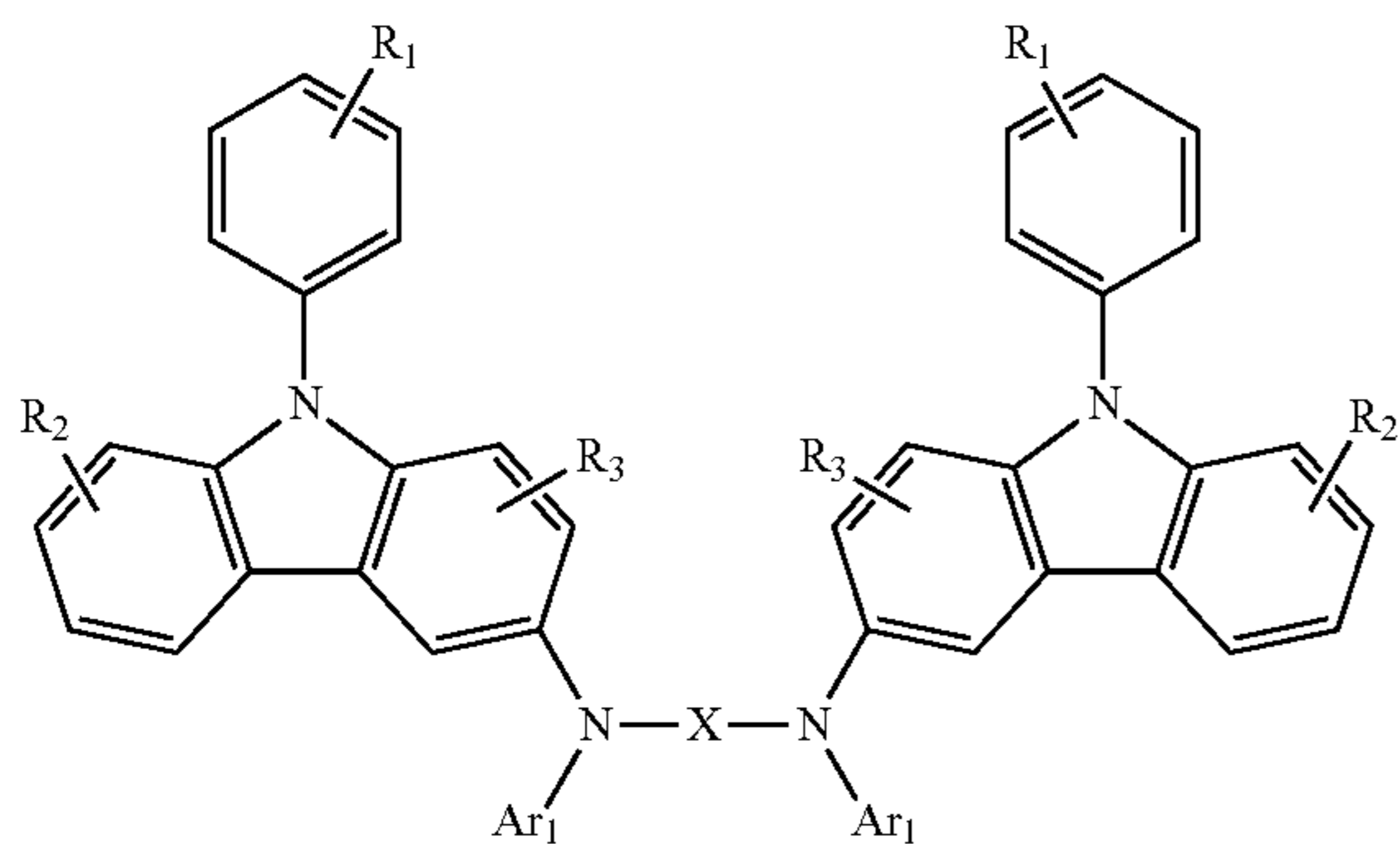
Formula 1
