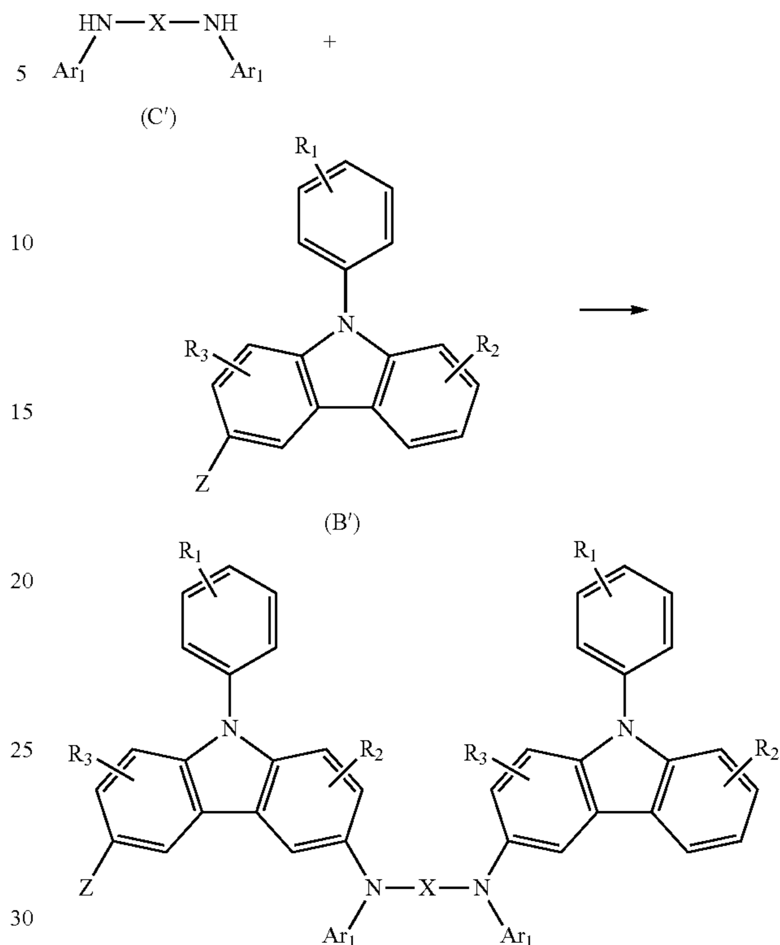
Reaction Scheme 1
