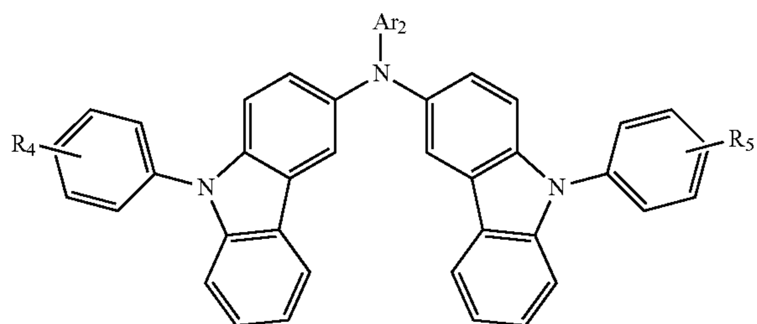
Formula 2
