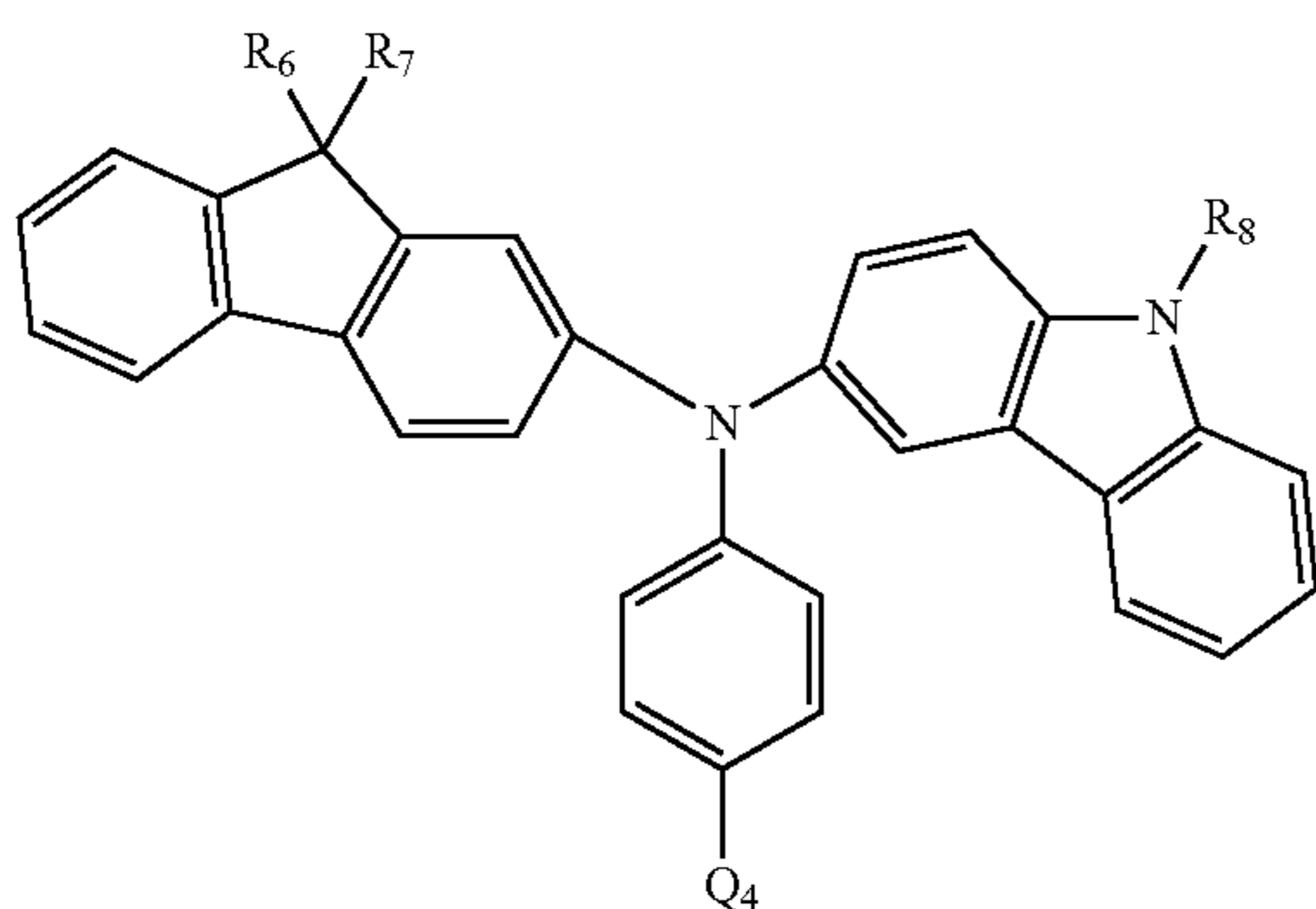
Formula 3a
