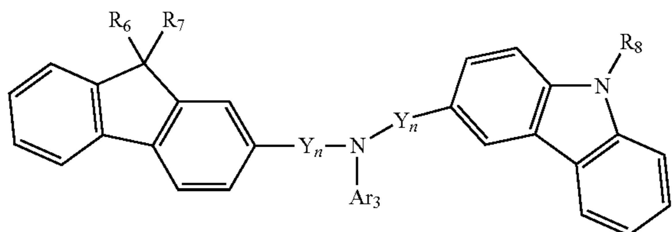
Formula 3
