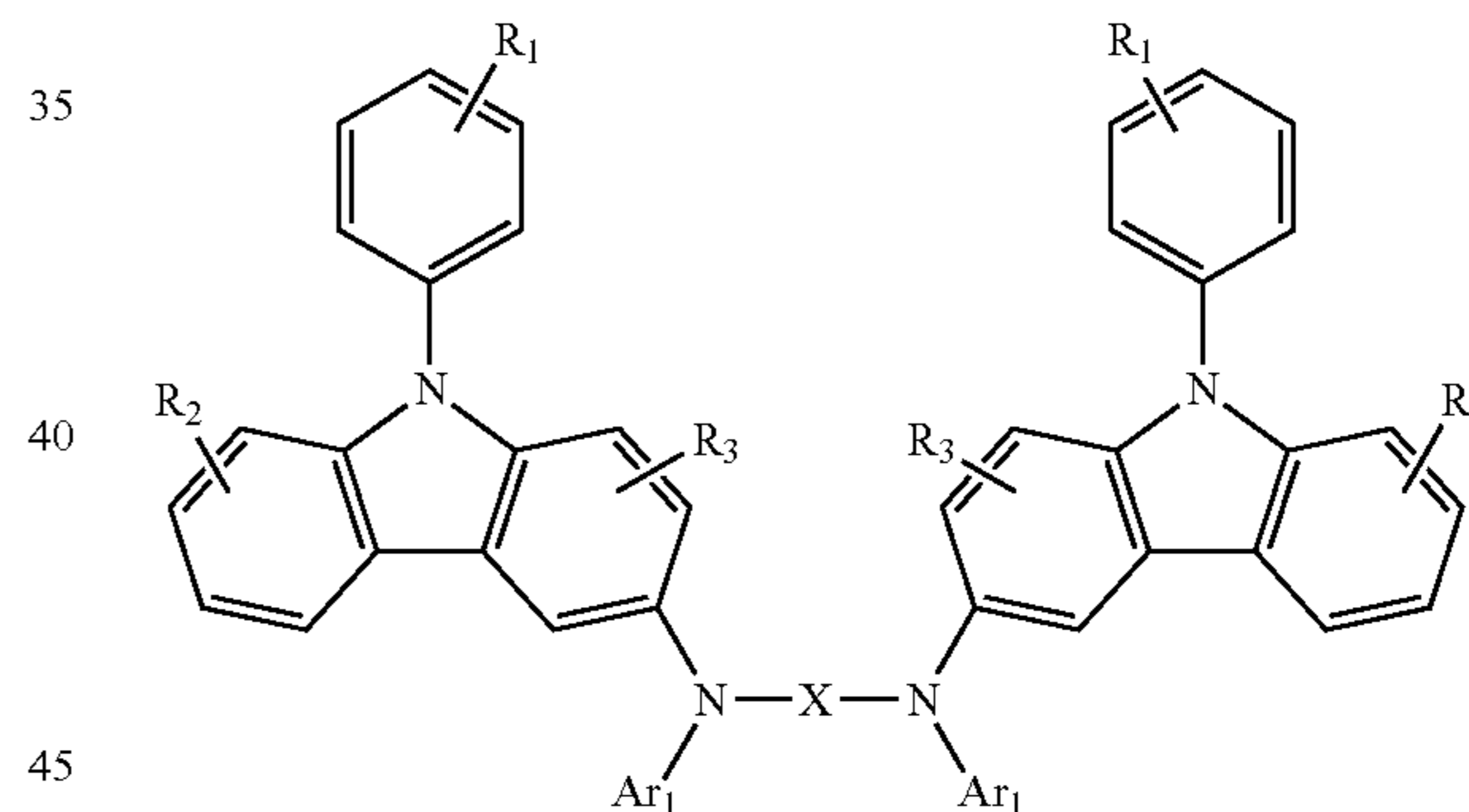
Formula 2
