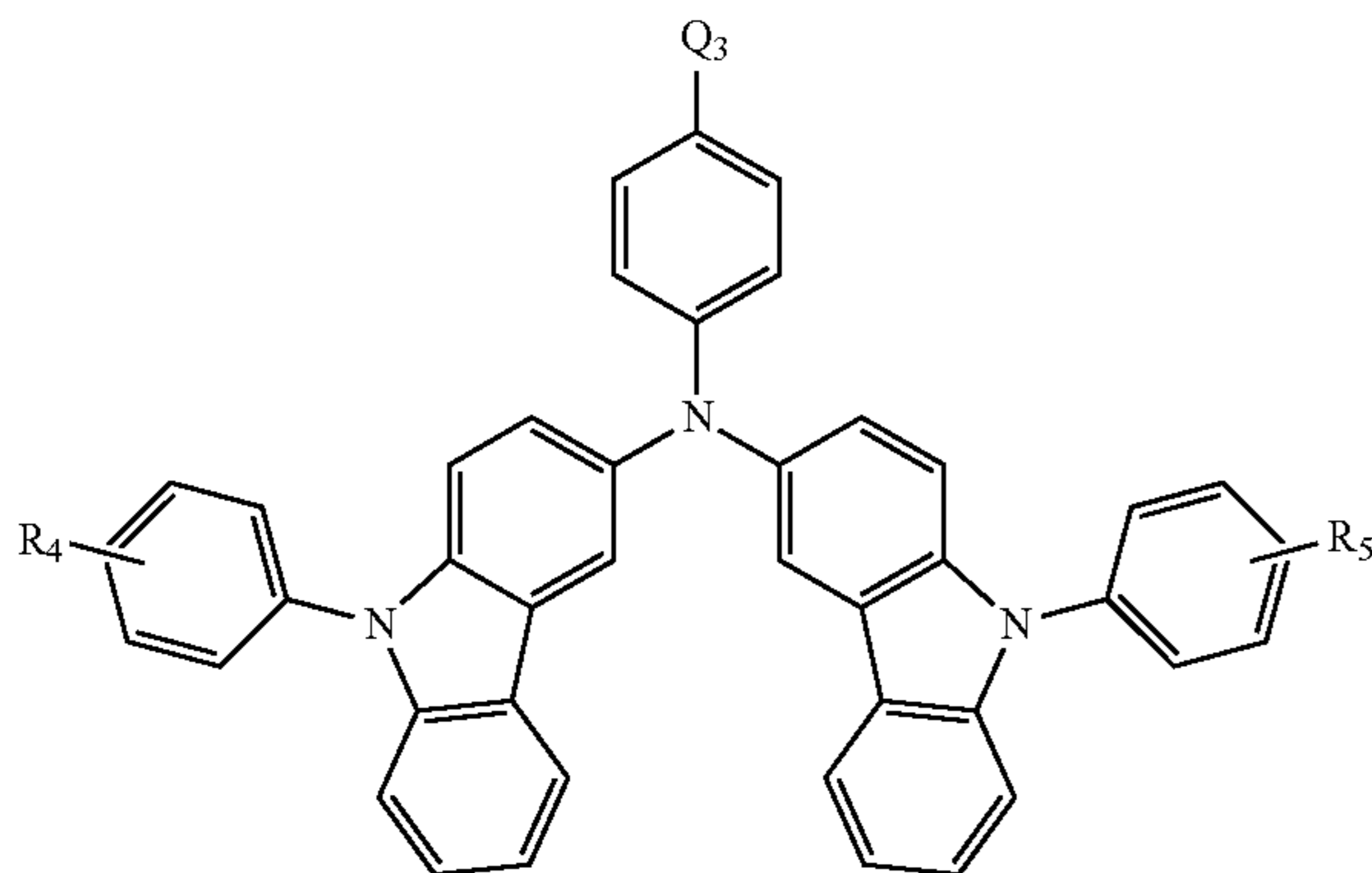
Formula 2a
