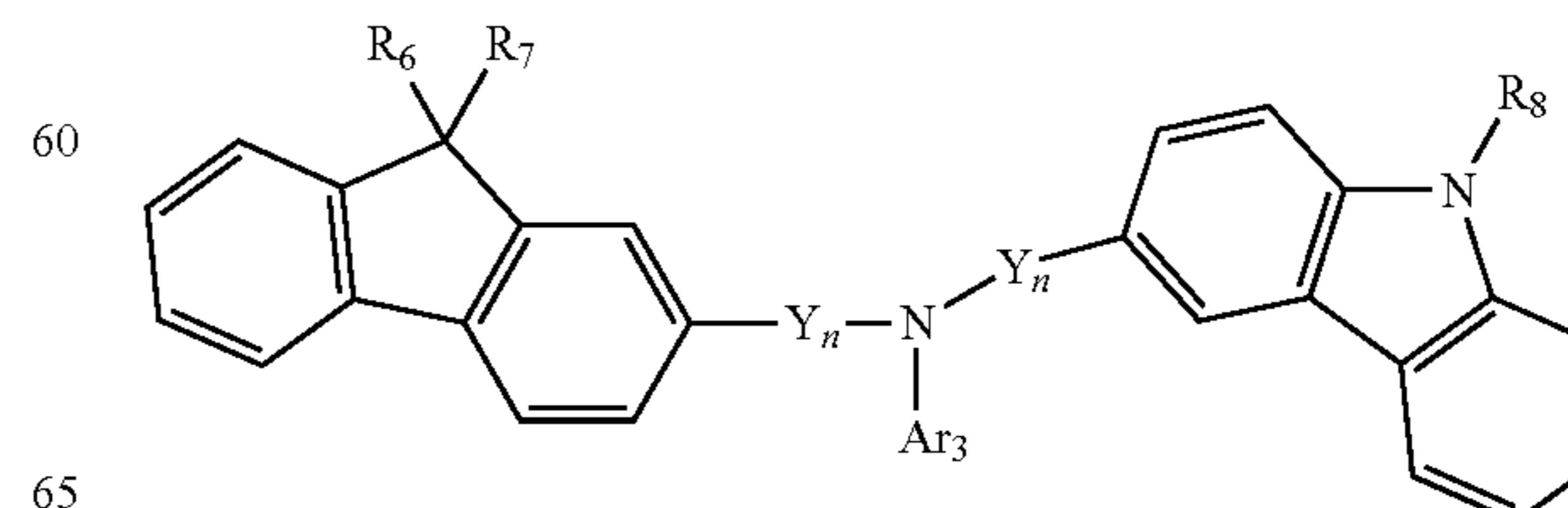
Formula 3
