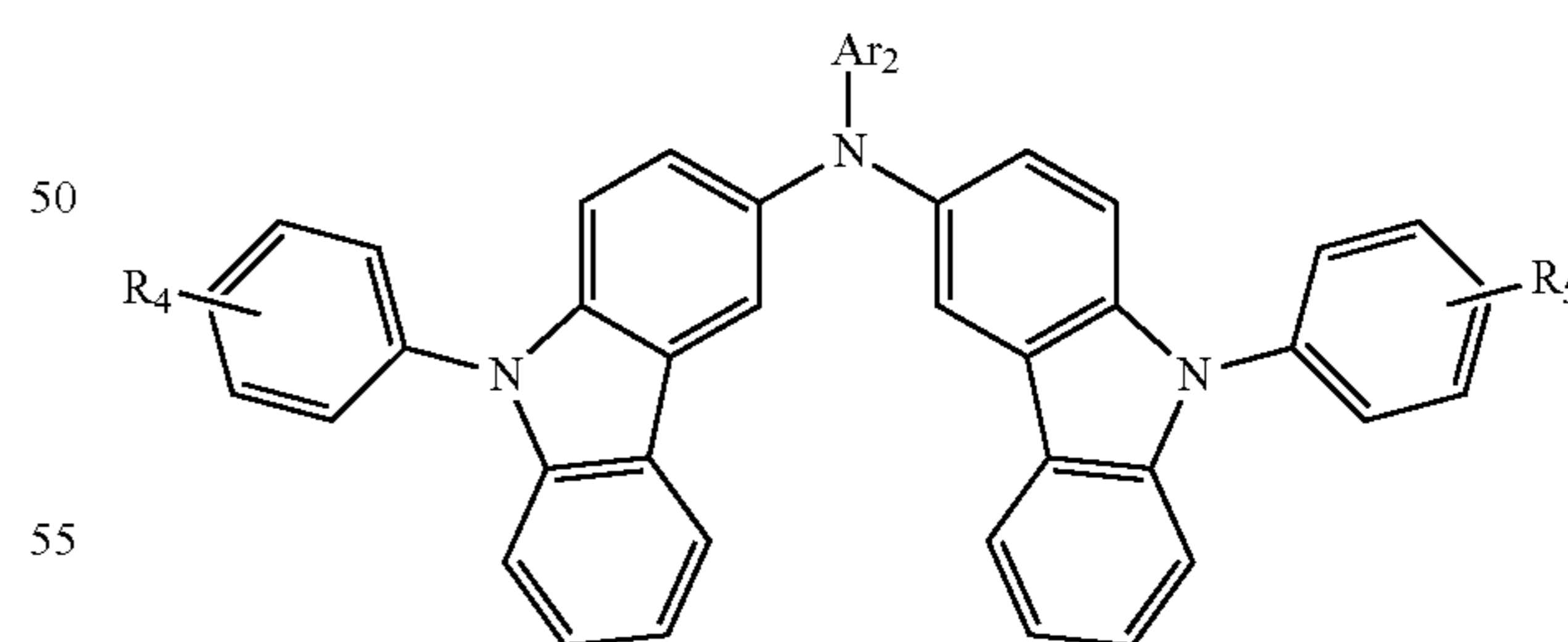
Formula 3
